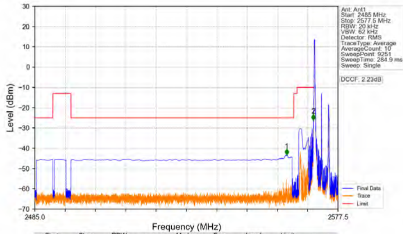
Band38_5MHz_16QAM_LCH_2572.5MHz_RB_1_0_NTNV
