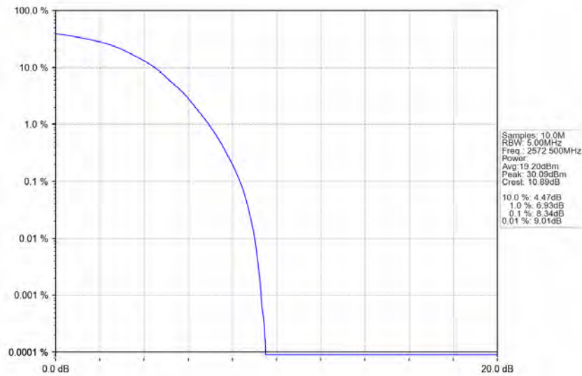
Band38_5MHz_64QAM_LCH_2572.5MHz_RB_25_0_NTNV
