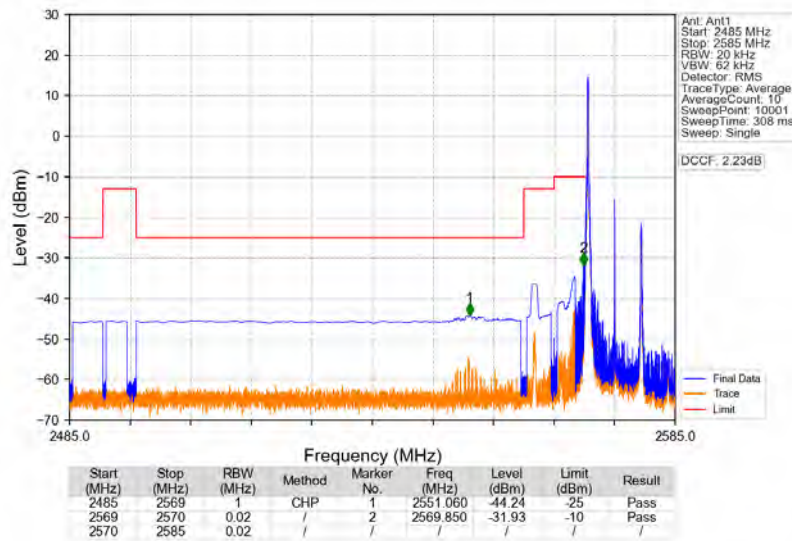
Band38_10MHz_64QAM_LCH_2575MHz_RB_1_0_NTNV
