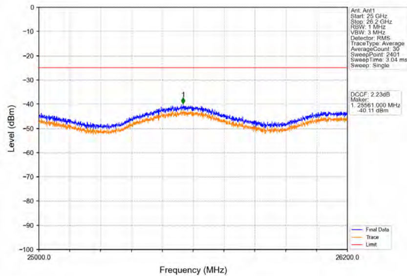
Band38_15MHz_QPSK_MCH_2595MHz_RB_1_0_NTNV
