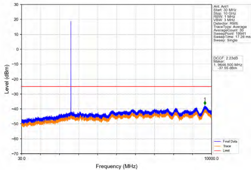
Band38_5MHz_16QAM_HCH_2617.5MHz_RB_1_0_NTNV
