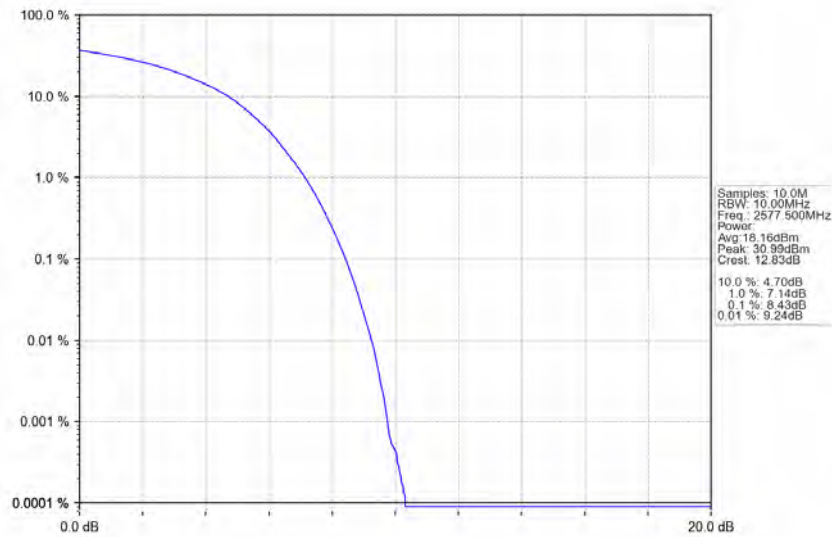
Band38_15MHz_64QAM_LCH_2577.5MHz_RB_75_0_NTNV
