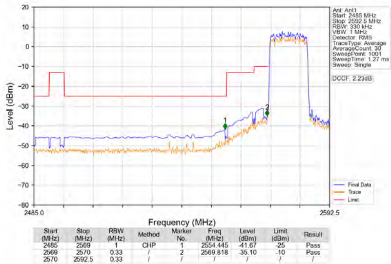
Band38_15MHz_64QAM_LCH_2577.5MHz_RB_75_0_NTNV
