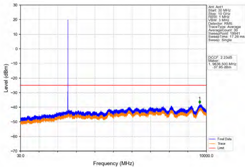
Band38_5MHz_64QAM_LCH_2572.5MHz_RB_1_0_NTNV
