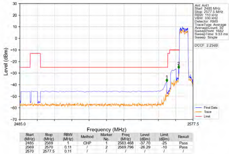
Band38_5MHz_QPSK_LCH_2572.5MHz_RB_25_0_NTNV
