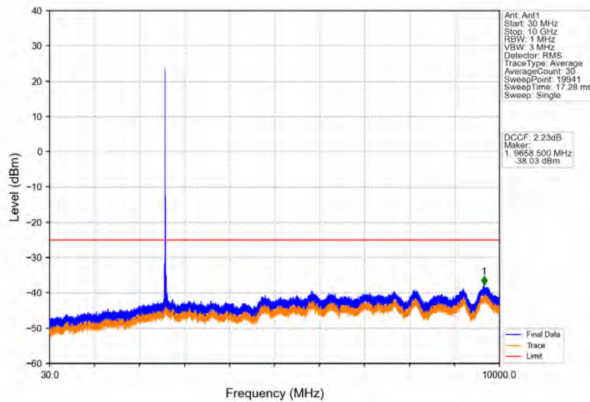
Band38_15MHz_16QAM_MCH_2595MHz_RB_1_0_NTNV
