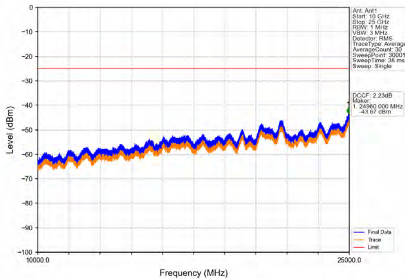
Band38_15MHz_16QAM_LCH_2577.5MHz_RB_1_0_NTNV
