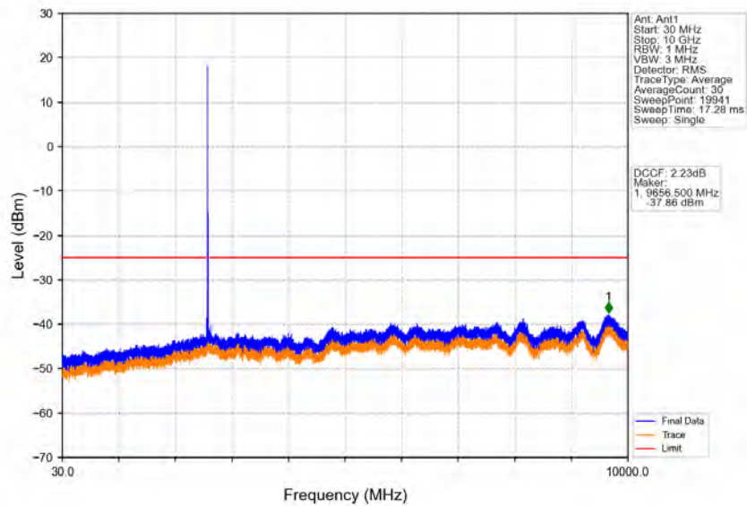
Band38_15MHz_64QAM_MCH_2595MHz_RB_1_0_NTNV
