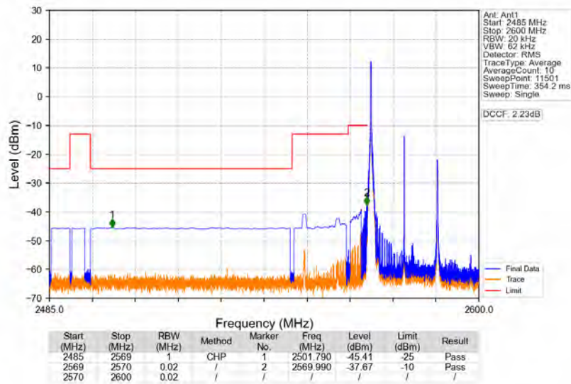
Band38_20MHz_64QAM_LCH_2580MHz_RB_1_0_NTNV
