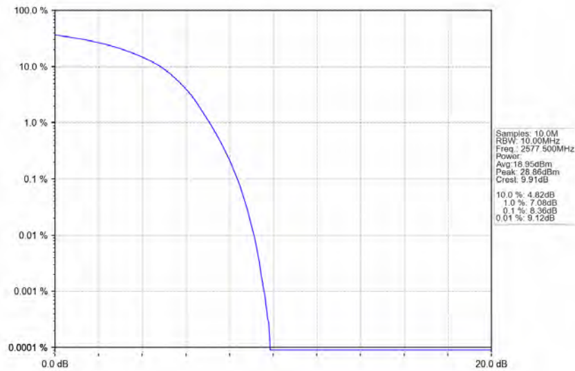
Band38_15MHz_16QAM_LCH_2577.5MHz_RB_75_0_NTNV
