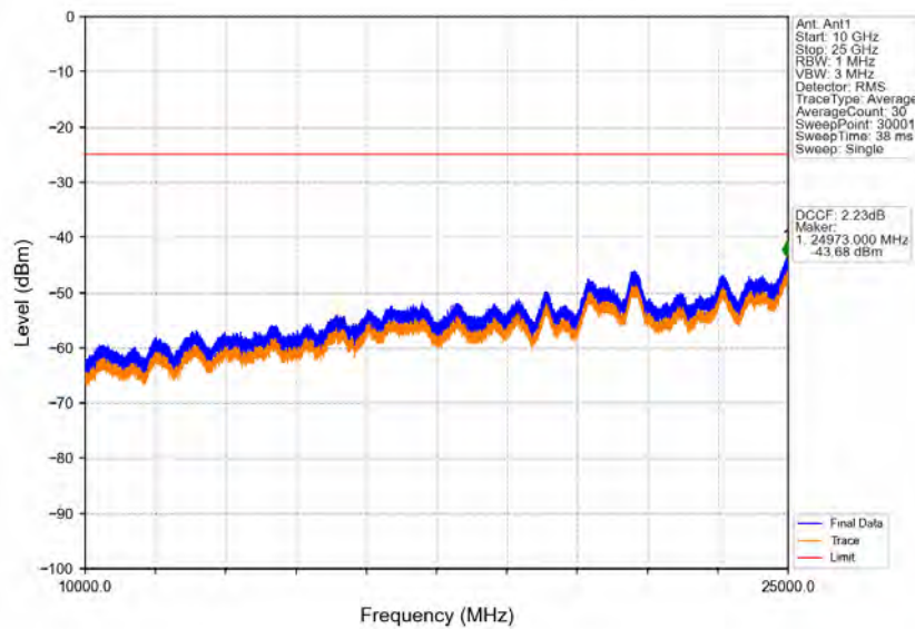
Band38_15MHz_64QAM_HCH_2612.5MHz_RB_1_0_NTNV
