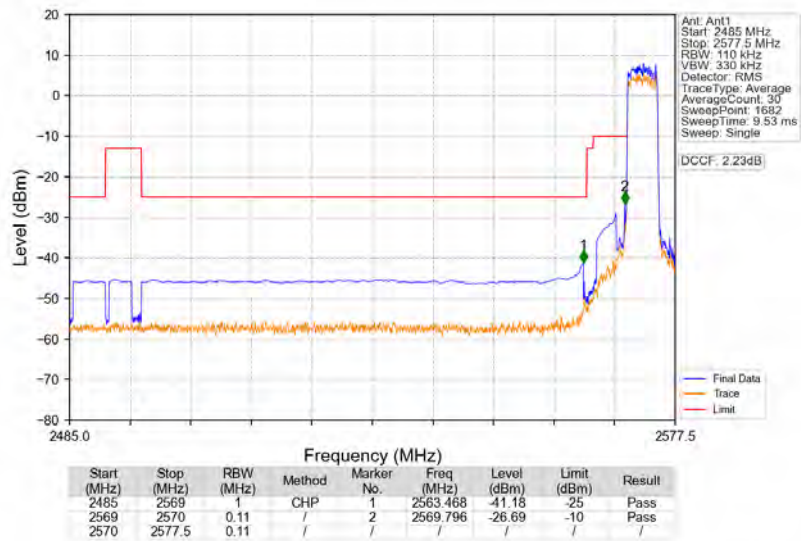
Band38_5MHz_64QAM_LCH_2572.5MHz_RB_25_0_NTNV
