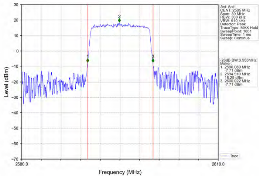
Band38_10MHz_16QAM_MCH_2595MHz_RB_50_0_NTNV
