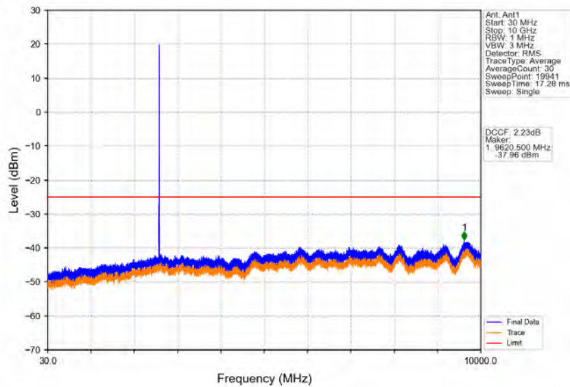
Band38_5MHz_16QAM_MCH_2595MHz_RB_1_0_NTNV
