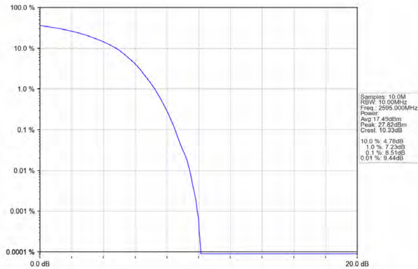
Band38_15MHz_64QAM_MCH_2595MHz_RB_75_0_NTNV
