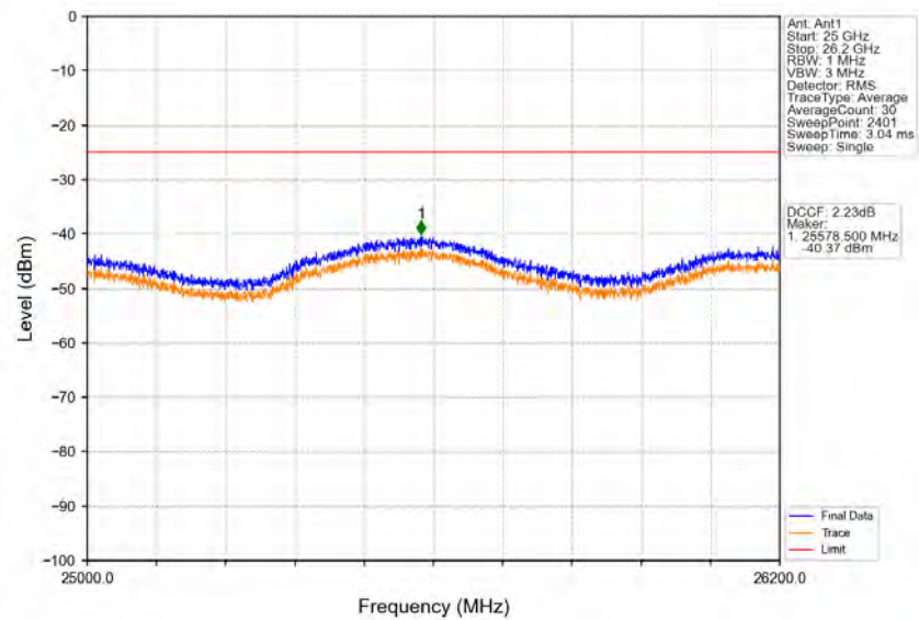
Band38_5MHz_16QAM_LCH_2572.5MHz_RB_25_0_NTNV
