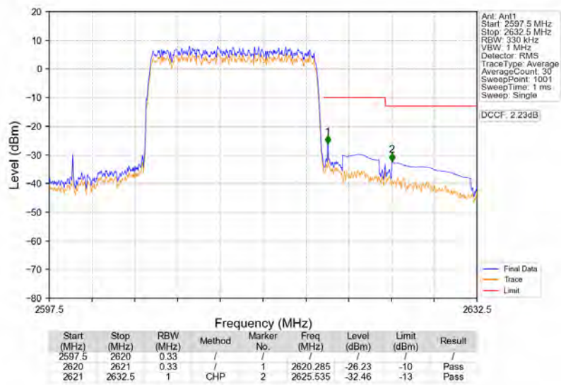
Band38_15MHz_16QAM_HCH_2612.5MHz_RB_75_0_NTNV
