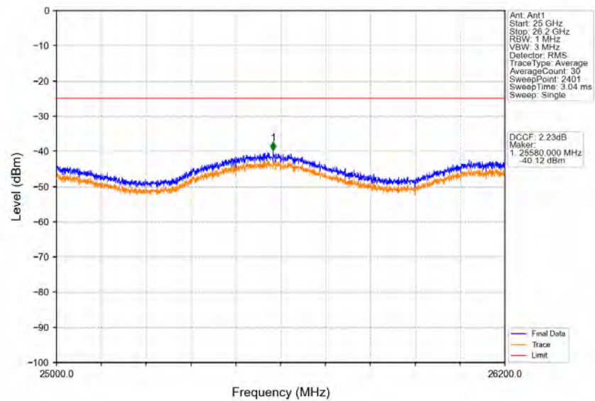
Band38_10MHz_16QAM_HCH_2615MHz_RB_1_0_NTNV
