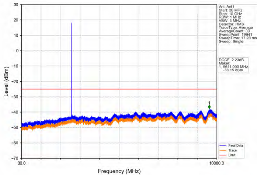
Band38_5MHz_16QAM_LCH_2572.5MHz_RB_1_0_NTNV
