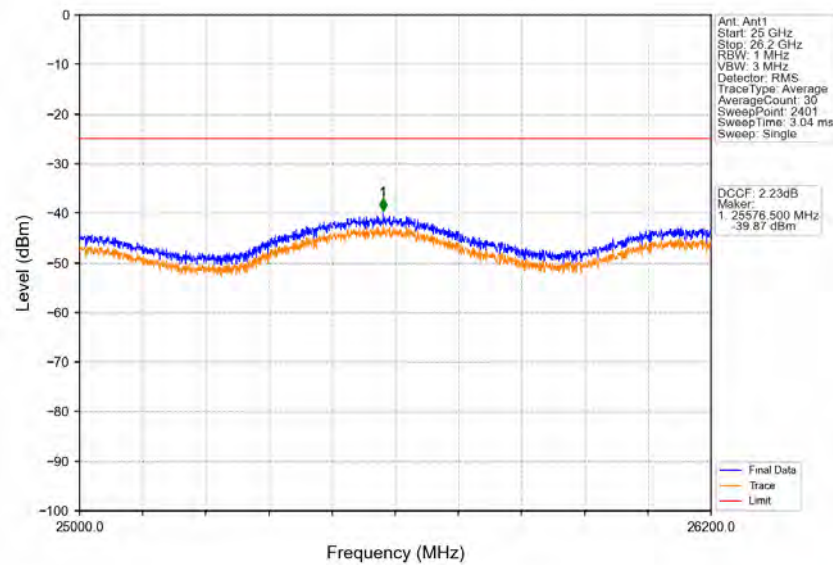
Band38_5MHz_16QAM_HCH_2617.5MHz_RB_1_0_NTNV
