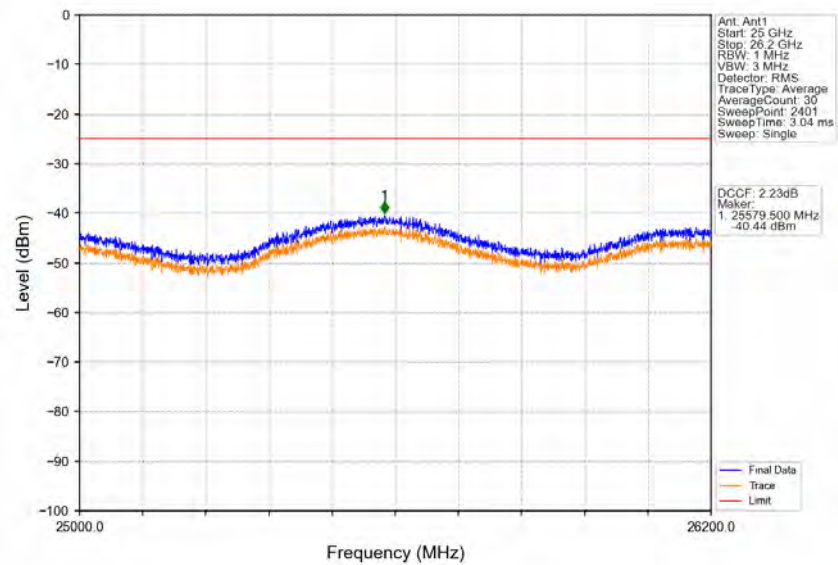
Band38_15MHz_16QAM_HCH_2612.5MHz_RB_1_0_NTNV
