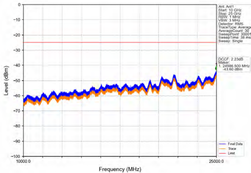
Band38_5MHz_16QAM_LCH_2572.5MHz_RB_1_0_NTNV
