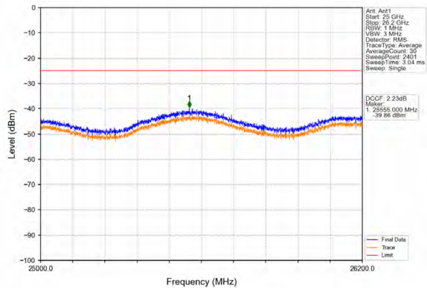
Band38_15MHz_QPSK_HCH_2612.5MHz_RB_1_74_NTNV
