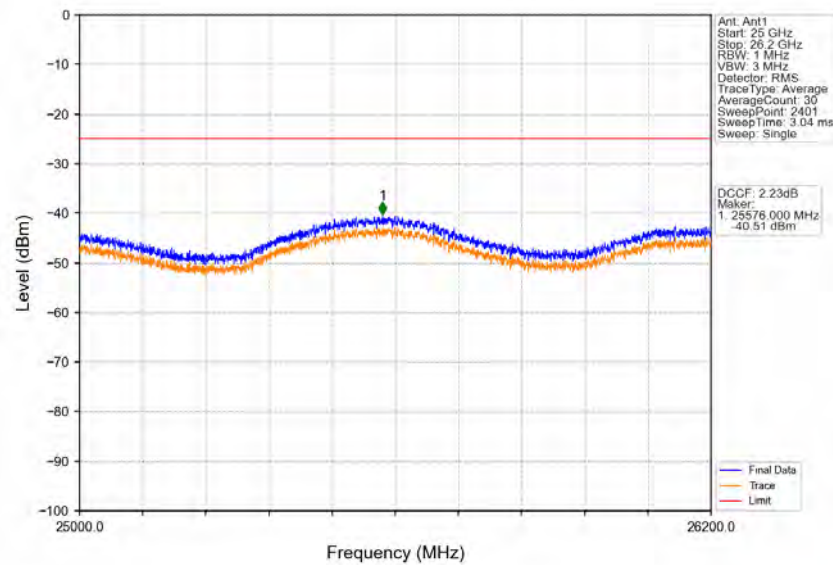
Band38_5MHz_64QAM_MCH_2595MHz_RB_1_0_NTNV
