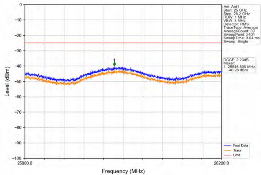
Band38_10MHz_16QAM_LCH_2575MHz_RB_50_0_NTNV
