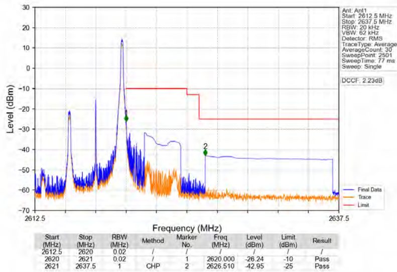
Band38_5MHz_16QAM_HCH_2617.5MHz_RB_1_24_NTNV
