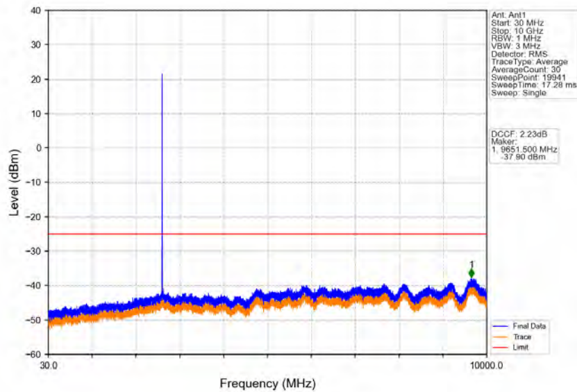
Band38_5MHz_QPSK_HCH_2617.5MHz_RB_1_0_NTNV
