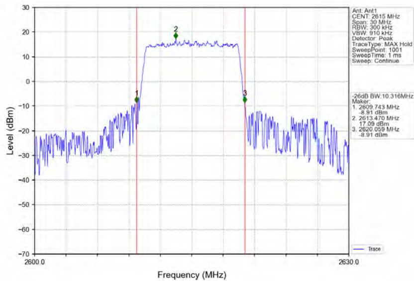
Band38_10MHz_64QAM_HCH_2615MHz_RB_50_0_NTNV
