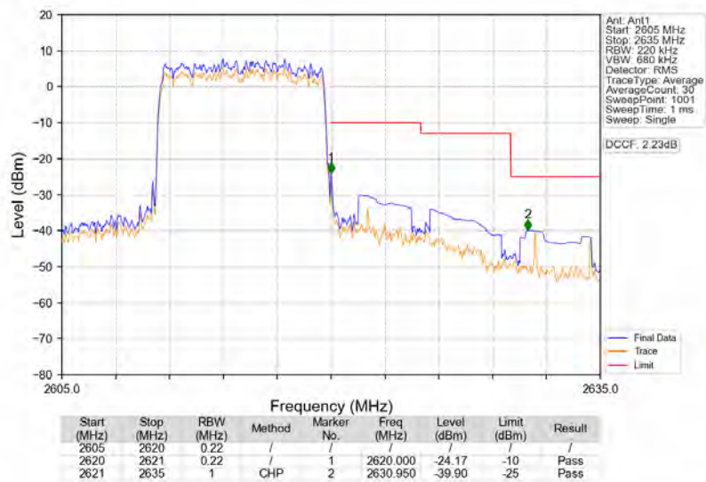
Band38_10MHz_16QAM_HCH_2615MHz_RB_50_0_NTNV
