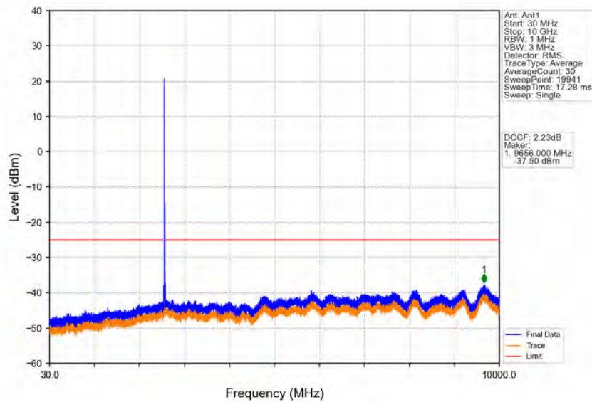
Band38_15MHz_16QAM_LCH_2577.5MHz_RB_1_0_NTNV
