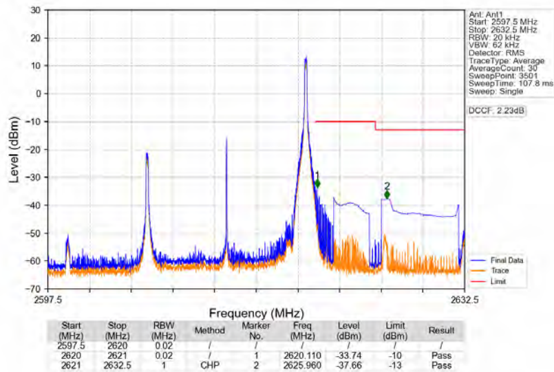
Band38_15MHz_64QAM_HCH_2612.5MHz_RB_1_74_NTNV
