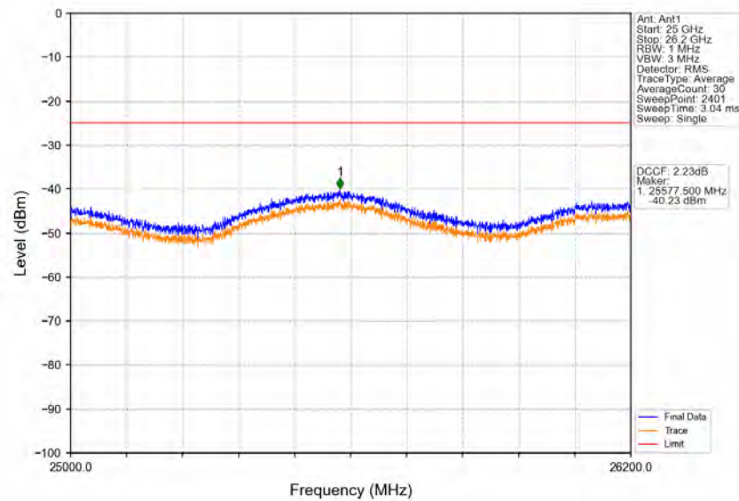
Band38_10MHz_16QAM_HCH_2615MHz_RB_1_0_NTNV
