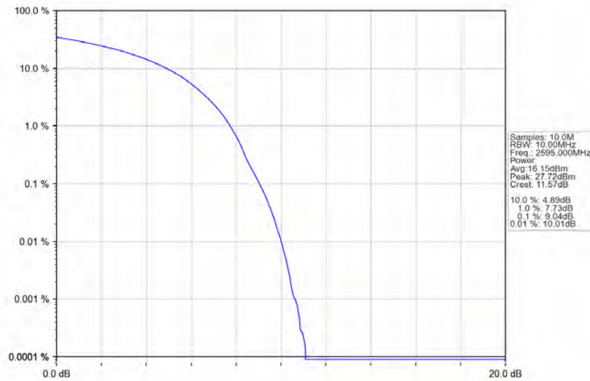
Band38_20MHz_64QAM_MCH_2595MHz_RB_100_0_NTNV
