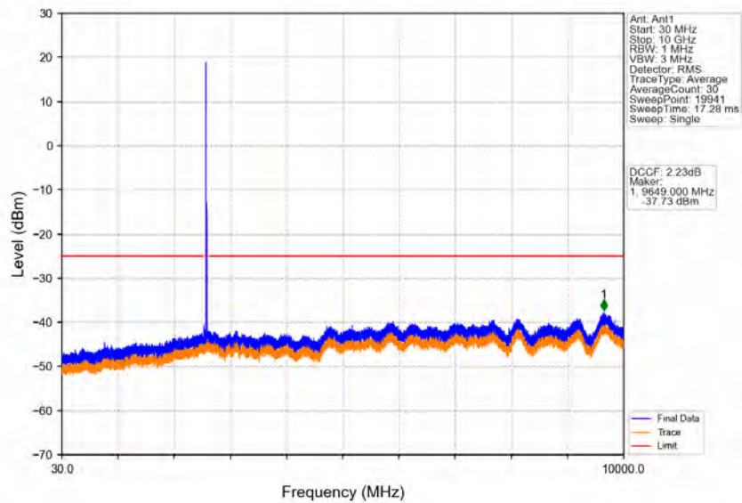
Band38_20MHz_64QAM_MCH_2595MHz_RB_1_0_NTNV
