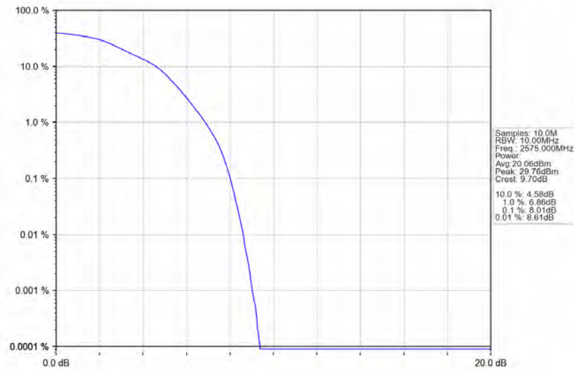
Band38_10MHz_16QAM_LCH_2575MHz_RB_50_0_NTNV
