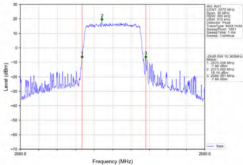
Band38_10MHz_64QAM_LCH_2575MHz_RB_50_0_NTNV
