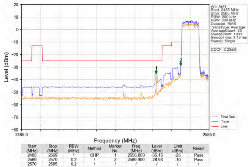
Band38_10MHz_16QAM_LCH_2575MHz_RB_50_0_NTNV
