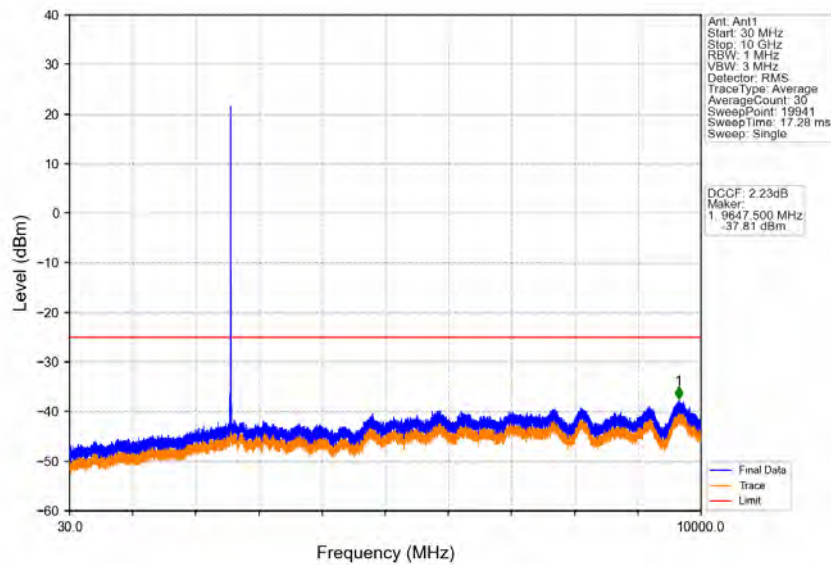
Band38_10MHz_16QAM_LCH_2575MHz_RB_1_0_NTNV
