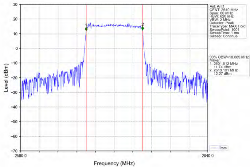
Band38_20MHz_64QAM_HCH_2610MHz_RB_100_0_NTNV
