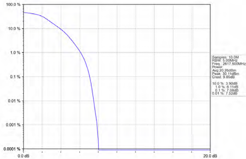
Band38_5MHz_QPSK_HCH_2617.5MHz_RB_25_0_NTNV
