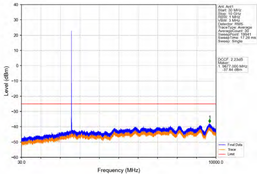
Band38_10MHz_64QAM_MCH_2595MHz_RB_1_0_NTNV
