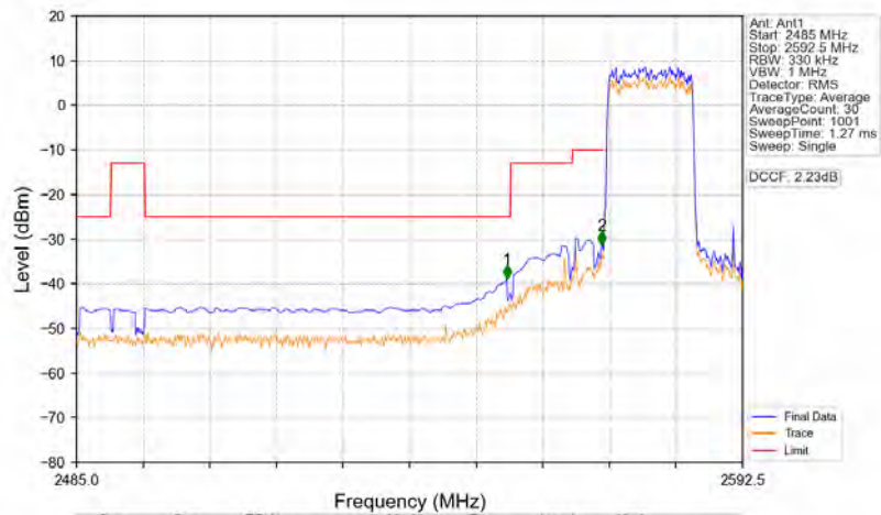
Band38_15MHz_16QAM_LCH_2577.5MHz_RB_75_0_NTNV
