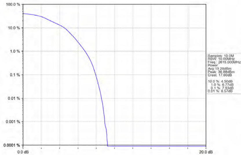
Band38_10MHz_16QAM_HCH_2615MHz_RB_50_0_NTNV
