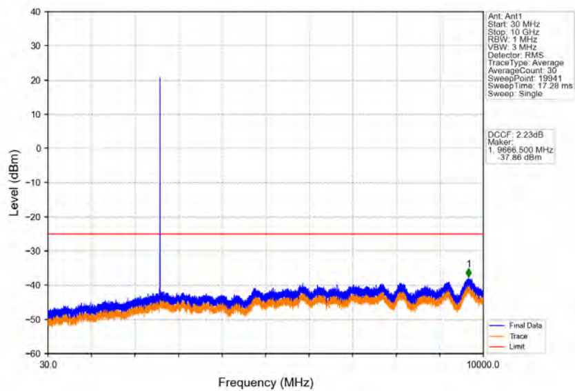
Band38_5MHz_64QAM_MCH_2595MHz_RB_1_0_NTNV
