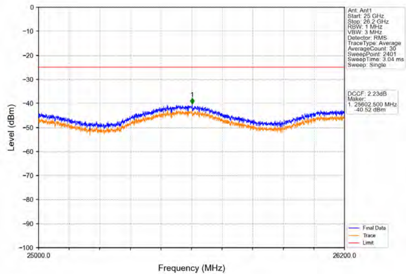
Band38_15MHz_16QAM_LCH_2577.5MHz_RB_75_0_NTNV
