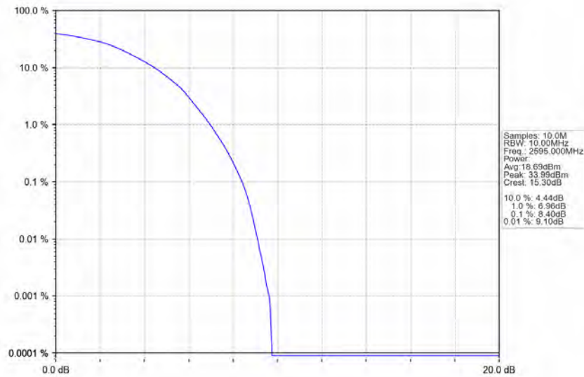
Band38_10MHz_64QAM_MCH_2595MHz_RB_50_0_NTNV
