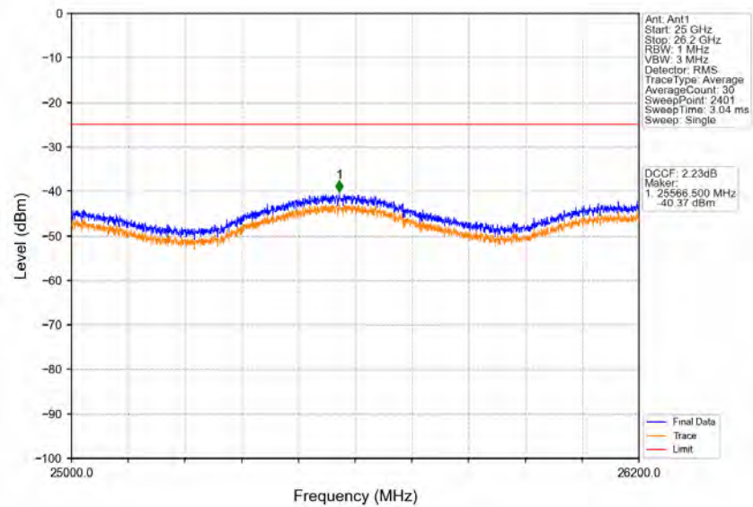
Band38_5MHz_16QAM_HCH_2617.5MHz_RB_1_0_NTNV
