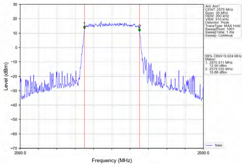
Band38_10MHz_64QAM_LCH_2575MHz_RB_50_0_NTNV
