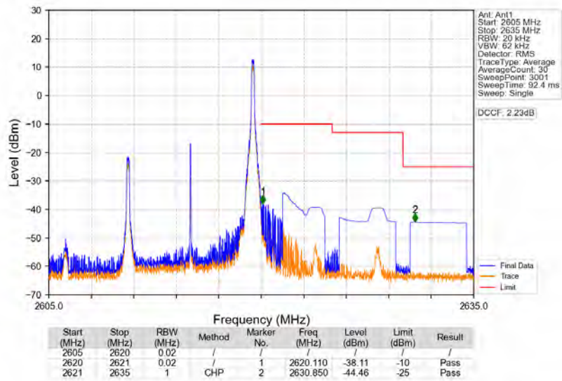
Band38_10MHz_64QAM_HCH_2615MHz_RB_1_49_NTNV
