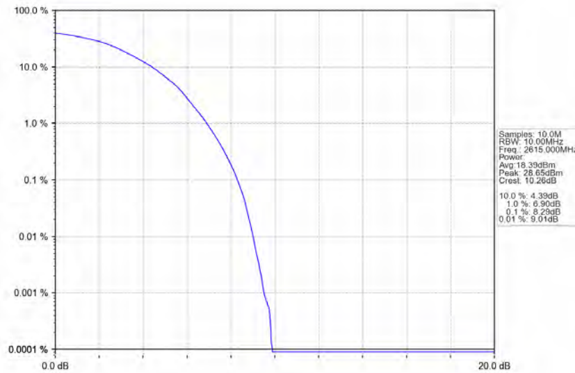
Band38_10MHz_64QAM_HCH_2615MHz_RB_50_0_NTNV
