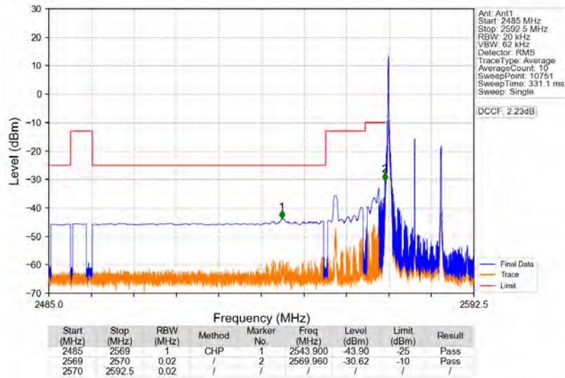
Band38_15MHz_16QAM_LCH_2577.5MHz_RB_1_0_NTNV
