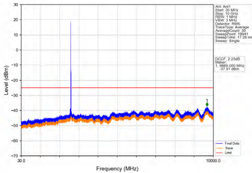
Band38_20MHz_64QAM_HCH_2610MHz_RB_1_0_NTNV
