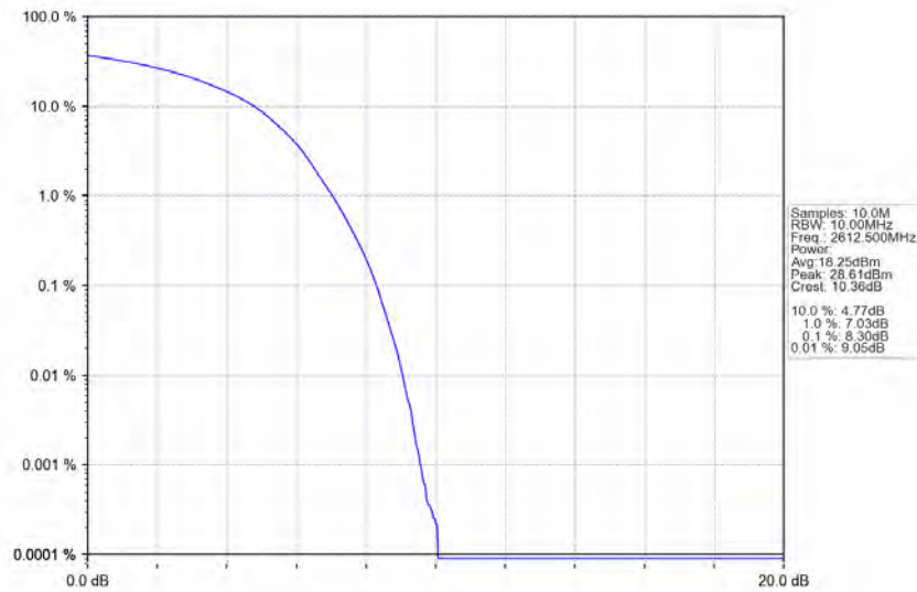
Band38_15MHz_16QAM_HCH_2612.5MHz_RB_75_0_NTNV
