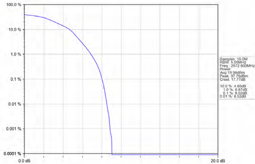
Band38_5MHz_16QAM_LCH_2572.5MHz_RB_25_0_NTNV
