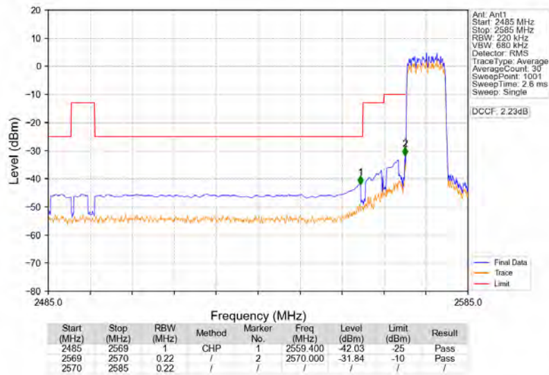
Band38_10MHz_64QAM_LCH_2575MHz_RB_50_0_NTNV
