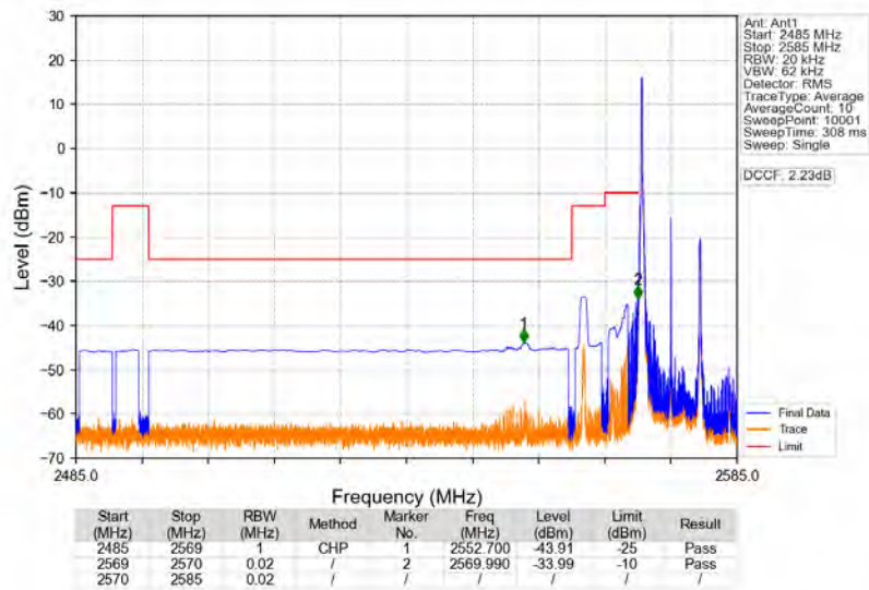
Band38_10MHz_16QAM_LCH_2575MHz_RB_1_0_NTNV
