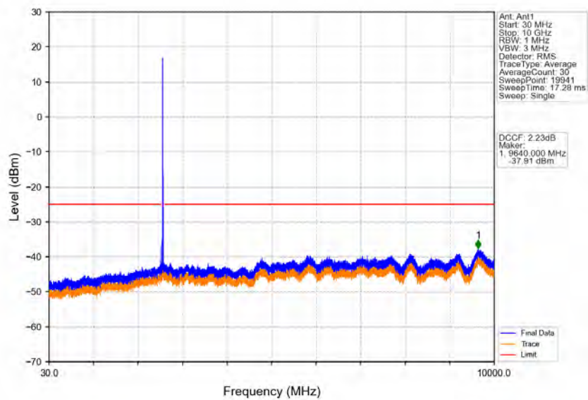
Band38_20MHz_64QAM_LCH_2580MHz_RB_1_0_NTNV
