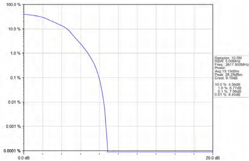
Band38_5MHz_16QAM_HCH_2617.5MHz_RB_25_0_NTNV
