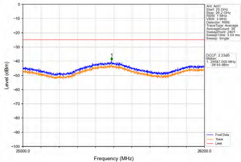
Band38_15MHz_64QAM_HCH_2612.5MHz_RB_1_74_NTNV
