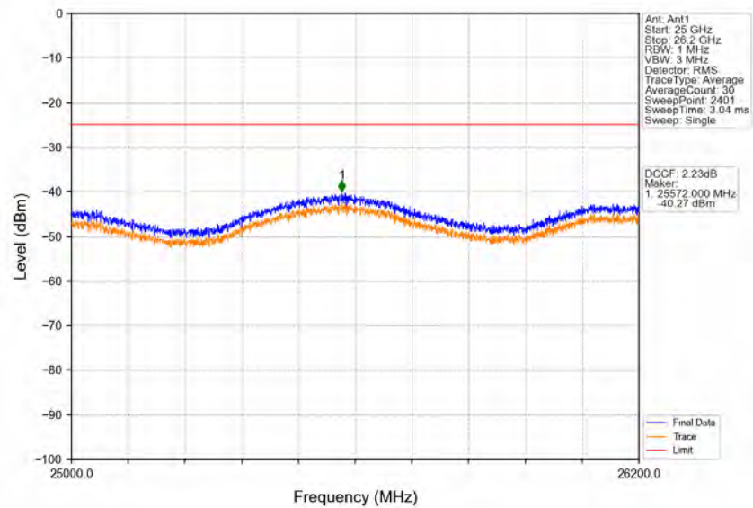
Band38_5MHz_64QAM_HCH_2617.5MHz_RB_1_24_NTNV
