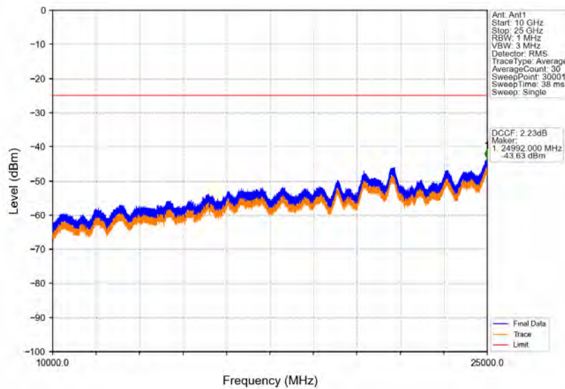
Band38_5MHz_16QAM_MCH_2595MHz_RB_1_0_NTNV
