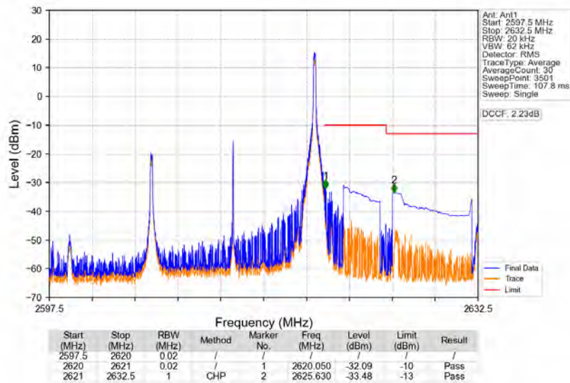
Band38_15MHz_QPSK_HCH_2612.5MHz_RB_1_74_NTNV
