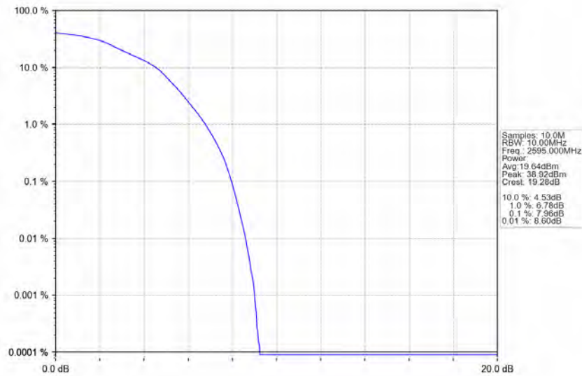
Band38_10MHz_16QAM_MCH_2595MHz_RB_50_0_NTNV
