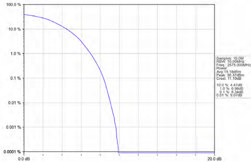
Band38_10MHz_64QAM_LCH_2575MHz_RB_50_0_NTNV
