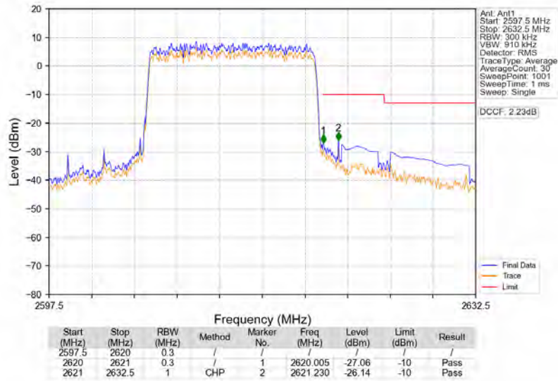
Band38_15MHz_QPSK_HCH_2612.5MHz_RB_75_0_NTNV
