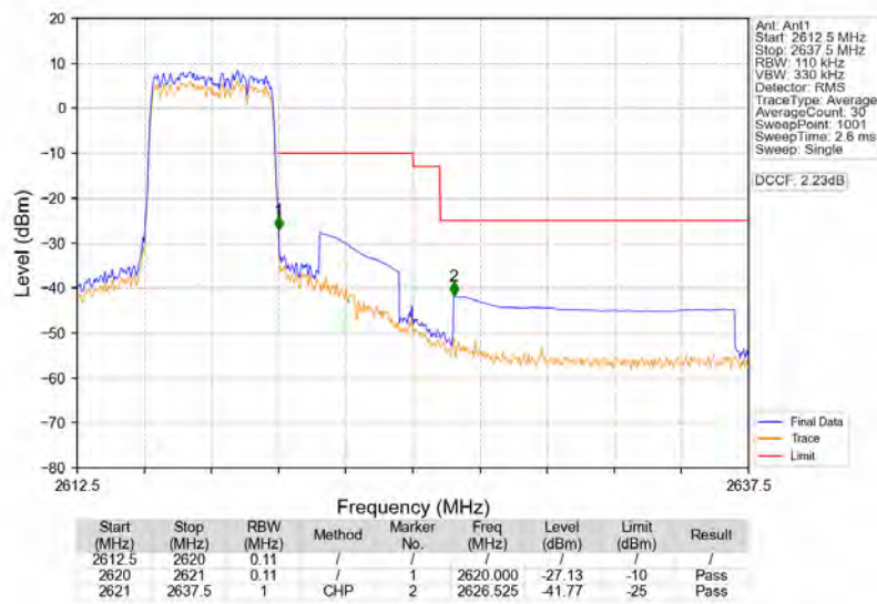
Band38_5MHz_16QAM_HCH_2617.5MHz_RB_25_0_NTNV
