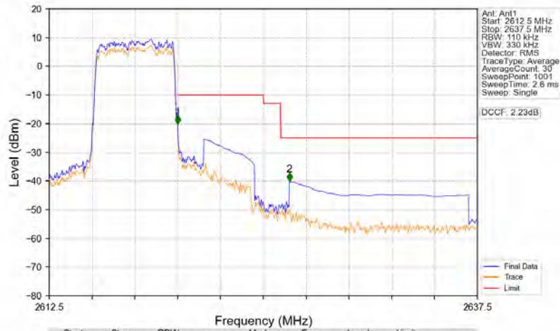
Band38_5MHz_QPSK_HCH_2617.5MHz_RB_25_0_NTNV
