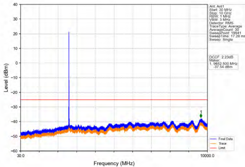
Band38_15MHz_64QAM_HCH_2612.5MHz_RB_1_0_NTNV
