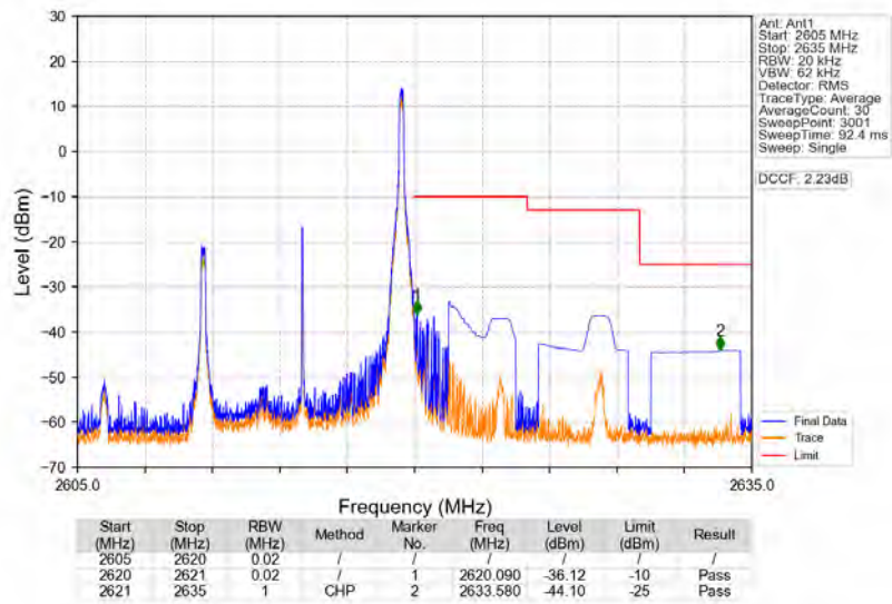
Band38_10MHz_16QAM_HCH_2615MHz_RB_1_49_NTNV
