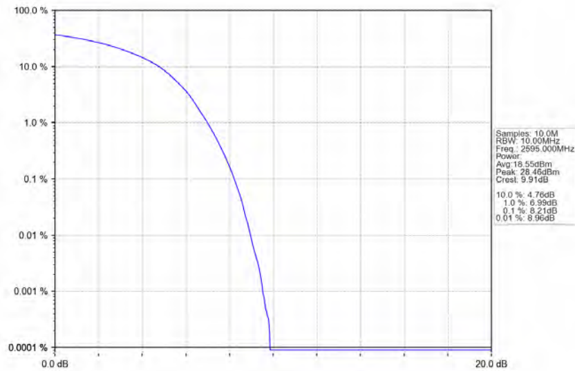
Band38_15MHz_16QAM_MCH_2595MHz_RB_75_0_NTNV
