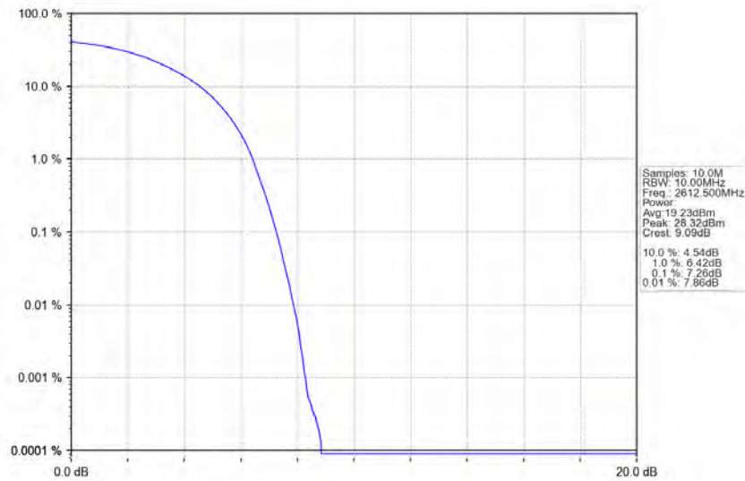
Band38_15MHz_QPSK_HCH_2612.5MHz_RB_75_0_NTNV
