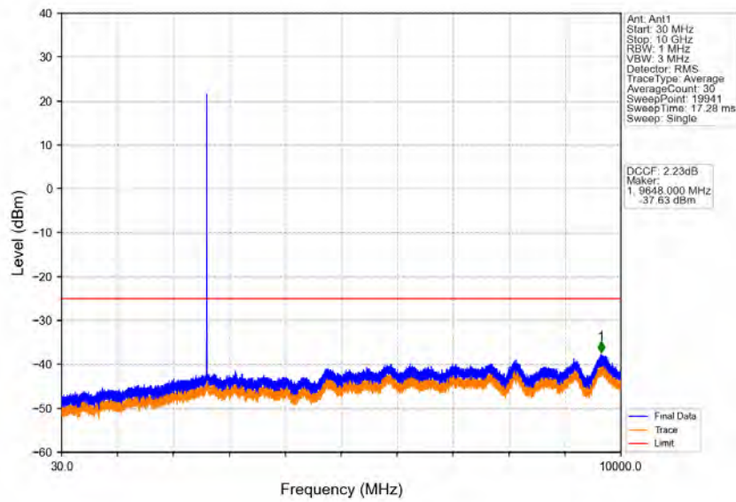
Band38_5MHz_64QAM_HCH_2617.5MHz_RB_1_0_NTNV
