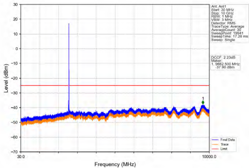
Band38_15MHz_64QAM_LCH_2577.5MHz_RB_1_0_NTNV
