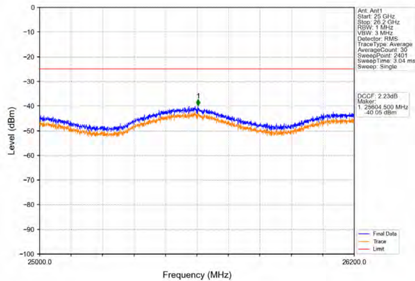
Band38_15MHz_QPSK_LCH_2577.5MHz_RB_1_0_NTNV
