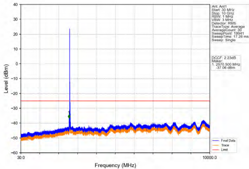
Band38_15MHz_16QAM_HCH_2612.5MHz_RB_1_0_NTNV
