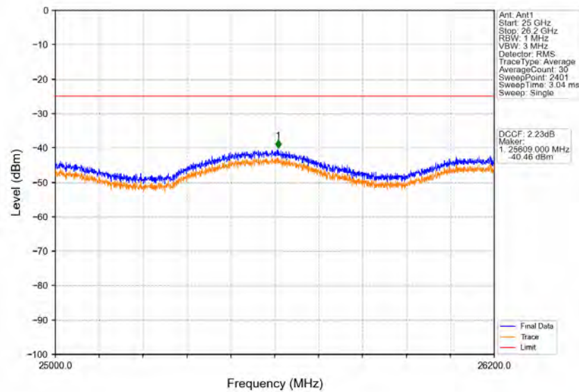
Band38_20MHz_64QAM_LCH_2580MHz_RB_1_0_NTNV
