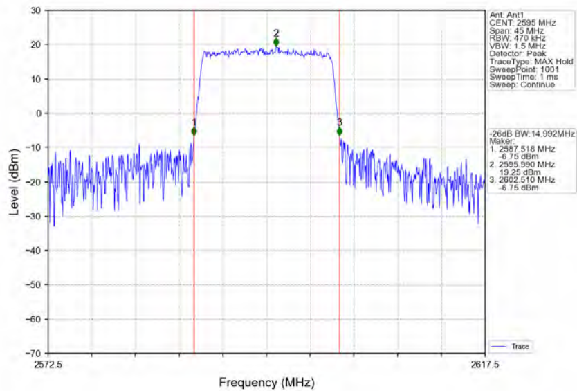
Band38_15MHz_QPSK_MCH_2595MHz_RB_75_0_NTNV
