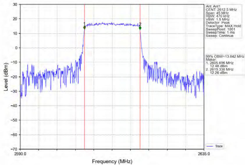
Band38_15MHz_16QAM_HCH_2612.5MHz_RB_75_0_NTNV
