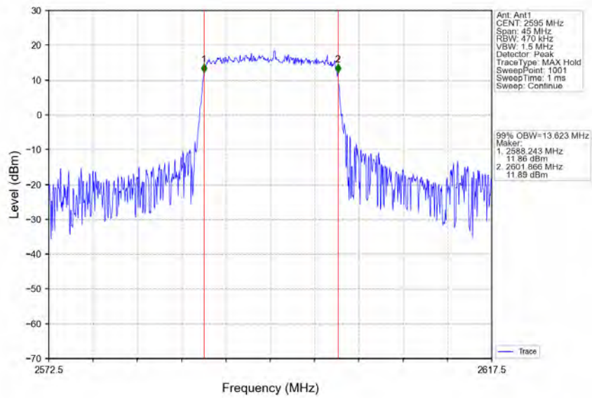
Band38_15MHz_64QAM_MCH_2595MHz_RB_75_0_NTNV
