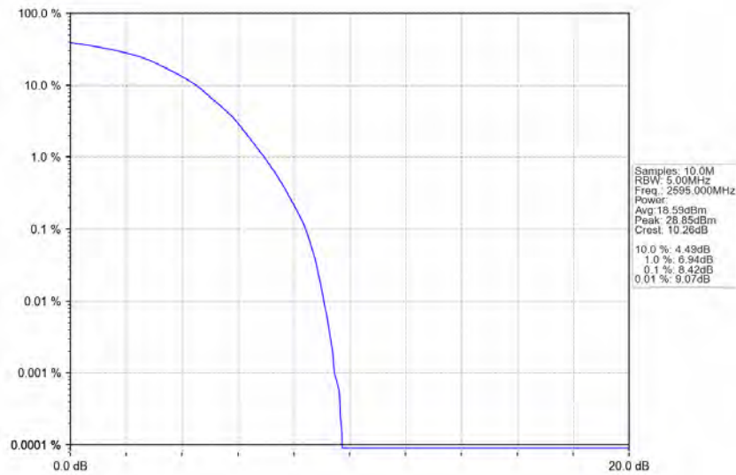
Band38_5MHz_64QAM_MCH_2595MHz_RB_25_0_NTNV
