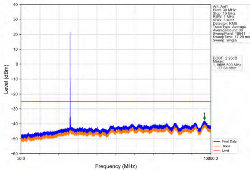
Band38_10MHz_64QAM_HCH_2615MHz_RB_1_0_NTNV
