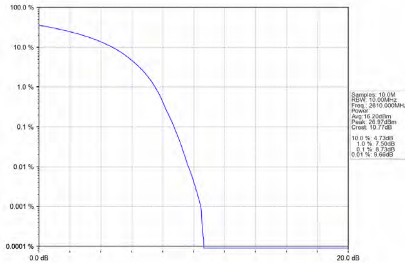
Band38_20MHz_64QAM_HCH_2610MHz_RB_100_0_NTNV
