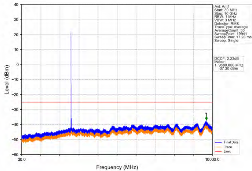
Band38_10MHz_16QAM_HCH_2615MHz_RB_1_0_NTNV
