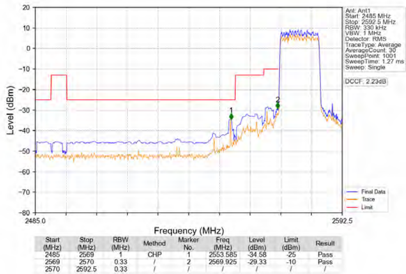
Band38_15MHz_QPSK_LCH_2577.5MHz_RB_75_0_NTNV
