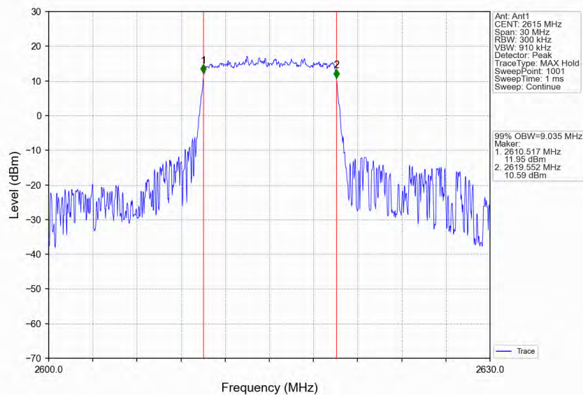
Band38_10MHz_64QAM_HCH_2615MHz_RB_50_0_NTNV
