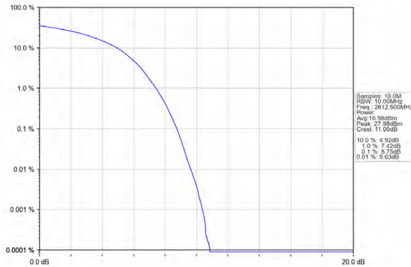
Band38_15MHz_64QAM_HCH_2612.5MHz_RB_75_0_NTNV
