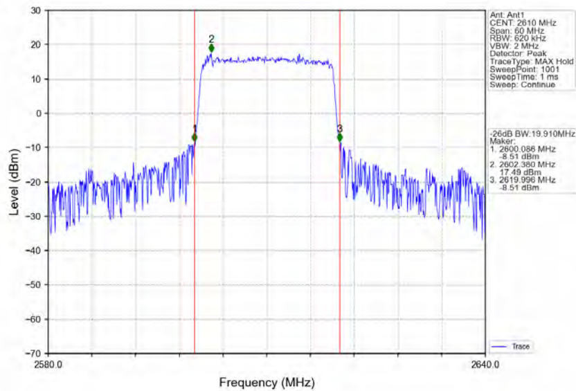
Band38_20MHz_64QAM_HCH_2610MHz_RB_100_0_NTNV
