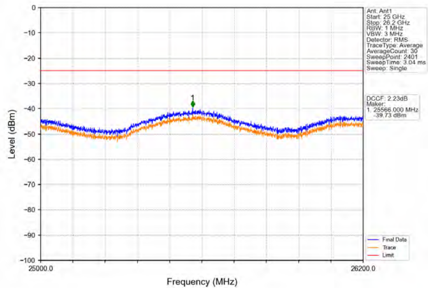
Band38_10MHz_64QAM_HCH_2615MHz_RB_1_49_NTNV
