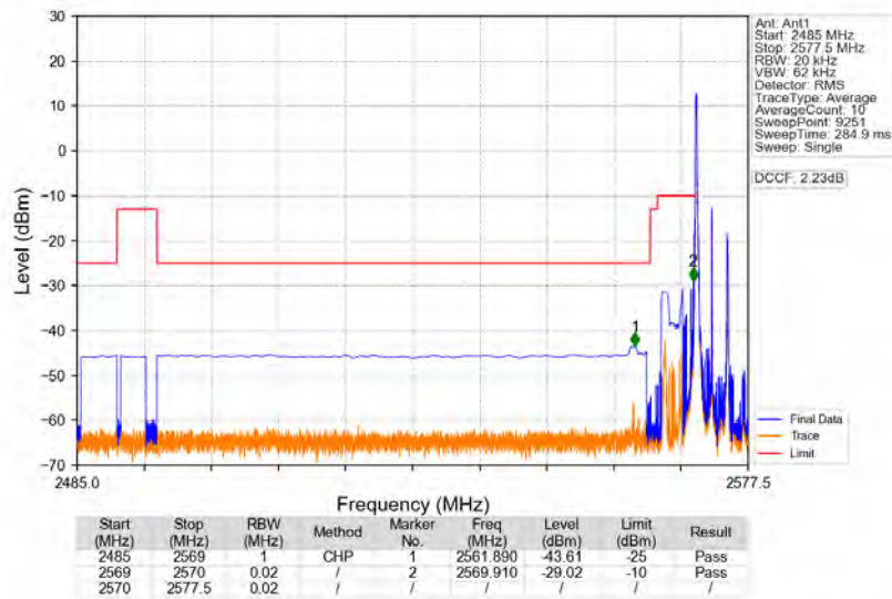
Band38_5MHz_64QAM_LCH_2572.5MHz_RB_1_0_NTNV
