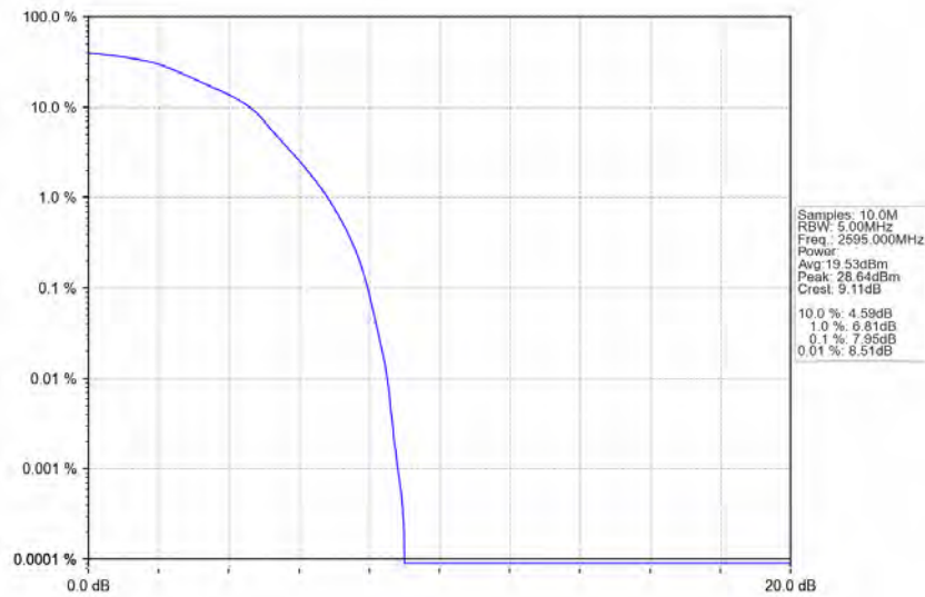
Band38_5MHz_16QAM_MCH_2595MHz_RB_25_0_NTNV
