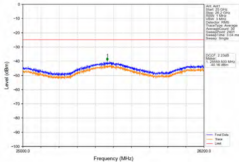
Band38_10MHz_64QAM_LCH_2575MHz_RB_1_0_NTNV
