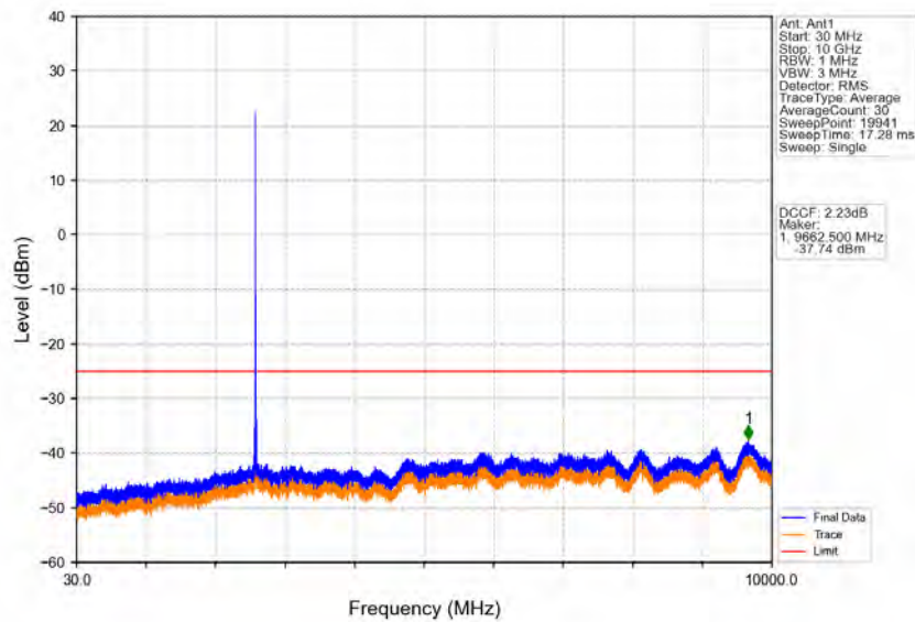
Band38_10MHz_16QAM_MCH_2595MHz_RB_1_0_NTNV
