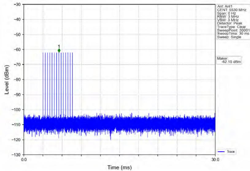
Signal Calibration 802.11ac(VHT80) 2C 5530MHz RadarType5 Trial0
