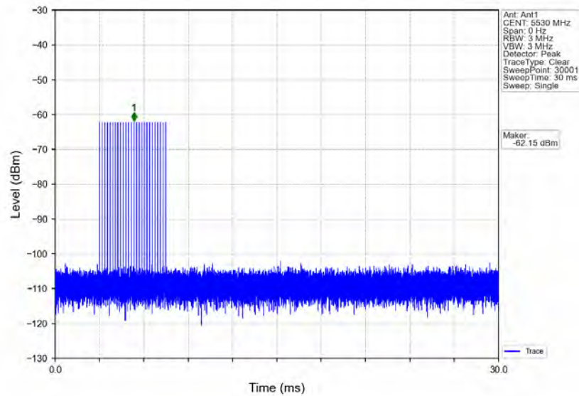
Signal Calibration 802.11ac(VHT80) 2C 5530MHz RadarType3 Trial0
