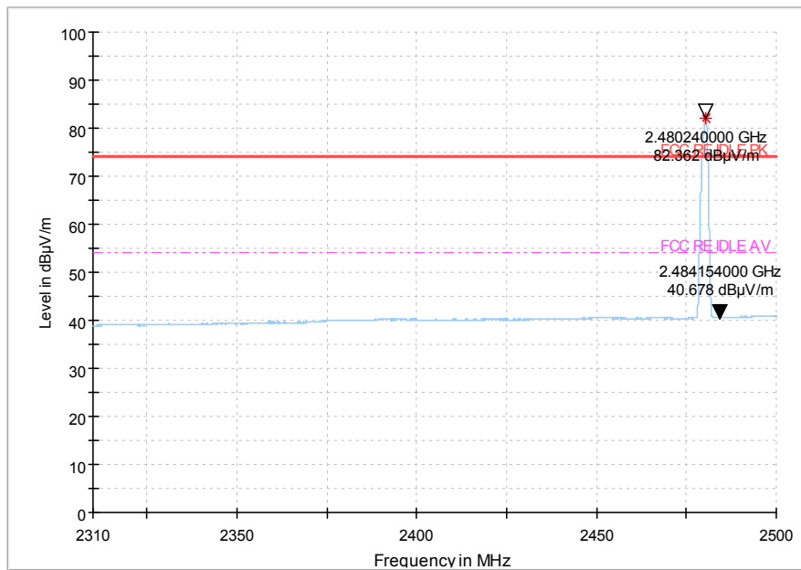
Fig.44 Radiated emission (High): \pi/4 DQPSK, high channel
