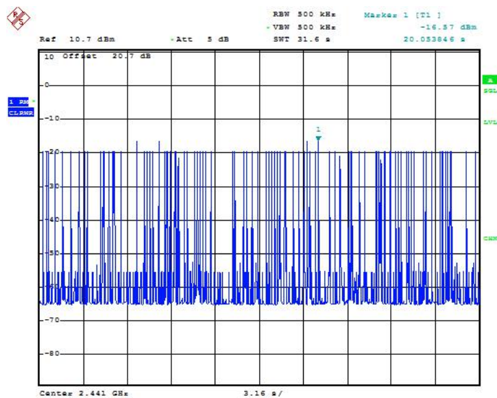
Fig.60 Time of occupancy (Dwell Time): Ch39, Packet 2-DH5
