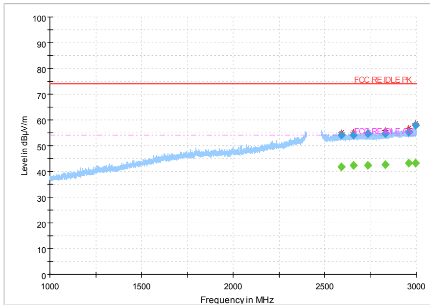
Fig.41 Radiated emission: \pi/4 DQPSK, Ch78, 1GHz~3GHz
