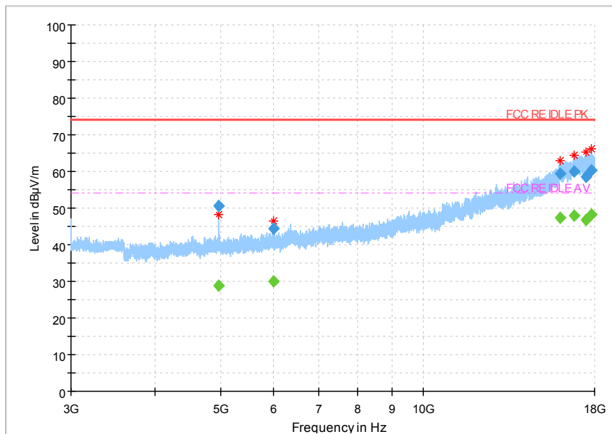
Fig.42 Radiated emission: \pi/4 DQPSK, Ch78, 3GHz~18GHz
