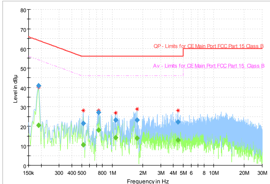
Fig.87 AC Powerline Conducted Emission
