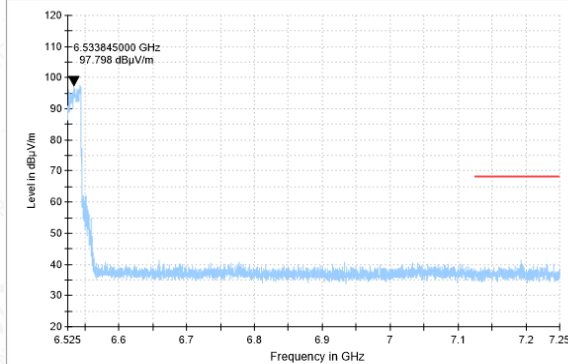
BANDEDGE-11AX-CH185-PK
