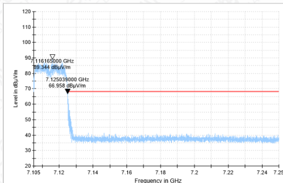
BANDEDGE-11AX-CH233-PK
