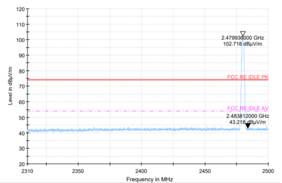
Bandedge:1M Ch39
