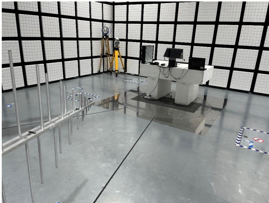
Description: Back view of Radiated Emission Test Setup (Below 1GHz)
