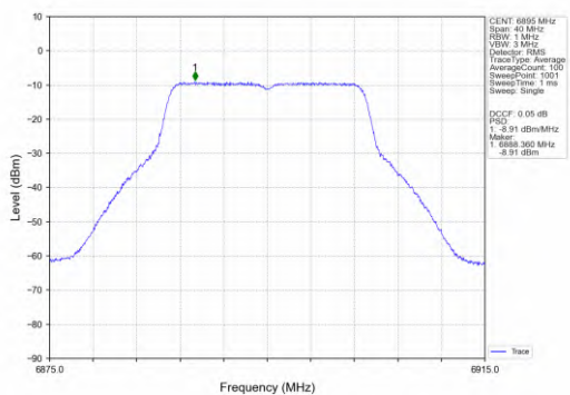
802.11ac(VHT20)_LCH_6895MHz_Ant2_NTNV
