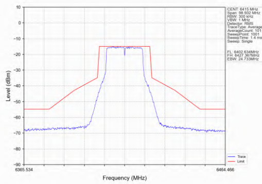
802.11ac(VHT20)_HCH_6415MHz_Ant1_NTNV
