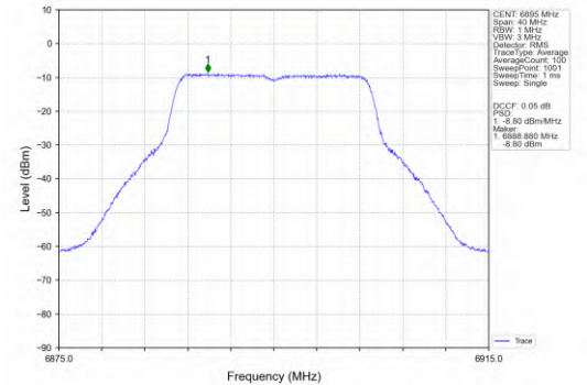
802.11ac(VHT20)_LCH_6895MHz_MIMO_NTNV
