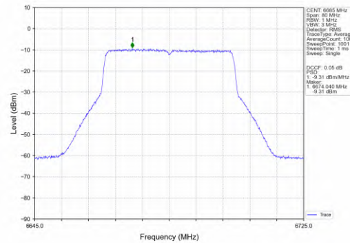
802.11ax(HEW40)_MCH_6685MHz_SU_/_MIMO_NTNV
