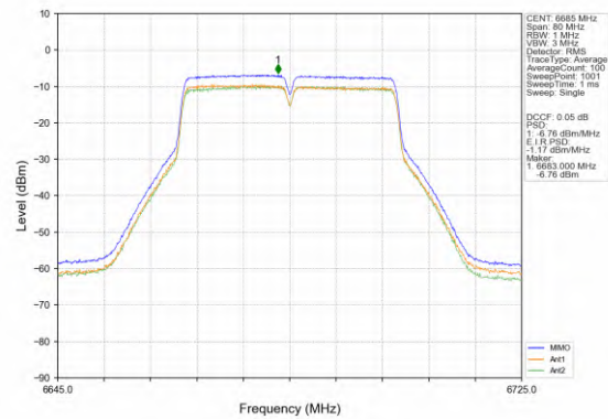
802.11n(HT40)_MCH_6685MHz_MIMO_NTNV
