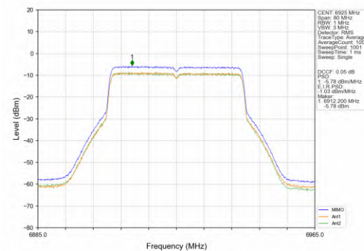
802.11ax(HEW40)_LCH_6925MHz_SU_/_MIMO_NTNV
