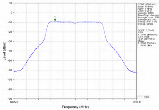
802.11ac(VHT20)_LCH_6895MHz_Ant2_NTNV
