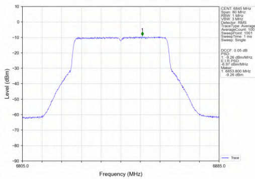
802.11ax(HEW40)_HCH_6845MHz_SU_/_MIMO_NTNV
