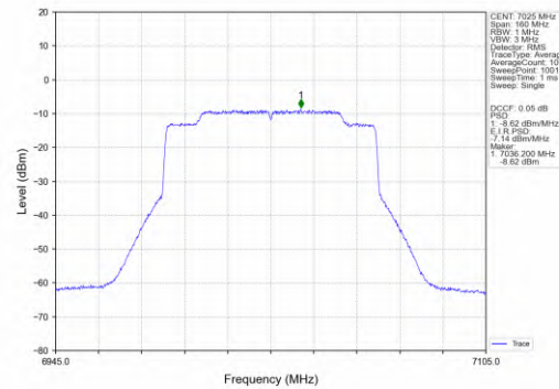
802.11ax(HEW80)_HCH_7025MHz_SU_/_MIMO_NTNV
