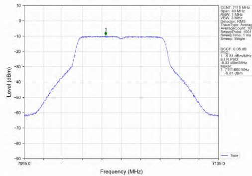
802.11ac(VHT20)_HCH_7115MHz_MIMO_NTNV
