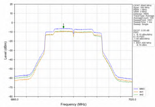
802.11ac(VHT80)_LCH_6945MHz_MIMO_NTNV
