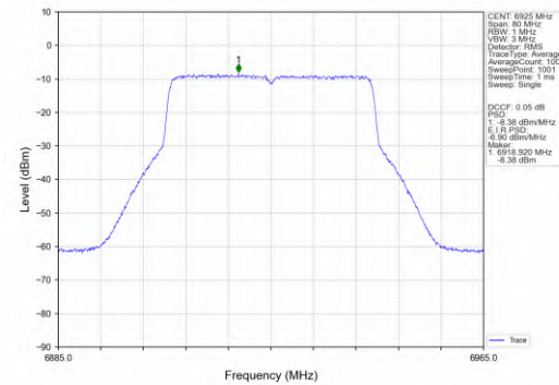
802.11ax(HEW40)_LCH_6925MHz_SU_/_MIMO_NTNV
