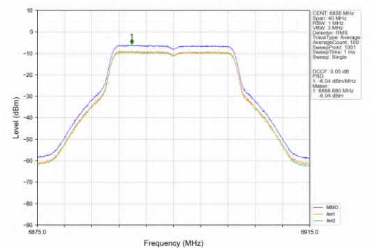
802.11ac(VHT20)_LCH_6895MHz_MIMO_NTNV
