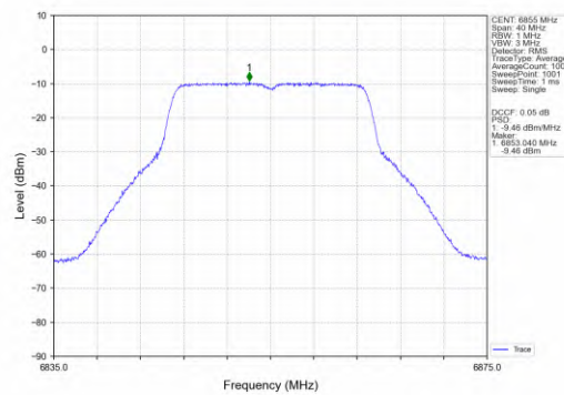
802.11ac(VHT20)_HCH_6855MHz_MIMO_NTNV
