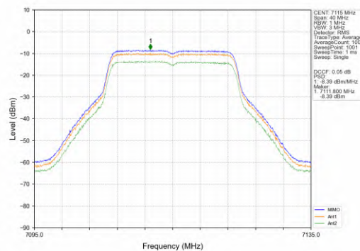
802.11ac(VHT20)_HCH_7115MHz_MIMO_NTNV
