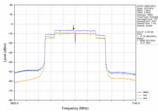
802.11ax(HEW160)_MCH_6985MHz_SU_ / _MIMO_NTNV
