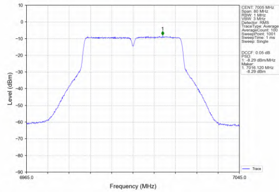
802.11n(HT40)_MCH_7005MHz_MIMO_NTNV
