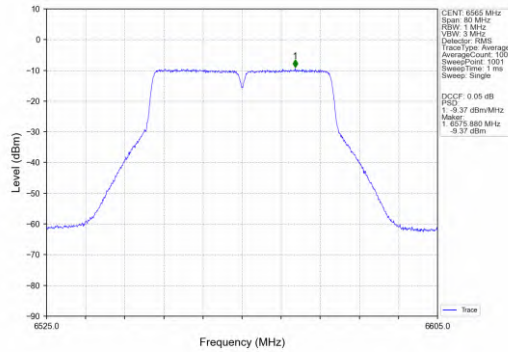
802.11ac(VHT40)_LCH_6565MHz_MIMO_NTNV
