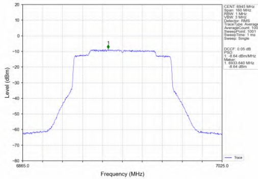
802.11ax(HEW80)_LCH_6945MHz_SU_/_MIMO_NTNV
