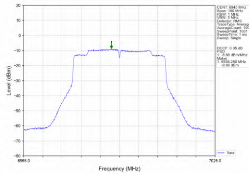
802.11ac(VHT80)_LCH_6945MHz_MIMO_NTNV
