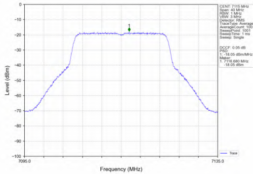
802.11ax(HEW20)_HCH_7115MHz_SU_/_MIMO_NTNV
