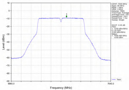
802.11n(HT40)_MCH_7005MHz_Ant2_NTNV
