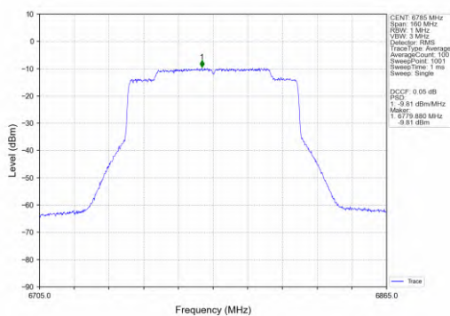
802.11ax(HEW80)_HCH_6785MHz_SU_/_Ant2_NTNV
