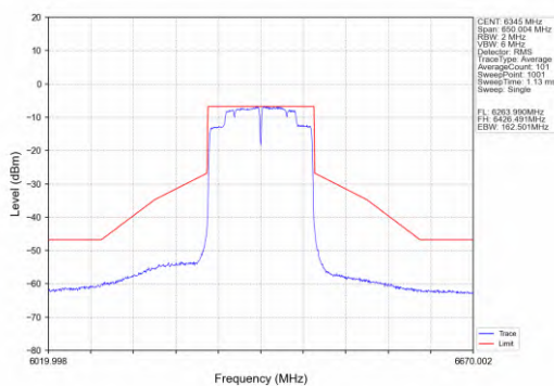
802.11ac(VHT160)_HCH_6345MHz_Ant1_NTNV
