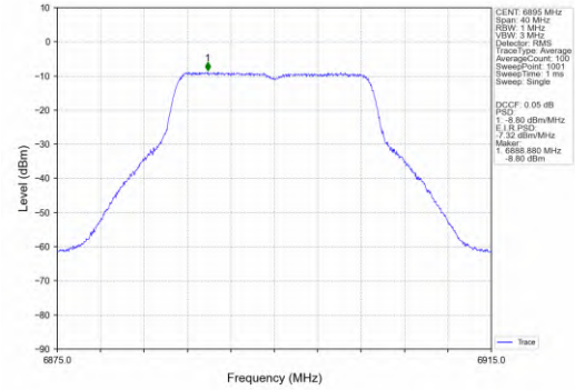
802.11ac(VHT20)_LCH_6895MHz_MIMO_NTNV
