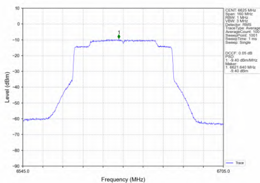
802.11ax(HEW80)_LCH_6625MHz_SU_/_Ant2_NTNV
