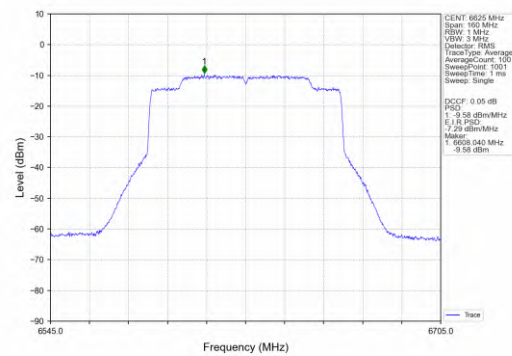
802.11ax(HEW80)_LCH_6625MHz_SU_ / _MIMO_NTNV
