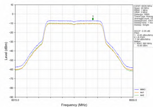
802.11ax(HEW20)_LCH_6535MHz_SU_/_MIMO_NTNV
