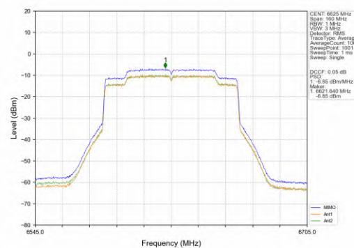
802.11ax(HEW80)_LCH_6625MHz_SU_/_MIMO_NTNV
