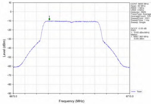
802.11ax(HEW20)_MCH_6695MHz_SU_/_MIMO_NTNV
