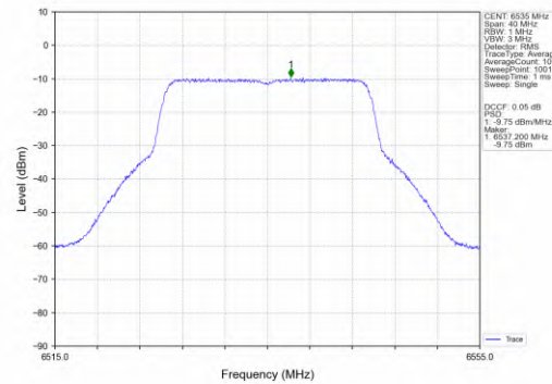
802.11ax(HEW20)_LCH_6535MHz_SU_/_MIMO_NTNV
