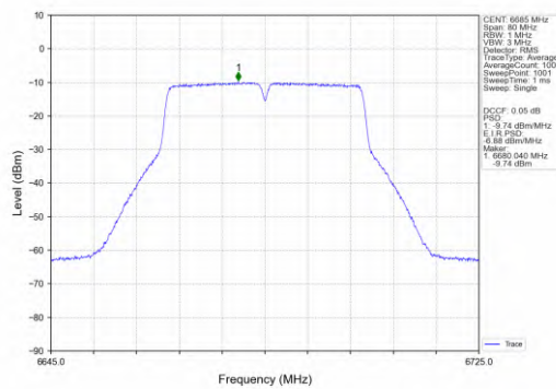
802.11ac(VHT40)_MCH_6685MHz_Ant2_NTNV
