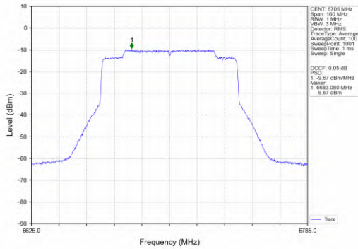
802.11ax(HEW80)_MCH_6705MHz_SU_/_MIMO_NTNV
