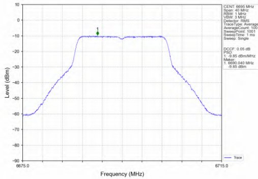
802.11ac(VHT20)_MCH_6695MHz_MIMO_NTNV
