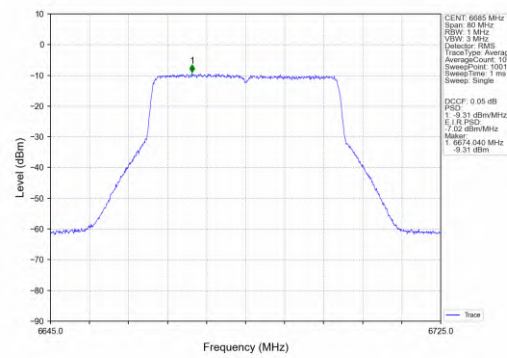
802.11ax(HEW40)_MCH_6685MHz_SU_/_MIMO_NTNV
