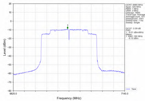
802.11ax(HEW160)_MCH_6985MHz_SU_ / _MIMO_NTNV
