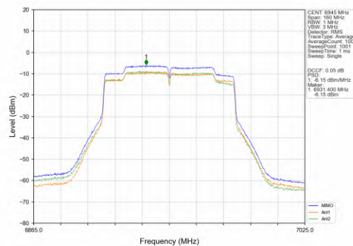
802.11ac(VHT80)_LCH_6945MHz_MIMO_NTNV
