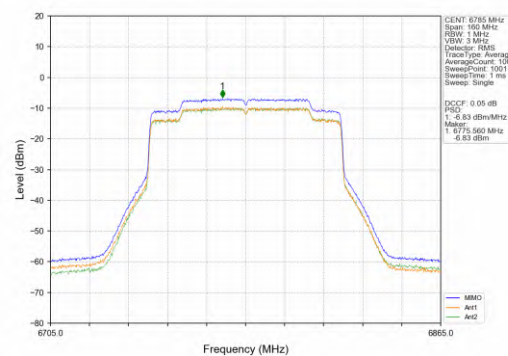
802.11ax(HEW80)_HCH_6785MHz_SU_/_MIMO_NTNV
