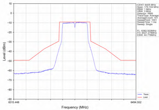
802.11n(HT40)_HCH_6405MHz_Ant1_NTNV
