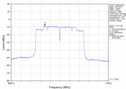
802.11ac(VHT160)_MCH_6985MHz_Ant2_NTNV
