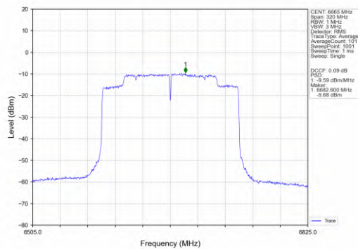
802.11ax(HEW160)_MCH_6665MHz_SU_ / _MIMO_NTNV
