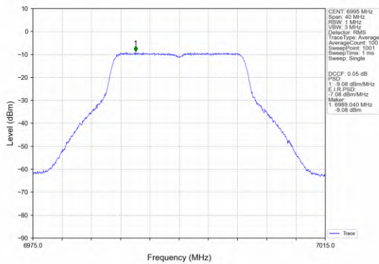
802.11n(HT20)_MCH_6995MHz_Ant2_NTNV
