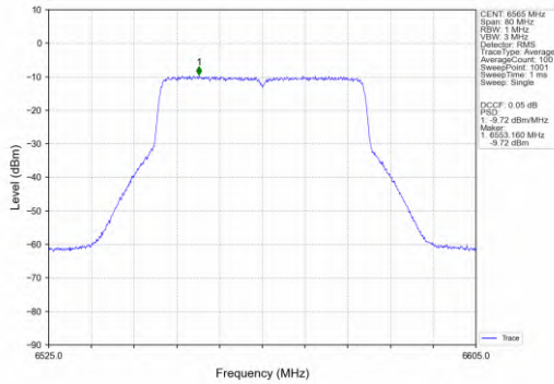
802.11ax(HEW40)_LCH_6565MHz_SU_/_MIMO_NTNV
