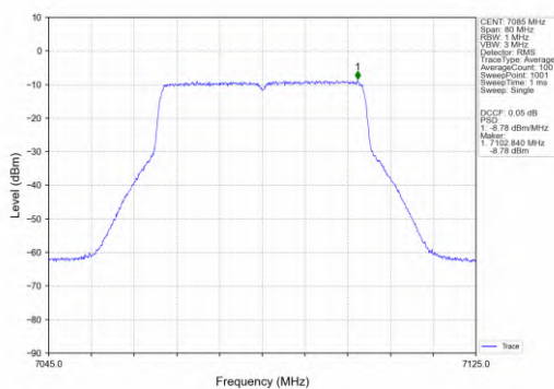
802.11ax(HEW40)_HCH_7085MHz_SU_/_Ant2_NTNV
