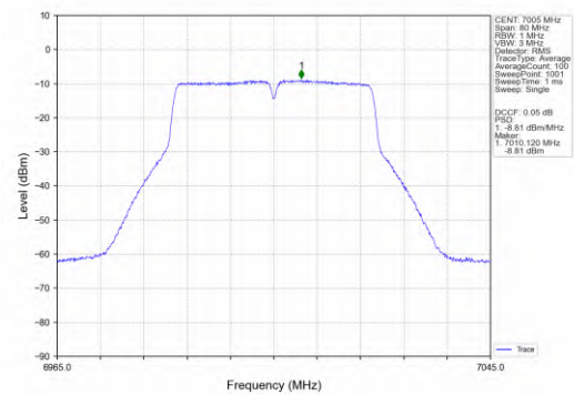
802.11ac(VHT40)_MCH_7005MHz_MIMO_NTNV
