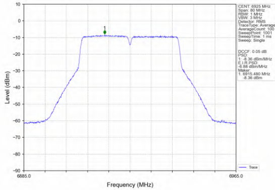
802.11n(HT40)_LCH_6925MHz_MIMO_NTNV
