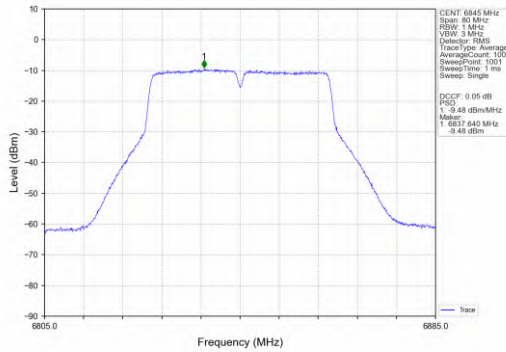
802.11ac(VHT40)_HCH_6845MHz_MIMO_NTNV
