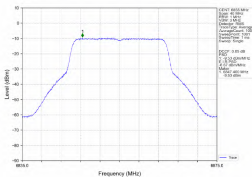
802.11ax(HEW20)_HCH_6855MHz_SU_/_Ant2_NTNV
