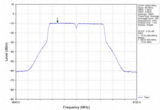
802.11ac(VHT40)_MCH_6685MHz_MIMO_NTNV
