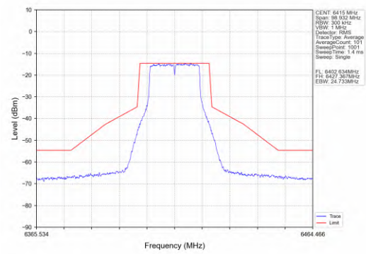
802.11ac(VHT20)_HCH_6415MHz_Ant2_NTNV
