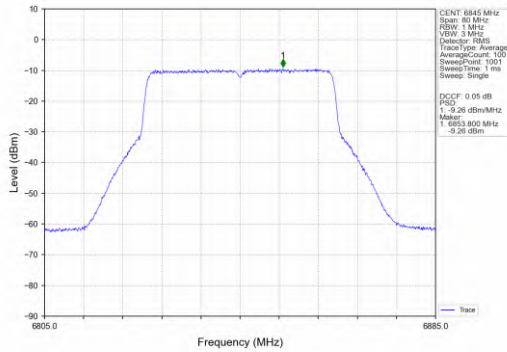
802.11ax(HEW40)_HCH_6845MHz_SU_/_MIMO_NTNV
