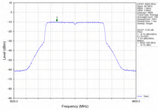
802.11ax(HEW40)_LCH_6565MHz_SU_/_MIMO_NTNV
