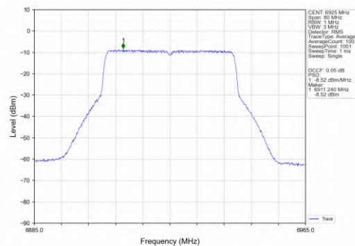
802.11ax(HEW40)_LCH_6925MHz_SU_/_Ant2_NTNV
