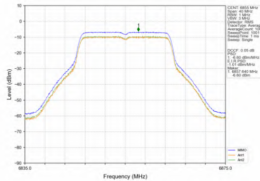
802.11ac(VHT20)_HCH_6855MHz_MIMO_NTNV
