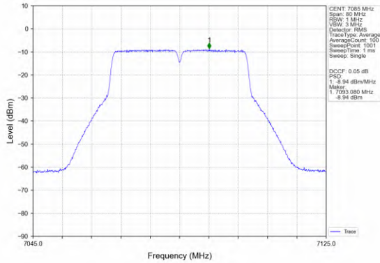
802.11n(HT40)_HCH_7085MHz_MIMO_NTNV
