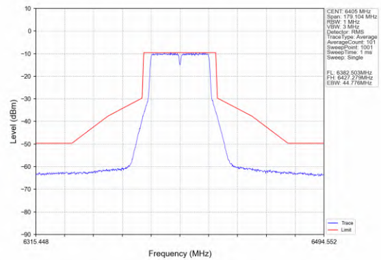
802.11n(HT40)_HCH_6405MHz_Ant2_NTNV
