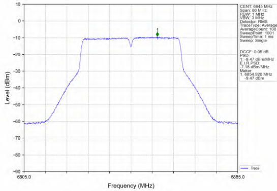
802.11n(HT40)_HCH_6845MHz_MIMO_NTNV
