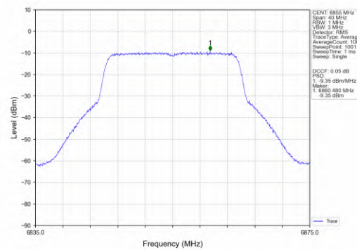
802.11ax(HEW20)_HCH_6855MHz_SU_/_MIMO_NTNV
