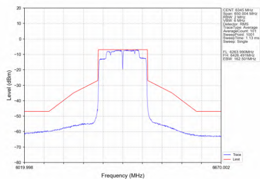
802.11ac(VHT160)_HCH_6345MHz_Ant2_NTNV
