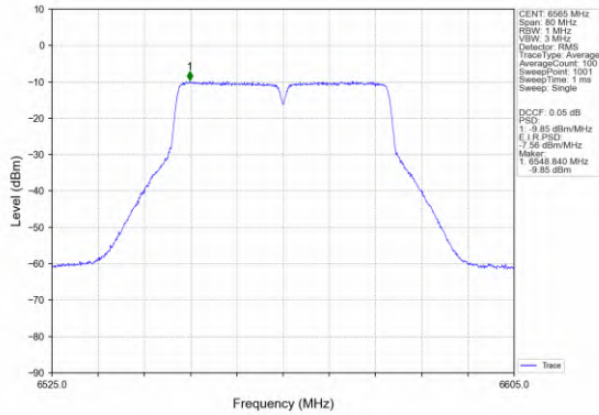
802.11n(HT40)_LCH_6565MHz_MIMO_NTNV
