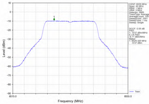
802.11ac(VHT20)_LCH_6535MHz_Ant2_NTNV
