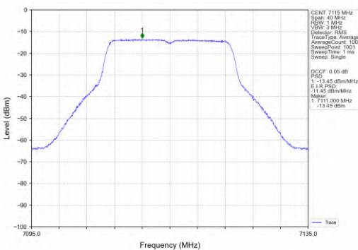
802.11ac(VHT20)_HCH_7115MHz_Ant2_NTNV
