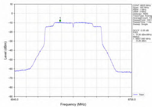
802.11ac(VHT80)_LCH_6625MHz_MIMO_NTNV
