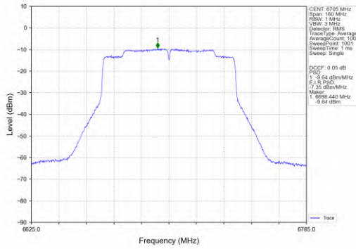
802.11ac(VHT80)_MCH_6705MHz_MIMO_NTNV
