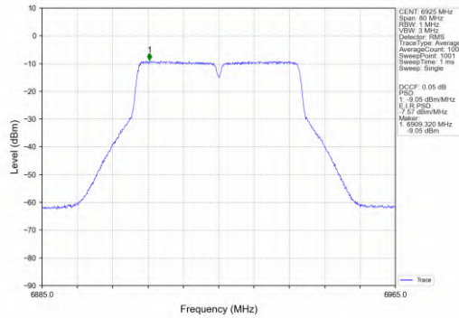
802.11ac(VHT40)_LCH_6925MHz_MIMO_NTNV
