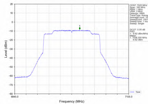
802.11ax(HEW80)_HCH_7025MHz_SU_/_MIMO_NTNV
