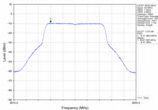
802.11ax(HEW20)_LCH_6535MHz_SU_/_Ant2_NTNV
