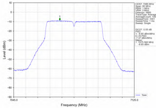
802.11ac(VHT40)_HCH_7085MHz_MIMO_NTNV
