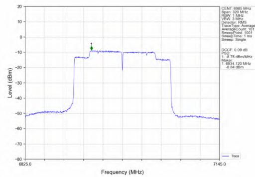
802.11ax(HEW160)_MCH_6985MHz_SU_/_Ant2_NTNV
