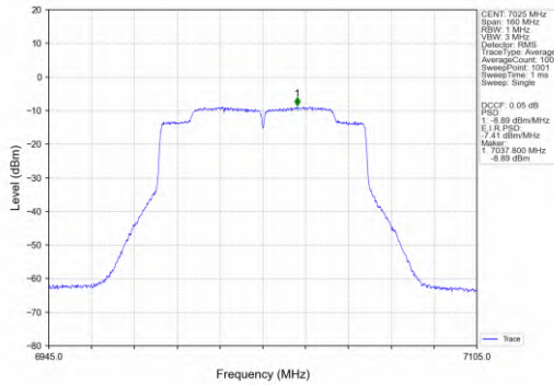
802.11ac(VHT80)_HCH_7025MHz_MIMO_NTNV
