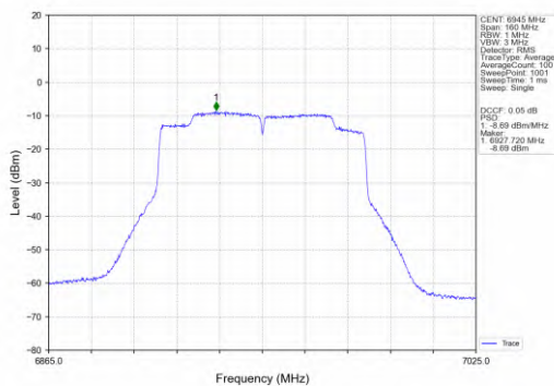
802.11ac(VHT80)_LCH_6945MHz_Ant2_NTNV
