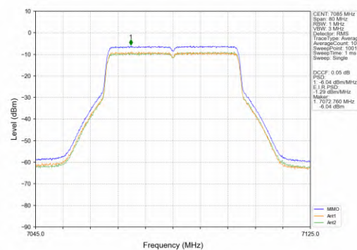
802.11ax(HEW40)_HCH_7085MHz_SU_ / _MIMO_NTNV
