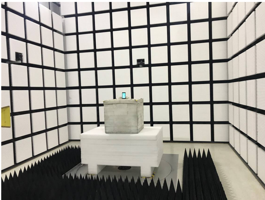
Radiated Emission Above 1GHz Type-2 View
