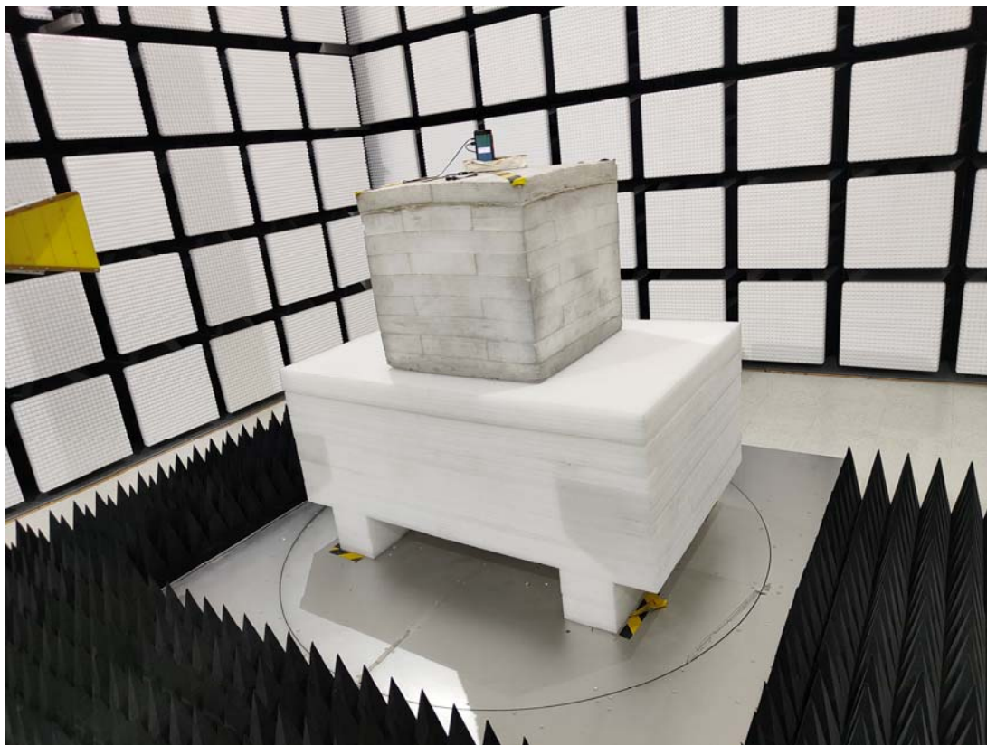
Radiated Emission Above 1GHz View Type-1 Adapter 1#
