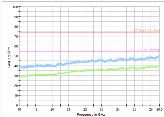
Radiated emission: GFSK, Ch78, 18GHz~26.5GHz
