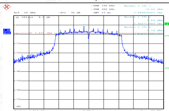
Occupied 6dB Bandwidth (MHz) (802.11n-20MHz, Ch11)
