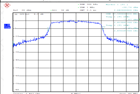
99% Occupied Bandwidth (802.11g, Ch11)
