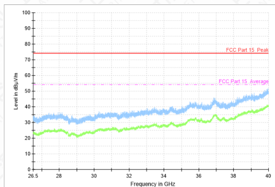
Radiated Spurious Emission (802.11g, Ch1, 26.5GHz~40GHz)
