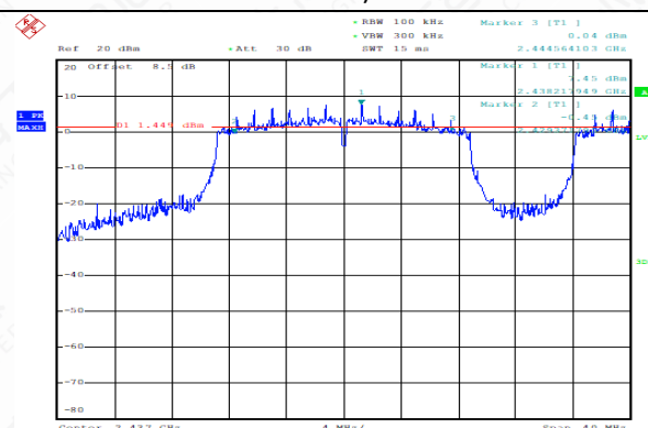
Occupied 6dB Bandwidth (MHz) (802.11n-20MHz, Ch6)
