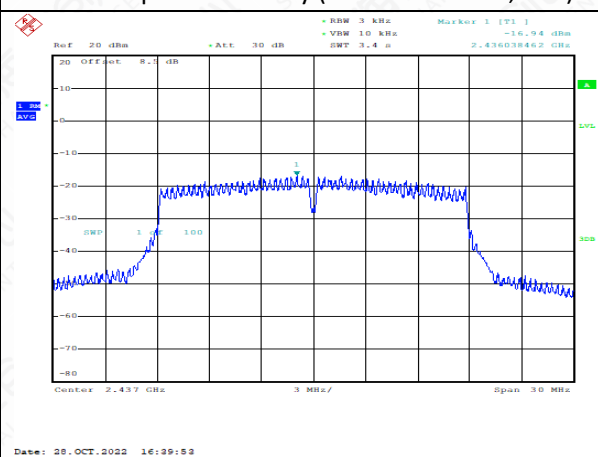
Power Spectral Density (802.11n-20MHz, Ch6)
