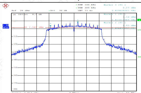
Occupied 6dB Bandwidth (MHz) (802.11n-20MHz, Ch1)
