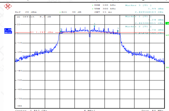
Occupied 6dB Bandwidth (MHz) (802.11g, Ch11)
