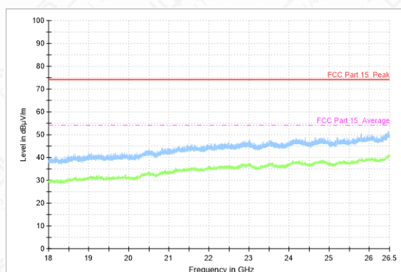
Radiated Spurious Emission (802.11b, Ch11, 18GHz~26.5GHz)
