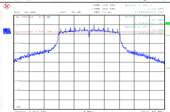
Occupied 6dB Bandwidth (MHz) (802.11g, Ch6)
