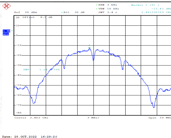
Power Spectral Density (802.11b, Ch11)
