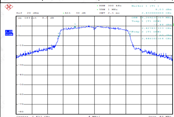
99% Occupied Bandwidth (802.11n-20MHz, Ch6)
