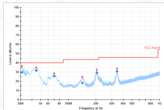
Radiated Spurious Emission (802.11n-20HT, Ch1, 30MHz~1GHz)
