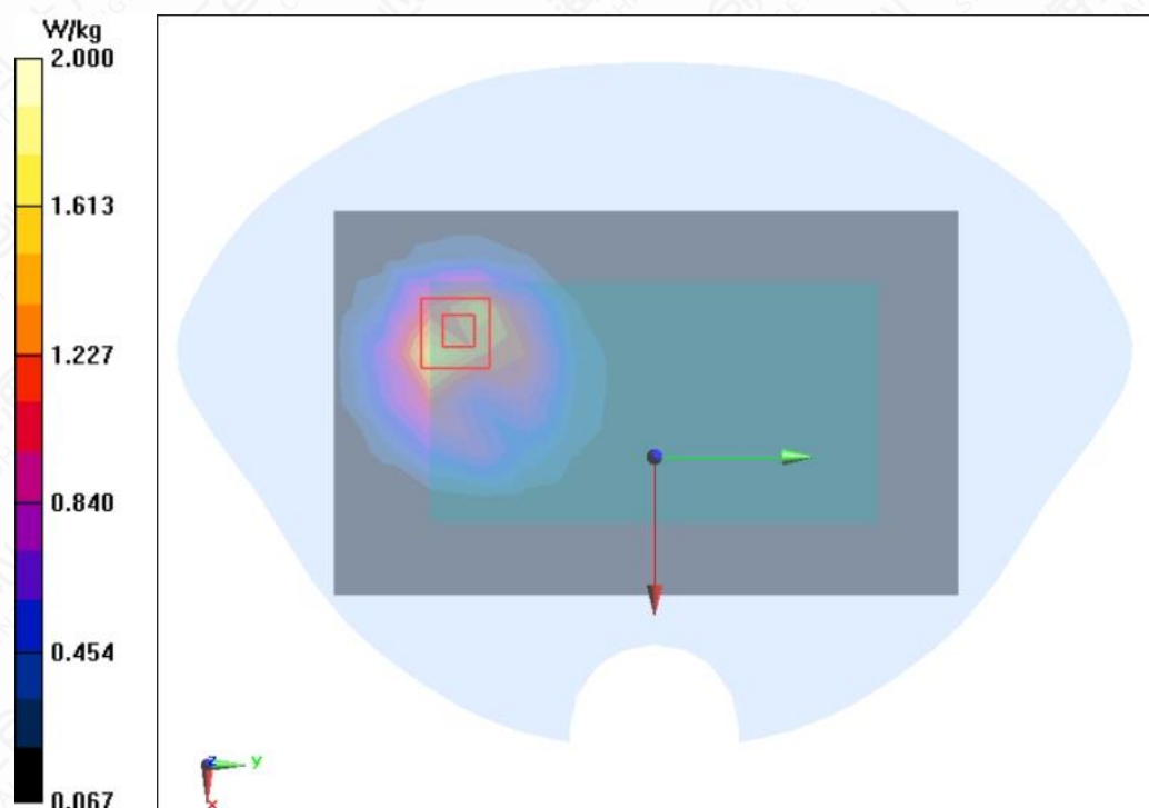
Figure A.1-20 LTE B12 10MHz 1RB 25offset Back Mode High 0mm
