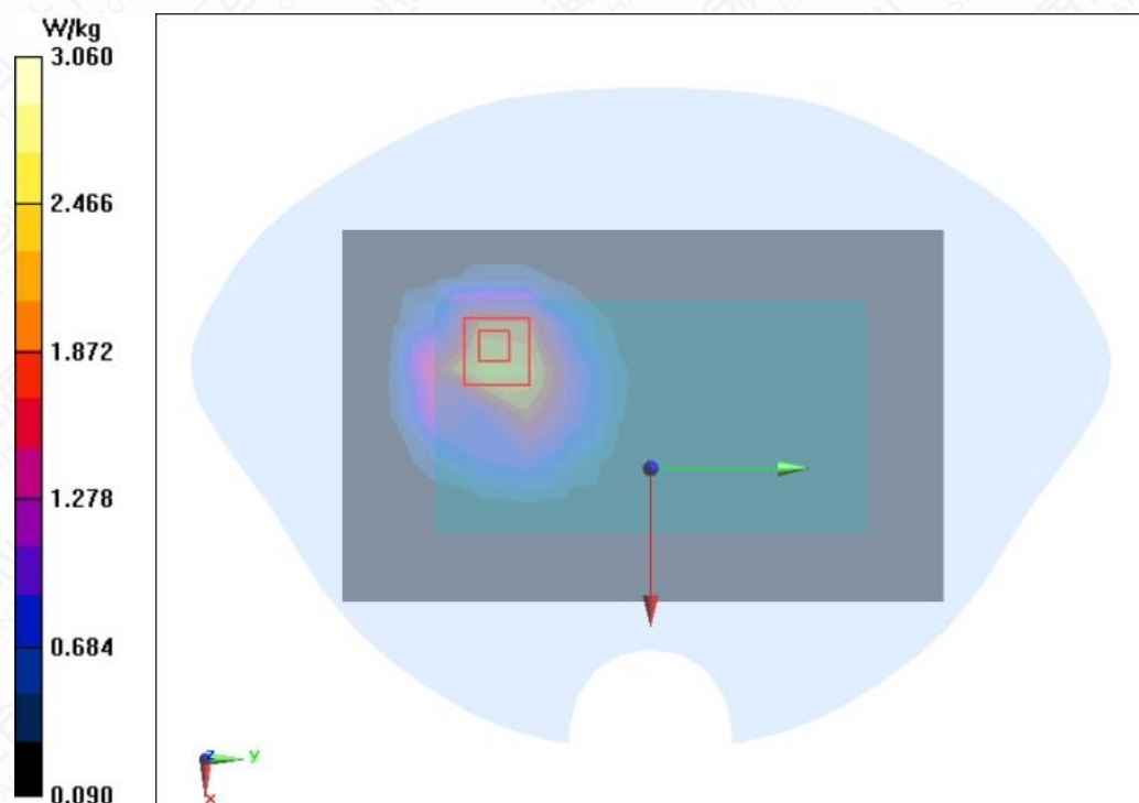
Figure A.1-16 LTE B5 10MHz 1RB 25offset Back Mode High 0mm
