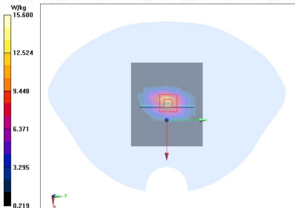
Figure A.2-7 Head 1900MHz
