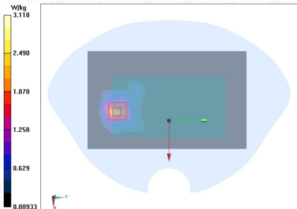
Figure A.1-18 LTE B7 20MHz 1RB 50offset Back Mode High 0mm
