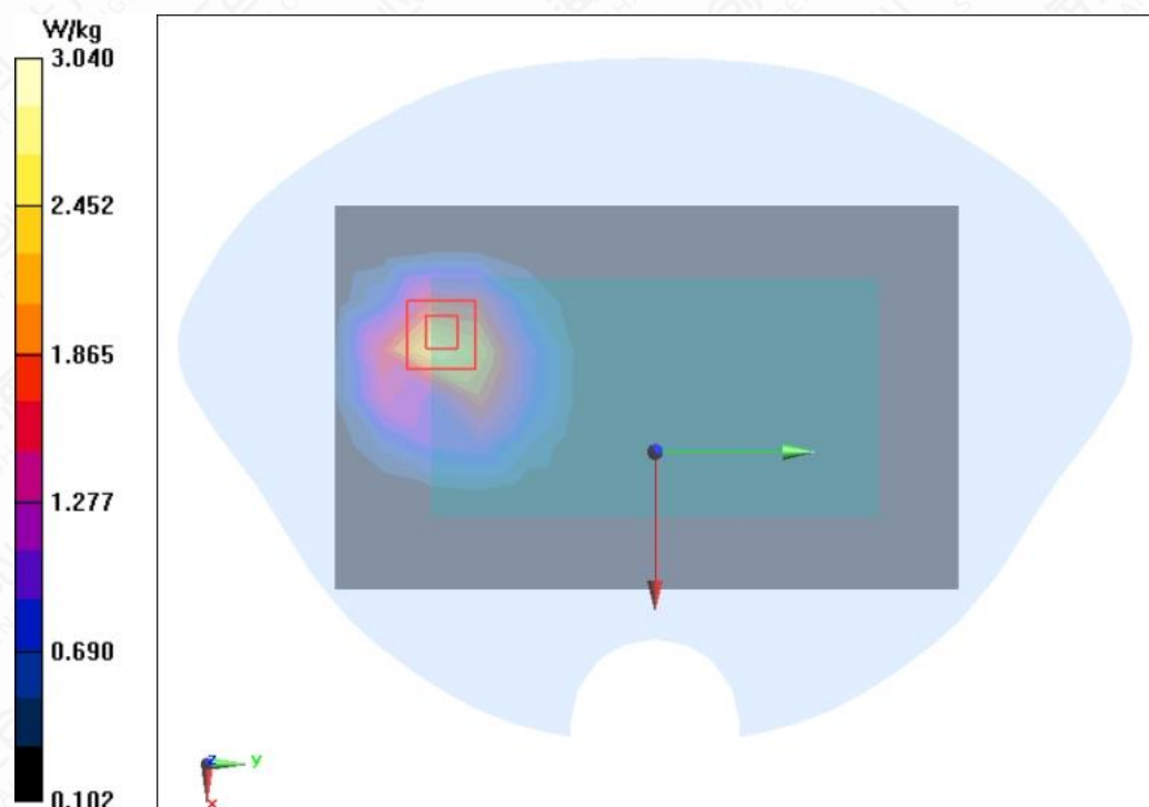
Figure A.1-10 WCDMA Band V Back Mode Low 0mm
