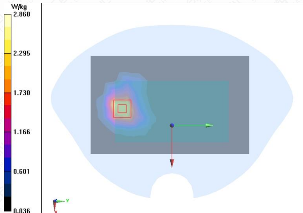
Figure A.1-12 LTE B2 20MHz 50RB 0offset Back Mode High 0mm
