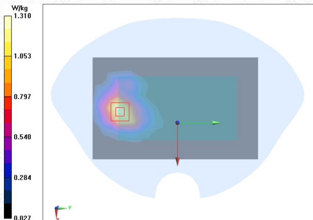
Figure A.1-5 WCDMA Band II Back Mode High 5mm
