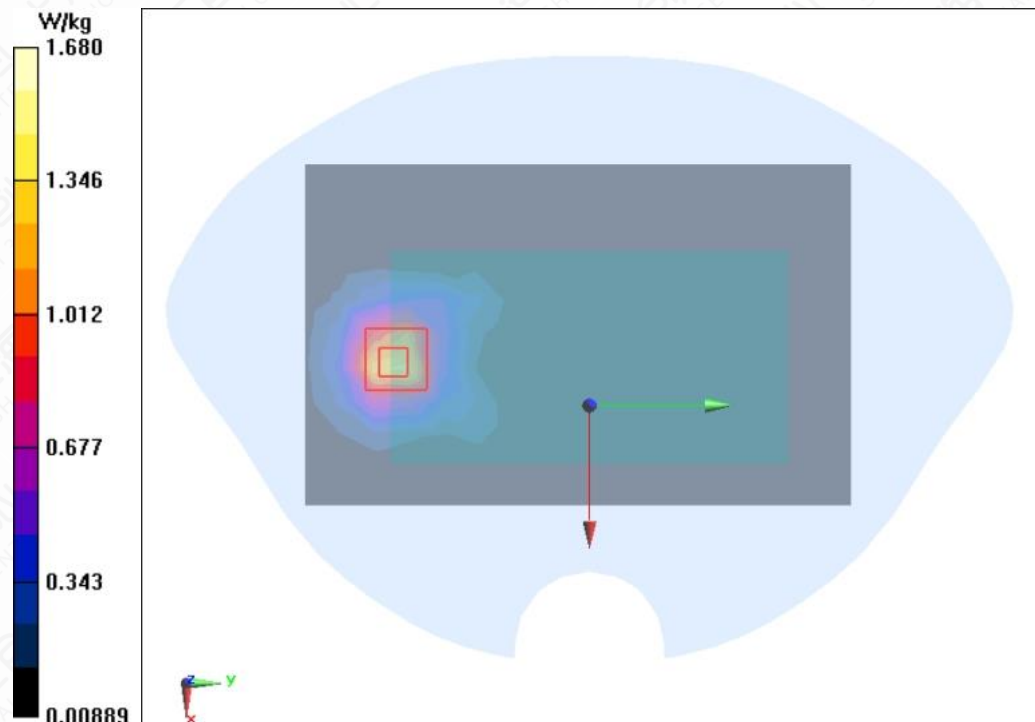
Figure A.1-17 LTE B7 20MHz 1RB 50offset Back Mode High 5mm
