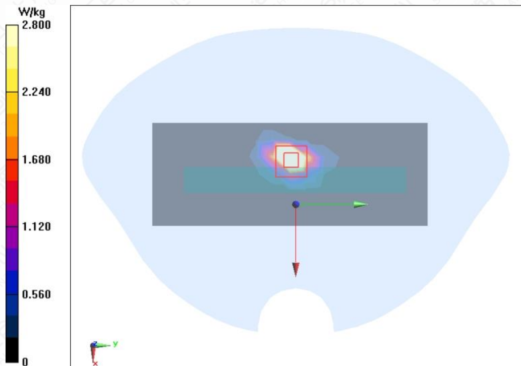
Figure A.1-30 Wi-Fi 5G U-NII-2C 11a Left Mode Middle 0mm
