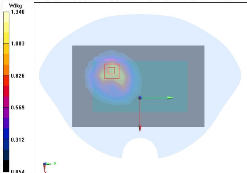
Figure A.1-1 GSM850 GPRS 4TS Back Mode High 5mm
