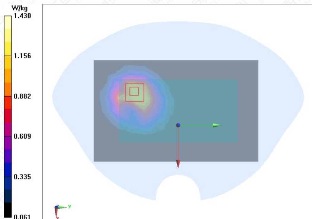
Figure A.1-9 WCDMA Band V Back Mode Middle 5mm
