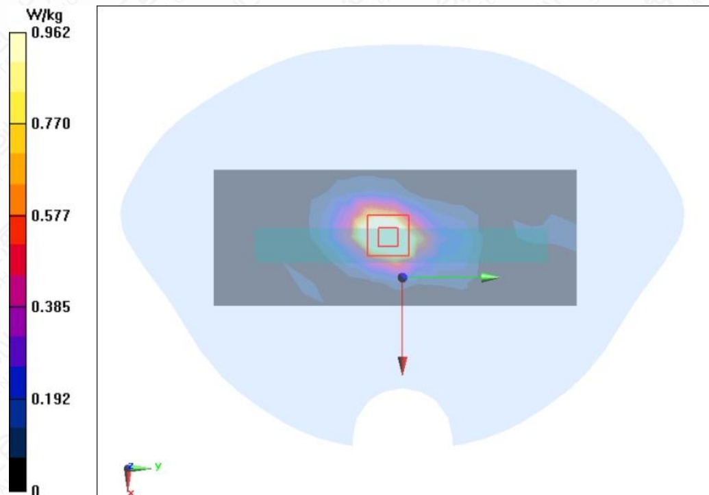
Figure A.1-27 Wi-Fi 5G U-NII-1 11a Left Mode Low 5mm
