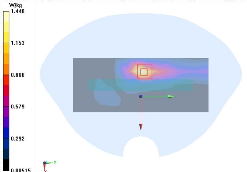
Figure A.1-26 Wi-Fi 2.4G 11b Left Mode Low 0mm
