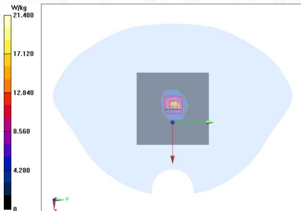
Figure A.2-16 Head 5800MHz
