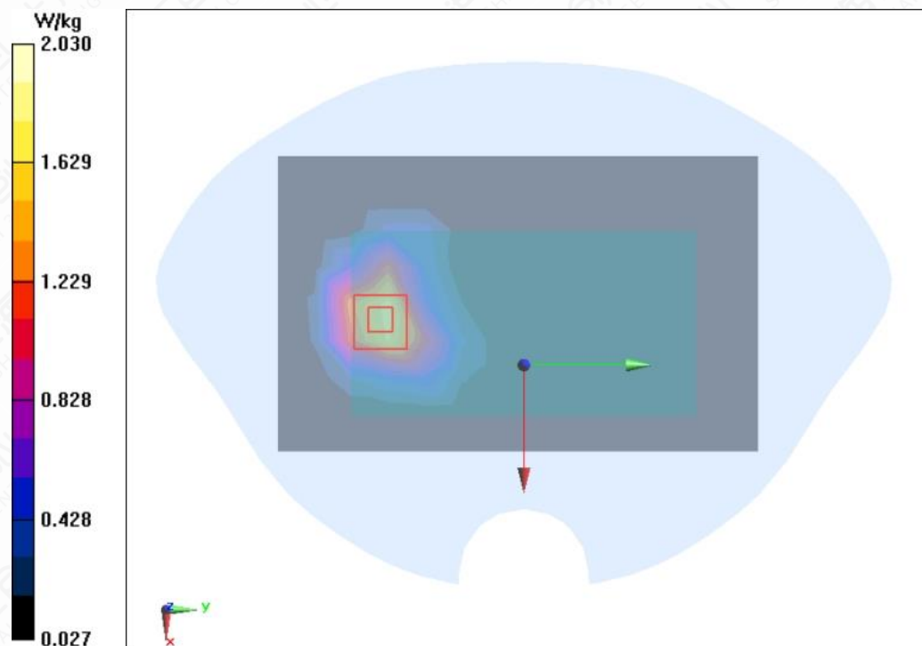
Figure A.1-4 GSM1900 GPRS 2TS Back Mode Middle 0mm
