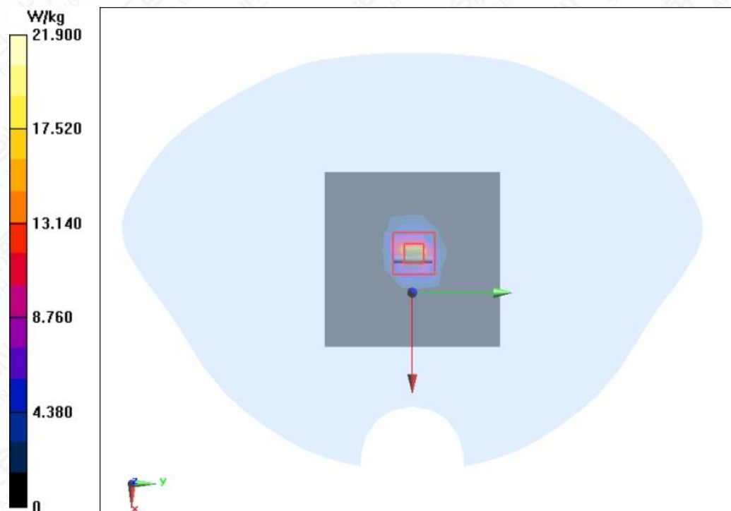
Figure A.2-15 Head 5600MHz
