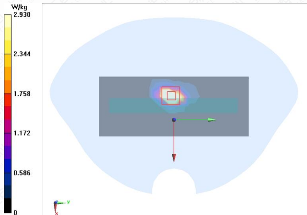
Figure A.1-32 Wi-Fi 5G U-NII-3 11a Left Mode High 0mm
