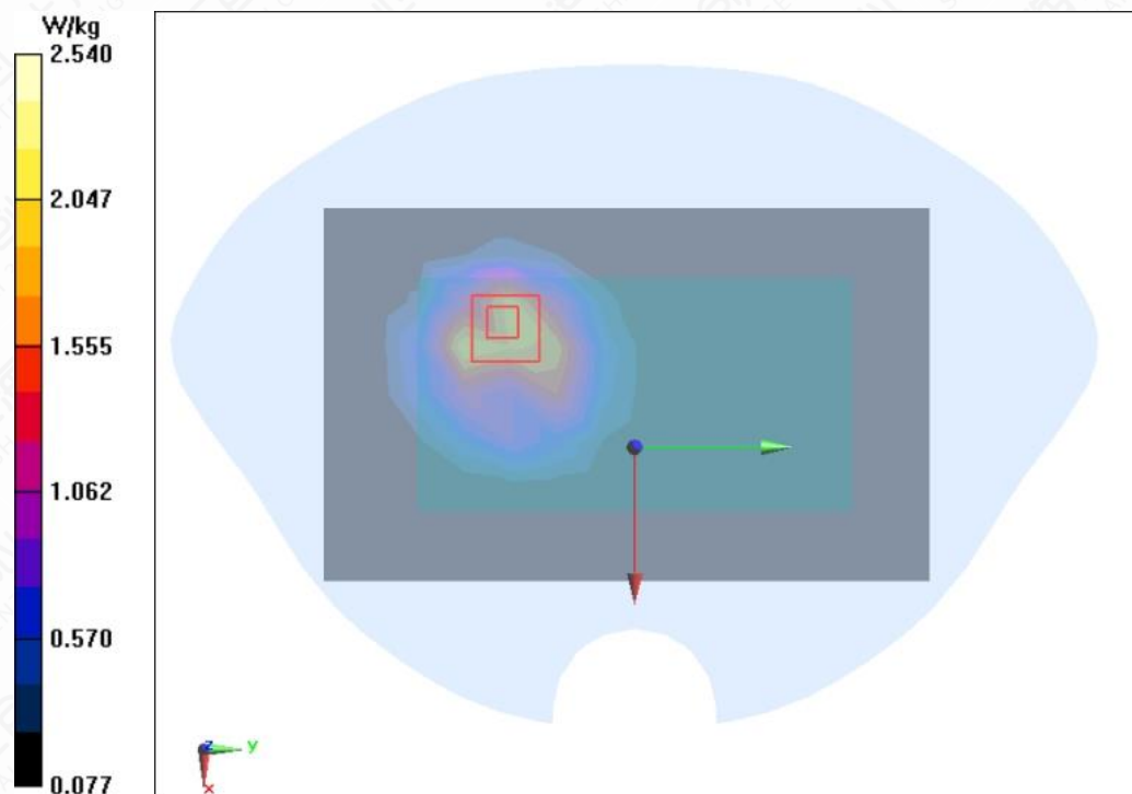
Figure A.1-2 GSM850 GPRS 4TS Back Mode High 0mm
