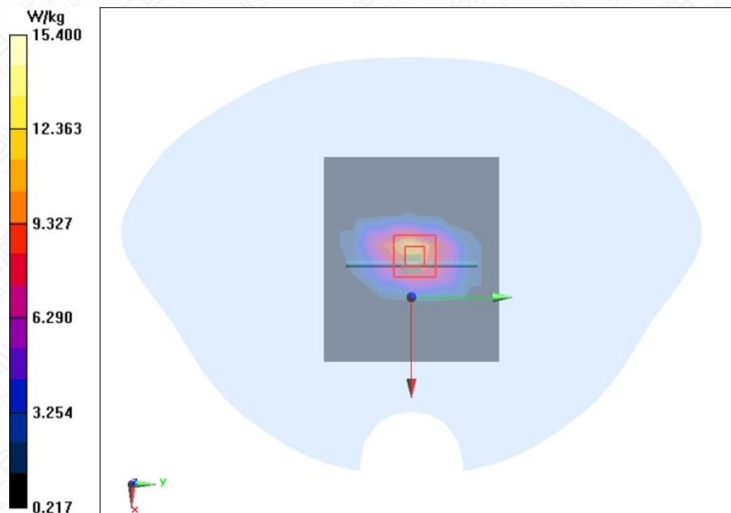
Figure A.2-8 Head 1900MHz
