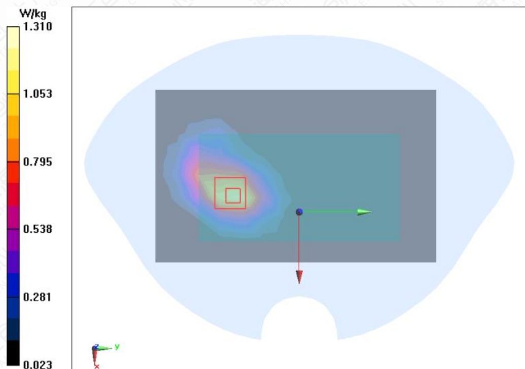
Figure A.1-7 WCDMA BandIV Back Mode Low 5mm
