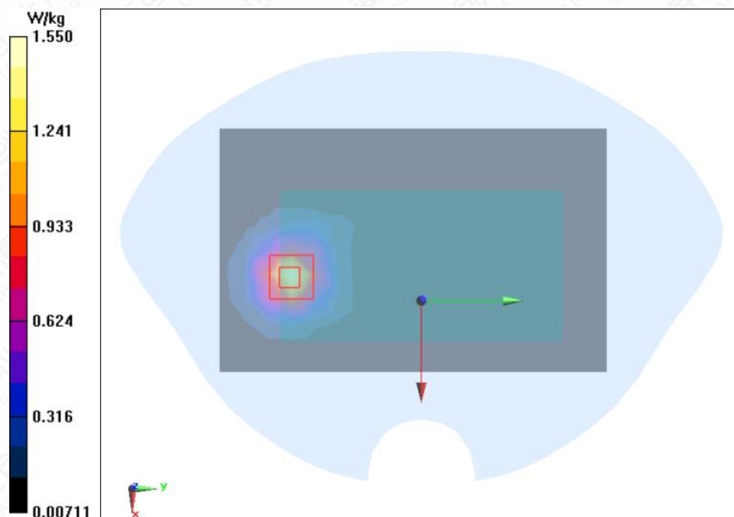
Figure A.1-21 LTE B41 20MHz 1RB 50offset Back Mode High 5mm
