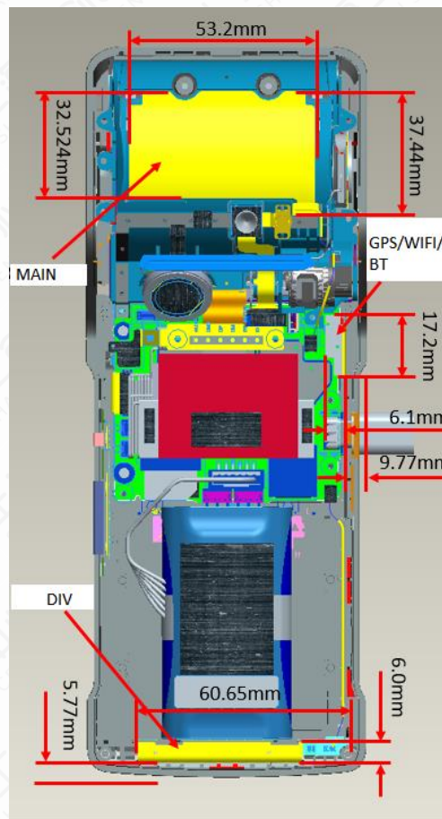
Figure 12.2-1 Antenna Locations
