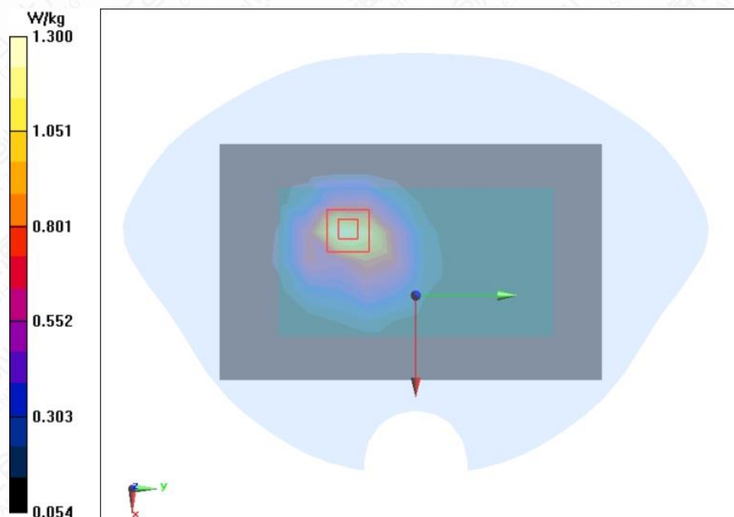
Figure A.1-15 LTE B5 10MHz 25RB 0offset Back Mode Middle 5mm
