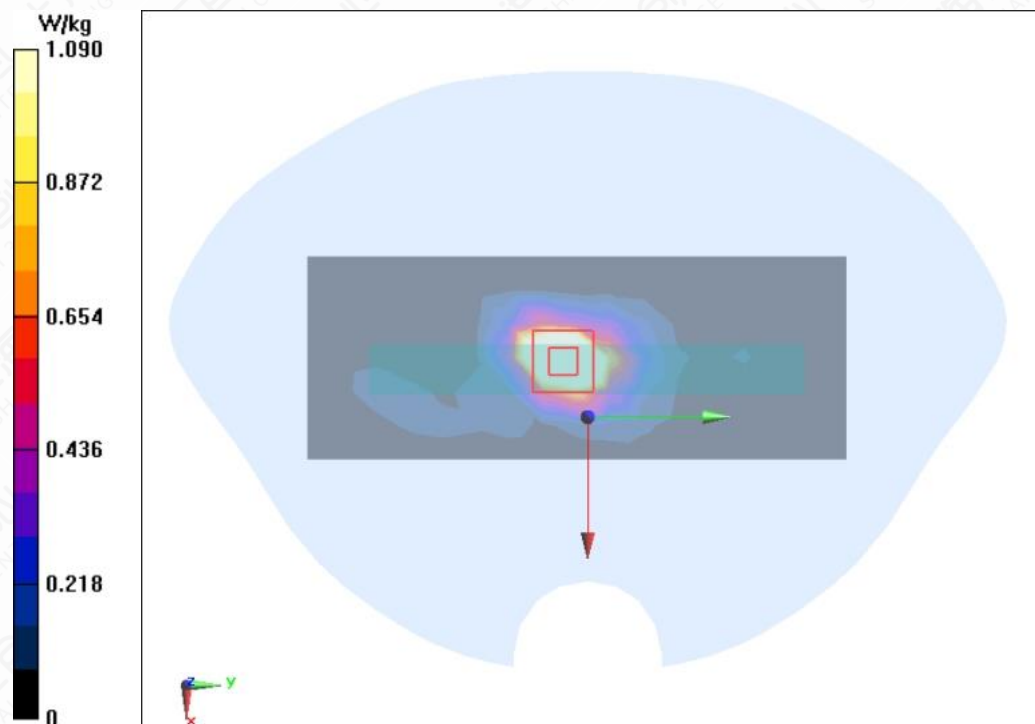
Figure A.1-31 Wi-Fi 5G U-NII-3 11a Left Mode High 5mm
