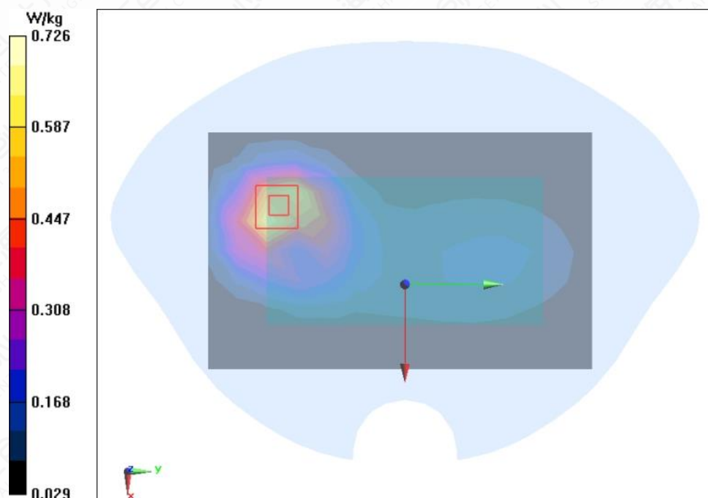
Figure A.1-19 LTE B12 10MHz 1RB 25offset Back Mode High 5mm
