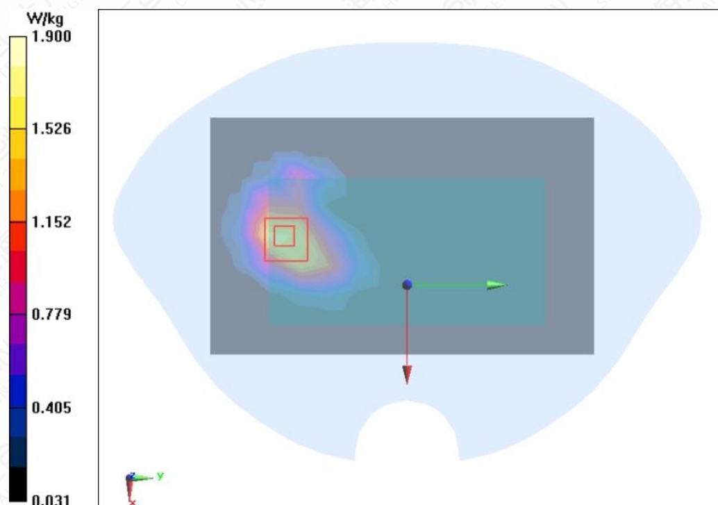
Figure A.1-8 WCDMA BandIV Back Mode High 0mm
