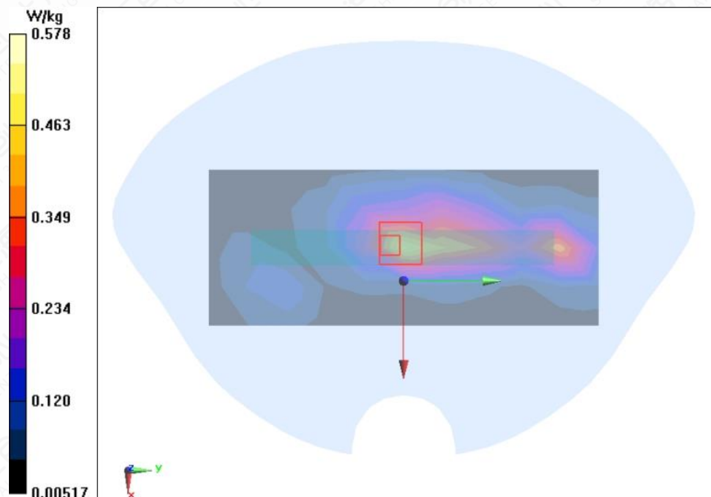
Figure A.1-25 Wi-Fi 2.4G 11b Left Mode Middle 5mm
