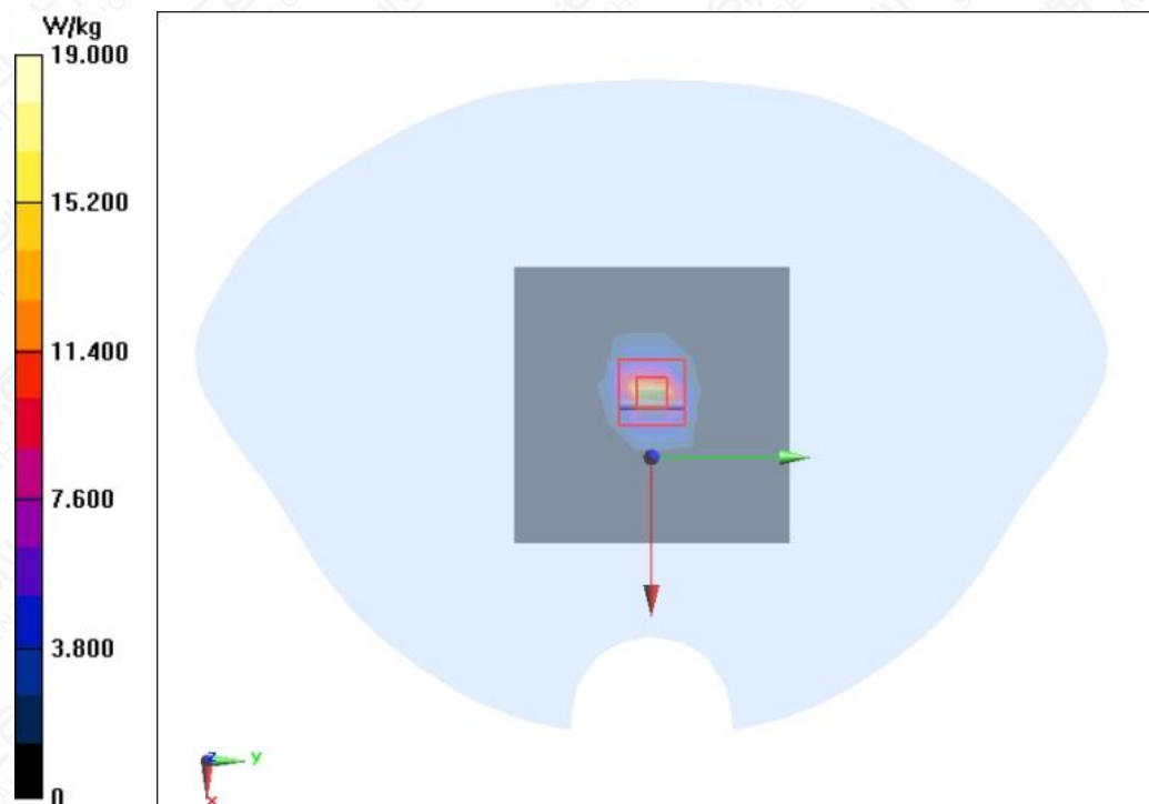
Figure A.2-13 Head 5200MHz
