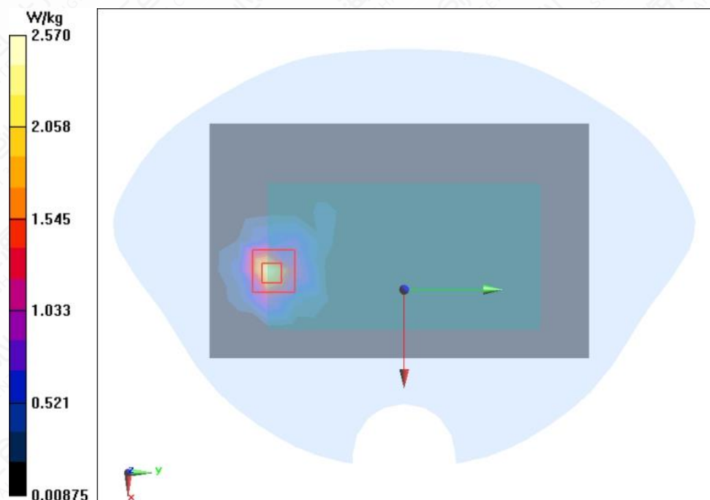
Figure A.1-22 LTE B41 20MHz 1RB 50offset Back Mode Middle 0mm
