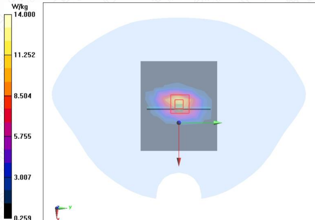
Figure A.2-5 Head 1750MHz
