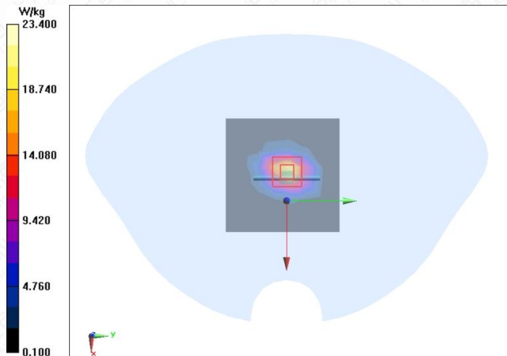
Figure A.2-11 Head 2600MHz
