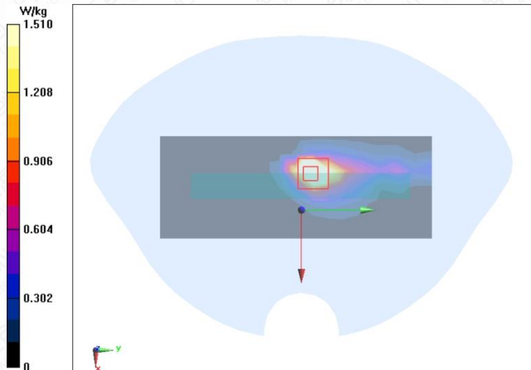
Figure A.1-28 Wi-Fi 5G U-NII-1 11a Left Mode Low 0mm
