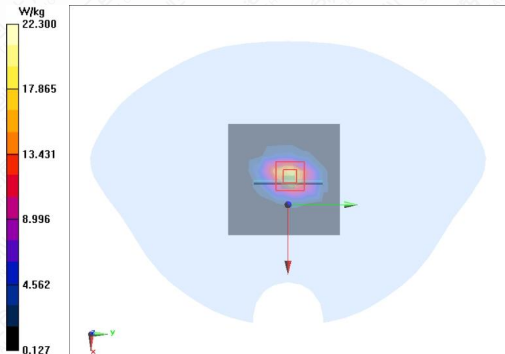
Figure A.2-10 Head 2450MHz
