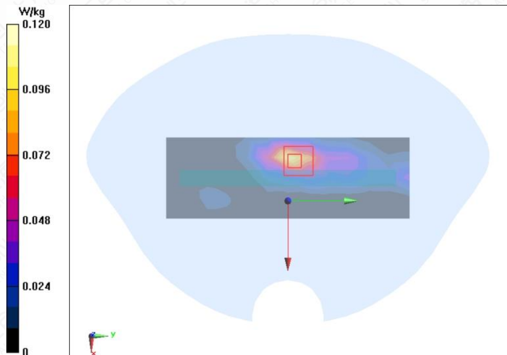
Figure A.1-24 BT DH5 Left Mode Middle 0mm
