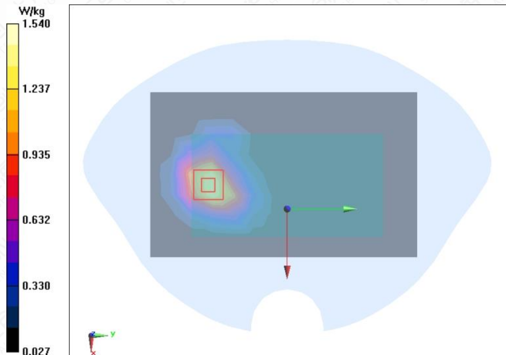
Figure A.1-11 LTE B2 20MHz 50RB 50offset Back Mode High 5mm
