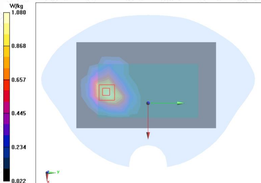
Figure A.1-3 GSM1900 GPRS 2TS Back Mode Middle 5mm
