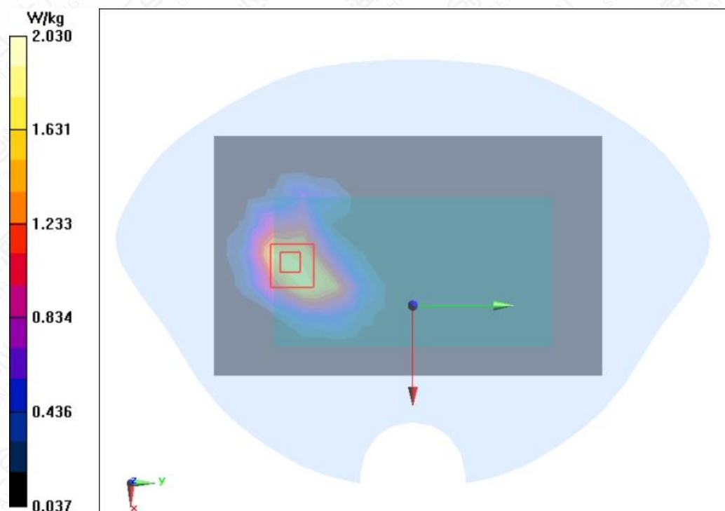
Figure A.1-14 LTE B4 20MHz 50RB 0offset Back Mode Low 0mm
