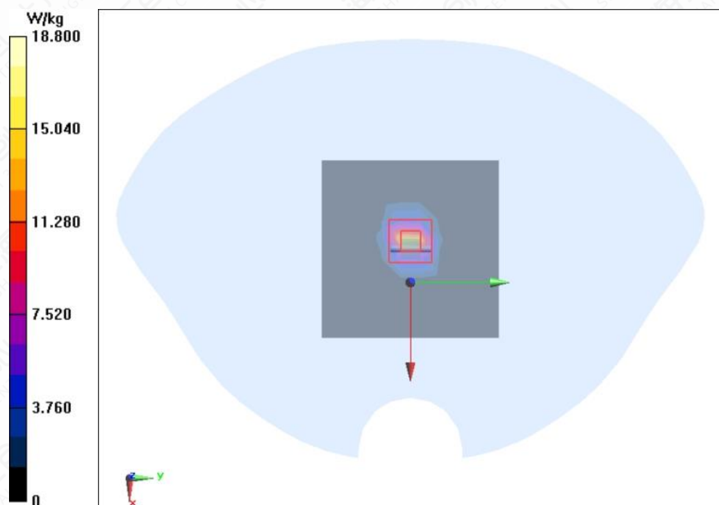
Figure A.2-14 Head 5200MHz
