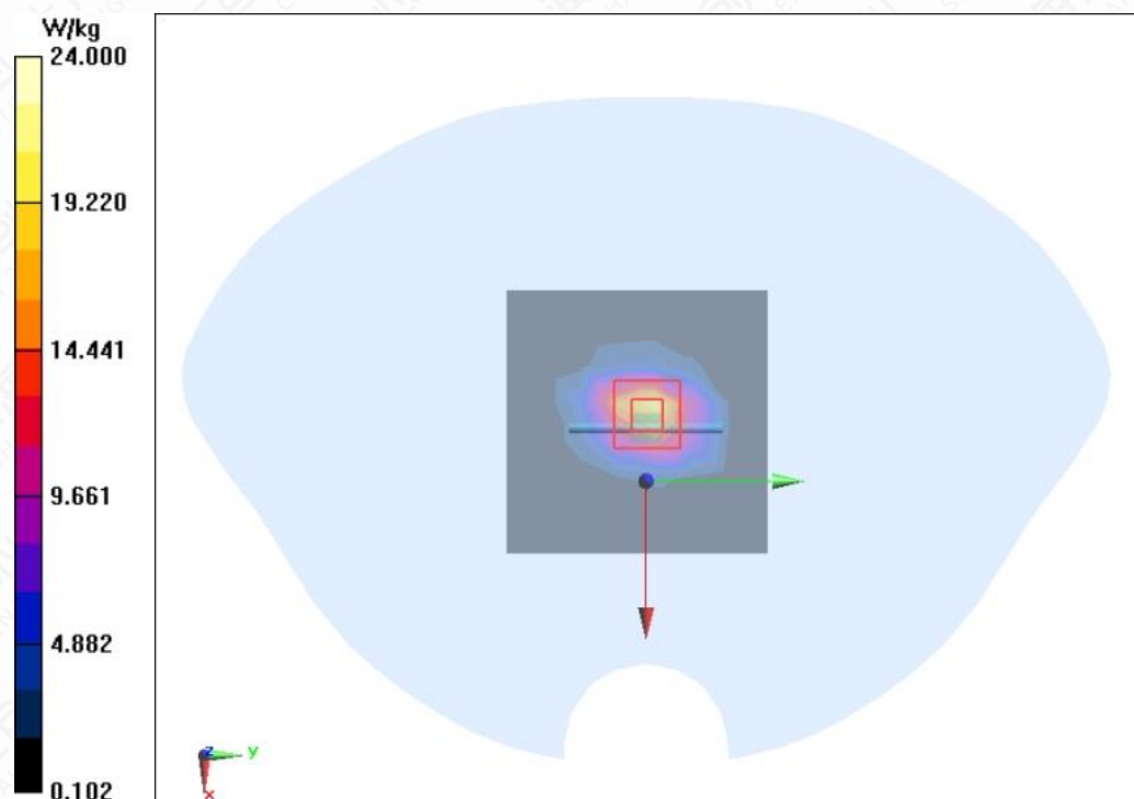
Figure A.2-12 Head 2600MHz
