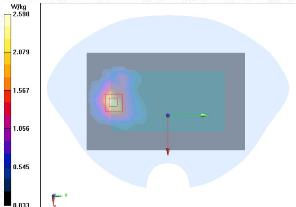
Figure A.1-6 WCDMA Band II Back Mode High 0mm
