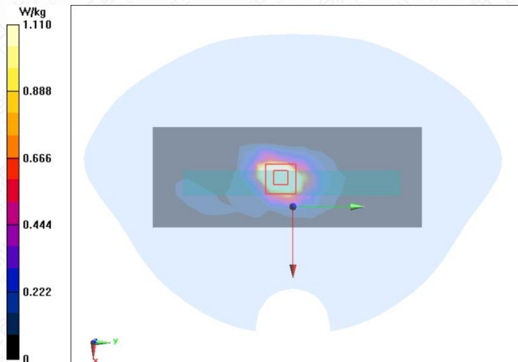
Figure A.1-29 Wi-Fi 5G U-NII-2C 11a Left Mode Middle 5mm
