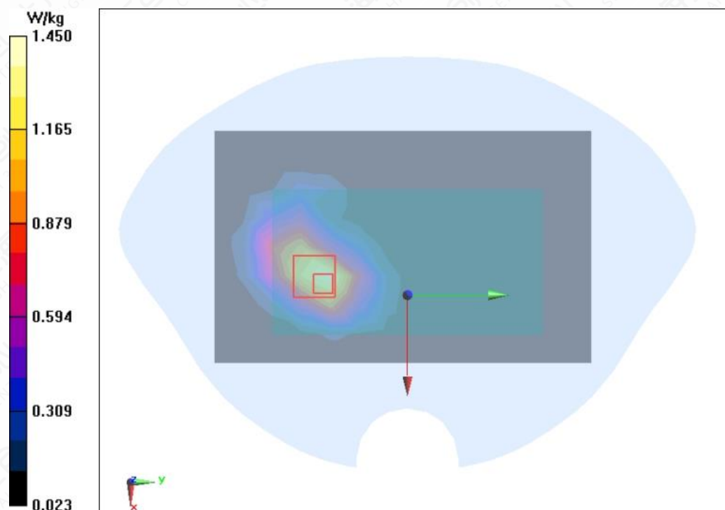
Figure A.1-13 LTE B4 20MHz 1RB 50offset Back Mode Middle 5mm
