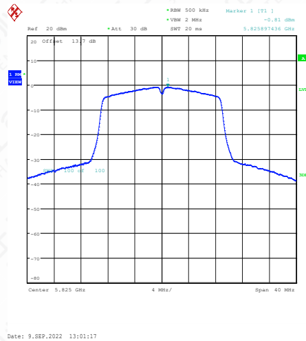
11AC20SISO-Ant1-5825--0.94-0.13-0.00-0.00
