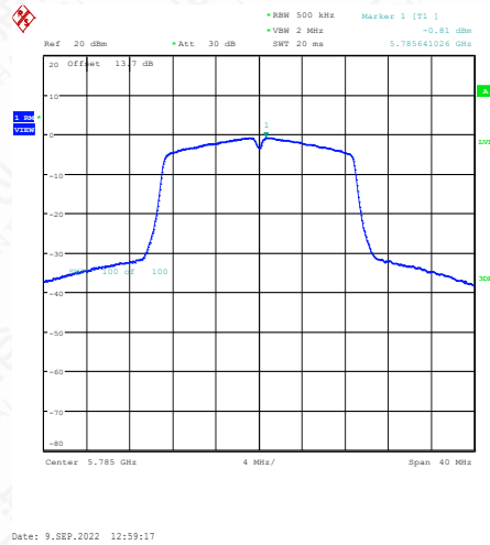
11AC20SISO-Ant1-5785--0.94-0.13-0.00-0.00
