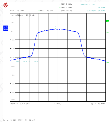
11N20SISO-Ant1-5580-1.96-0.13-0.00-0.00
