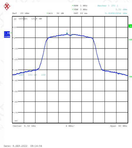
11A-Ant1-5320-3.17-0.15-0.00-0.00
