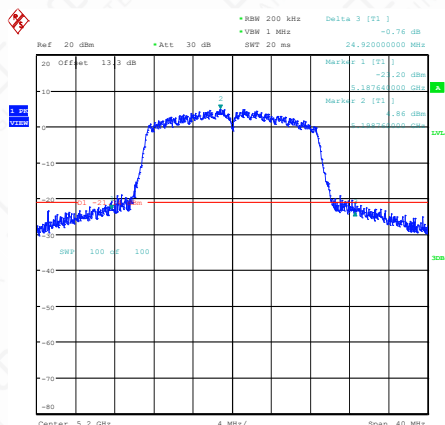
11AC20SISO-Ant1-5180
