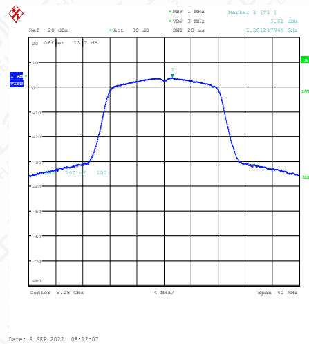
11A-Ant1-5280-3.47-0.15-0.00-0.00
