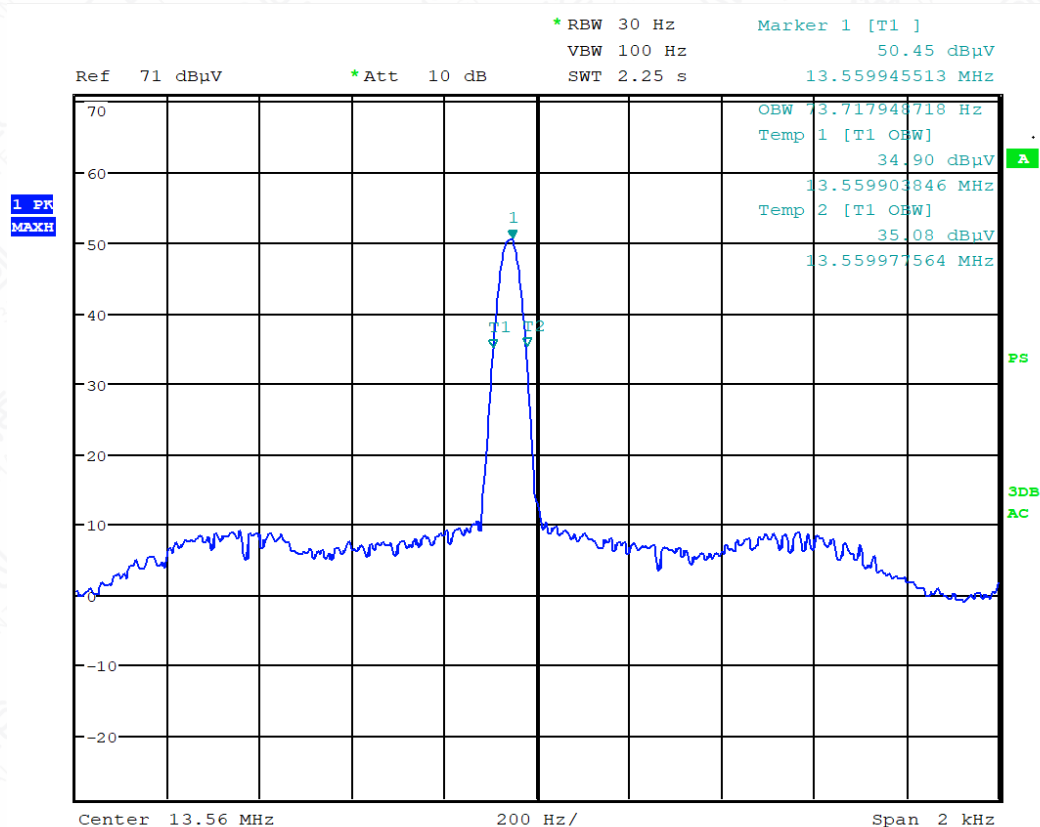
Figure A.4-1 Mode 1 Occupied bandwidth
