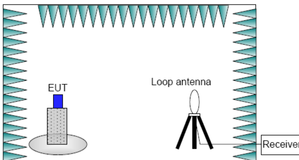
Figure 6.3.1.2-1 Electric Field Strength of Fundamental Emissions Connection Diagram
