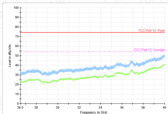
Radiated emission: \pi/4 DQPSK, Ch78, 26.5GHz~40GHz
