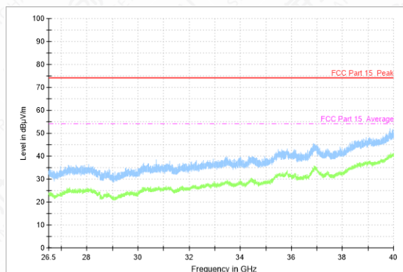
Radiated emission: \pi/4 DQPSK, Ch0, 26.5GHz~40GHz
