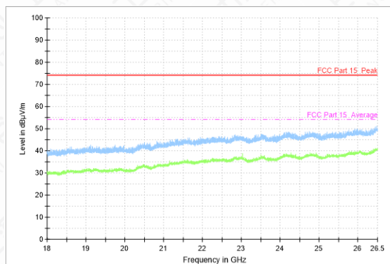
Radiated emission: \pi/4 DQPSK, Ch78, 18GHz~26.5GHz
