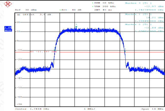
Channel 1450- Emission Bandwidth (-26dBc BW)
