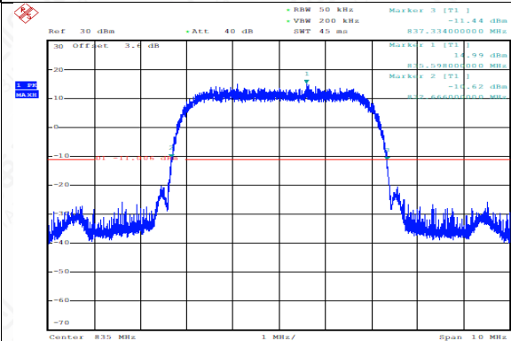
Channel 4175- Emission Bandwidth (-26dBc BW)
