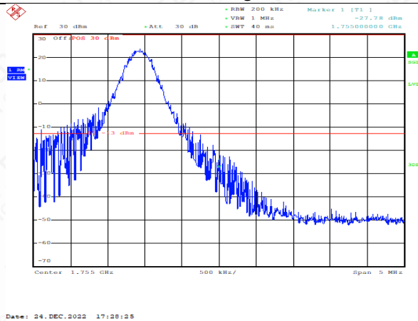
HighRange_FDD04_20MHz_1745_fullRB_High_QPSK
