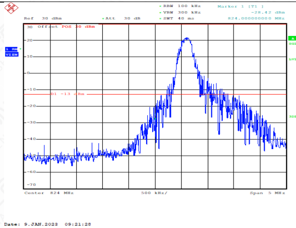
LowRange_FDD05_10MHz_829_fullIRB_Low_QPSK
