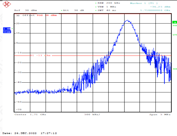
LowRange_FDD04_20MHz_1720_fullRB_Low_QPSK
