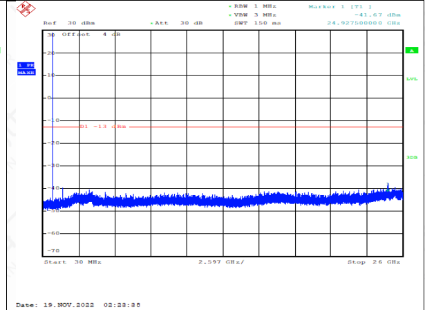
FDD17_MidRange_5MHz_30MHz~26GHz
