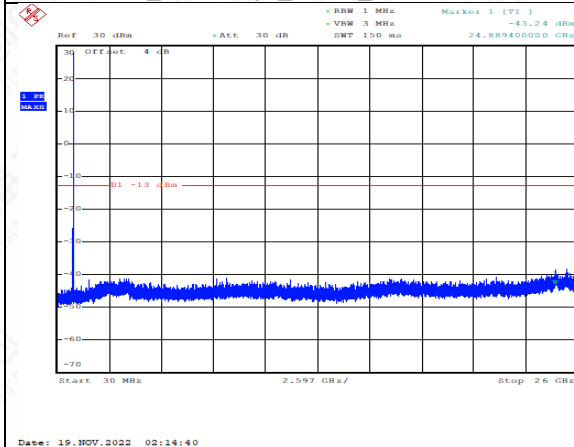
FDD05_HighRange_5MHz_30MHz~26GHz
