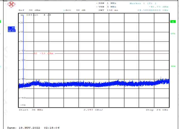
FDD05_MidRange_5MHz_30MHz~26GHz
