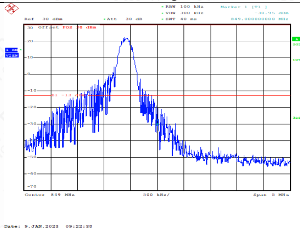
HighRange_FDD05_10MHz_844_fullIRB_High_QPSK
