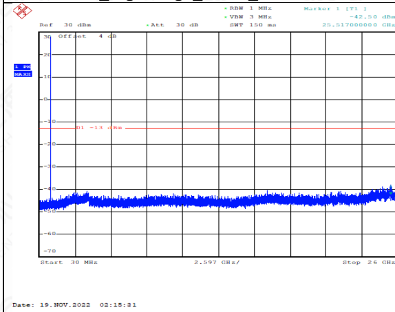
FDD05_HighRange_5MHz_30MHz~26GHz
