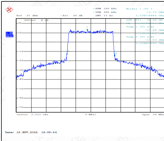
LTE band 7, 15MHz (-26dBc)mid
