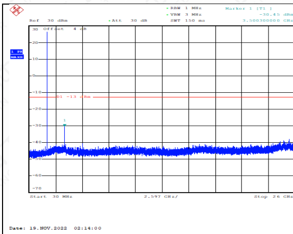
FDD05_LowRange_5MHz_30MHz~26GHz
