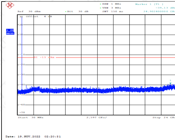
FDD17_LowRange_5MHz_30MHz~26GHz
