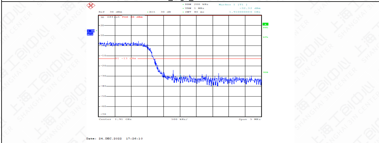
HighRange_FDD02_20MHz_1900_fullRB _High_QPSK
