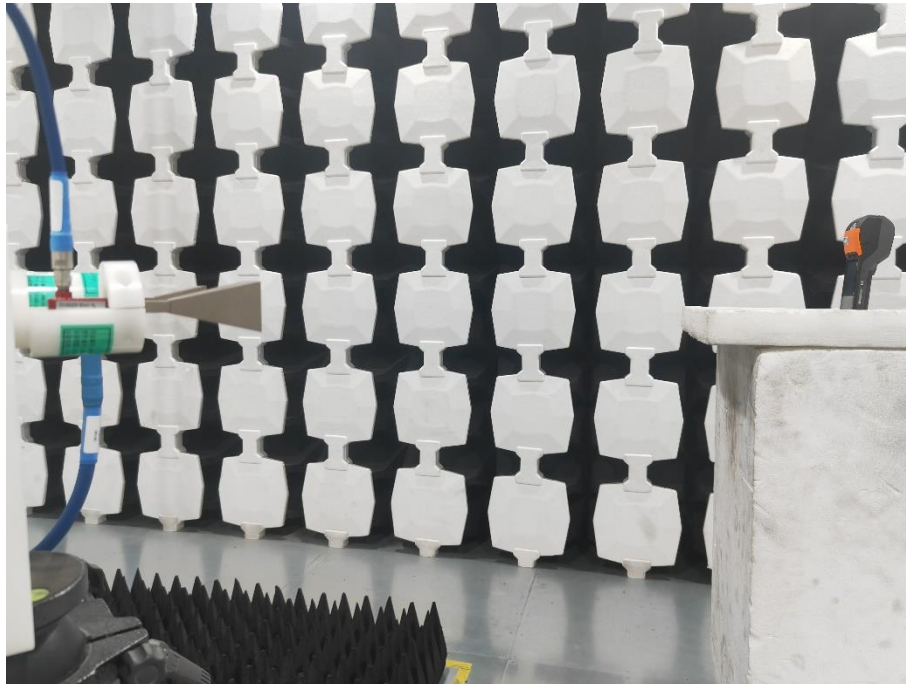
Description: Radiated Emission Test Setup (18GHz -40GHz)
