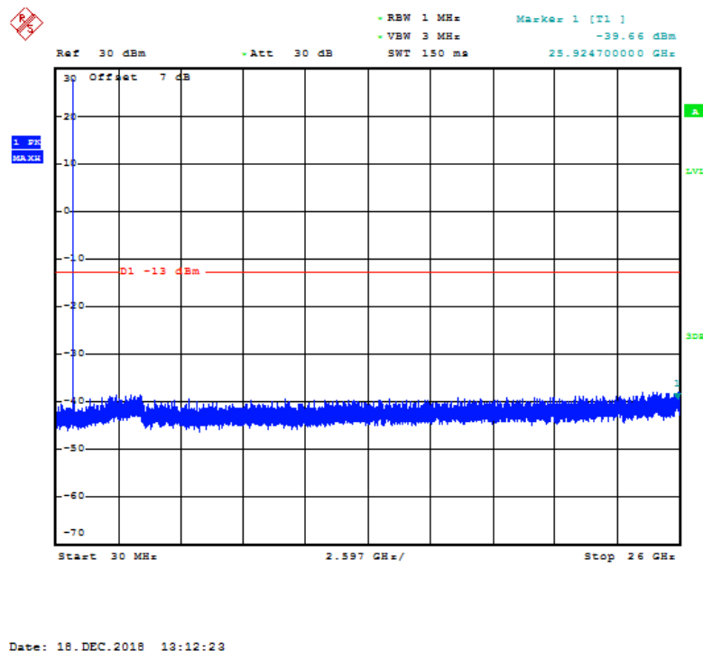
Fig.92 LTE band 17: 30MHz – 26GHz
