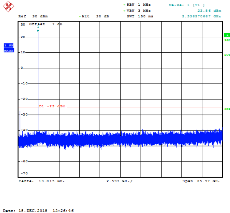
Fig.91 LTE band 7: 30MHz – 26GHz
