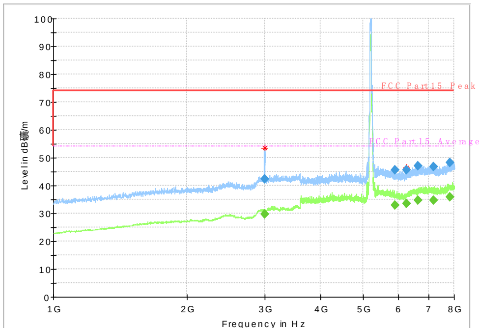
Fig. 48 Radiated Spurious Emission (802.11n-HT40, ch38, 1 GHz-8 GHz)
