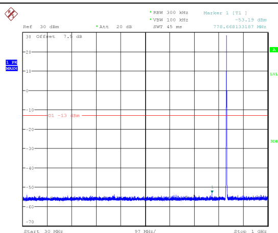
Channel 189: 30MHz~1GHz
