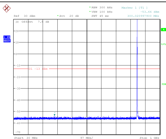
Channel 251: 30MHz~1GHz
