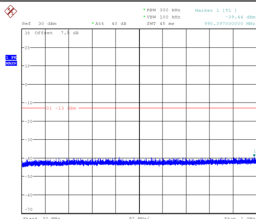
Channel 9263: 30MHz~1GHz
