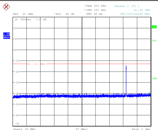
Channel 4175: 30MHz~1GHz
