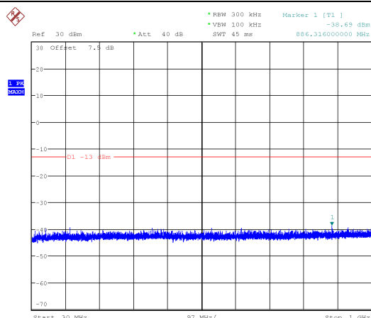
Channel 1313: 30MHz~1GHz
