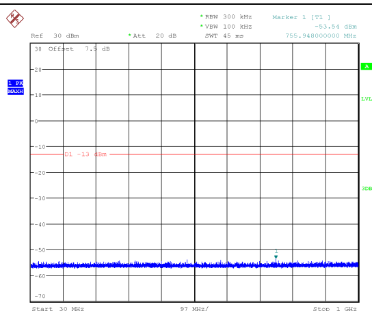
Channel 661: 30MHz~1GHz
