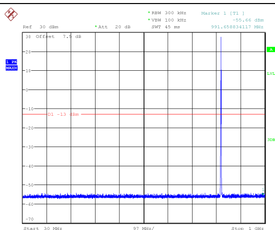
Channel 128: 30MHz~1GHz
