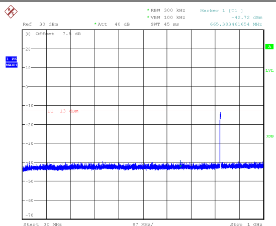
Channel 4232: 30MHz~1GHz
