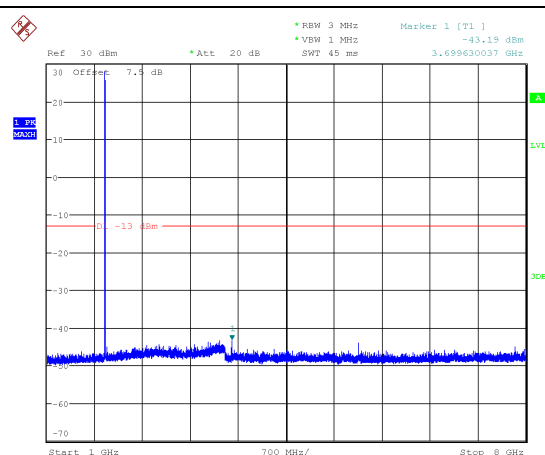
Channel 512: 1GHz~8GHz
