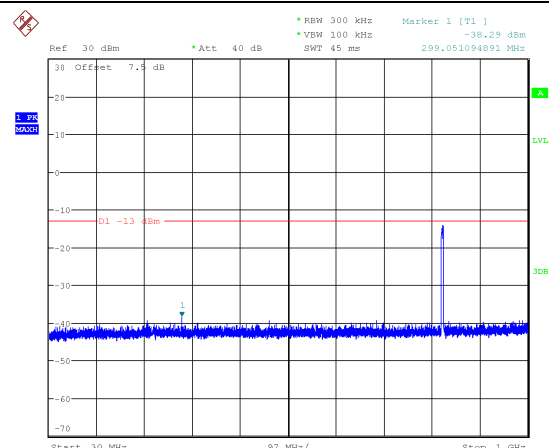
Channel 4133: 30MHz~1GHz
