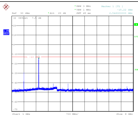
Channel 251: 1GHz~8GHz
