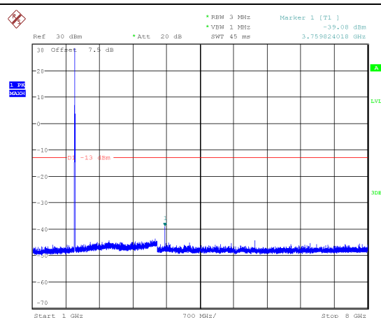
Channel 661: 1GHz~8GHz
