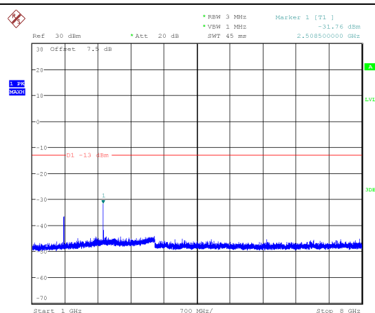
Channel 189: 1GHz~8GHz
