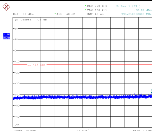
Channel 9537: 30MHz~1GHz
