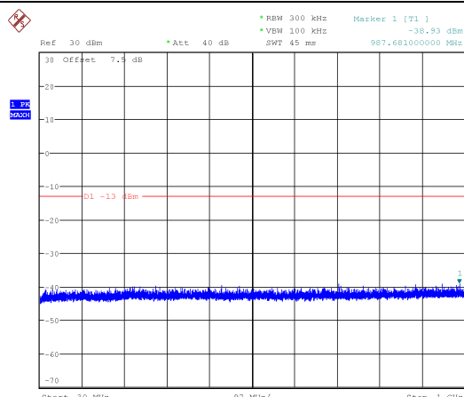
Channel 1450: 30MHz~1GHz
