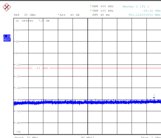
Channel 1512: 30MHz~1GHz
