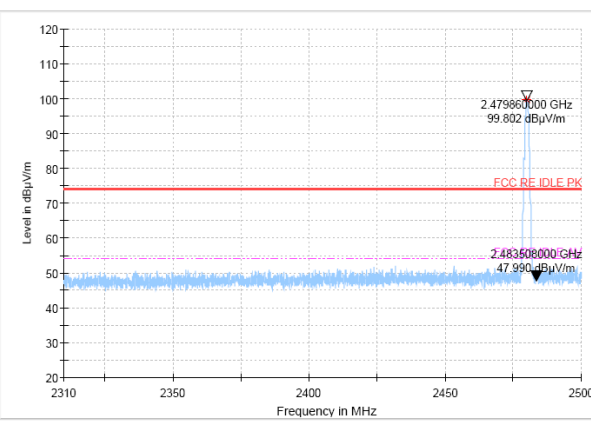
Bandedge (High): GFSK, high channel
