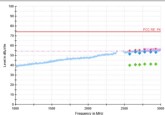
Bandedge:Ch39
