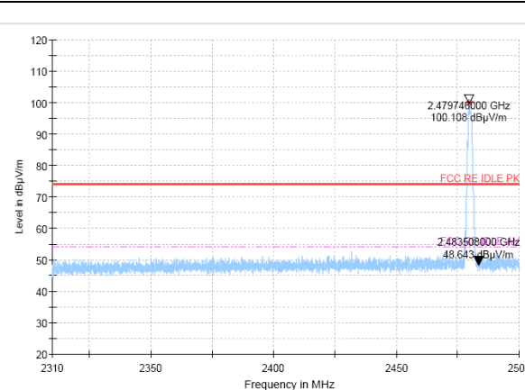
Bandedge:Ch39
