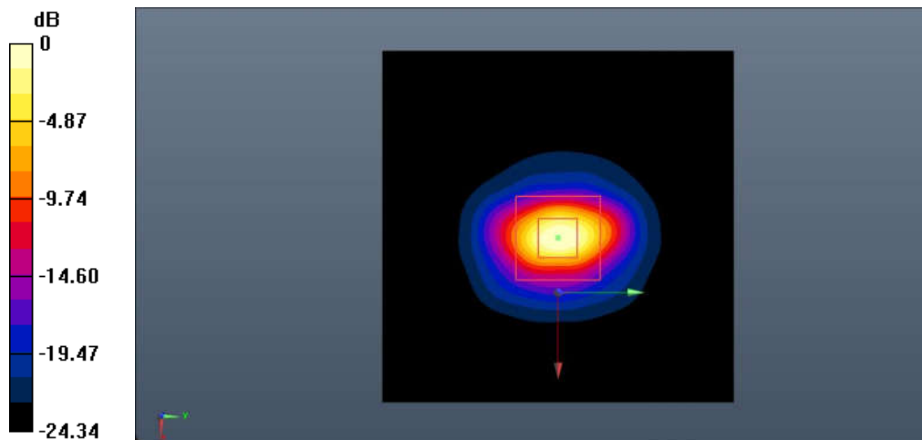
Fig.B.10. Check 2550MHz 50mW
