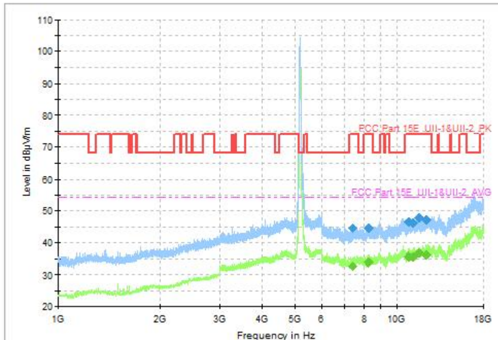
Fig. 52 Transmitter Spurious Emission (802.11ac-VHT40, CH38 5190MHz, 1GHz-18GHz)
