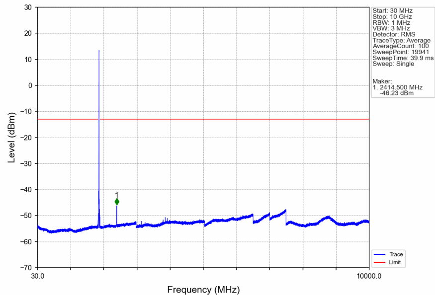
Band2_HSDPA_MCH_1880MHz_Subtest 1_NTNV
