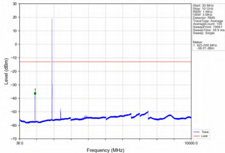
Band25_3MHz_QPSK_HCH_1913.5MHz_RB_1_0_NTNV
