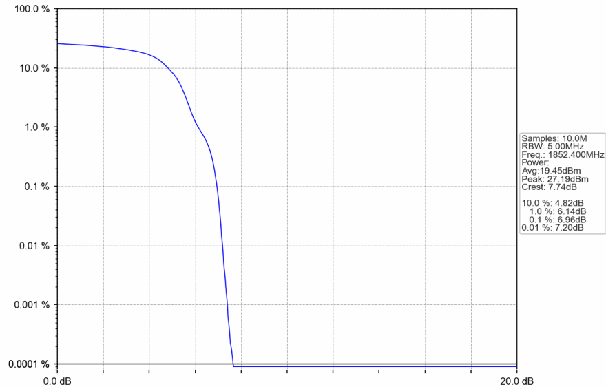
Band2_HSUPA_LCH_1852.4MHz_Subtest 1_NTNV
