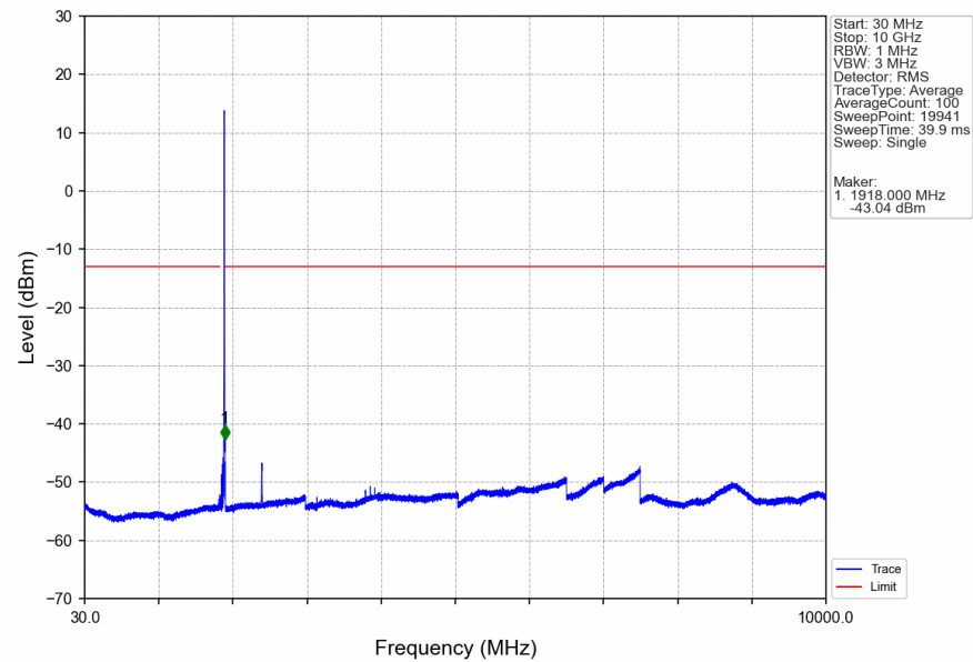
Band2_HSUPA_HCH_1907.6MHz_Subtest 1_NTNV
