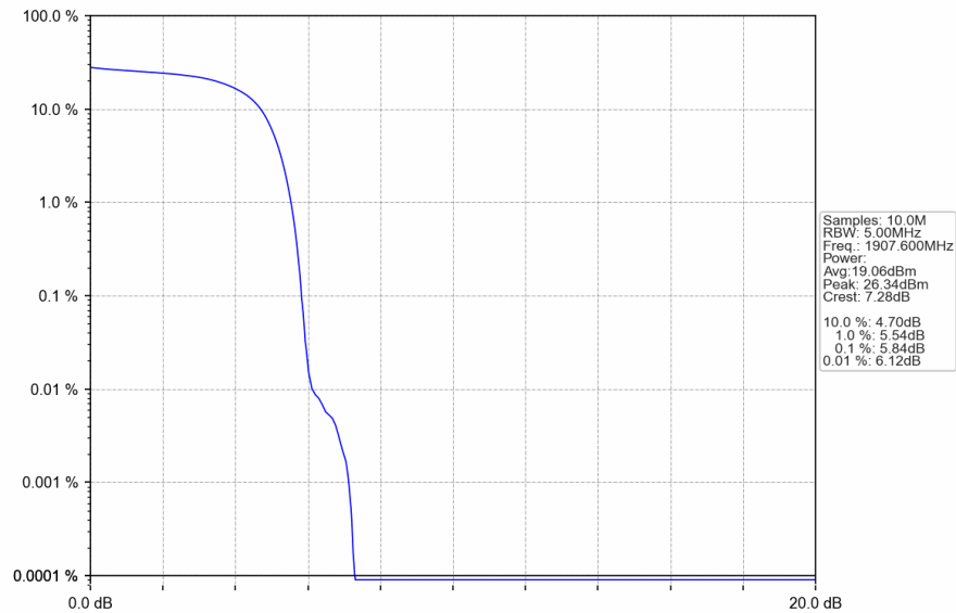
Band2_HSDPA_HCH_1907.6MHz_Subtest 1_NTNV
