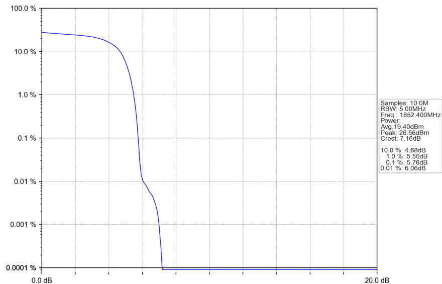
Band2_HSDPA_LCH_1852.4MHz_Subtest 1_NTNV
