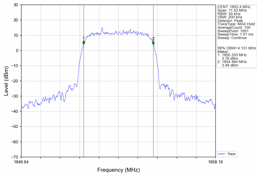
Band2_HSDPA_LCH_1852.4MHz_Subtest 1_NTNV
