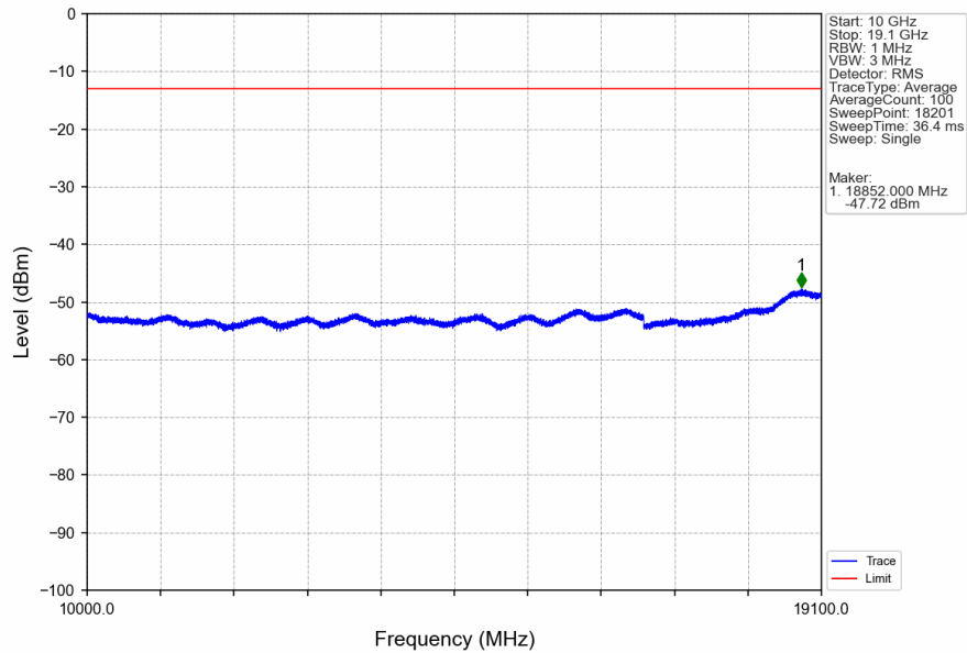
Band2_RMC_MCH_1880MHz_12.2kbps RMC_NTNV
