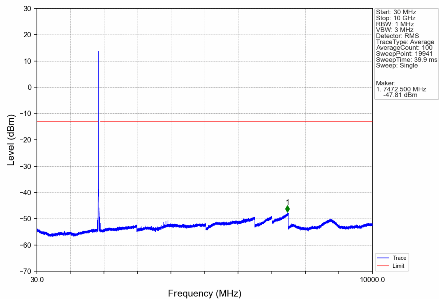
Band2_HSDPA_LCH_1852.4MHz_Subtest 1_NTNV
