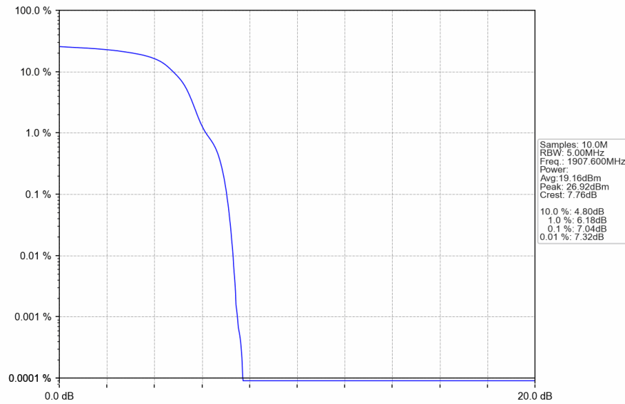
Band2_HSUPA_HCH_1907.6MHz_Subtest 1_NTNV
