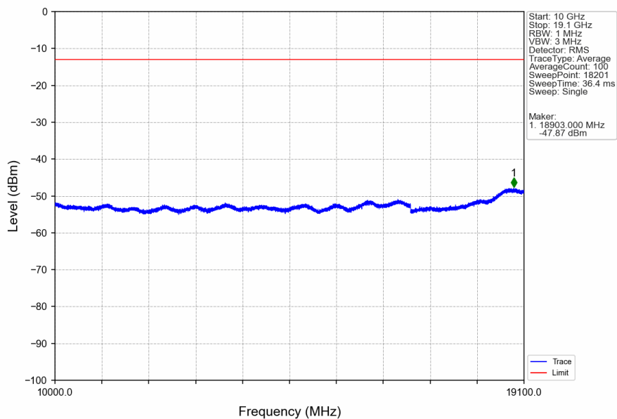
Band2_HSDPA_HCH_1907.6MHz_Subtest 1_NTNV
