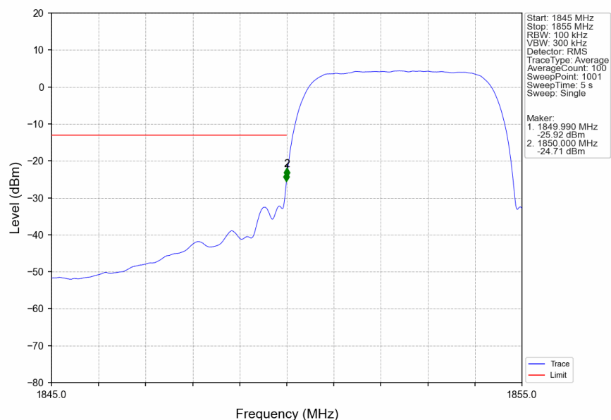
Band2_HSDPA_LCH_1852.4MHz_Subtest 1_NTNV
