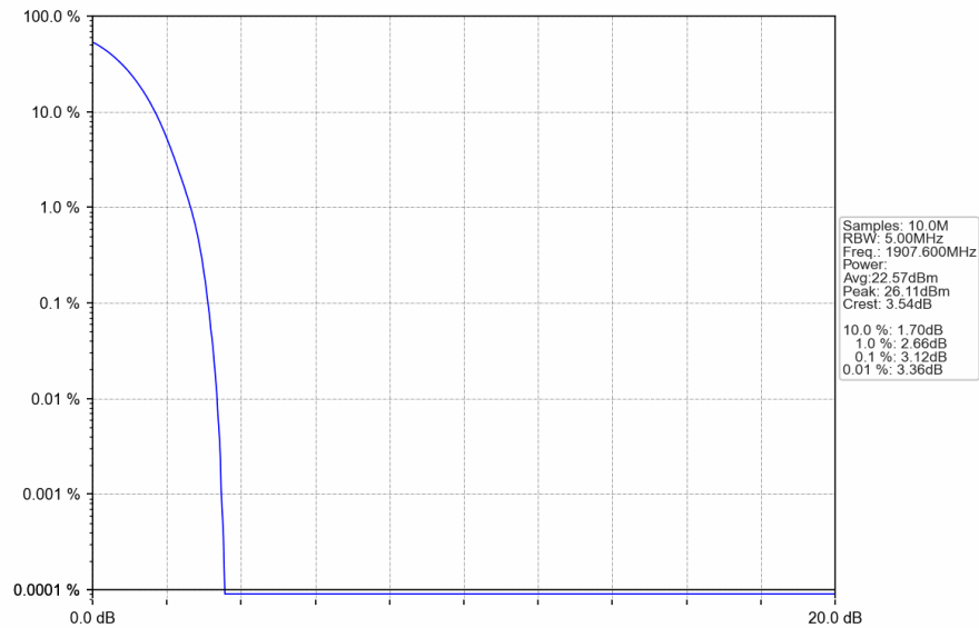
Band2_RMC_HCH_1907.6MHz_12.2kbps RMC_NTNV
