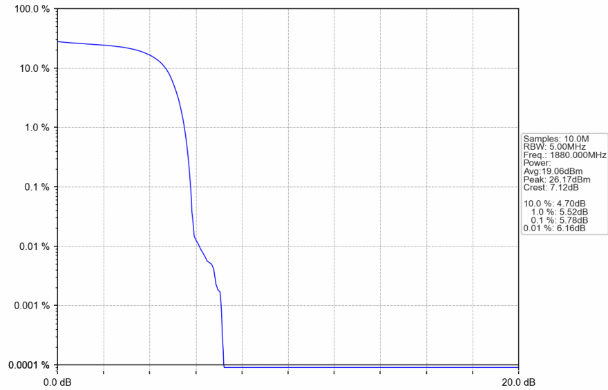
Band2_HSDPA_MCH_1880MHz_Subtest 1_NTNV
