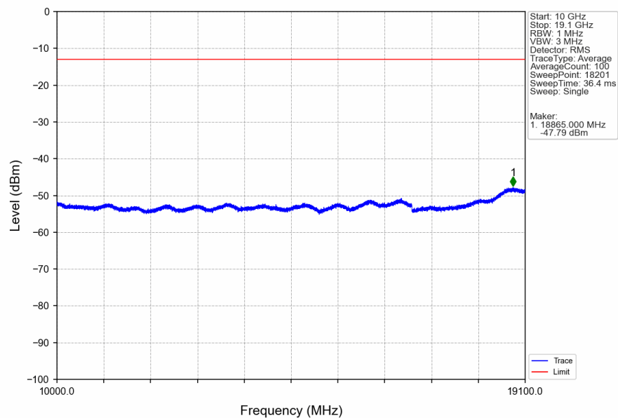
Band2_HSUPA_HCH_1907.6MHz_Subtest 1_NTNV
