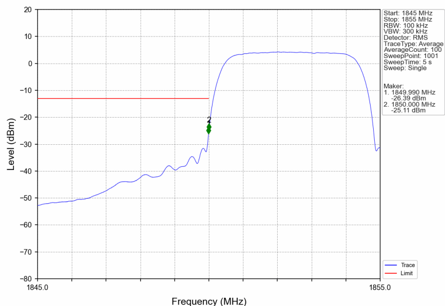
Band2_HSUPA_LCH_1852.4MHz_Subtest 1_NTNV
