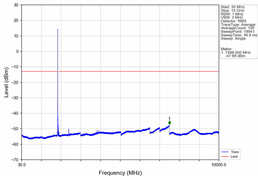
Band2_HSUPA_LCH_1852.4MHz_Subtest 1_NTNV
