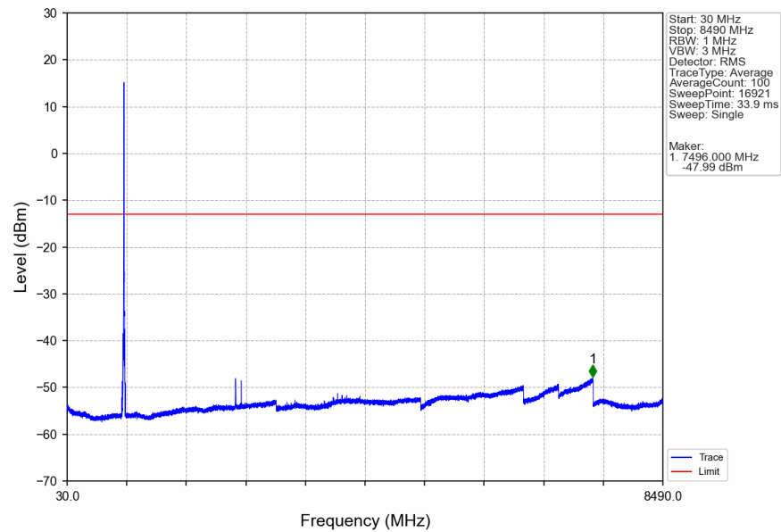
Band5_HSUPA_HCH_846.6MHz_Subtest 1_NTNV
