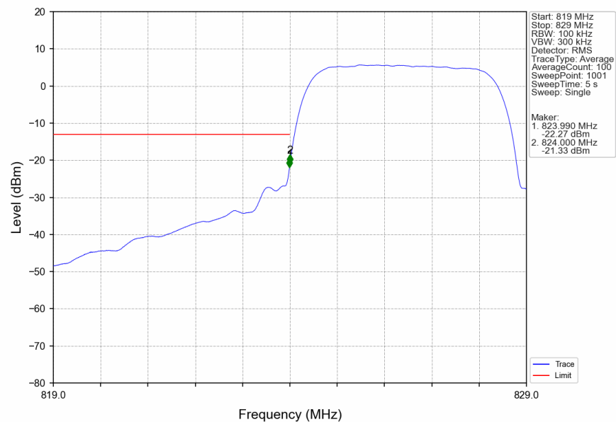
Band5_HSDPA_LCH_826.4MHz_Subtest 1_NTNV
