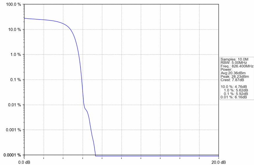
Band5_HSDPA_LCH_826.4MHz_Subtest 1_NTNV
