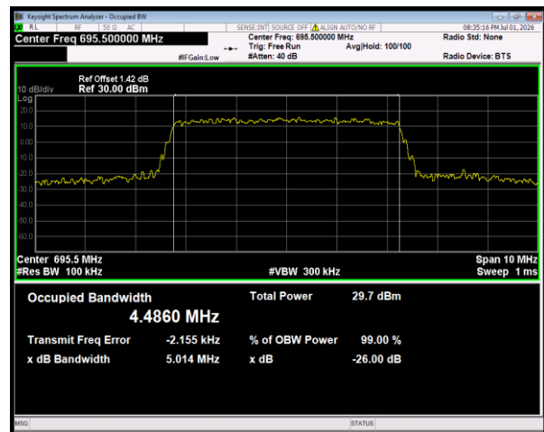
Band71 QPSK BW=5MHz Channel=133447 RB Size=25 Position=#0
