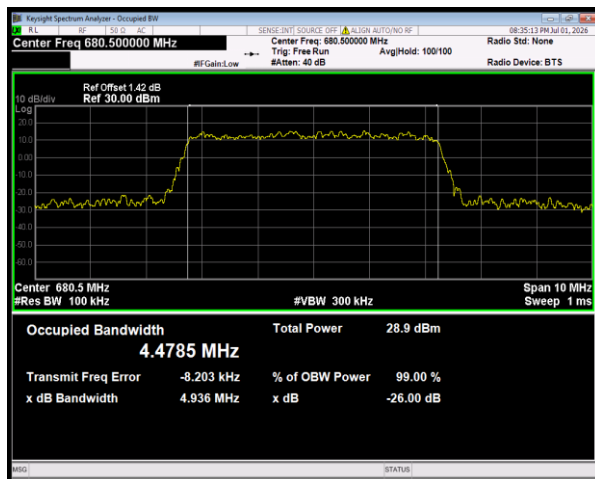
Band71 64QAM BW=5MHz Channel=133297 RB Size=25 Position=#0
