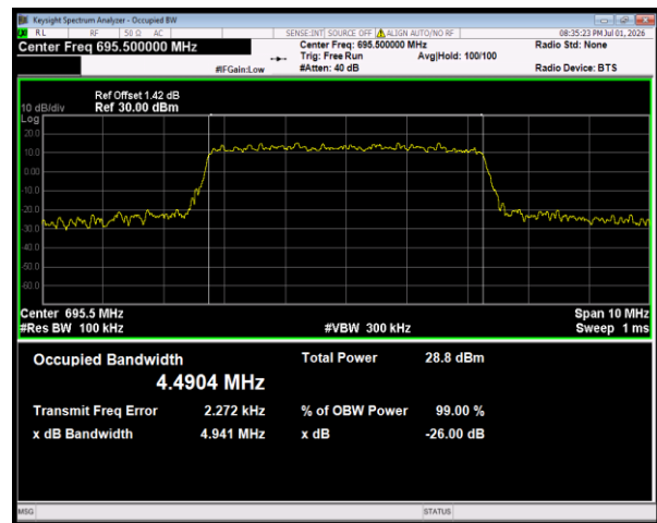
Band71 64QAM BW=5MHz Channel=133447 RB Size=25 Position=#0
