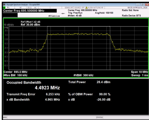
Band71 16QAM BW=5MHz Channel=133447 RB Size=25 Position=#0
