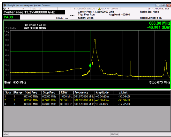
Band71 64QAM BW=10MHz LowChannel=133172 RB Size=1 Position=#0
