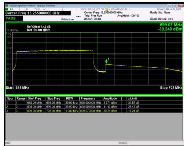
Band71 64QAM BW=10MHz HighChannel=133422 RB Size=50 Position=#0
