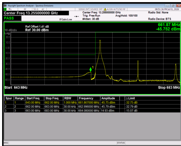
Band71 16QAM BW=20MHz LowChannel=133222 RB Size=1 Position=#0
