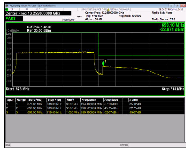
Band71 64QAM BW=20MHz HighChannel=133372 RB Size=100 Position=#0
