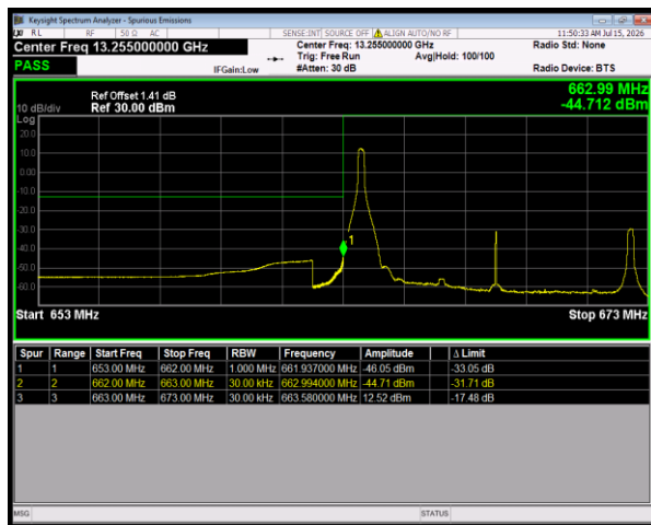
Band71 16QAM BW=10MHz LowChannel=133172 RB Size=1 Position=#0
