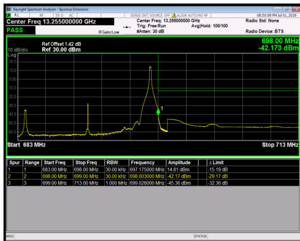
Band71 64QAM BW=15MHz HighChannel=133397 RB Size=1 Position=#Max
