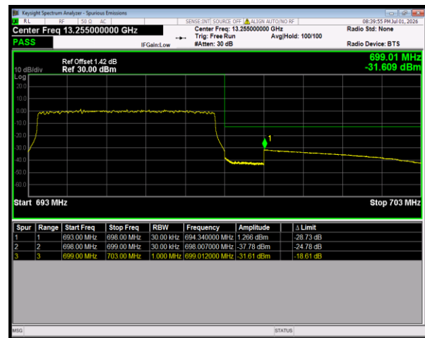
Band71 16QAM BW=5MHz HighChannel=133447 RB Size=25 Position=#0
