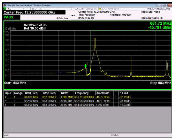
Band71 64QAM BW=20MHz LowChannel=133222 RB Size=1 Position=#0
