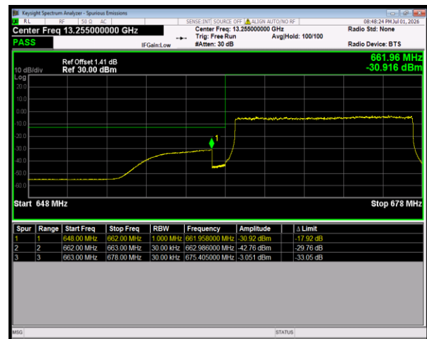
Band71 64QAM BW=15MHz LowChannel=133197 RB Size=75 Position=#0
