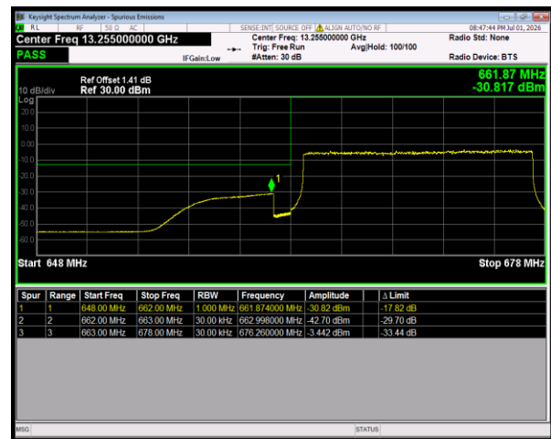
Band71 16QAM BW=15MHz LowChannel=133197 RB Size=75 Position=#0
