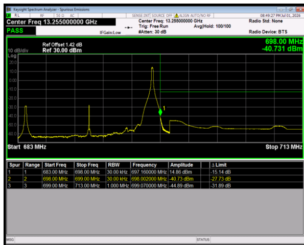
Band71 16QAM BW=15MHz HighChannel=133397 RB Size=1 Position=#Max
