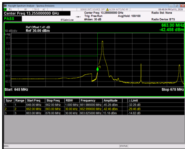
Band71 64QAM BW=15MHz LowChannel=133197 RB Size=1 Position=#0
