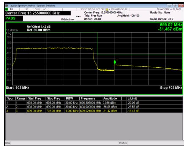
Band71 64QAM BW=5MHz HighChannel=133447 RB Size=25 Position=#0
