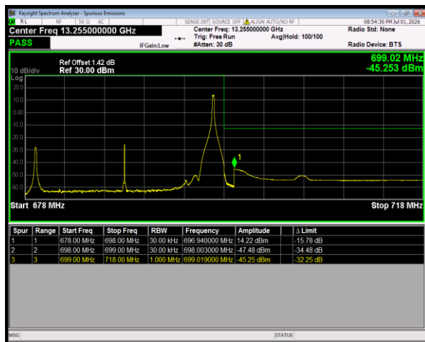
Band71 64QAM BW=20MHz HighChannel=133372 RB Size=1 Position=#Max
