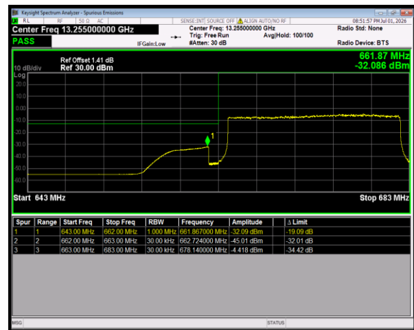
Band71 16QAM BW=20MHz LowChannel=133222 RB Size=100 Position=#0
