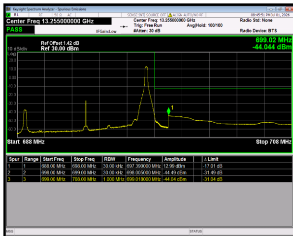
Band71 64QAM BW=10MHz HighChannel=133422 RB Size=1 Position=#Max
