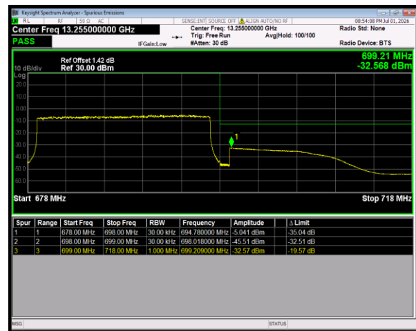
Band71 16QAM BW=20MHz HighChannel=133372 RB Size=100 Position=#0
