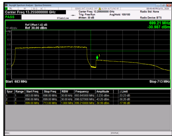
Band71 16QAM BW=15MHz HighChannel=133397 RB Size=75 Position=#0
