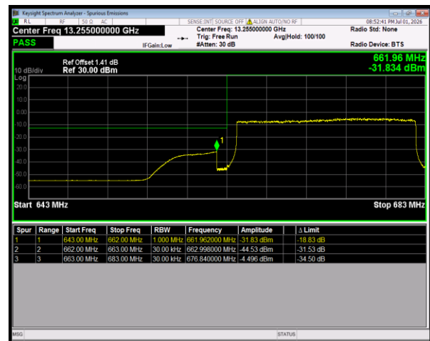
Band71 64QAM BW=20MHz LowChannel=133222 RB Size=100 Position=#0
