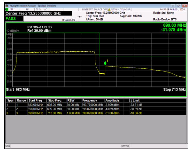
Band71 64QAM BW=15MHz HighChannel=133397 RB Size=75 Position=#0
