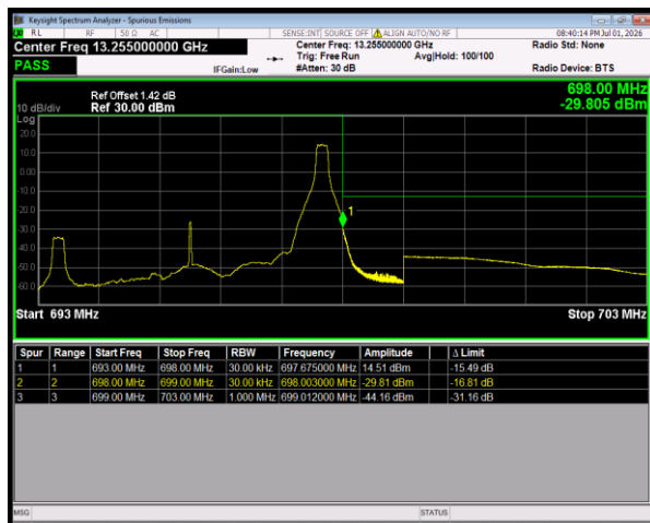
Band71 64QAM BW=5MHz HighChannel=133447 RB Size=1 Position=#Max
