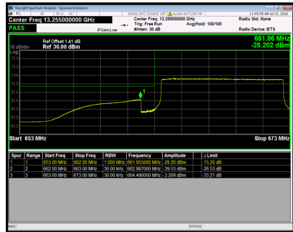
Band71 QPSK BW=10MHz LowChannel=133172 RB Size=50 Position=#0
