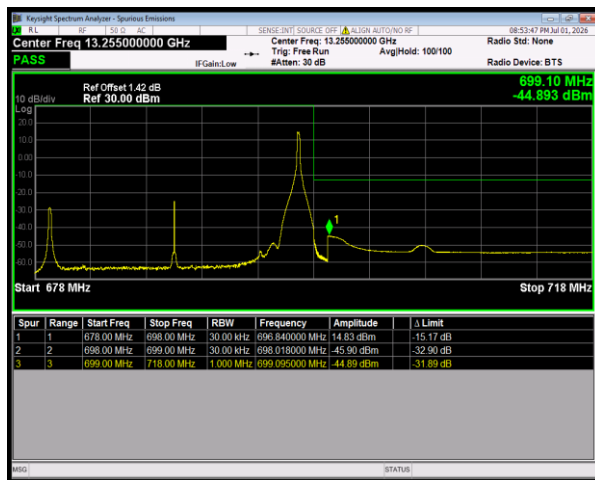
Band71 16QAM BW=20MHz HighChannel=133372 RB Size=1 Position=#Max
