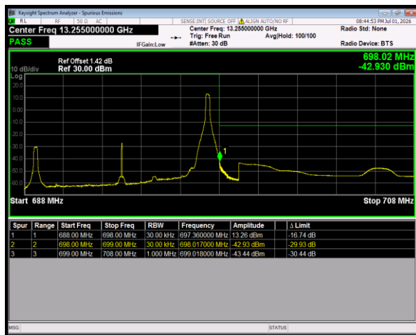
Band71 16QAM BW=10MHz HighChannel=133422 RB Size=1 Position=#Max
