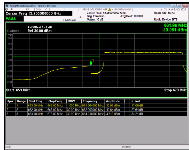
Band71 64QAM BW=10MHz LowChannel=133172 RB Size=50 Position=#0
