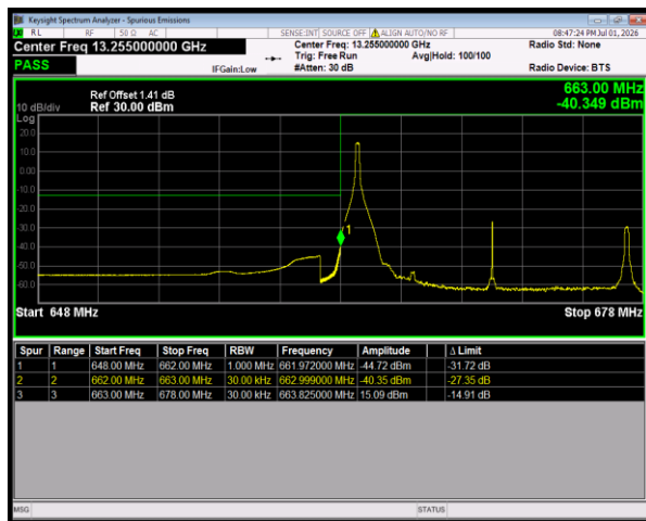
Band71 16QAM BW=15MHz LowChannel=133197 RB Size=1 Position=#0
