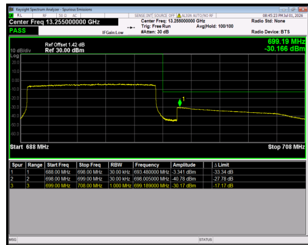
Band71 16QAM BW=10MHz HighChannel=133422 RB Size=50 Position=#0
