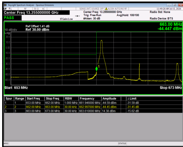
Band71 QPSK BW=10MHz LowChannel=133172 RB Size=1 Position=#0
