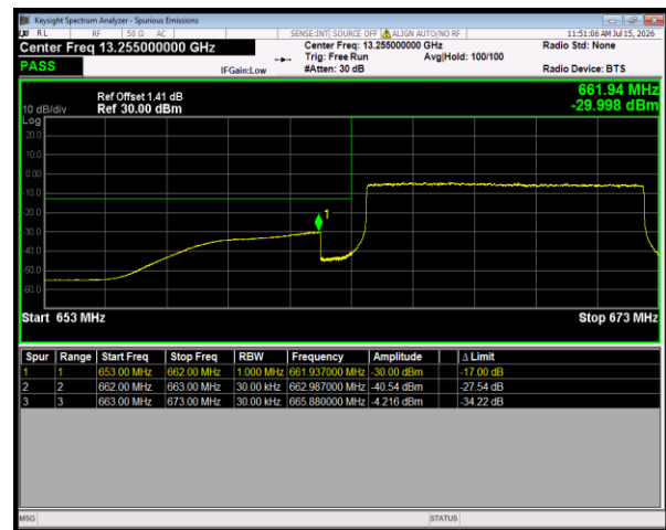
Band71 16QAM BW=10MHz LowChannel=133172 RB Size=50 Position=#0
