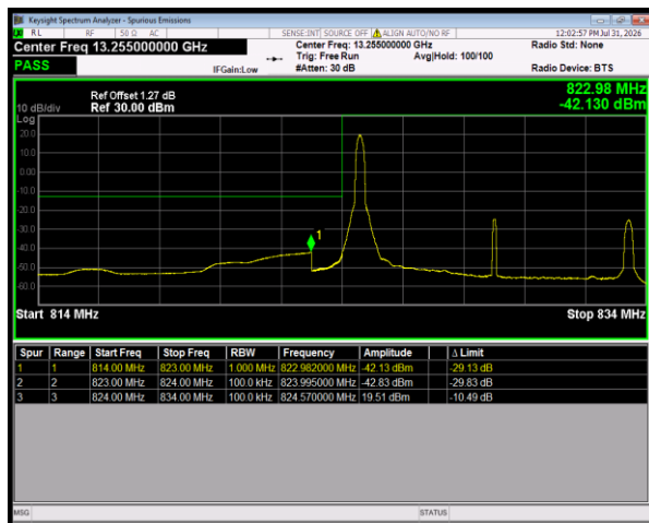
Band26(824-849) QPSK BW=10MHz LowChannel=26840 RB Size=1 Position=#0
