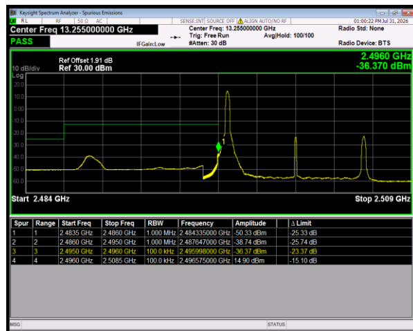
Band41 QPSK BW=10MHz LowChannel=39700 RB Size=1 Position=#0
