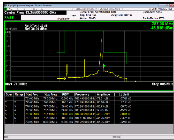
Band13 QPSK BW=10MHz HighChannel=23230 RB Size=1 Position=#Max
