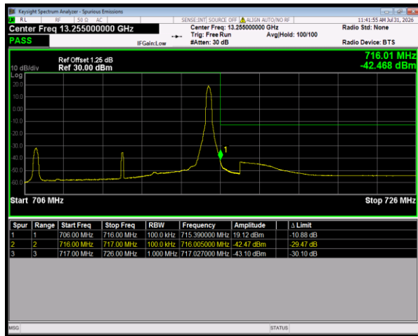
Band17 QPSK BW=10MHz HighChannel=23800 RB Size=1 Position=#Max
