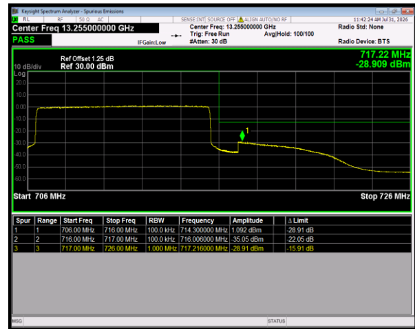
Band17 QPSK BW=10MHz HighChannel=23800 RB Size=50 Position=#0
