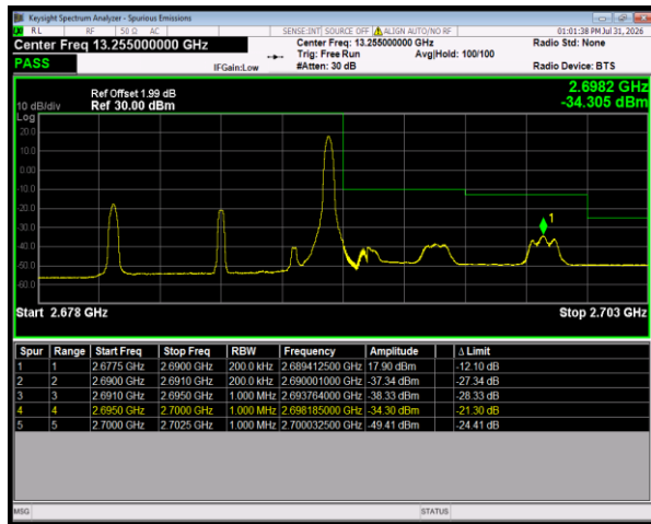
Band41 QPSK BW=10MHz HighChannel=41540 RB Size=1 Position=#Max
