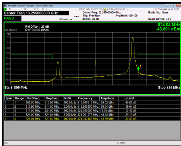
Band26(814-824) QPSK BW=10MHz HighChannel=26740 RB Size=1 Position=#Max
