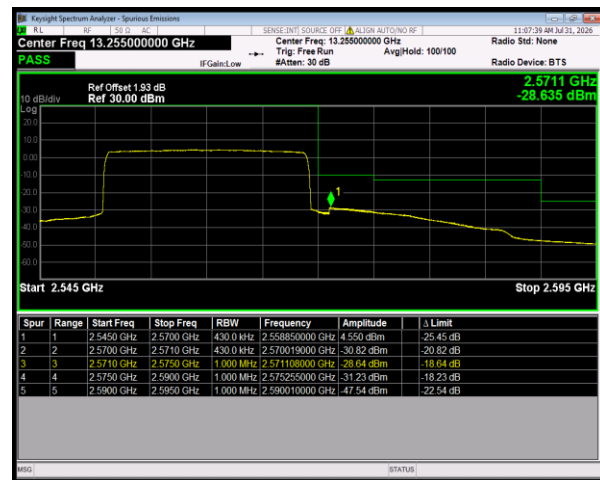
Band7 QPSK BW=20MHz HighChannel=21350 RB Size=100 Position=#0
