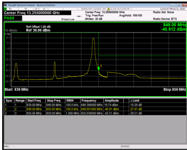
Band26(824-849) QPSK BW=10MHz HighChannel=26990 RB Size=1 Position=#Max
