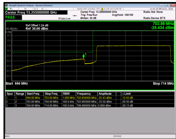
Band17 QPSK BW=10MHz LowChannel=23780 RB Size=50 Position=#0
