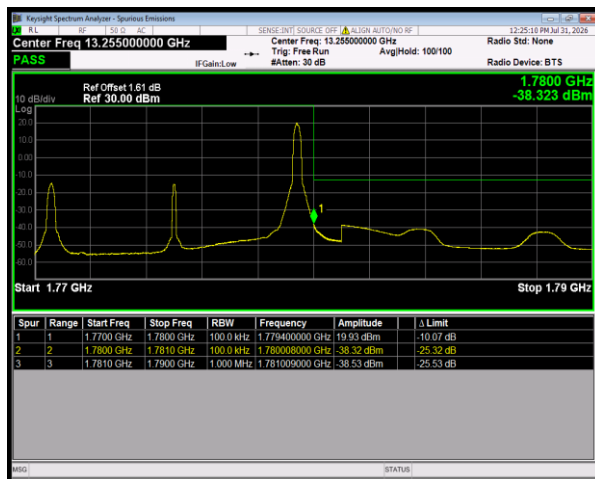
Band66 QPSK BW=10MHz HighChannel=132622 RB Size=1 Position=#Max
