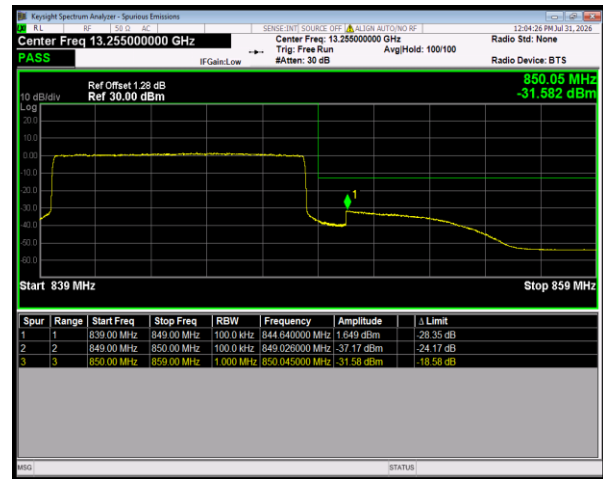
Band26(824-849) QPSK BW=10MHz HighChannel=26990 RB Size=50 Position=#0
