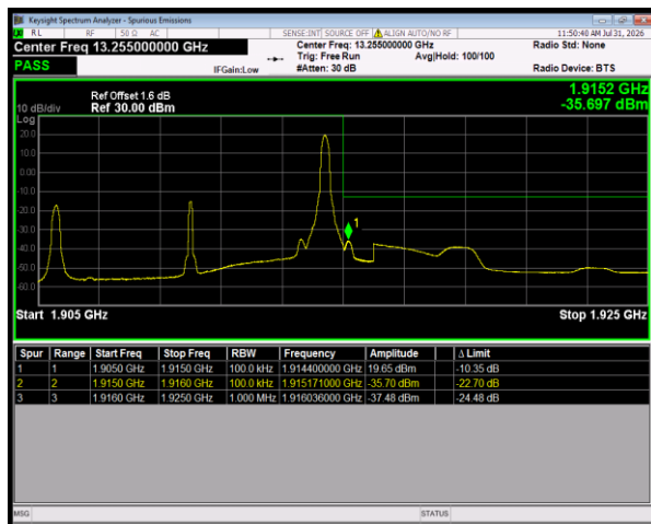
Band25 QPSK BW=10MHz HighChannel=26640 RB Size=1 Position=#Max
