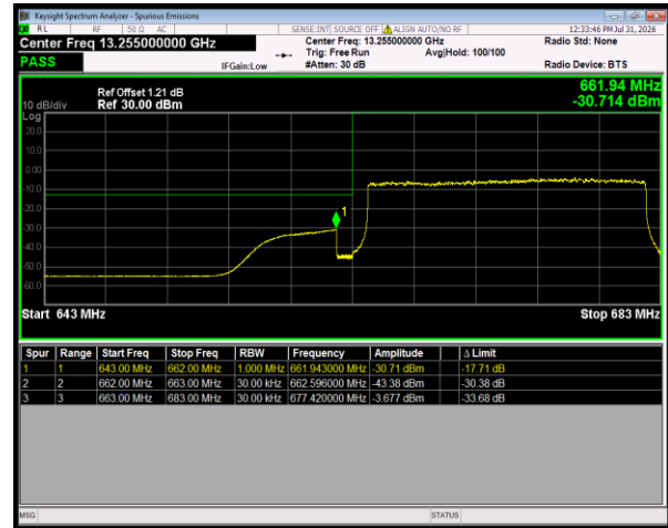
Band71 QPSK BW=20MHz LowChannel=133222 RB Size=100 Position=#0
