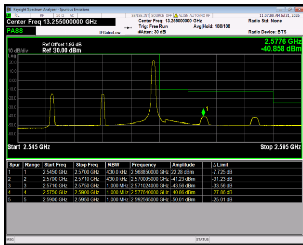
Band7 QPSK BW=20MHz HighChannel=21350 RB Size=1 Position=#Max
