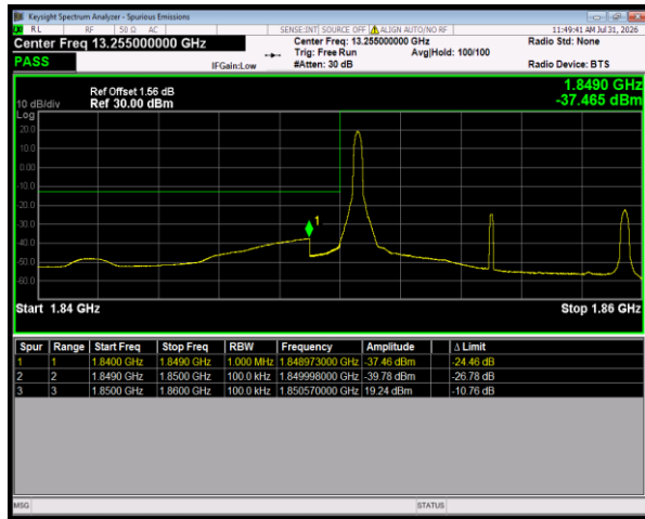
Band25 QPSK BW=10MHz LowChannel=26090 RB Size=1 Position=#0
