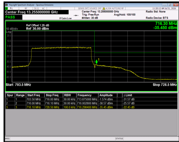
Band12 QPSK BW=10MHz HighChannel=23130 RB Size=50 Position=#0
