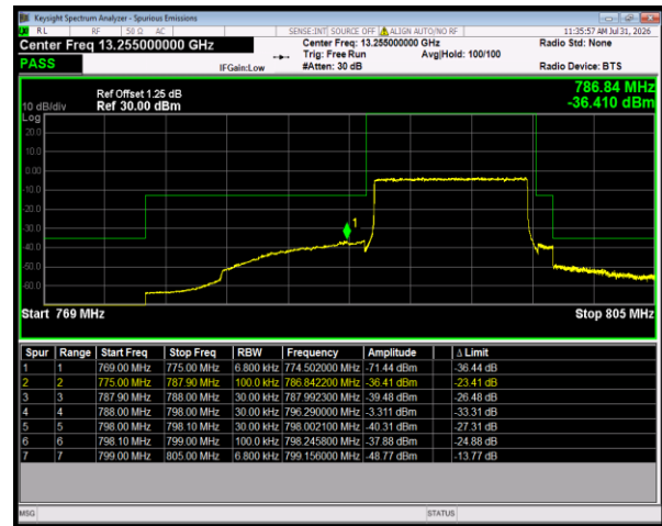
Band14 QPSK BW=10MHz LowChannel=23330 RB Size=50 Position=#0
