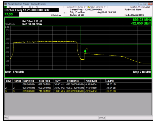
Band71 QPSK BW=20MHz HighChannel=133372 RB Size=100 Position=#0
