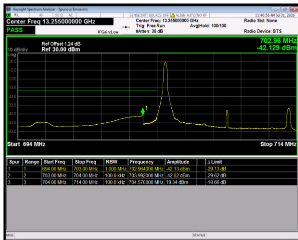
Band17 QPSK BW=10MHz LowChannel=23780 RB Size=1 Position=#0
