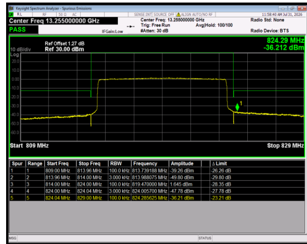
Band26(814-824) QPSK BW=10MHz LowChannel=26740 RB Size=50 Position=#0
