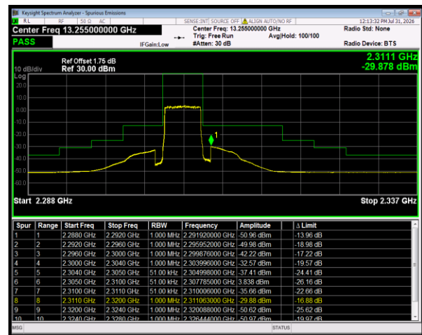
Band30 QPSK BW=5MHz LowChannel=27685 RB Size=25 Position=#0
