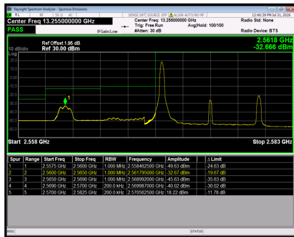
Band38 QPSK BW=10MHz LowChannel=37800 RB Size=1 Position=#0
