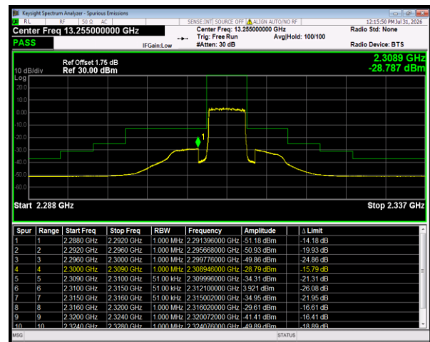
Band30 QPSK BW=5MHz HighChannel=27735 RB Size=25 Position=#0
