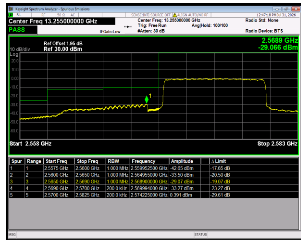
Band38 QPSK BW=10MHz LowChannel=37800 RB Size=50 Position=#0
