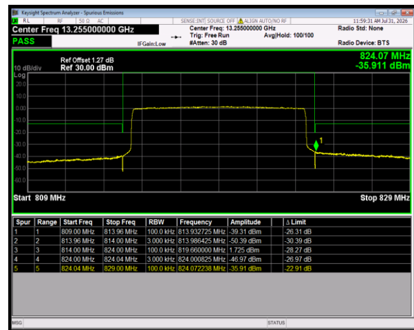
Band26(814-824) QPSK BW=10MHz HighChannel=26740 RB Size=50 Position=#0
