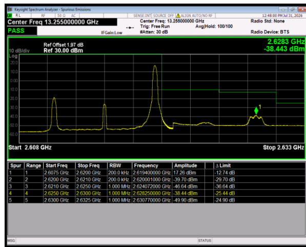
Band38 QPSK BW=10MHz HighChannel=38200 RB Size=1 Position=#Max
