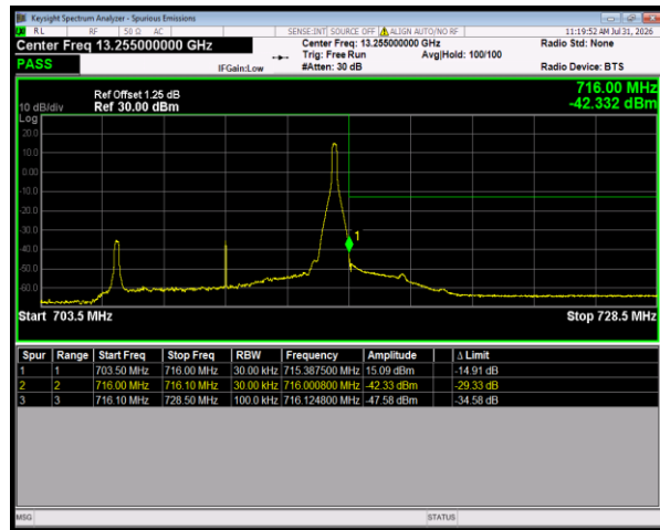
Band12 QPSK BW=10MHz HighChannel=23130 RB Size=1 Position=#Max
