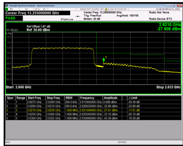
Band38 QPSK BW=10MHz HighChannel=38200 RB Size=50 Position=#0
