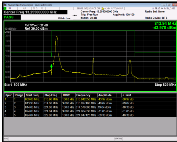
Band26(814-824) QPSK BW=10MHz LowChannel=26740 RB Size=1 Position=#0
