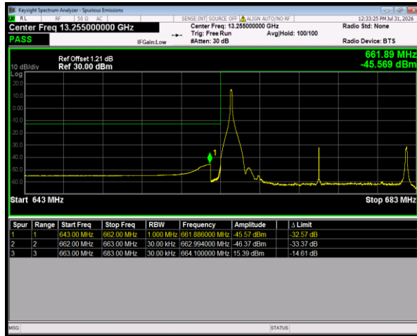
Band71 QPSK BW=20MHz LowChannel=133222 RB Size=1 Position=#0
