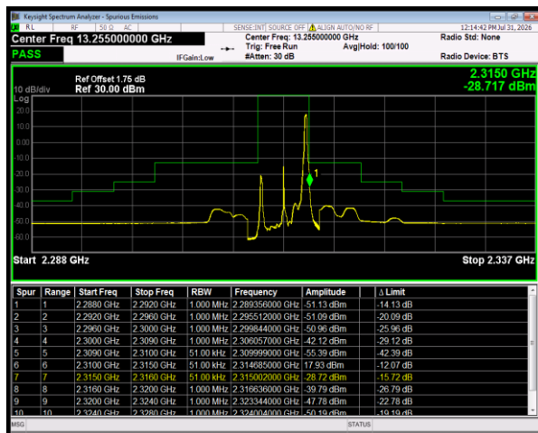
Band30 QPSK BW=5MHz HighChannel=27735 RB Size=1 Position=#Max
