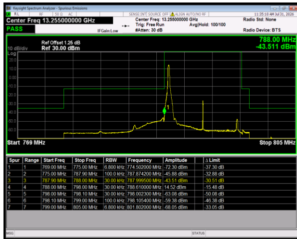
Band14 QPSK BW=10MHz LowChannel=23330 RB Size=1 Position=#0
