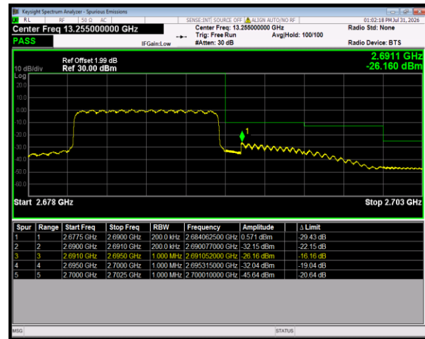
Band41 QPSK BW=10MHz HighChannel=41540 RB Size=50 Position=#0
