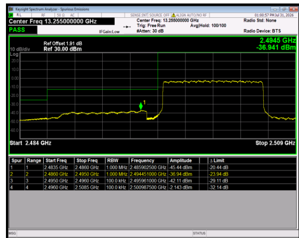
Band41 QPSK BW=10MHz LowChannel=39700 RB Size=50 Position=#0
