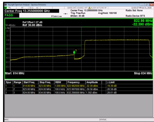
Band26(824-849) QPSK BW=10MHz LowChannel=26840 RB Size=50 Position=#0
