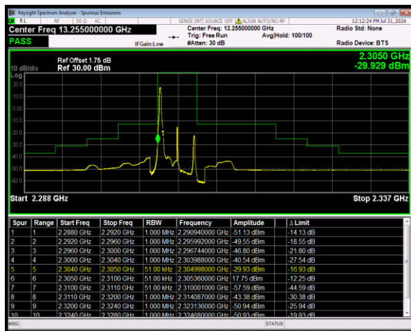
Band30 QPSK BW=5MHz LowChannel=27685 RB Size=1 Position=#0
