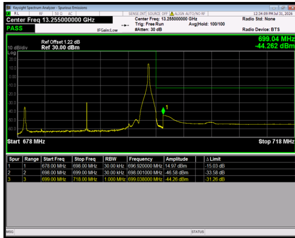
Band71 QPSK BW=20MHz HighChannel=133372 RB Size=1 Position=#Max
