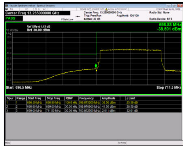
Band12 16QAM BW=10MHz LowChannel=23060 RB Size=50 Position=#0
