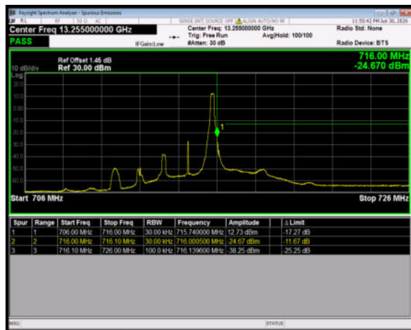
Band12 64QAM BW=3MHz HighChannel=23165 RB Size=1 Position=#Max
