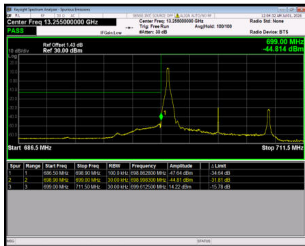
Band12 64QAM BW=10MHz LowChannel=23060 RB Size=1 Position=#0
