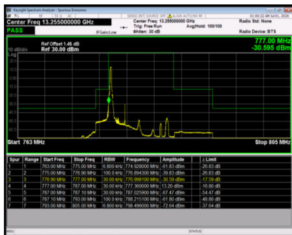
Band13 64QAM BW=5MHz LowChannel=23205 RB Size=1 Position=#0
