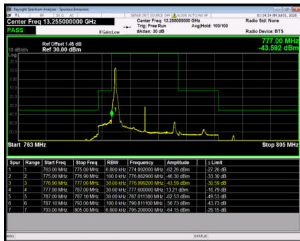
Band13 64QAM BW=10MHz LowChannel=23230 RB Size=1 Position=#0
