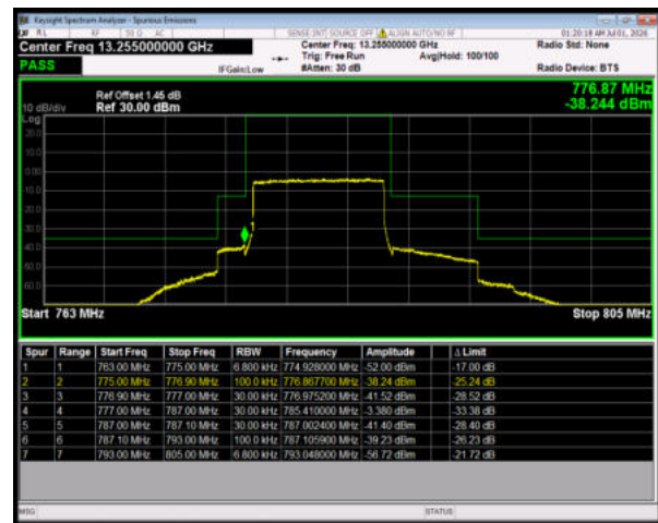
Band13 16QAM BW=10MHz HighChannel=23230 RB Size=50 Position=#0
