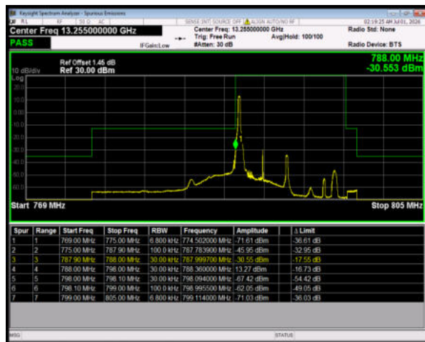
Band14 64QAM BW=5MHz LowChannel=23305 RB Size=1 Position=#0
