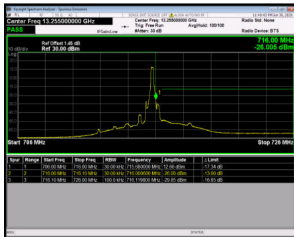
Band12 64QAM BW=1.4MHz HighChannel=23173 RB Size=1 Position=#Max
