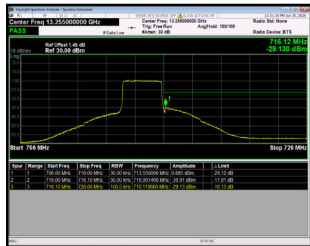
Band12 64QAM BW=3MHz HighChannel=23165 RB Size=15 Position=#0
