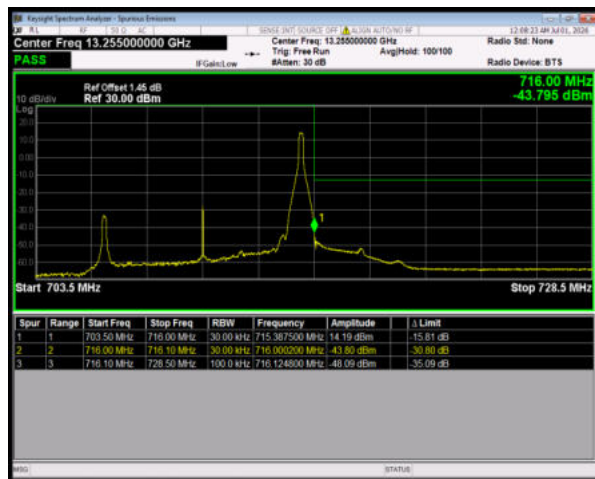
Band12 64QAM BW=10MHz HighChannel=23130 RB Size=1 Position=#Max
