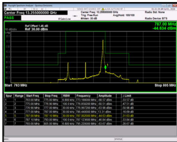
Band13 64QAM BW=10MHz HighChannel=23230 RB Size=1 Position=#Max
