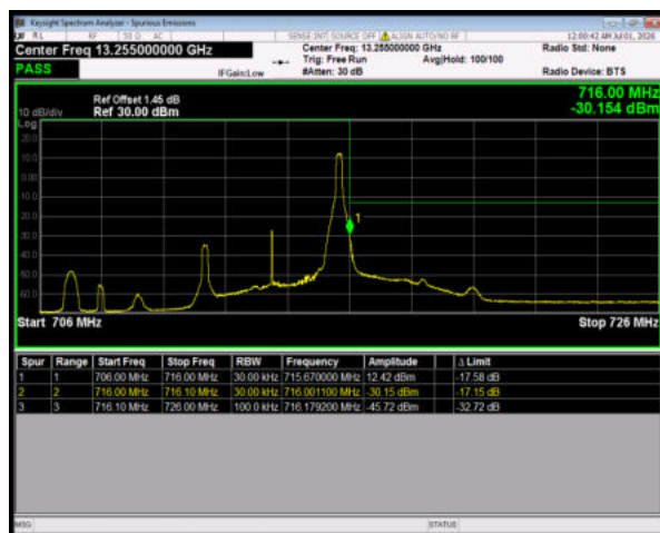
Band12 64QAM BW=5MHz HighChannel=23155 RB Size=1 Position=#Max
