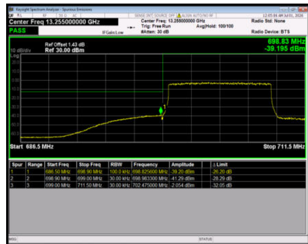
Band12 64QAM BW=10MHz LowChannel=23060 RB Size=50 Position=#0
