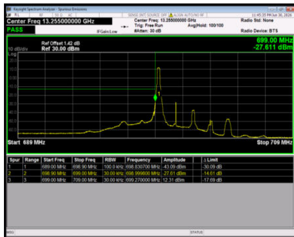
Band12 64QAM BW=3MHz LowChannel=23025 RB Size=1 Position=#0
