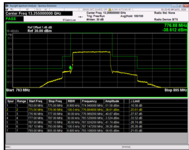
Band13 64QAM BW=10MHz HighChannel=23230 RB Size=50 Position=#0
