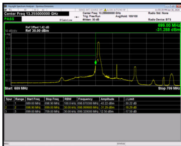
Band12 64QAM BW=5MHz LowChannel=23035 RB Size=1 Position=#0
