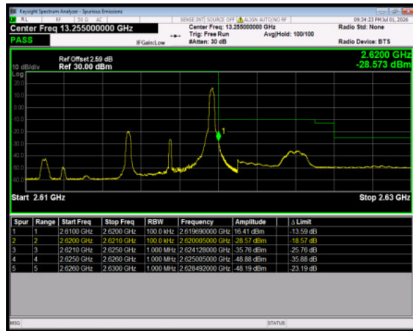
Band38 QPSK BW=5MHz HighChannel=38225 RB Size=1 Position=#Max
