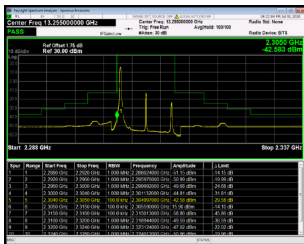
Band30 64QAM BW=10MHz LowChannel=27710 RB Size=1 Position=#0
