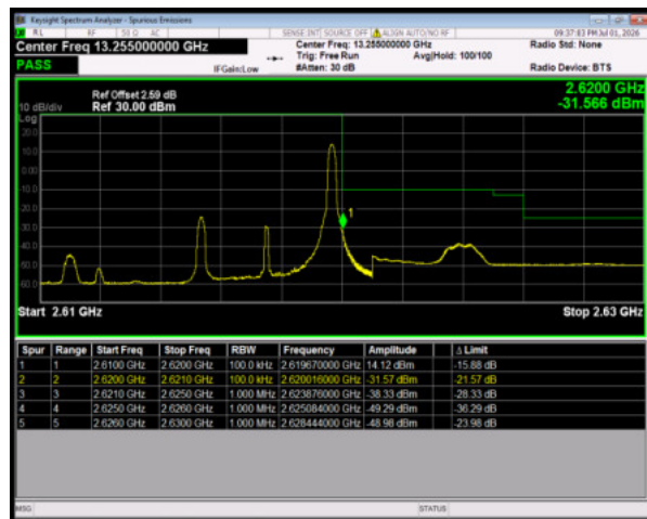
Band38 64QAM BW=5MHz HighChannel=38225 RB Size=1 Position=#Max
