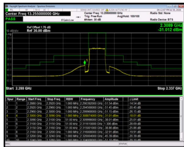
Band30 16QAM BW=5MHz HighChannel=27735 RB Size=25 Position=#0
