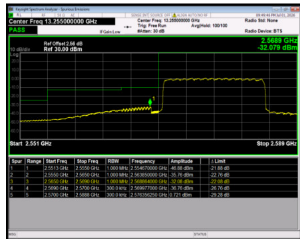
Band38 64QAM BW=15MHz LowChannel=37825 RB Size=75 Position=#0
