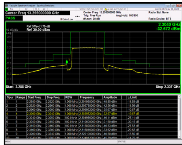
Band30 QPSK BW=10MHz HighChannel=27710 RB Size=50 Position=#0
