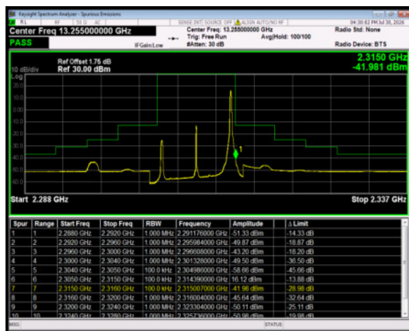
Band30 64QAM BW=10MHz HighChannel=27710 RB Size=1 Position=#Max
