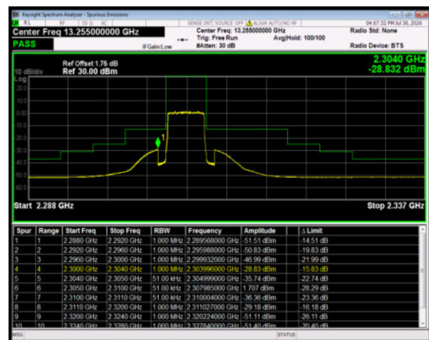
Band30 64QAM BW=5MHz LowChannel=27685 RB Size=25 Position=#0
