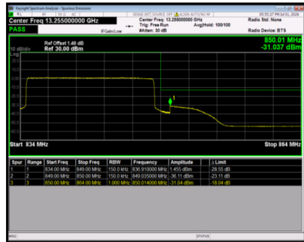
Band26(824-849) QPSK BW=15MHz HighChannel=26965 RB Size=75 Position=#0
