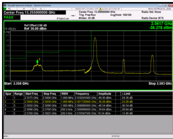
Band38 64QAM BW=10MHz LowChannel=37800 RB Size=1 Position=#0
