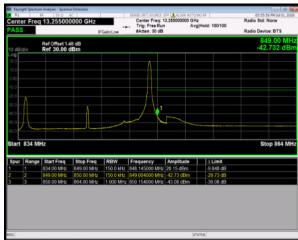
Band26(824-849) 16QAM BW=15MHz HighChannel=26965 RB Size=1 Position=#Max
