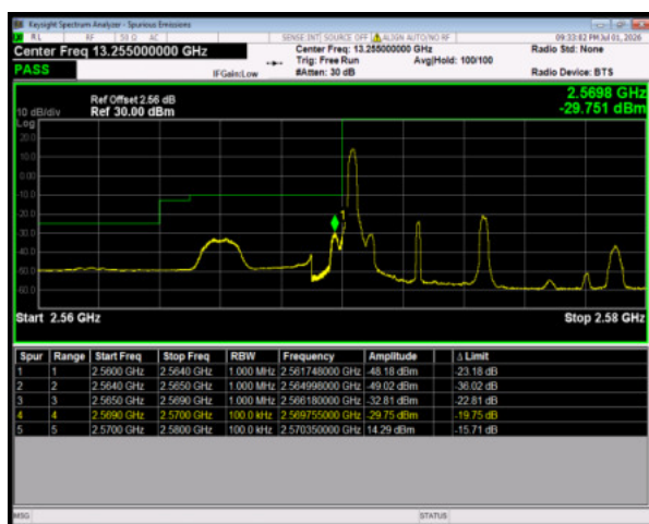
Band38 64QAM BW=5MHz LowChannel=37775 RB Size=1
