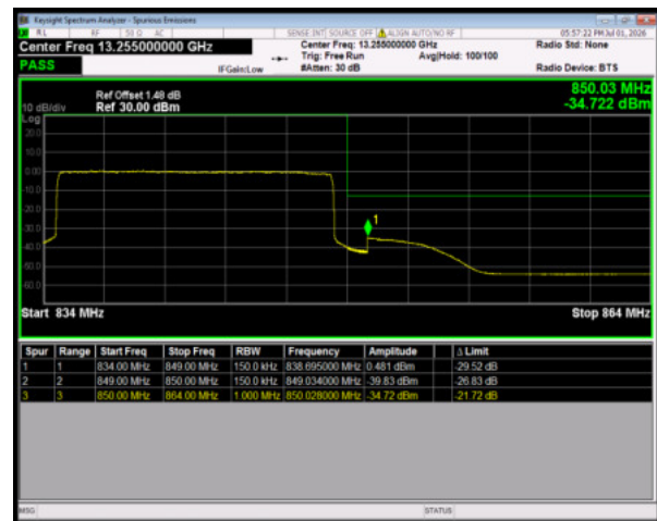
Band26(824-849) 64QAM BW=15MHz HighChannel=26965 RB Size=75 Position=#0
