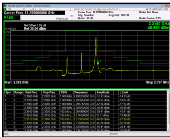
Band30 16QAM BW=10MHz HighChannel=27710 RB Size=1 Position=#Max
