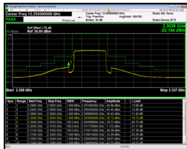
Band30 64QAM BW=10MHz LowChannel=27710 RB Size=50 Position=#0
