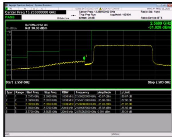
Band38 64QAM BW=10MHz LowChannel=37800 RB Size=50 Position=#0
