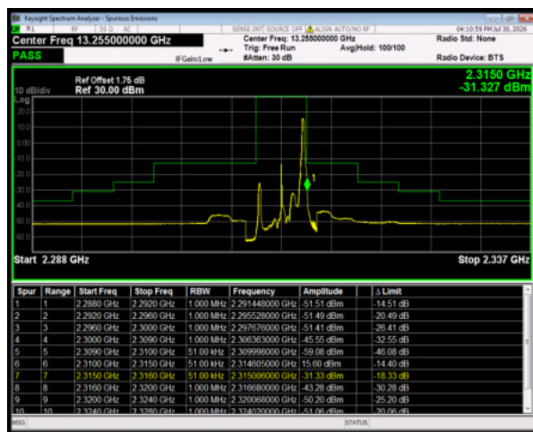
Band30 16QAM BW=5MHz HighChannel=27735 RB Size=1 Position=#Max
