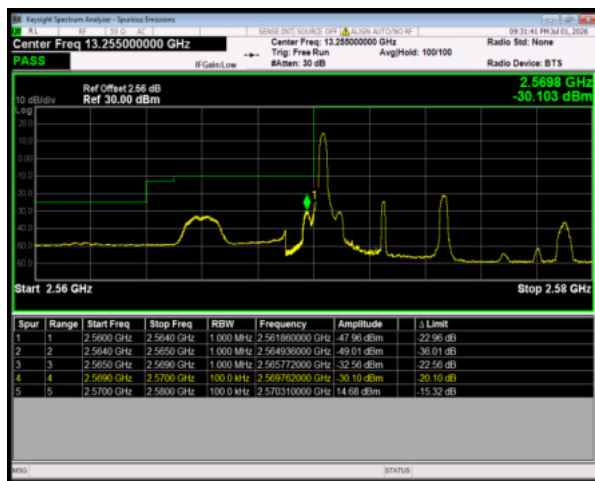
Band38 16QAM BW=5MHz LowChannel=37775 RB Size=1
