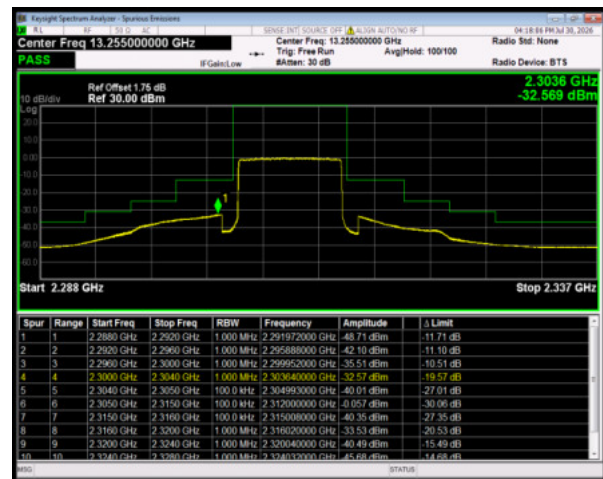
Band30 QPSK BW=10MHz LowChannel=27710 RB Size=50 Position=#0
