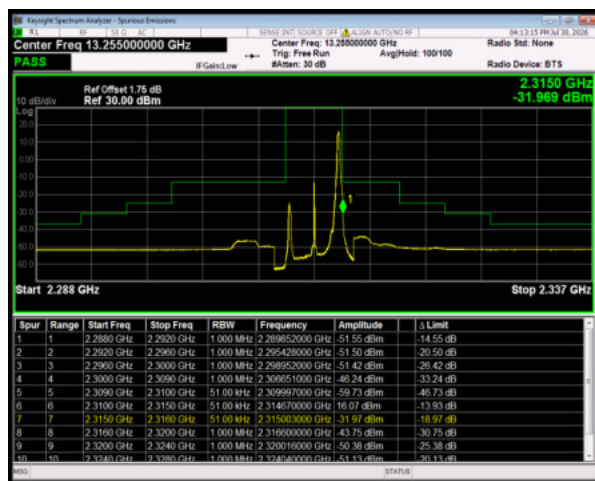
Band30 64QAM BW=5MHz HighChannel=27735 RB Size=1 Position=#Max
