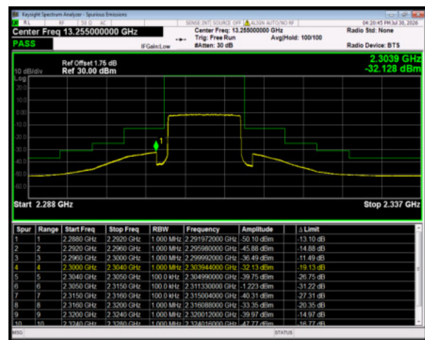
Band30 16QAM BW=10MHz LowChannel=27710 RB Size=50 Position=#0
