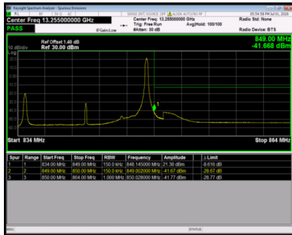
Band26(824-849) QPSK BW=15MHz HighChannel=26965 RB Size=1 Position=#Max
