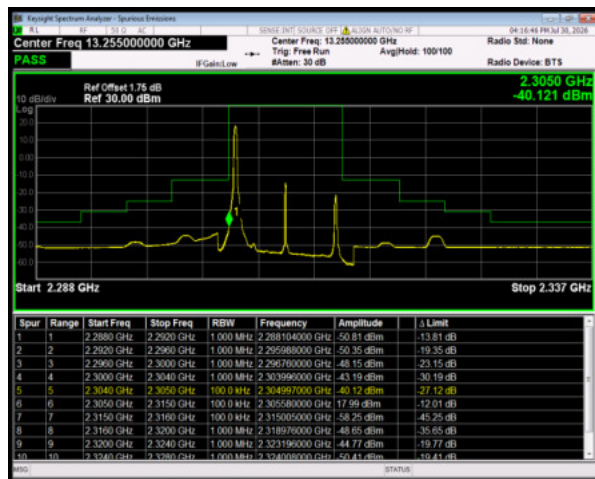
Band30 QPSK BW=10MHz LowChannel=27710 RB Size=1 Position=#0
