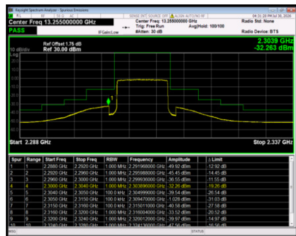
Band30 64QAM BW=10MHz HighChannel=27710 RB Size=50 Position=#0
