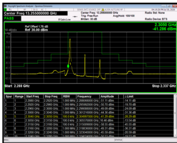
Band30 16QAM BW=10MHz LowChannel=27710 RB Size=1 Position=#0
