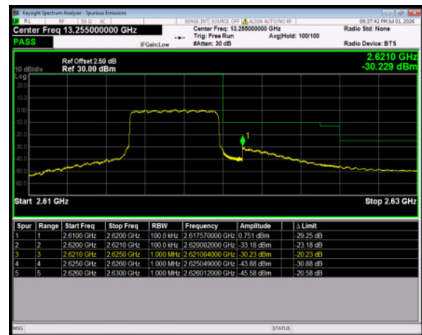
Band38 64QAM BW=5MHz HighChannel=38225 RB Size=25 Position=#0
