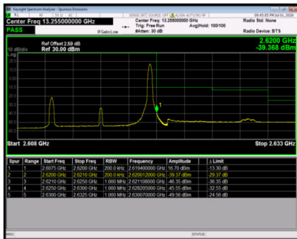
Band38 64QAM BW=10MHz HighChannel=38200 RB Size=1 Position=#Max
