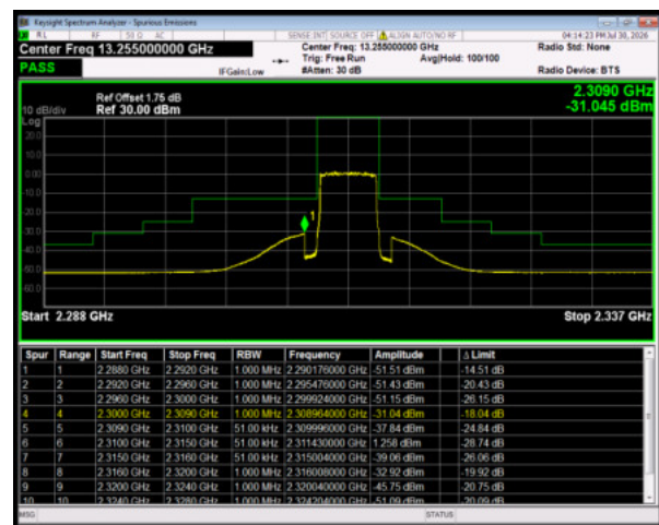
Band30 64QAM BW=5MHz HighChannel=27735 RB Size=25 Position=#0
