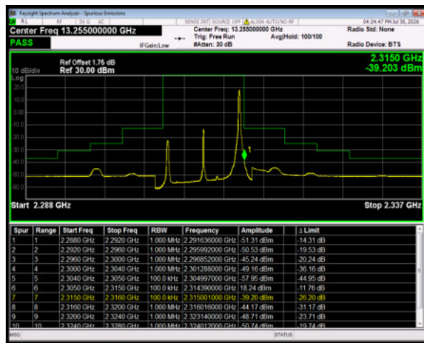
Band30 QPSK BW=10MHz HighChannel=27710 RB Size=1 Position=#Max
