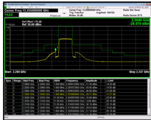
Band30 16QAM BW=5MHz LowChannel=27685 RB Size=25 Position=#0
