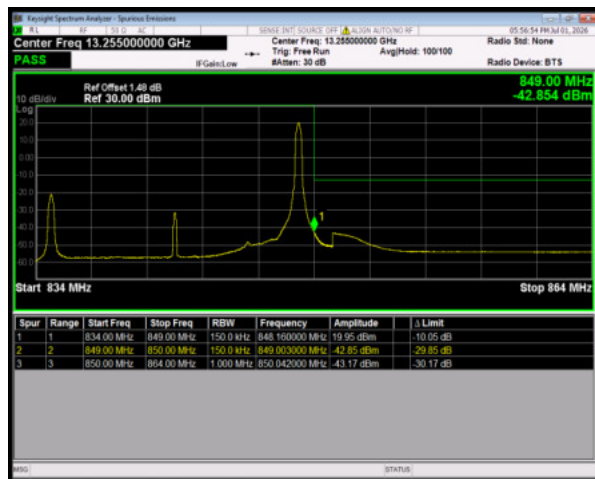
Band26(824-849) 64QAM BW=15MHz HighChannel=26965 RB Size=1 Position=#Max
