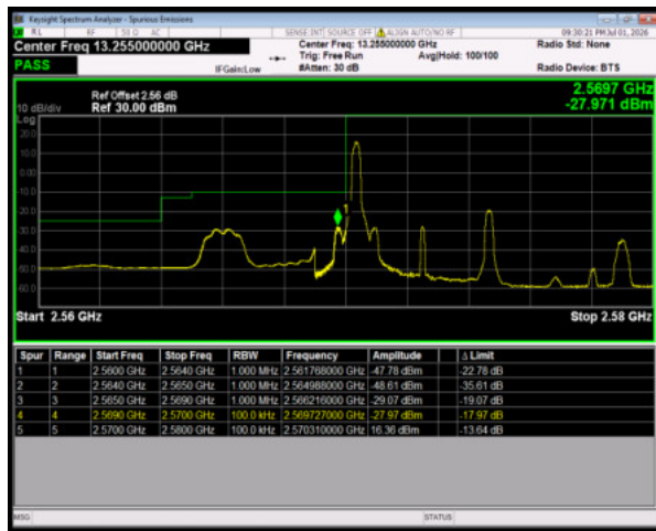
Band38 QPSK BW=5MHz LowChannel=37775 RB Size=1
