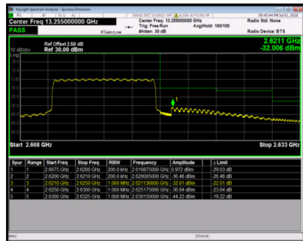
Band38 64QAM BW=10MHz HighChannel=38200 RB Size=50 Position=#0
