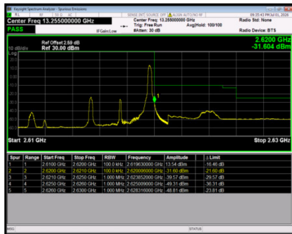
Band38 16QAM BW=5MHz HighChannel=38225 RB Size=1 Position=#Max
