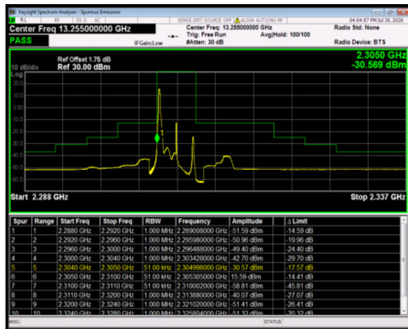
Band30 16QAM BW=5MHz LowChannel=27685 RB Size=1 Position=#0
