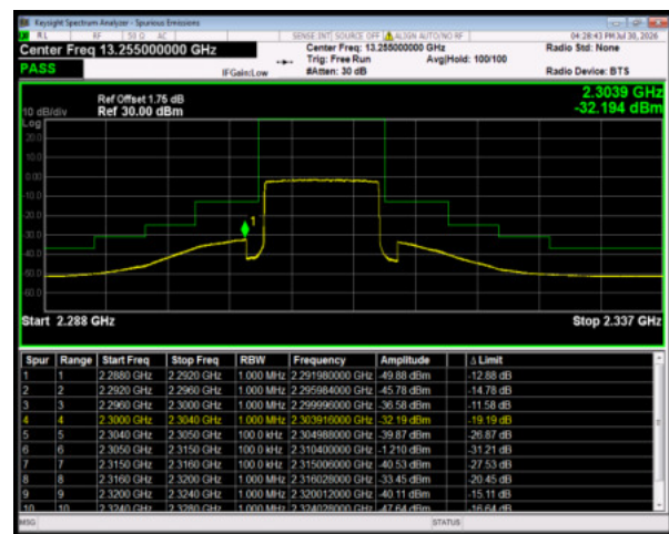
Band30 16QAM BW=10MHz HighChannel=27710 RB Size=50 Position=#0
