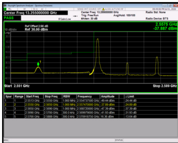
Band38 64QAM BW=15MHz LowChannel=37825 RB Size=1 Position=#0
