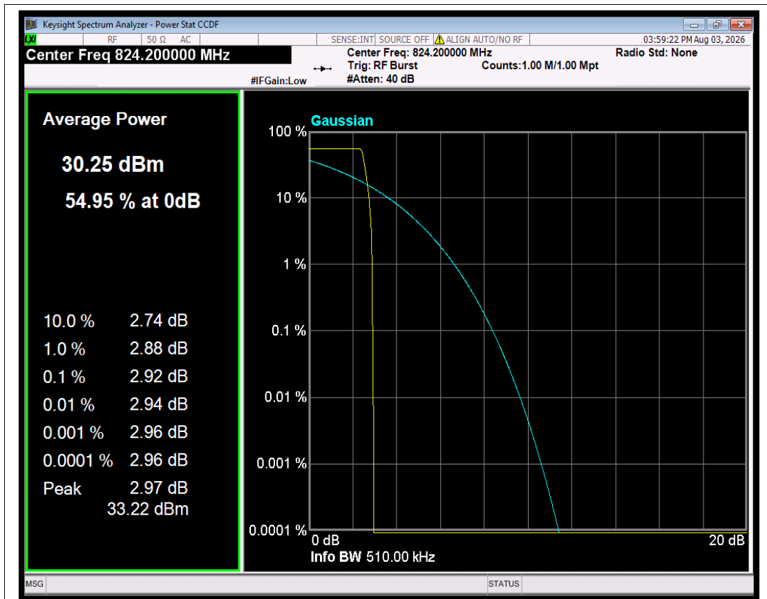
GPRS850 Channel=128
