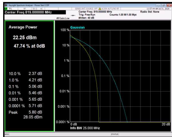
Band26(814-824) QPSK BW=10MHz Channel=26740 RB Size=50 Position=#0
