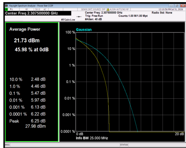
Band30 QPSK BW=5MHz Channel=27685 RB Size=25 Position=#0
