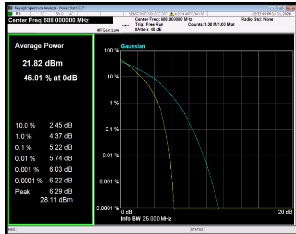
Band71 QPSK BW=20MHz Channel=133372 RB Size=100 Position=#0
