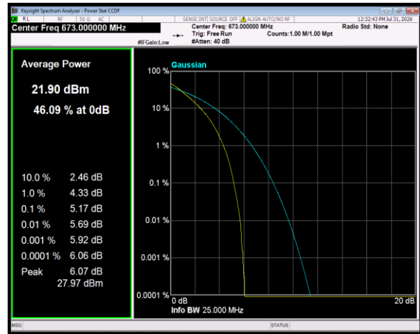
Band71 QPSK BW=20MHz Channel=133222 RB Size=100 Position=#0
