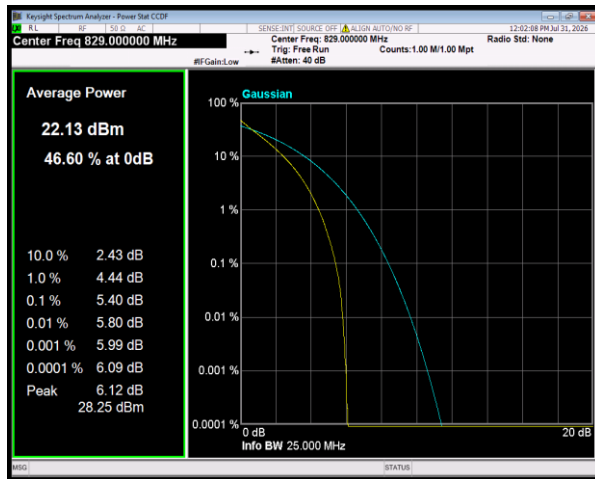
Band26(824-849) QPSK BW=10MHz Channel=26840 RB Size=50 Position=#0
