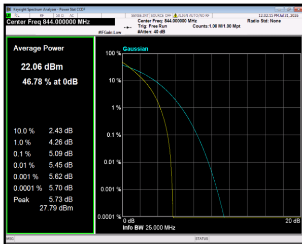
Band26(824-849) QPSK BW=10MHz Channel=26990 RB Size=50 Position=#0
