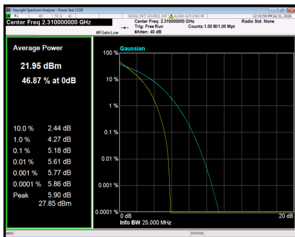
Band30 QPSK BW=5MHz Channel=27710 RB Size=25 Position=#0
