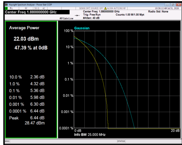
Band2 QPSK BW=20MHz Channel=18900 RB Size=100 Position=#0
