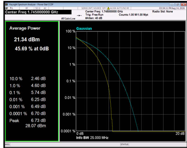
Band66 QPSK BW=10MHz Channel=132322 RB Size=50 Position=#0
