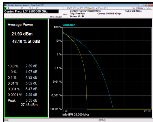
Band30 QPSK BW=5MHz Channel=27735 RB Size=25 Position=#0
