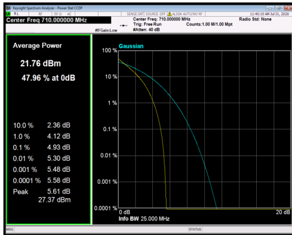
Band17 QPSK BW=10MHz Channel=23790 RB Size=50 Position=#0
