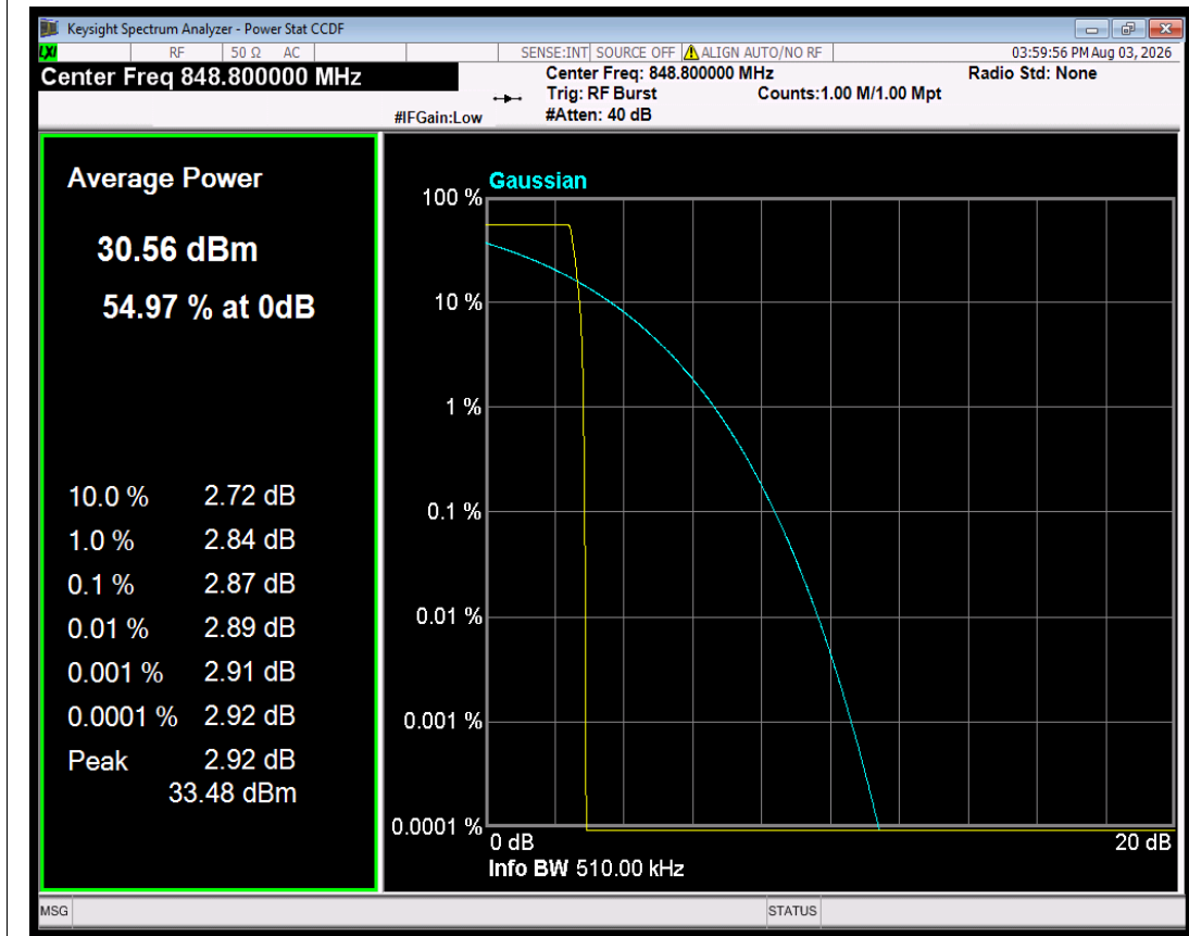
GPRS850 Channel=251
