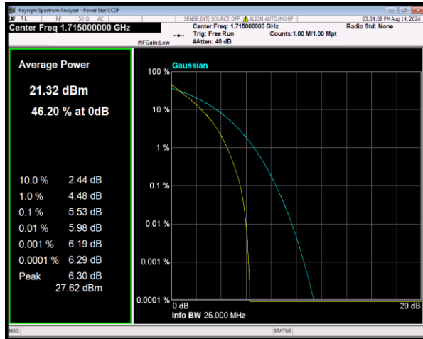
Band66 QPSK BW=10MHz Channel=132022 RB Size=50 Position=#0
