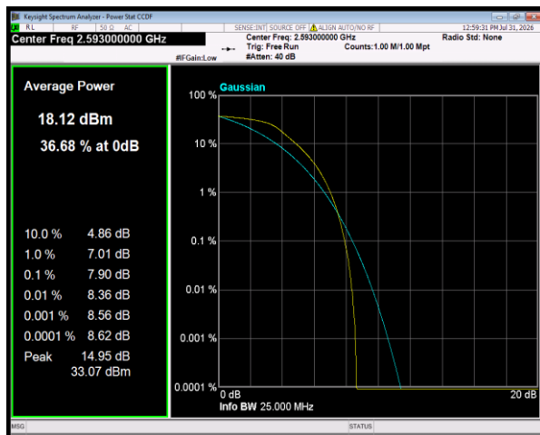
Band41 QPSK BW=10MHz Channel=40620 RB Size=50 Position=#0
