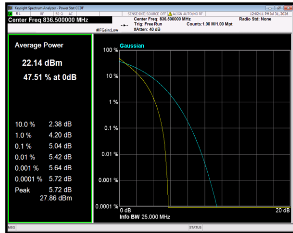
Band26(824-849) QPSK BW=10MHz Channel=26915 RB Size=50 Position=#0
