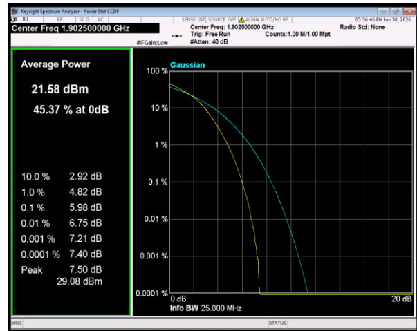
Band2 16QAM BW=15MHz Channel=19125 RB Size=75 Position=#0
