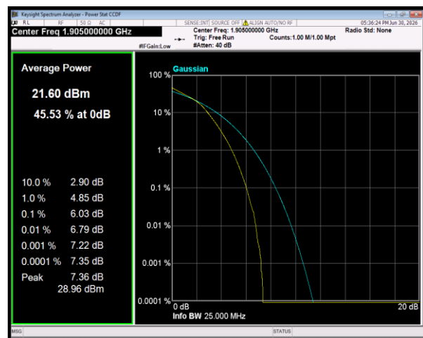
Band2 64QAM BW=10MHz Channel=19150 RB Size=50 Position=#0
