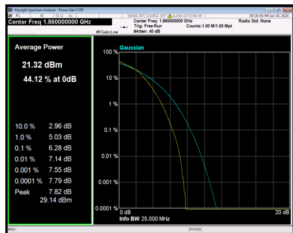
Band2 64QAM BW=20MHz Channel=18700 RB Size=100 Position=#0
