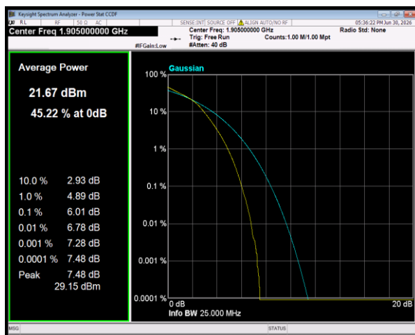
Band2 16QAM BW=10MHz Channel=19150 RB Size=50 Position=#0
