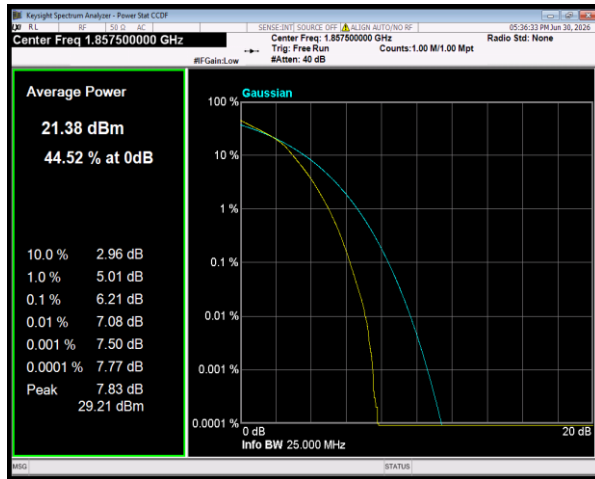
Band2 64QAM BW=15MHz Channel=18675 RB Size=75 Position=#0
