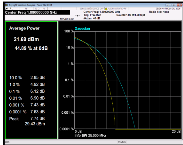
Band2 64QAM BW=15MHz Channel=18900 RB Size=75 Position=#0
