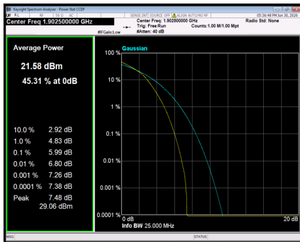
Band2 64QAM BW=15MHz Channel=19125 RB Size=75 Position=#0
