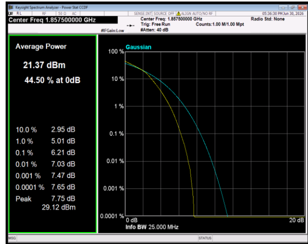
Band2 16QAM BW=15MHz Channel=18675 RB Size=75 Position=#0
