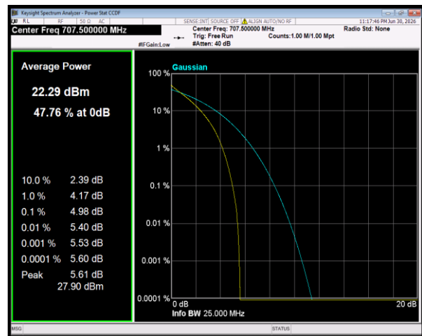
Band12 QPSK BW=5MHz Channel=23095 RB Size=25 Position=#0
