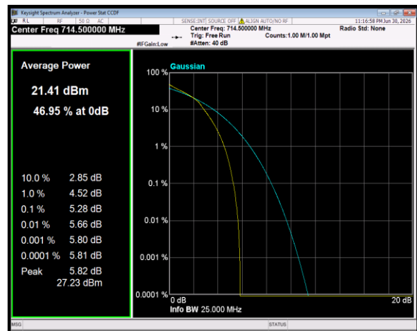
Band12 64QAM BW=3MHz Channel=23165 RB Size=15 Position=#0
