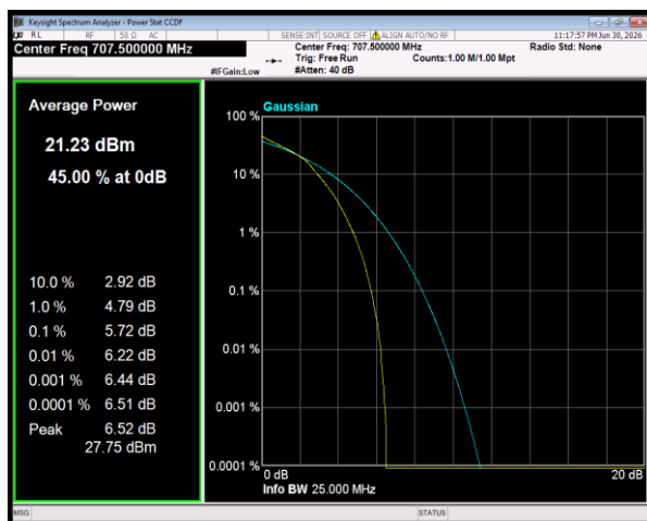
Band12 16QAM BW=5MHz Channel=23095 RB Size=25 Position=#0
