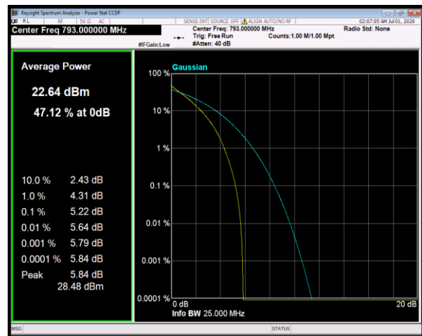
Band14 QPSK BW=5MHz Channel=23330 RB Size=25 Position=#0
