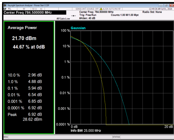
Band13 64QAM BW=5MHz Channel=23255 RB Size=25 Position=#0
