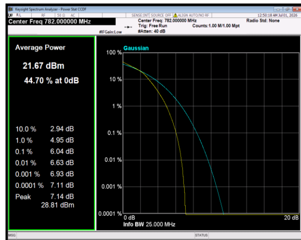
Band13 64QAM BW=10MHz Channel=23230 RB Size=50 Position=#0
