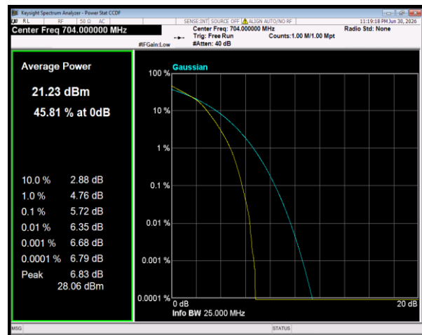
Band12 64QAM BW=10MHz Channel=23060 RB Size=50 Position=#0
