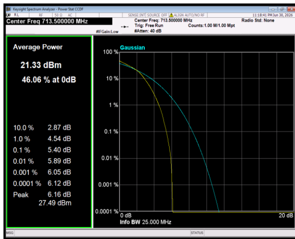
Band12 64QAM BW=5MHz Channel=23155 RB Size=25 Position=#0
