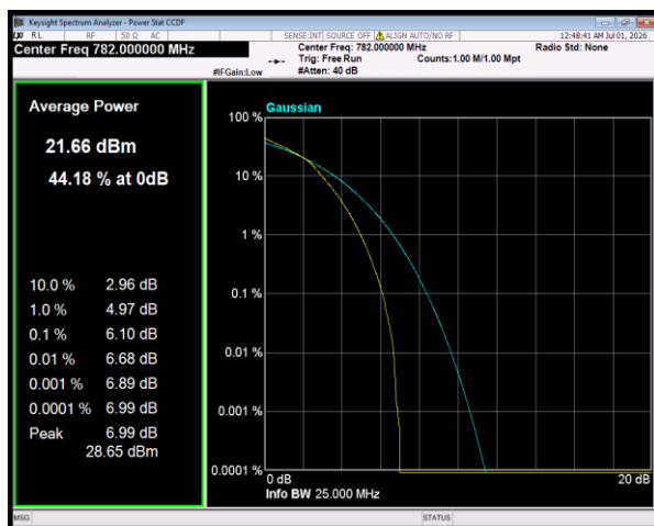
Band13 16QAM BW=5MHz Channel=23230 RB Size=25 Position=#0
