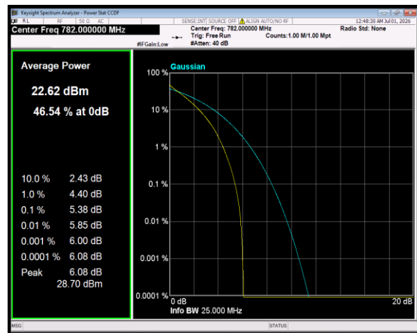
Band13 QPSK BW=5MHz Channel=23230 RB Size=25 Position=#0
