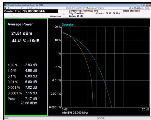
Band13 64QAM BW=5MHz Channel=23230 RB Size=25 Position=#0
