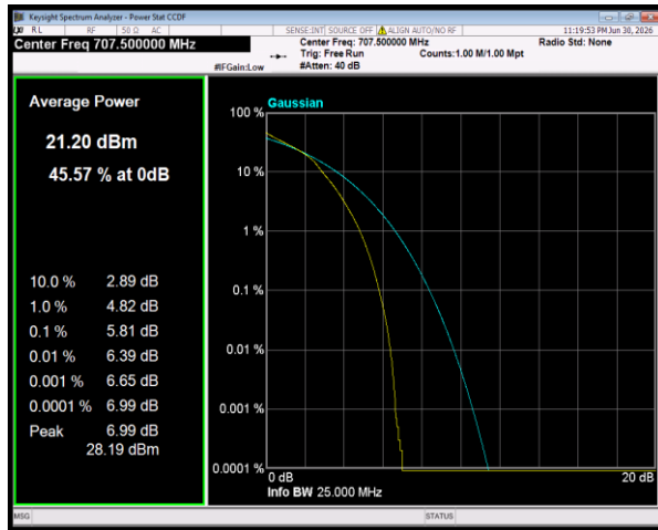
Band12 64QAM BW=10MHz Channel=23095 RB Size=50 Position=#0
