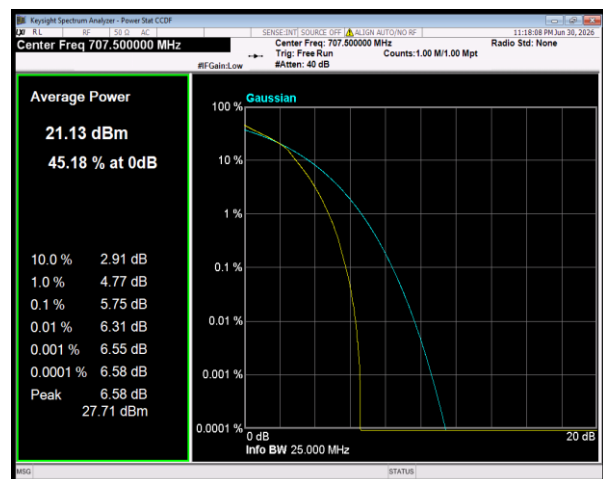
Band12 64QAM BW=5MHz Channel=23095 RB Size=25 Position=#0
