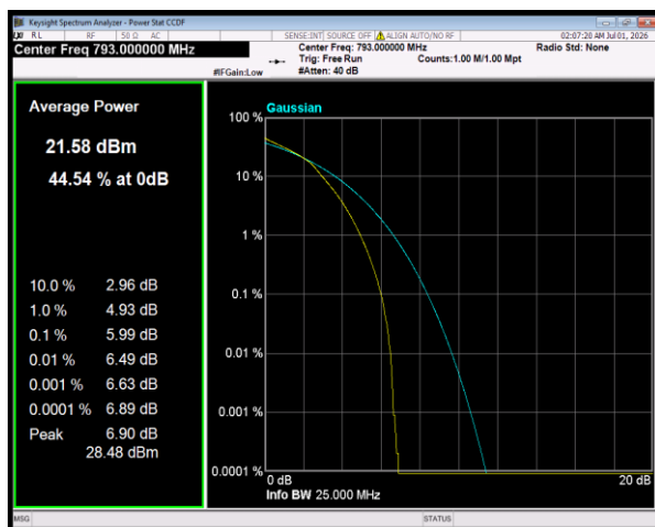
Band14 16QAM BW=5MHz Channel=23330 RB Size=25 Position=#0
