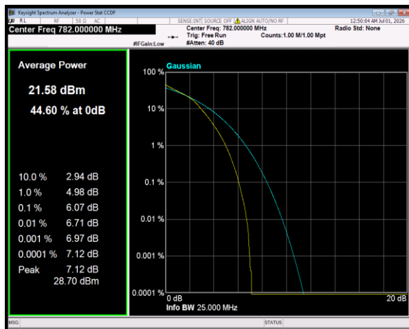
Band13 16QAM BW=10MHz Channel=23230 RB Size=50 Position=#0
