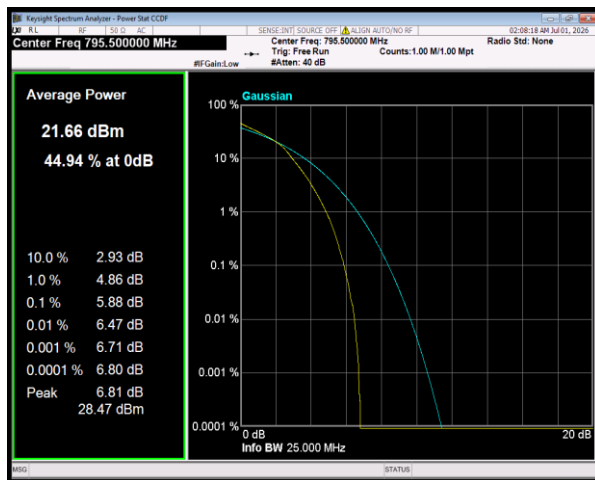
Band14 64QAM BW=5MHz Channel=23355 RB Size=25 Position=#0
