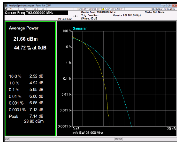
Band14 64QAM BW=10MHz Channel=23330 RB Size=50 Position=#0
