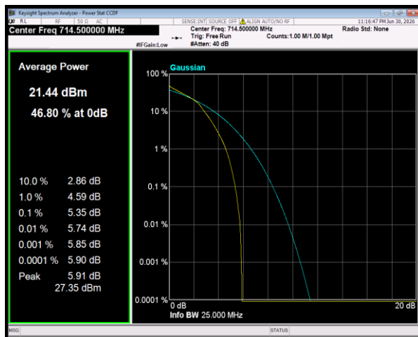
Band12 16QAM BW=3MHz Channel=23165 RB Size=15 Position=#0
