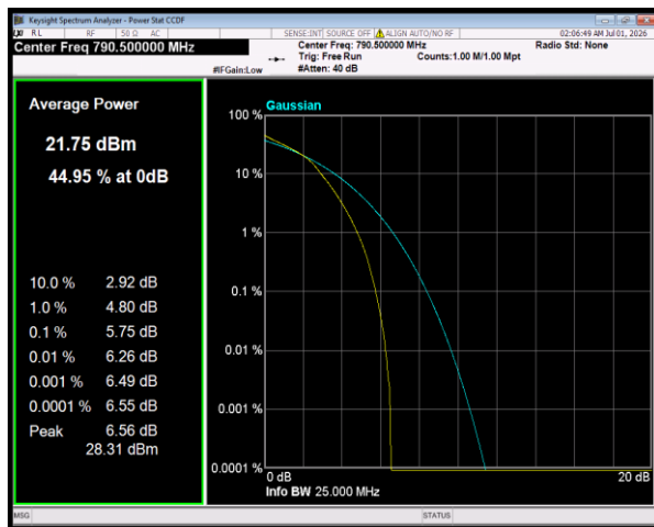
Band14 64QAM BW=5MHz Channel=23305 RB Size=25 Position=#0
