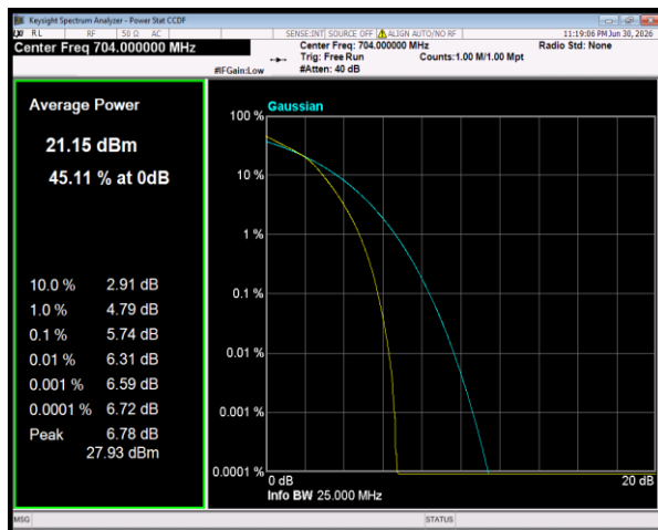
Band12 16QAM BW=10MHz Channel=23060 RB Size=50 Position=#0
