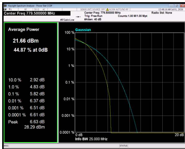
Band13 64QAM BW=5MHz Channel=23205 RB Size=25 Position=#0
