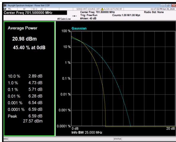
Band12 64QAM BW=5MHz Channel=23035 RB Size=25 Position=#0
