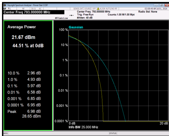
Band14 16QAM BW=10MHz Channel=23330 RB Size=50 Position=#0
