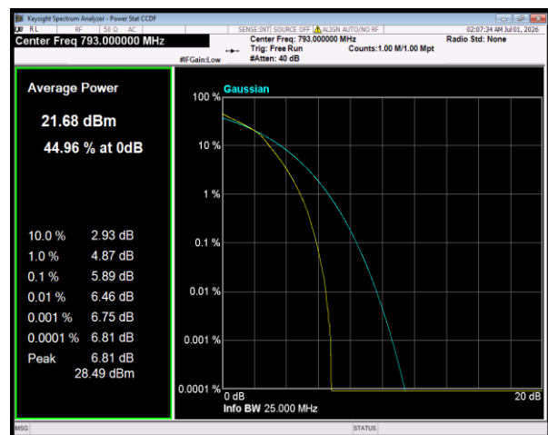
Band14 64QAM BW=5MHz Channel=23330 RB Size=25 Position=#0
