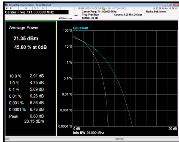
Band12 64QAM BW=10MHz Channel=23130 RB Size=50 Position=#0
