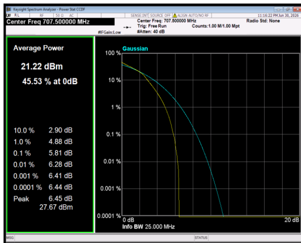
Band12 64QAM BW=3MHz Channel=23095 RB Size=15 Position=#0
