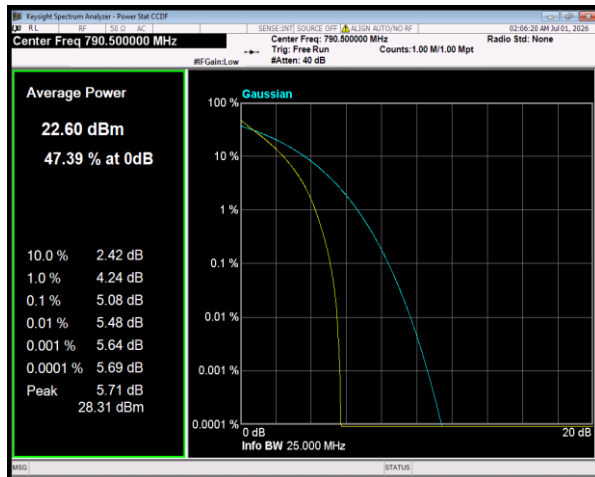
Band14 QPSK BW=5MHz Channel=23305 RB Size=25 Position=#0
