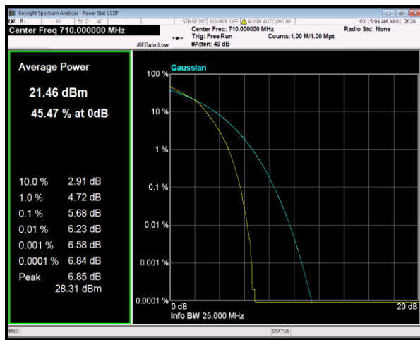
Band17 64QAM BW=10MHz Channel=23790 RB Size=50 Position=#0
