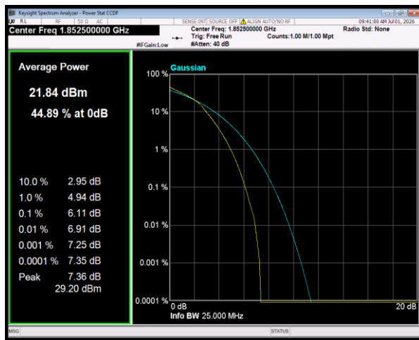
Band25 64QAM BW=5MHz Channel=26065 RB Size=25 Position=#0
