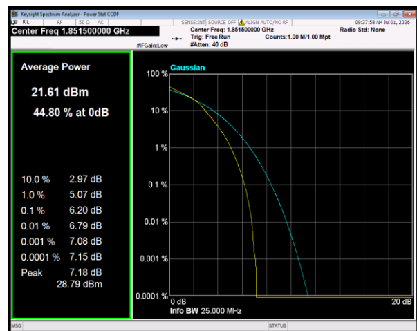
Band25 64QAM BW=3MHz Channel=26055 RB Size=15 Position=#0
