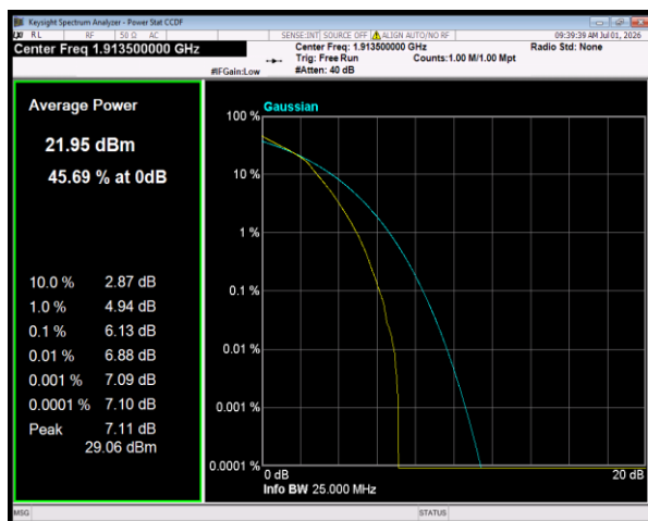
Band25 16QAM BW=3MHz Channel=26675 RB Size=15 Position=#0
