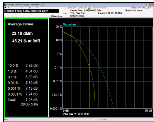
Band25 64QAM BW=5MHz Channel=26365 RB Size=25 Position=#0
