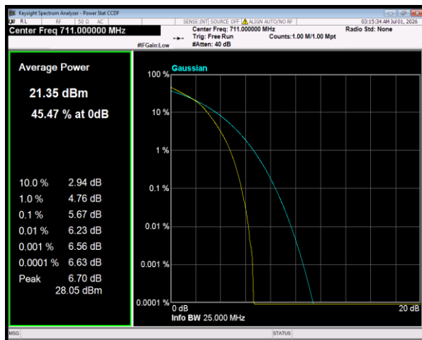
Band17 16QAM BW=10MHz Channel=23800 RB Size=50 Position=#0
