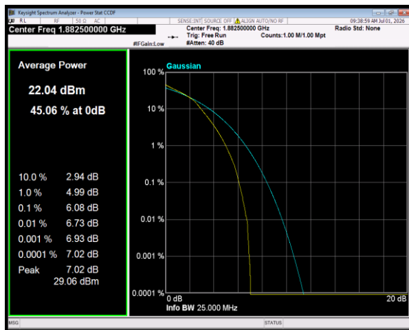
Band25 64QAM BW=3MHz Channel=26365 RB Size=15 Position=#0
