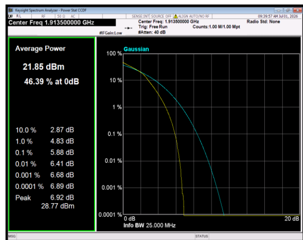
Band25 64QAM BW=3MHz Channel=26675 RB Size=15 Position=#0
