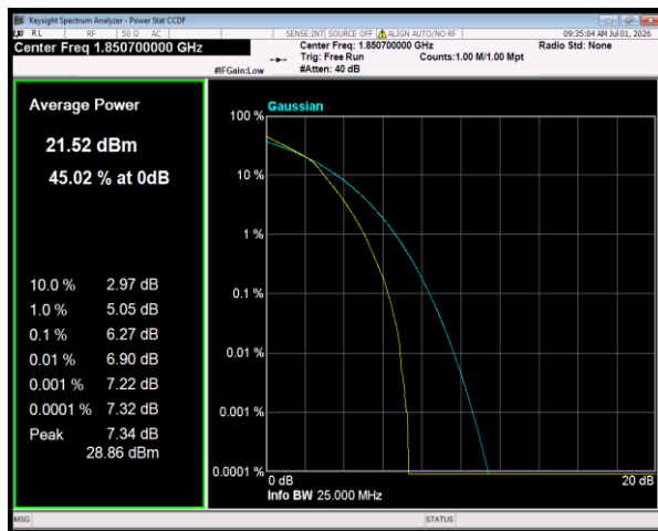
Band25 64QAM BW=1.4MHz Channel=26047 RB Size=6 Position=#0
