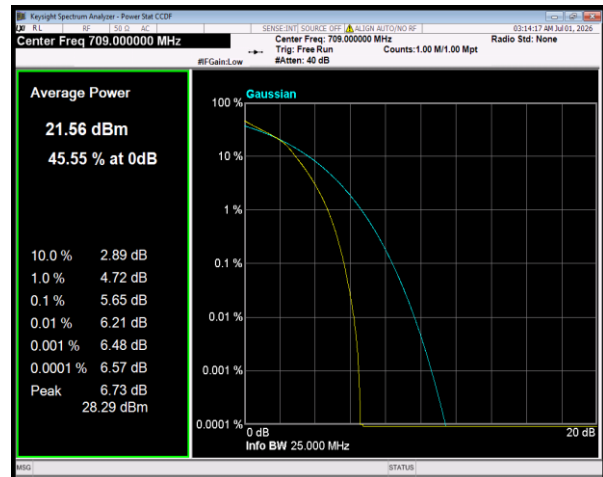
Band17 64QAM BW=10MHz Channel=23780 RB Size=50 Position=#0
