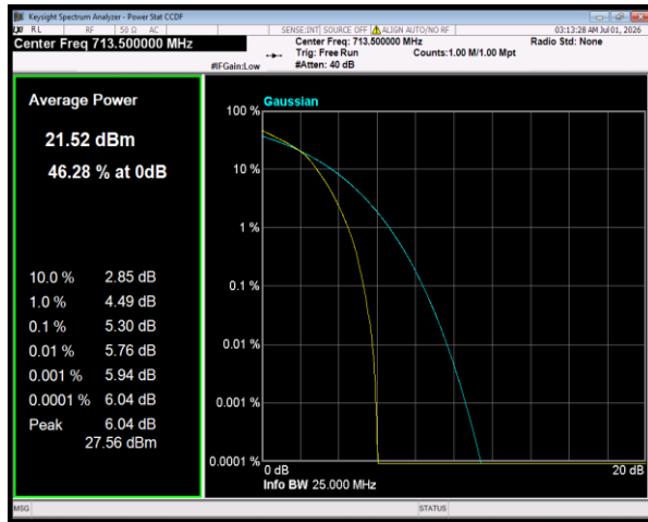
Band17 64QAM BW=5MHz Channel=23825 RB Size=25 Position=#0
