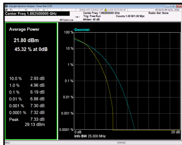
Band25 64QAM BW=1.4MHz Channel=26365 RB Size=6 Position=#0
