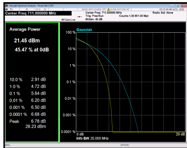
Band17 64QAM BW=10MHz Channel=23800 RB Size=50 Position=#0
