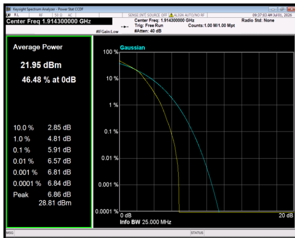
Band25 64QAM BW=1.4MHz Channel=26683 RB Size=6 Position=#0
