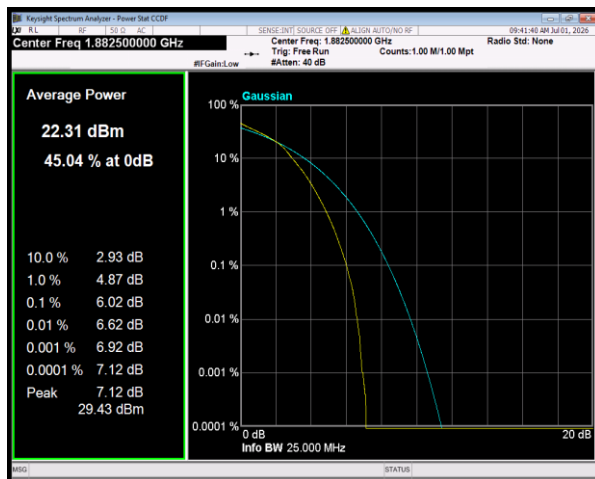
Band25 16QAM BW=5MHz Channel=26365 RB Size=25 Position=#0
