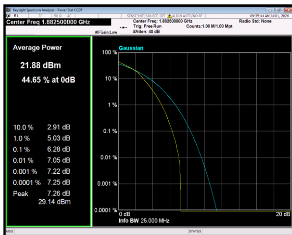
Band25 16QAM BW=1.4MHz Channel=26365 RB Size=6 Position=#0
