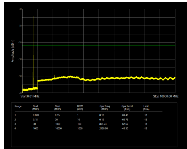
Band17 QPSK BW=10MHz Channel=23800 RB Size=1 Position=#0
