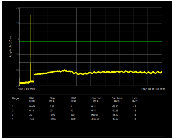
Band14 QPSK BW=5MHz Channel=23355 RB Size=1 Position=#0
