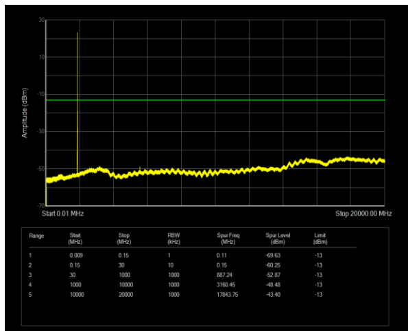
Band25 QPSK BW=5MHz Channel=26065 RB Size=1 Position=#0
