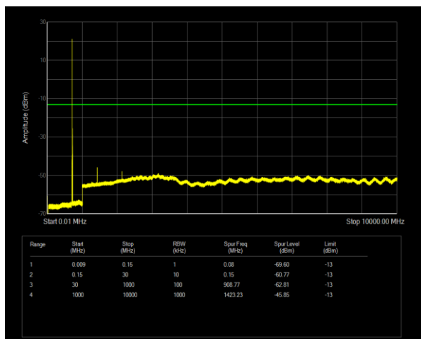
Band17 QPSK BW=5MHz Channel=23825 RB Size=1 Position=#0
