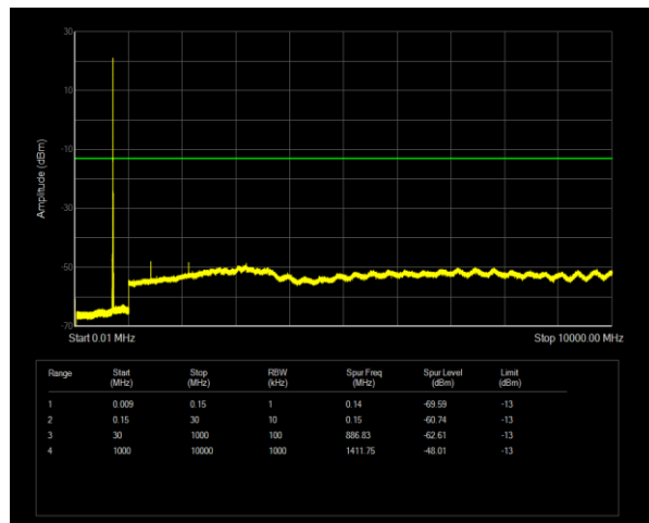
Band17 QPSK BW=10MHz Channel=23790 RB Size=1 Position=#0
