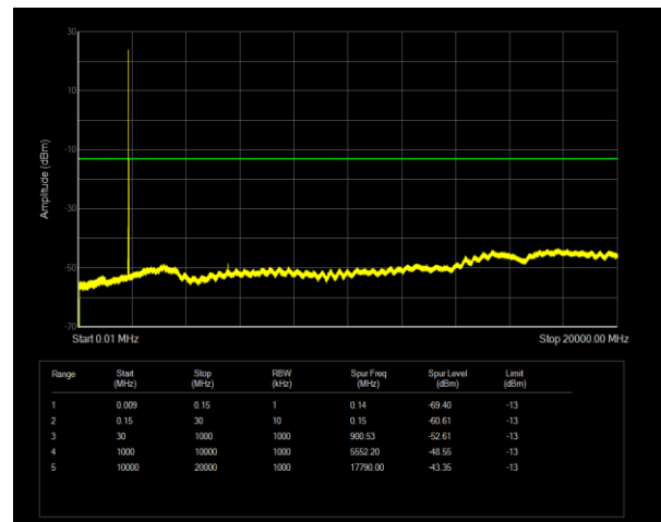
Band25 QPSK BW=10MHz Channel=26090 RB Size=1 Position=#0
