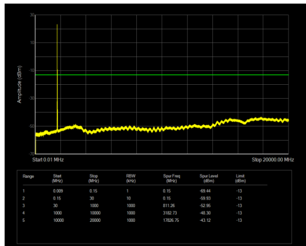
Band4 QPSK BW=20MHz Channel=20175 RB Size=1 Position=#0
