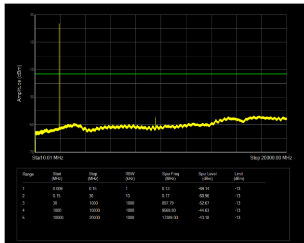
Band25 QPSK BW=1.4MHz Channel=26683 RB Size=1 Position=#0
