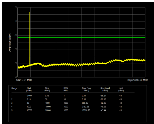
Band25 QPSK BW=1.4MHz Channel=26047 RB Size=1 Position=#0
