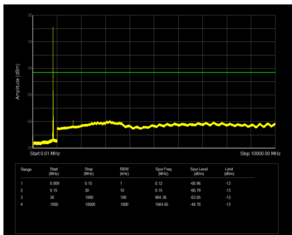
Band5 QPSK BW=10MHz Channel=20525 RB Size=1 Position=#0
