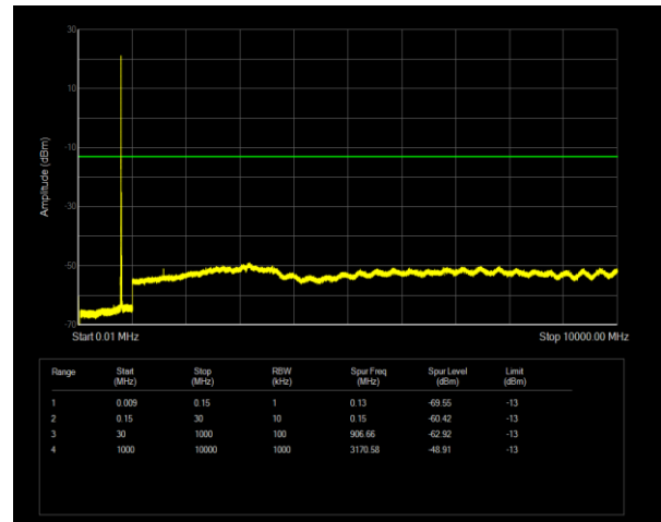
Band14 QPSK BW=10MHz Channel=23330 RB Size=1 Position=#0
