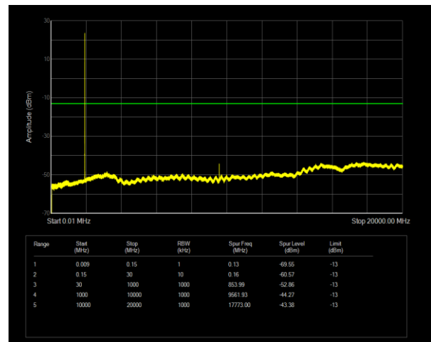
Band25 QPSK BW=3MHz Channel=26675 RB Size=1 Position=#0
