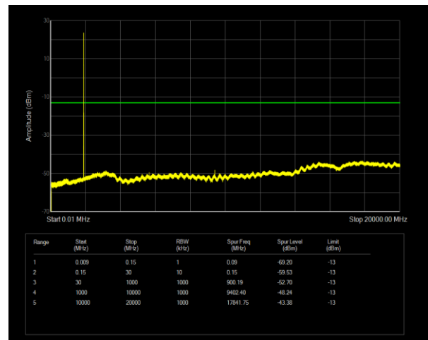
Band25 QPSK BW=5MHz Channel=26365 RB Size=1 Position=#0
