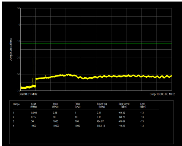
Band5 QPSK BW=5MHz Channel=20425 RB Size=1 Position=#0
