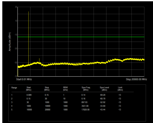
Band4 QPSK BW=1.4MHz Channel=19957 RB Size=1 Position=#0
