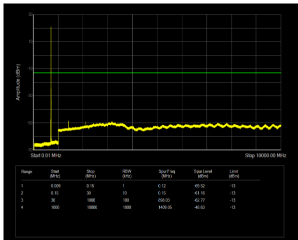
Band17 QPSK BW=5MHz Channel=23755 RB Size=1 Position=#0
