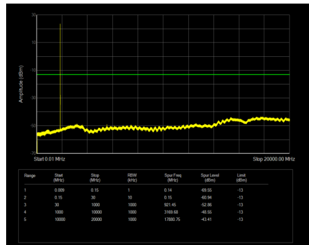
Band25 QPSK BW=3MHz Channel=26055 RB Size=1 Position=#0
