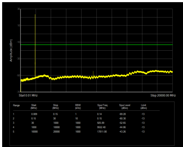
Band25 QPSK BW=5MHz Channel=26665 RB Size=1 Position=#0
