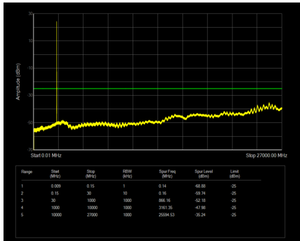
Band7 QPSK BW=5MHz Channel=20775 RB Size=1 Position=#0
