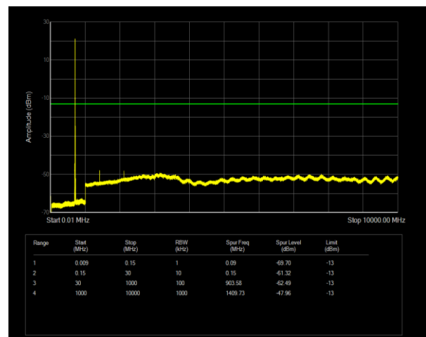
Band17 QPSK BW=10MHz Channel=23780 RB Size=1 Position=#0
