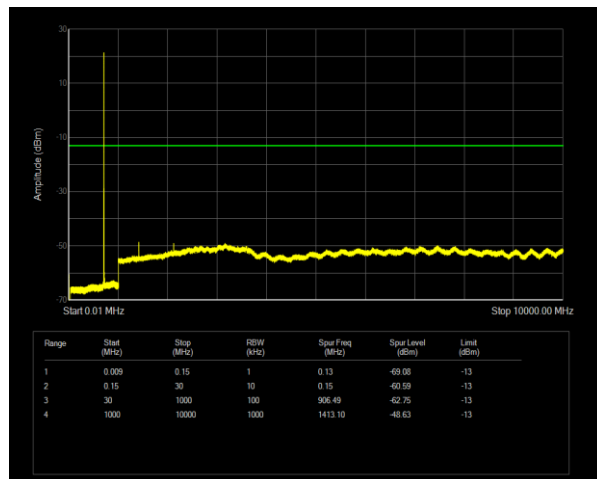
Band12 QPSK BW=3MHz Channel=23095 RB Size=1 Position=#0
