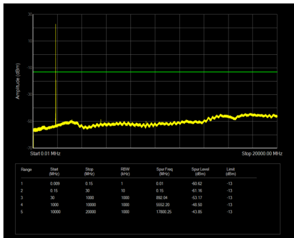
Band25 QPSK BW=10MHz Channel=26090 RB Size=1 Position=#0
