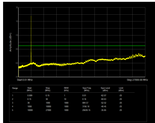
Band41 QPSK BW=10MHz Channel=41540 RB Size=1 Position=#0
