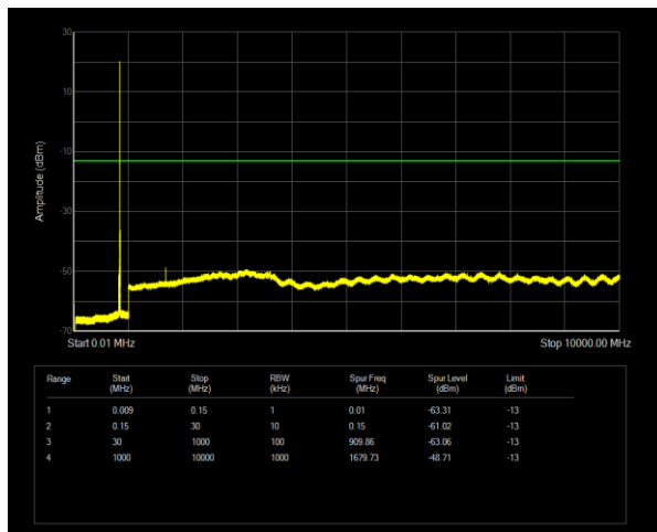
Band5 QPSK BW=10MHz Channel=20600 RB Size=1 Position=#0
