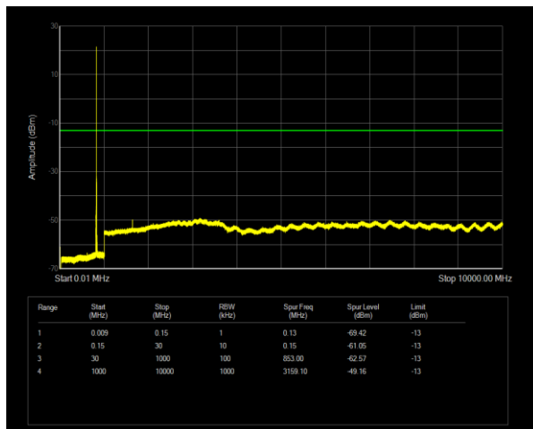
Band26(814-824) QPSK BW=5MHz Channel=26765 RB Size=1 Position=#0
