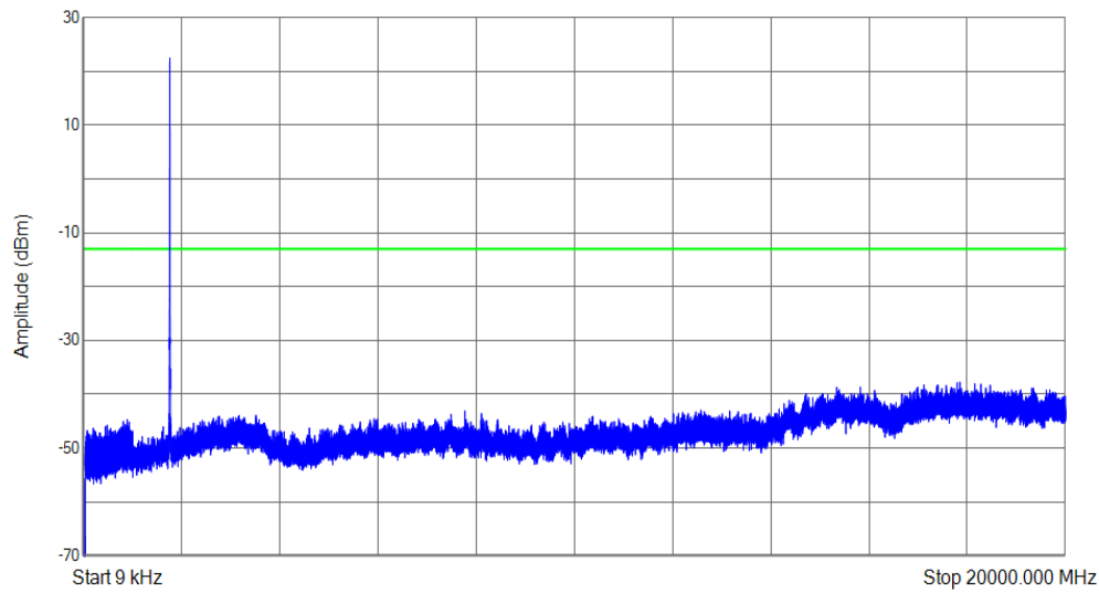
WCDMA Band4 Channel=1450
