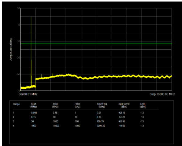
Band12 QPSK BW=10MHz Channel=23060 RB Size=1 Position=#0
