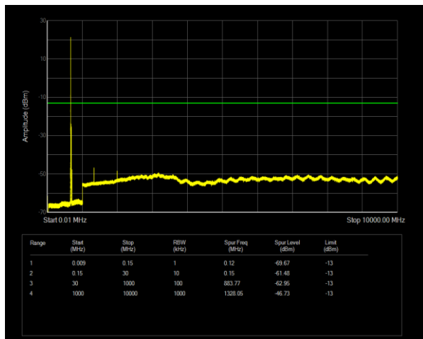
Band71 QPSK BW=20MHz Channel=133222 RB Size=1 Position=#0
