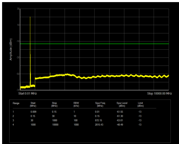
Band71 QPSK BW=20MHz Channel=133297 RB Size=1 Position=#0
