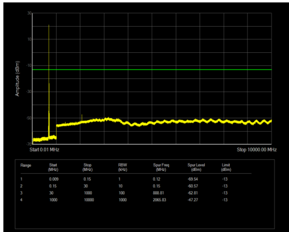
Band71 QPSK BW=10MHz Channel=133422 RB Size=1 Position=#0
