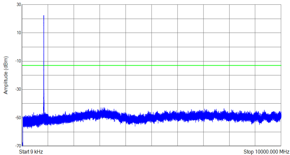
WCDMA Band5 Channel=4132
