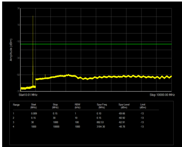
Band26(814-824) QPSK BW=3MHz Channel=26740 RB Size=1 Position=#0
