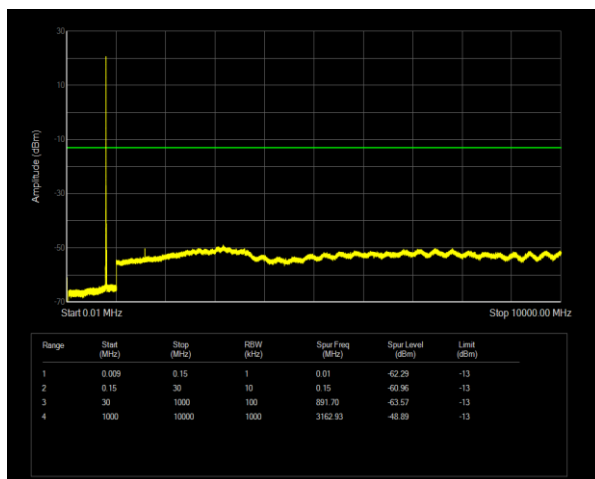
Band14 QPSK BW=10MHz Channel=23330 RB Size=1 Position=#0
