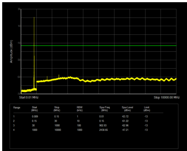
Band26(824-849) QPSK BW=10MHz Channel=26990 RB Size=1 Position=#0
