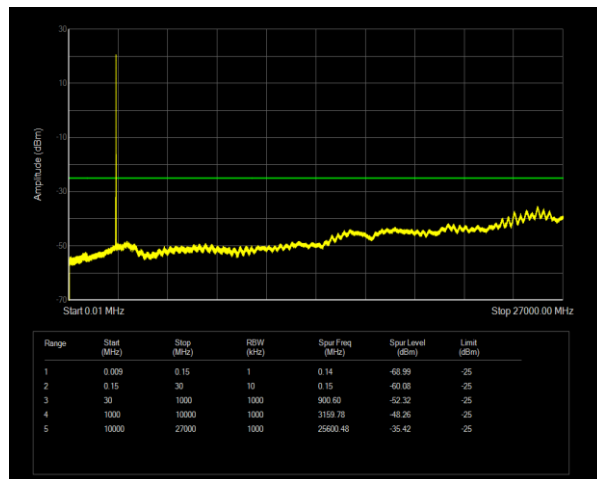
Band38 QPSK BW=10MHz Channel=37800 RB Size=1 Position=#0
