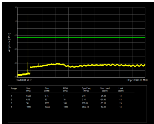
Band5 QPSK BW=10MHz Channel=20450 RB Size=1 Position=#0
