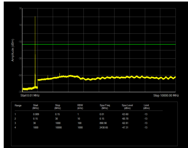
Band26(824-849) QPSK BW=10MHz Channel=26915 RB Size=1 Position=#0
