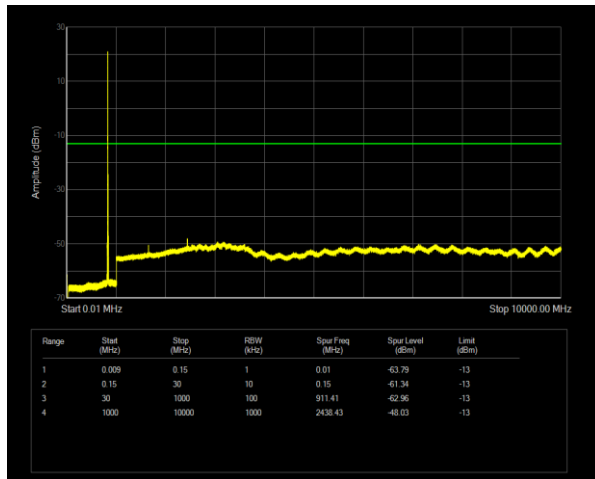
Band26(824-849) QPSK BW=10MHz Channel=26840 RB Size=1 Position=#0
