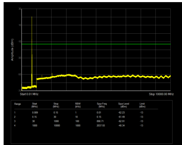
Band71 QPSK BW=20MHz Channel=133372 RB Size=1 Position=#0
