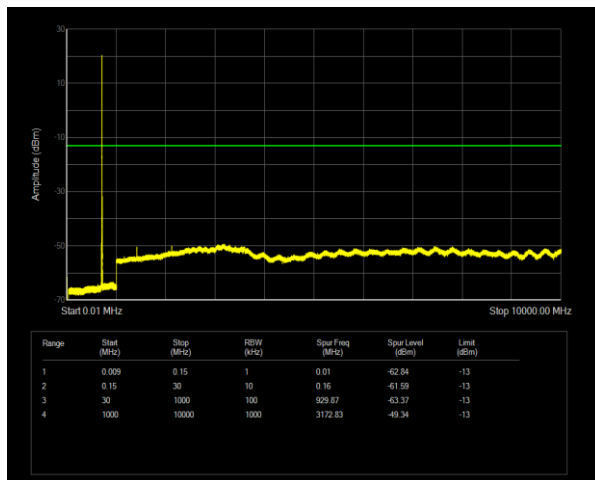
Band12 QPSK BW=10MHz Channel=23130 RB Size=1 Position=#0
