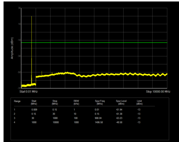
Band12 QPSK BW=10MHz Channel=23095 RB Size=1 Position=#0
