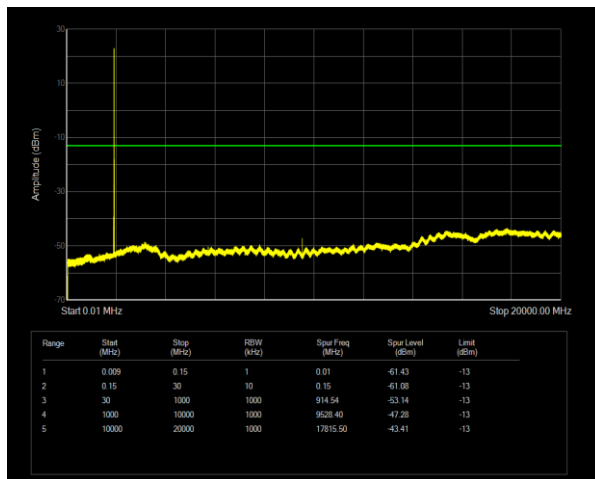
Band25 QPSK BW=10MHz Channel=26640 RB Size=1 Position=#0
