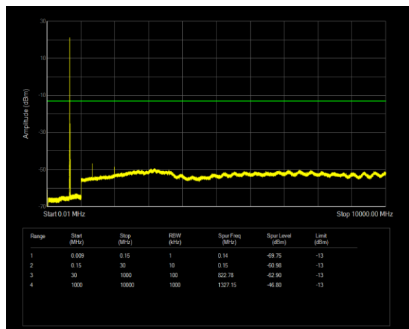
Band71 QPSK BW=10MHz Channel=133172 RB Size=1 Position=#0
