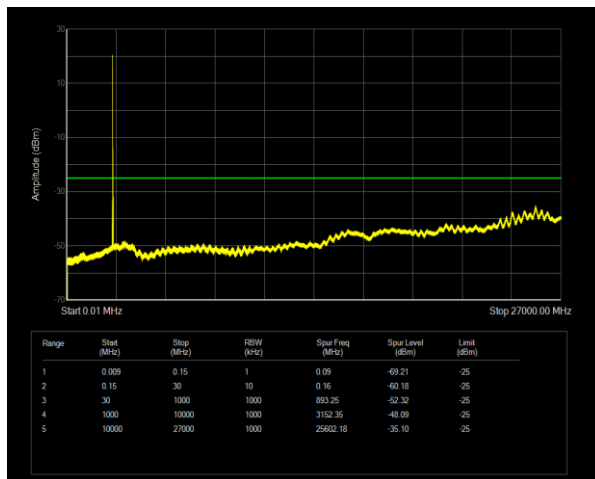
Band41 QPSK BW=10MHz Channel=39700 RB Size=1 Position=#0
