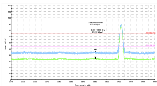
DH5-Channel 0: Peak + Average
