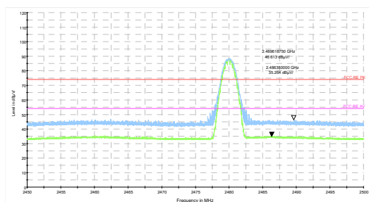
DH5-Channel 78: Peak + Average
