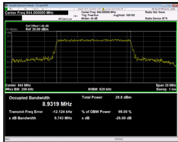
Band26(824-849) 64QAM BW=10MHz Channel=26990 RB Size=50 Position=#0
