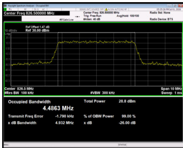
Band26(824-849) 64QAM BW=5MHz Channel=26815 RB Size=25 Position=#0
