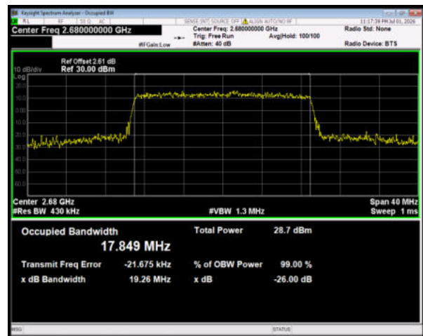
Band41 16QAM BW=20MHz Channel=41490 RB Size=100 Position=#0
