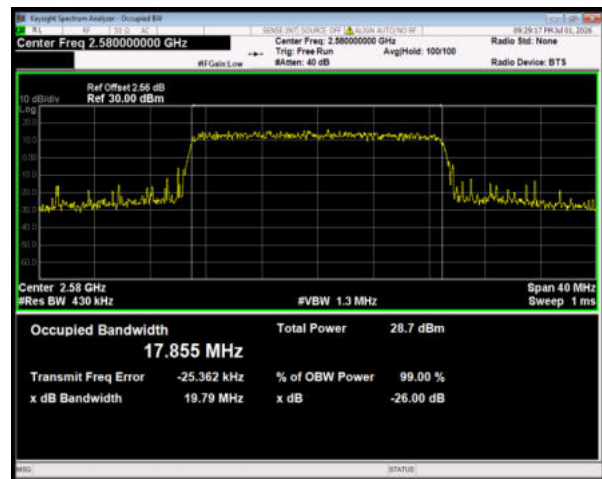
Band38 16QAM BW=20MHz Channel=37850 RB Size=100 Position=#0
