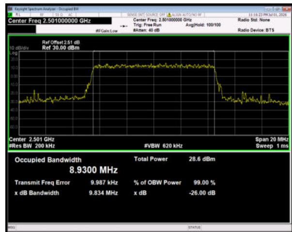
Band41 16QAM BW=10MHz Channel=39700 RB Size=50 Position=#0
