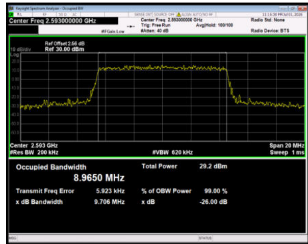
Band41 QPSK BW=10MHz Channel=40620 RB Size=50 Position=#0
