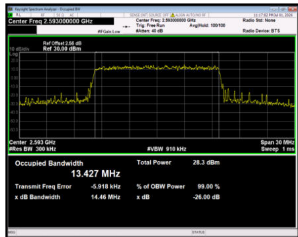
Band41 16QAM BW=15MHz Channel=40620 RB Size=75 Position=#0
