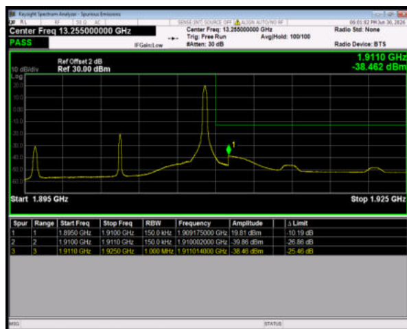
Band2 64QAM BW=15MHz HighChannel=19125 RB Size=1 Position=#Max
