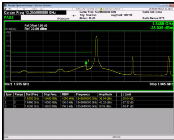
Band2 64QAM BW=15MHz LowChannel=18675 RB Size=1 Position=#0
