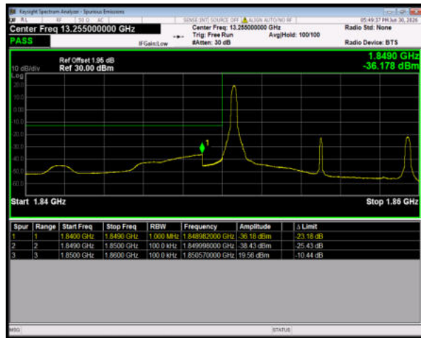
Band2 QPSK BW=10MHz LowChannel=18650 RB Size=1 Position=#0
