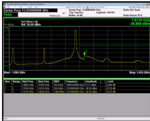
Band2 QPSK BW=15MHz HighChannel=19125 RB Size=1 Position=#Max
