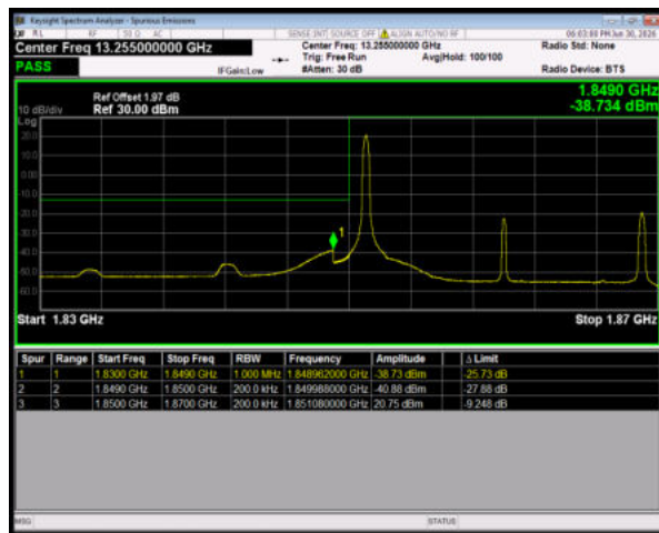
Band2 16QAM BW=20MHz LowChannel=18700 RB Size=1 Position=#0
