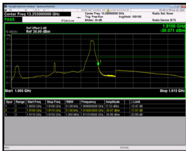
Band2 16QAM BW=5MHz HighChannel=19175 RB Size=1 Position=#Max
