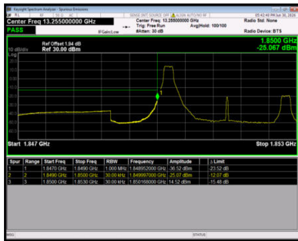
Band2 16QAM BW=3MHz LowChannel=18615 RB Size=1 Position=#0
