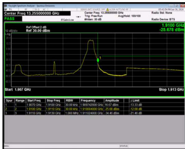
Band2 QPSK BW=3MHz HighChannel=19185 RB Size=1 Position=#Max
