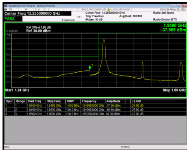
Band2 64QAM BW=10MHz LowChannel=18650 RB Size=1 Position=#0
