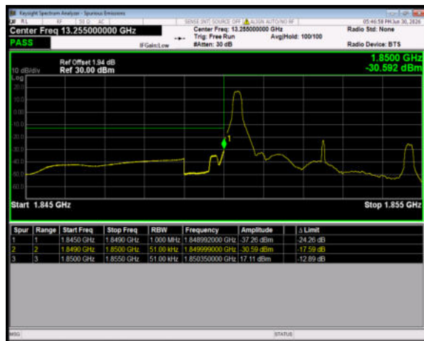
Band2 64QAM BW=5MHz LowChannel=18625 RB Size=1 Position=#0
