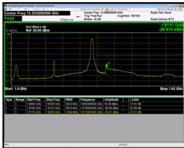
Band2 16QAM BW=10MHz HighChannel=19150 RB Size=1 Position=#Max
