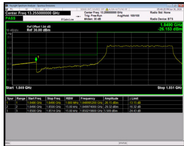
Band2 QPSK BW=1.4MHz LowChannel=18607 RB Size=6 Position=#0
