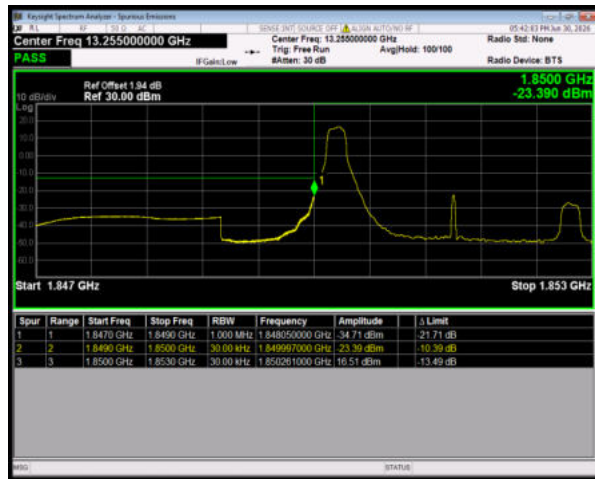
Band2 QPSK BW=3MHz LowChannel=18615 RB Size=1 Position=#0
