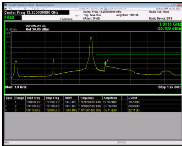
Band2 QPSK BW=10MHz HighChannel=19150 RB Size=1 Position=#Max
