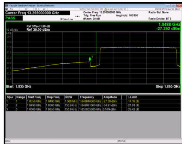
Band2 64QAM BW=15MHz LowChannel=18675 RB Size=75 Position=#0
