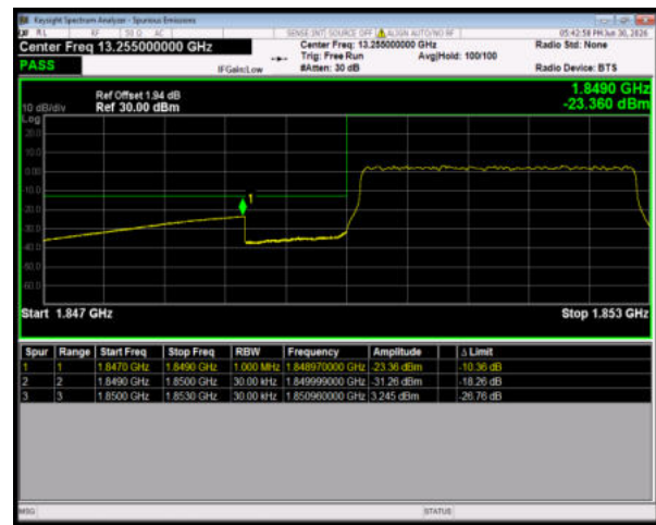
Band2 16QAM BW=3MHz LowChannel=18615 RB Size=15 Position=#0
