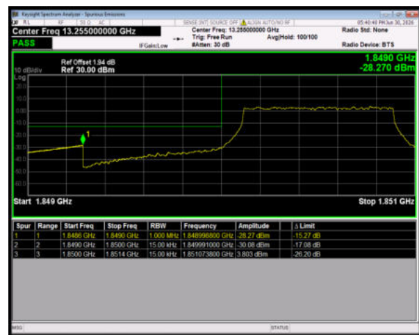
Band2 16QAM BW=1.4MHz LowChannel=18607 RB Size=6 Position=#0
