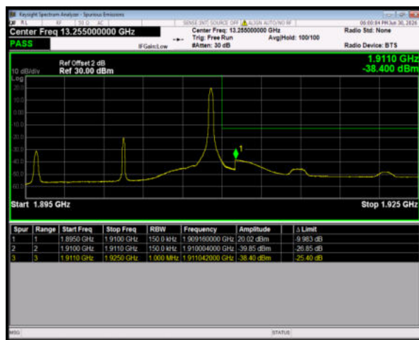
Band2 16QAM BW=15MHz HighChannel=19125 RB Size=1 Position=#Max
