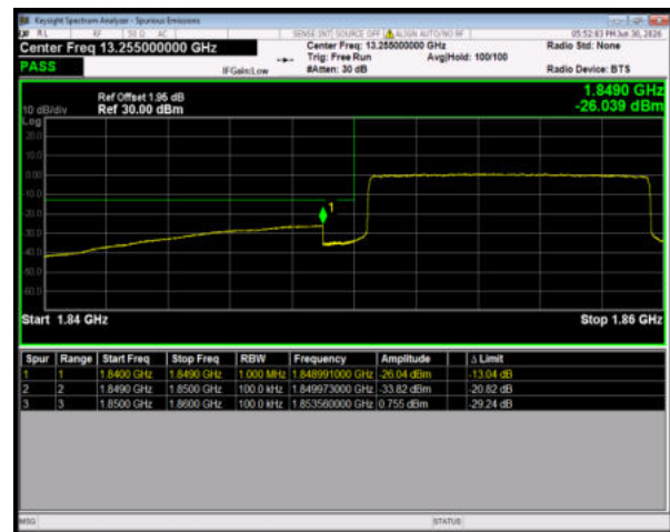
Band2 64QAM BW=10MHz LowChannel=18650 RB Size=50 Position=#0
