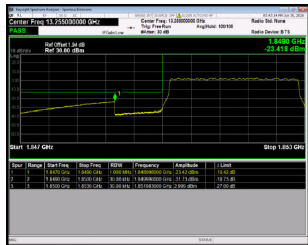
Band2 64QAM BW=3MHz LowChannel=18615 RB Size=15 Position=#0
