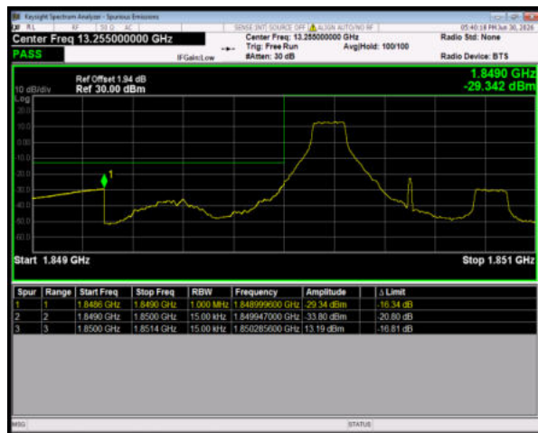
Band2 QPSK BW=1.4MHz LowChannel=18607 RB Size=1 Position=#0
