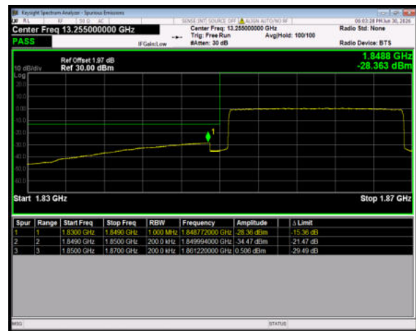
Band2 16QAM BW=20MHz LowChannel=18700 RB Size=100 Position=#0
