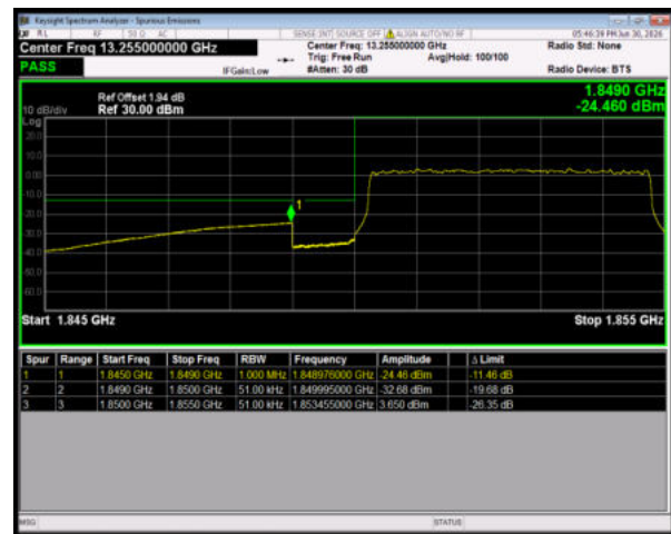
Band2 16QAM BW=5MHz LowChannel=18625 RB Size=25 Position=#0
