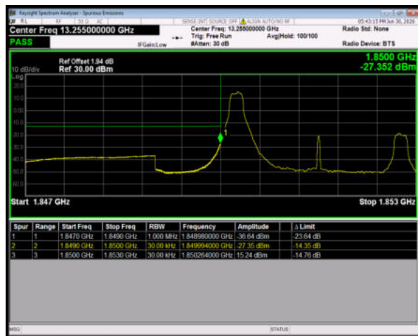
Band2 64QAM BW=3MHz LowChannel=18615 RB Size=1 Position=#0
