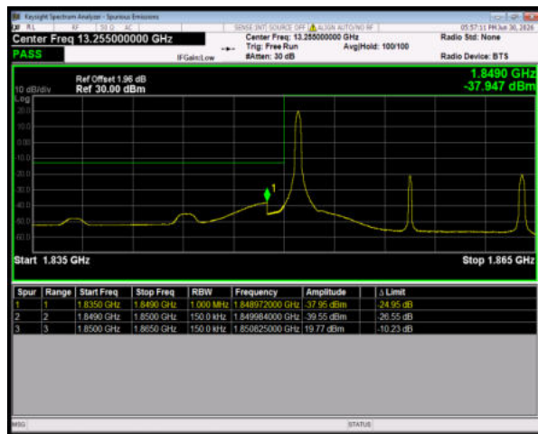
Band2 16QAM BW=15MHz LowChannel=18675 RB Size=1 Position=#0
