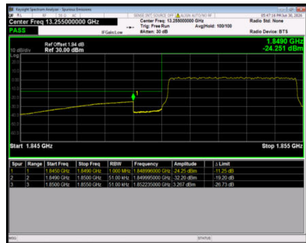
Band2 64QAM BW=5MHz LowChannel=18625 RB Size=25 Position=#0
