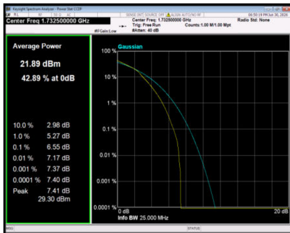
Band4 16QAM BW=1.4MHz Channel=20175 RB Size=6 Position=#0
