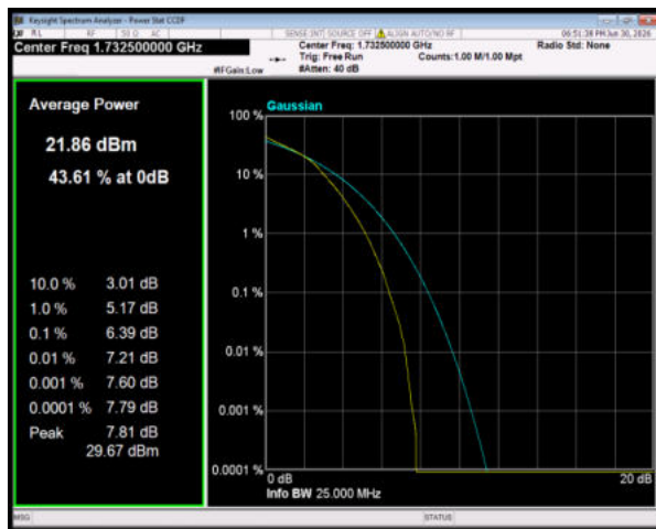
Band4 64QAM BW=10MHz Channel=20175 RB Size=50 Position=#0
