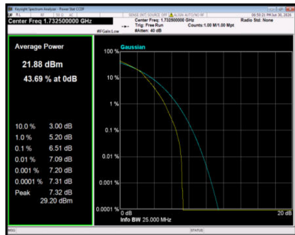
Band4 64QAM BW=1.4MHz Channel=20175 RB Size=6 Position=#0
