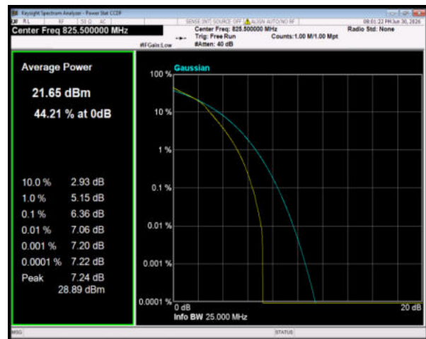
Band5 64QAM BW=3MHz Channel=20415 RB Size=15 Position=#0
