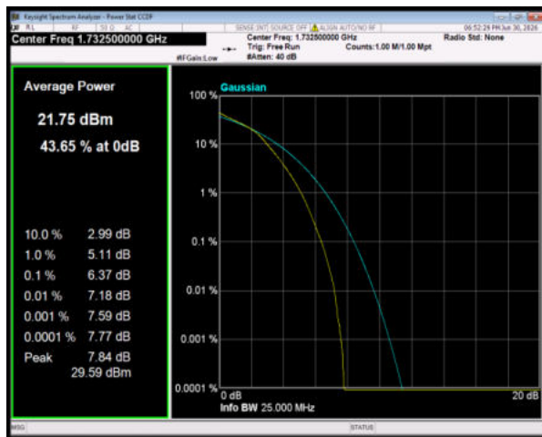
Band4 64QAM BW=20MHz Channel=20175 RB Size=100 Position=#0
