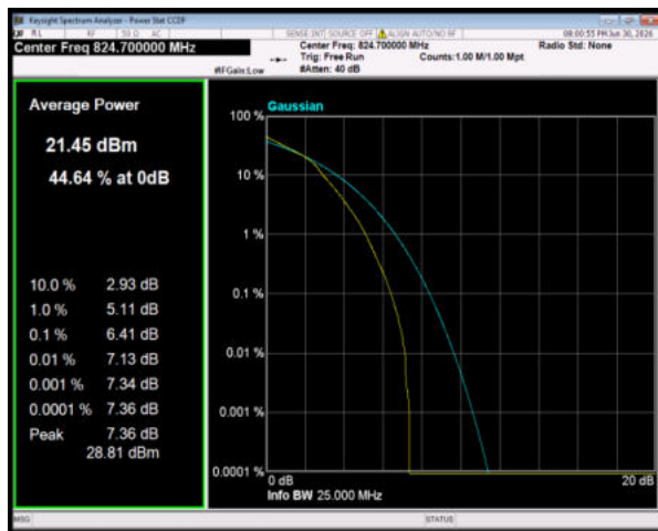
Band5 64QAM BW=1.4MHz Channel=20407 RB Size=6 Position=#0
