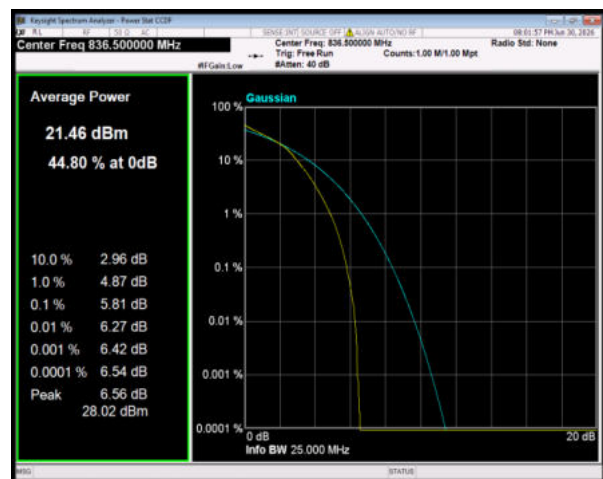
Band5 64QAM BW=5MHz Channel=20525 RB Size=25 Position=#0
