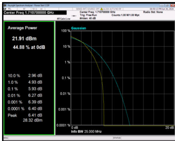
Band4 64QAM BW=1.4MHz Channel=19957 RB Size=6 Position=#0
