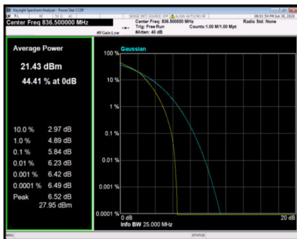
Band5 16QAM BW=5MHz Channel=20525 RB Size=25 Position=#0
