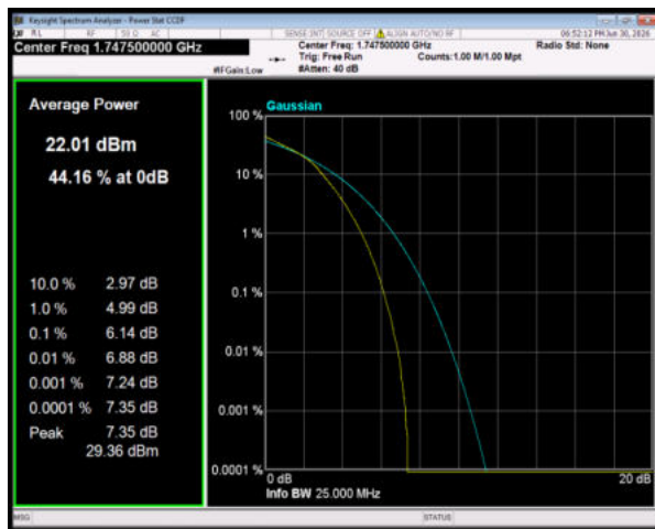
Band4 64QAM BW=15MHz Channel=20325 RB Size=75 Position=#0
