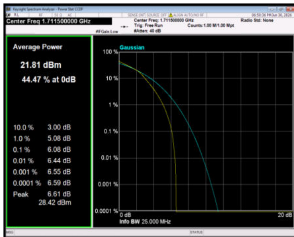
Band4 16QAM BW=3MHz Channel=19965 RB Size=15 Position=#0
