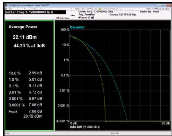
Band4 64QAM BW=10MHz Channel=20350 RB Size=50 Position=#0
