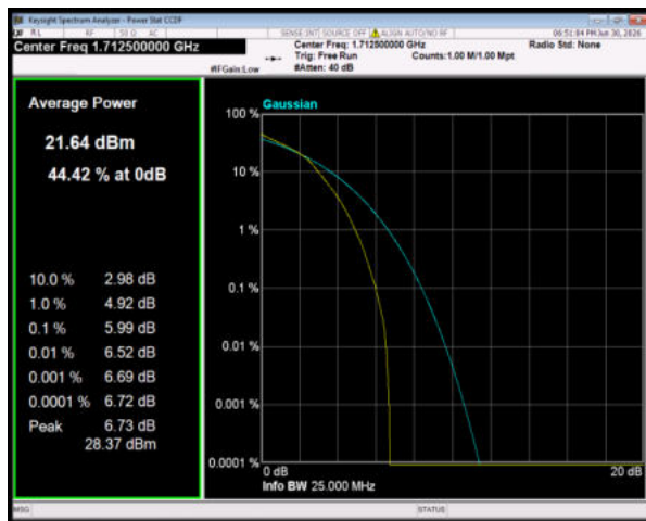
Band4 64QAM BW=5MHz Channel=19975 RB Size=25 Position=#0
