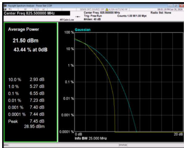
Band5 16QAM BW=3MHz Channel=20415 RB Size=15 Position=#0
