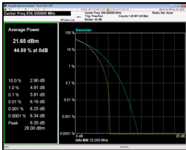
Band5 16QAM BW=1.4MHz Channel=20525 RB Size=6 Position=#0
