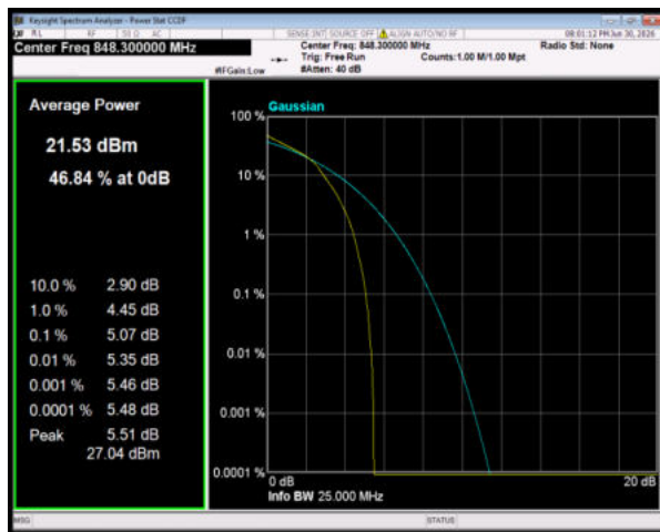
Band5 64QAM BW=1.4MHz Channel=20643 RB Size=6 Position=#0
