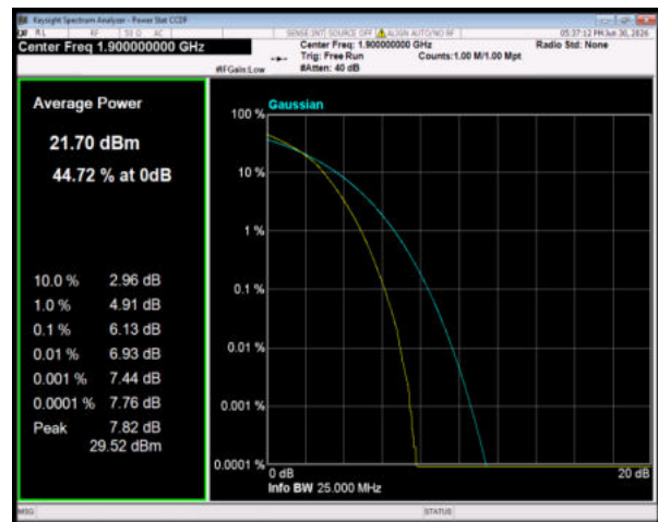
Band2 64QAM BW=20MHz Channel=19100 RB Size=100 Position=#0
