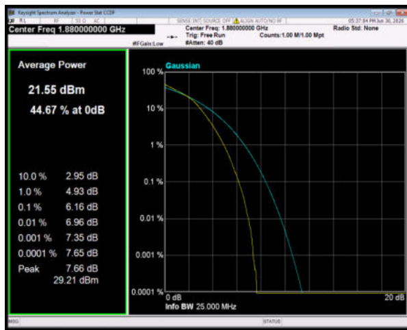
Band2 64QAM BW=20MHz Channel=18900 RB Size=100 Position=#0
