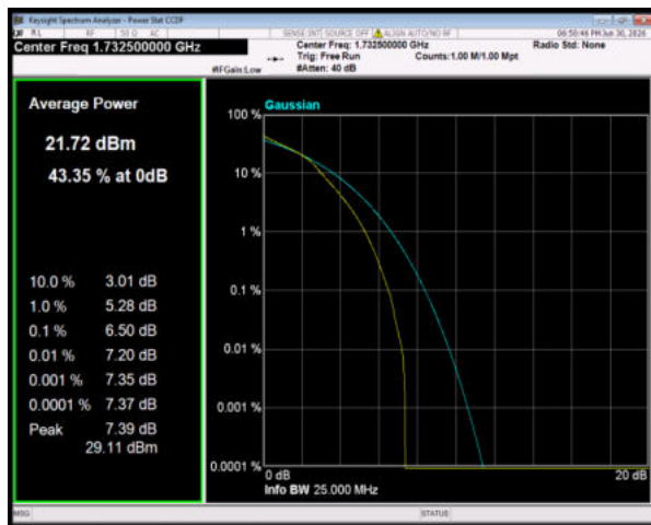
Band4 64QAM BW=3MHz Channel=20175 RB Size=15 Position=#0
