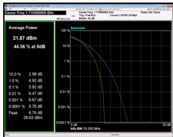
Band4 64QAM BW=10MHz Channel=20000 RB Size=50 Position=#0
