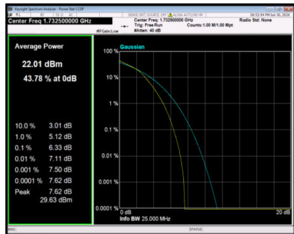
Band4 64QAM BW=15MHz Channel=20175 RB Size=75 Position=#0
