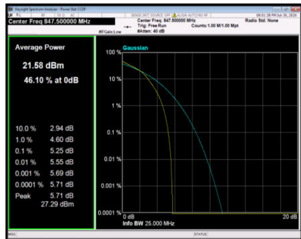
Band5 64QAM BW=3MHz Channel=20635 RB Size=15 Position=#0
