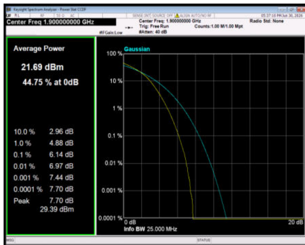
Band2 16QAM BW=20MHz Channel=19100 RB Size=100 Position=#0
