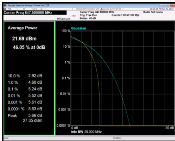
Band5 16QAM BW=3MHz Channel=20635 RB Size=15 Position=#0
