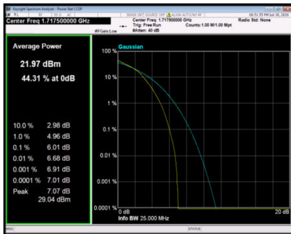
Band4 64QAM BW=15MHz Channel=20025 RB Size=75 Position=#0
