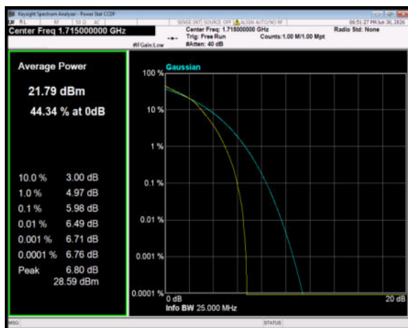
Band4 16QAM BW=10MHz Channel=20000 RB Size=50 Position=#0
