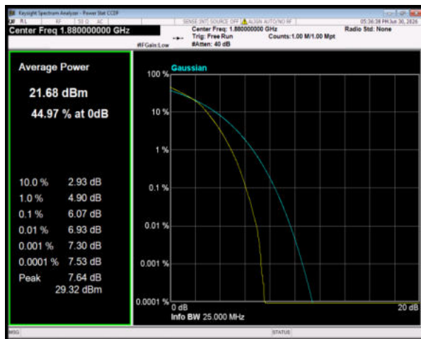
Band2 16QAM BW=15MHz Channel=18900 RB Size=75 Position=#0
