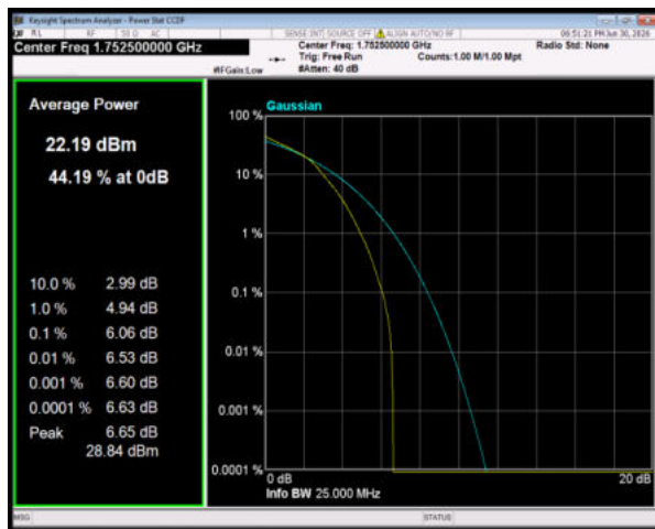
Band4 64QAM BW=5MHz Channel=20375 RB Size=25 Position=#0
