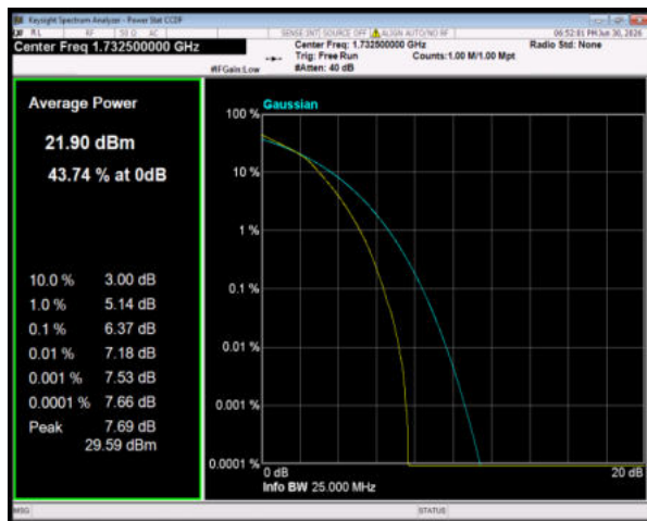
Band4 16QAM BW=15MHz Channel=20175 RB Size=75 Position=#0
