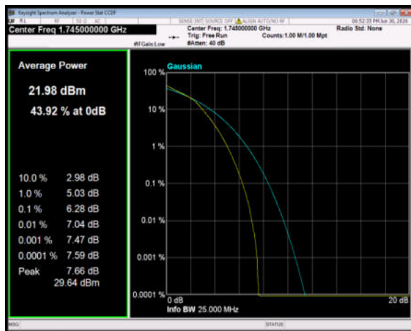
Band4 16QAM BW=20MHz Channel=20300 RB Size=100 Position=#0
