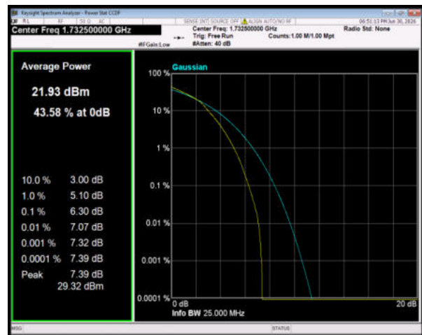
Band4 64QAM BW=5MHz Channel=20175 RB Size=25 Position=#0
