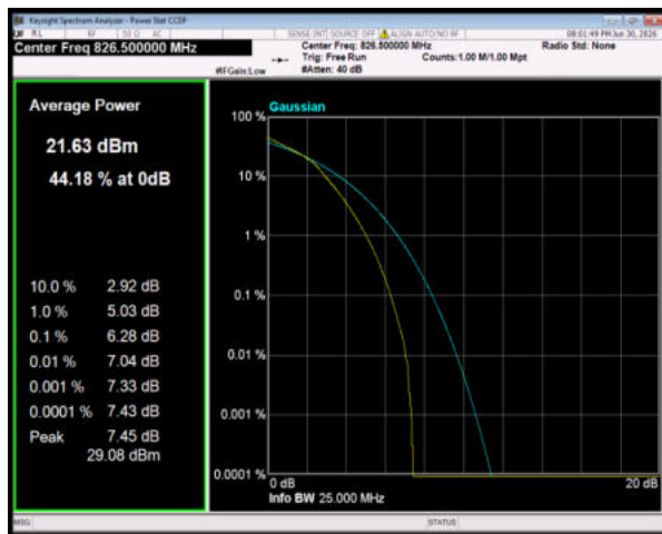
Band5 64QAM BW=5MHz Channel=20425 RB Size=25 Position=#0
