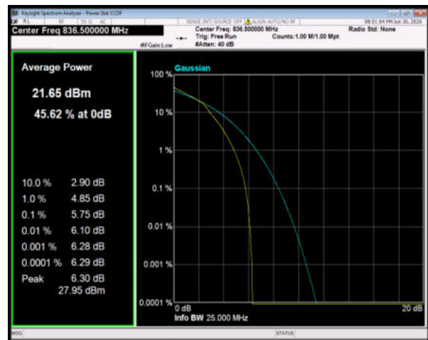
Band5 64QAM BW=1.4MHz Channel=20525 RB Size=6 Position=#0
