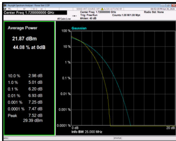
Band4 16QAM BW=20MHz Channel=20050 RB Size=100 Position=#0
