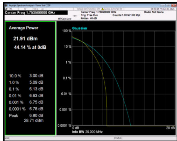
Band4 64QAM BW=3MHz Channel=20385 RB Size=15 Position=#0
