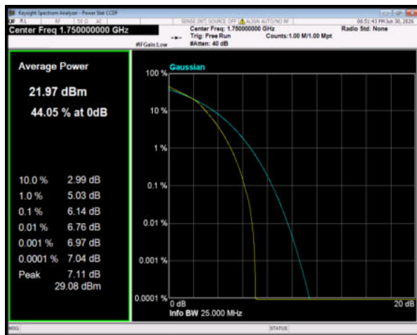
Band4 16QAM BW=10MHz Channel=20350 RB Size=50 Position=#0
