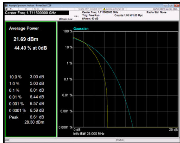
Band4 64QAM BW=3MHz Channel=19965 RB Size=15 Position=#0
