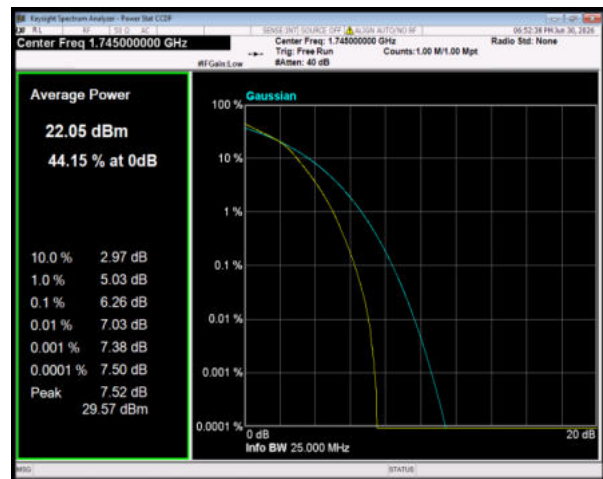
Band4 64QAM BW=20MHz Channel=20300 RB Size=100 Position=#0
