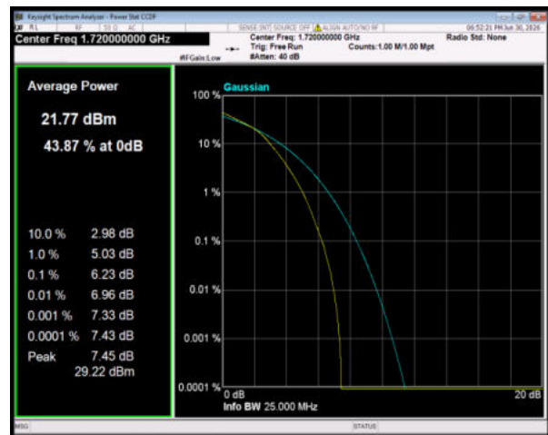
Band4 64QAM BW=20MHz Channel=20050 RB Size=100 Position=#0
