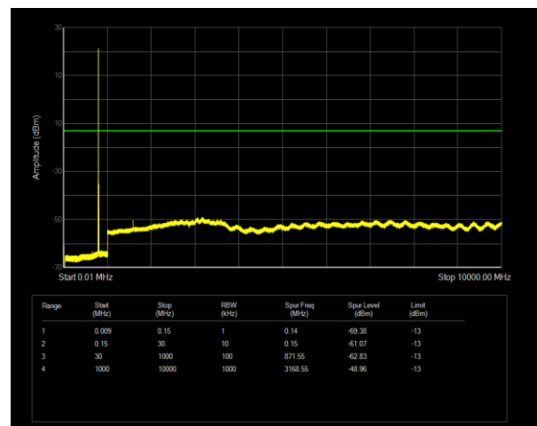
Band14 QPSK BW=5MHz Channel=23330 RB Size=1 Position=#0
