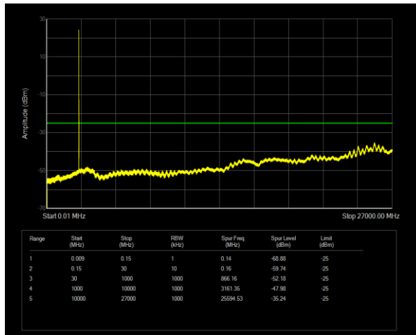
Band7 QPSK BW=5MHz Channel=20775 RB Size=1 Position=#0
