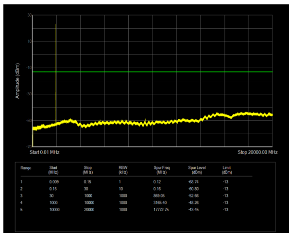
Band2 QPSK BW=3MHz Channel=18900 RB Size=1 Position=#0
