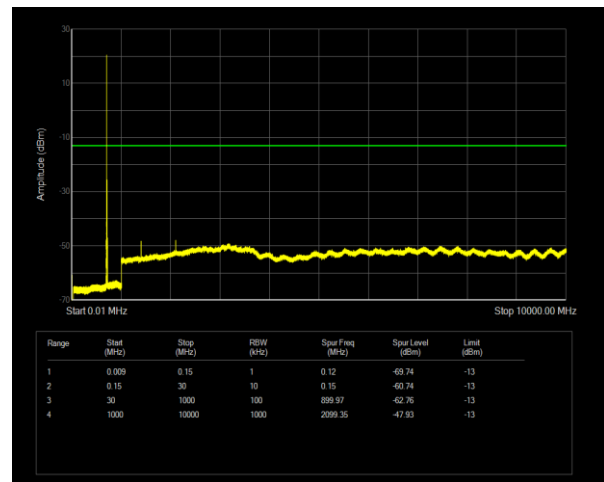
Band12 QPSK BW=10MHz Channel=23060 RB Size=1 Position=#0
