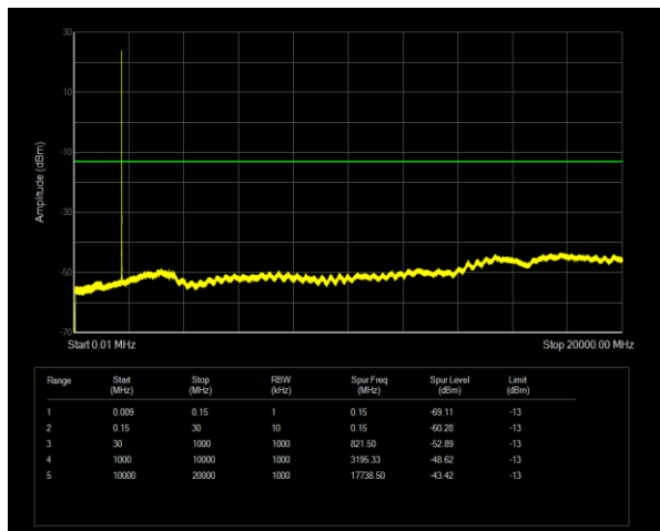
Band4 QPSK BW=3MHz Channel=20175 RB Size=1 Position=#0
