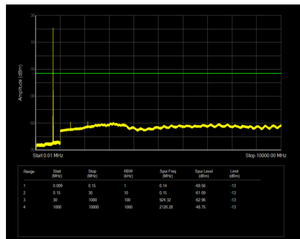
Band12 QPSK BW=10MHz Channel=23130 RB Size=1 Position=#0
