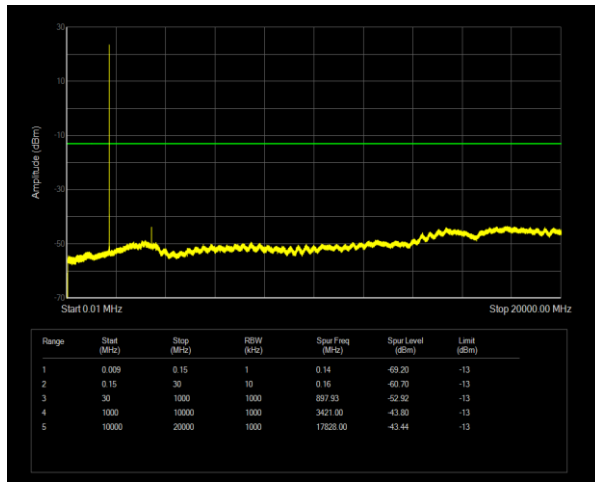
Band4 QPSK BW=1.4MHz Channel=19957 RB Size=1 Position=#0
