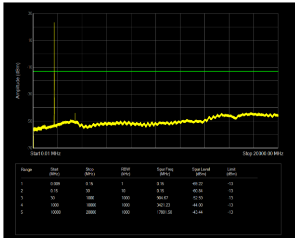
Band4 QPSK BW=5MHz Channel=19975 RB Size=1 Position=#0
