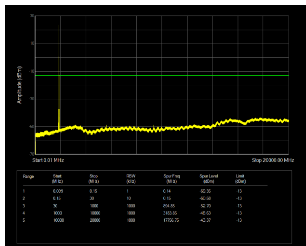
Band2 QPSK BW=20MHz Channel=18900 RB Size=1 Position=#0
