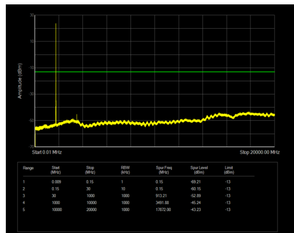
Band4 QPSK BW=10MHz Channel=20350 RB Size=1 Position=#0
