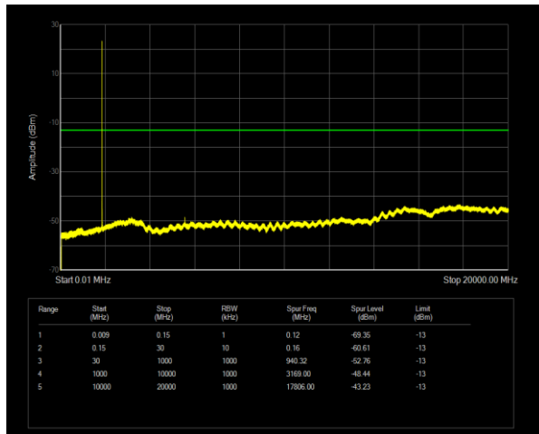
Band2 QPSK BW=1.4MHz Channel=18607 RB Size=1 Position=#0
