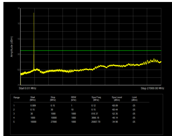
Band7 QPSK BW=20MHz Channel=21350 RB Size=1 Position=#0
