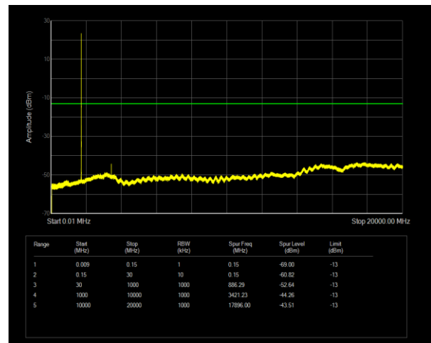
Band4 QPSK BW=3MHz Channel=19965 RB Size=1 Position=#0
