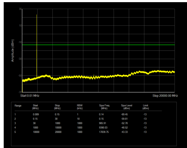
Band2 QPSK BW=5MHz Channel=18900 RB Size=1 Position=#0
