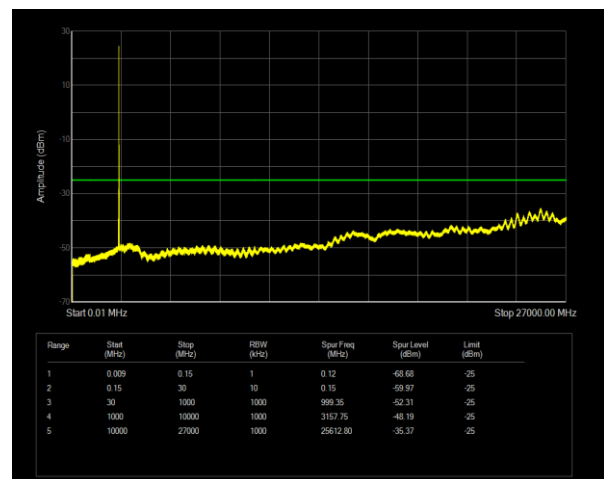
Band7 QPSK BW=10MHz Channel=21400 RB Size=1 Position=#0
