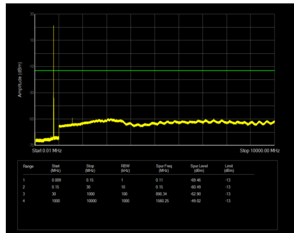
Band13 QPSK BW=5MHz Channel=23230 RB Size=1 Position=#0
