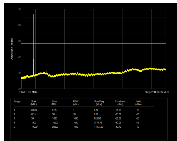
Band4 QPSK BW=20MHz Channel=20300 RB Size=1 Position=#0
