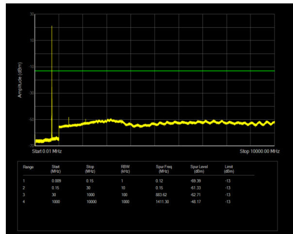
Band12 QPSK BW=5MHz Channel=23095 RB Size=1 Position=#0
