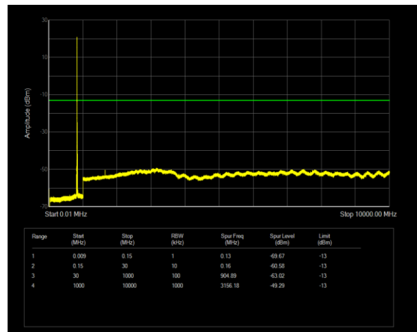
Band5 QPSK BW=10MHz Channel=20450 RB Size=1 Position=#0
