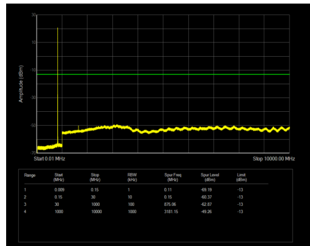
Band5 QPSK BW=3MHz Channel=20415 RB Size=1 Position=#0
