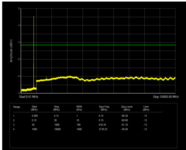
Band5 QPSK BW=1.4MHz Channel=20407 RB Size=1 Position=#0
