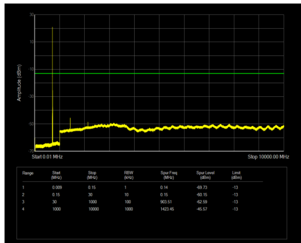
Band12 QPSK BW=5MHz Channel=23155 RB Size=1 Position=#0
