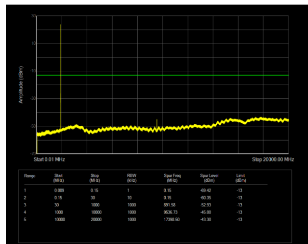
Band2 QPSK BW=3MHz Channel=19185 RB Size=1 Position=#0
