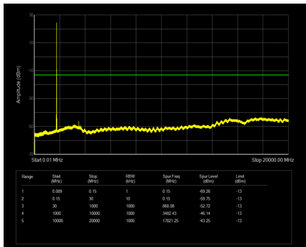
Band4 QPSK BW=15MHz Channel=20325 RB Size=1 Position=#0
