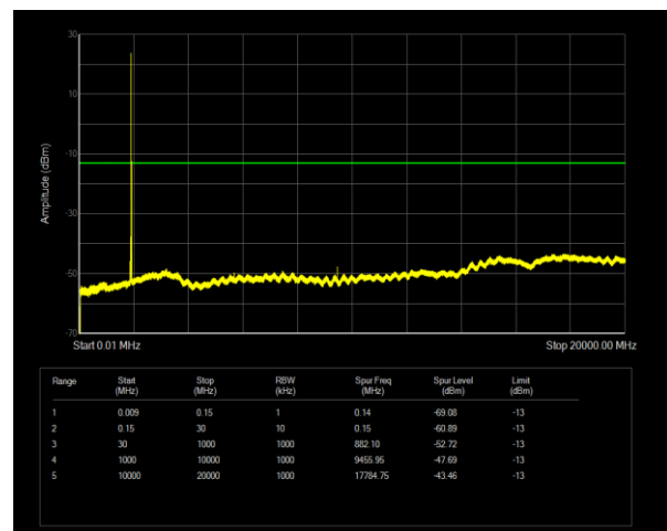
Band2 QPSK BW=20MHz Channel=19100 RB Size=1 Position=#0
