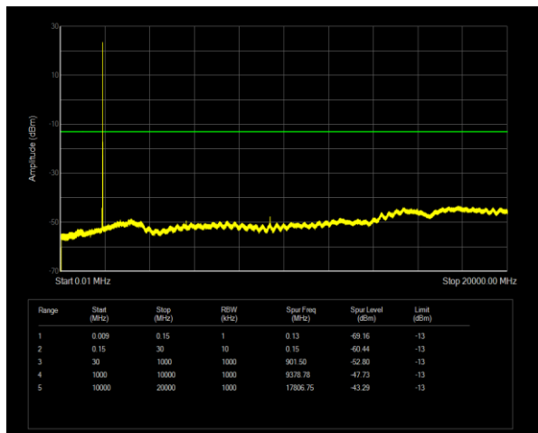
Band2 QPSK BW=10MHz Channel=18900 RB Size=1 Position=#0
