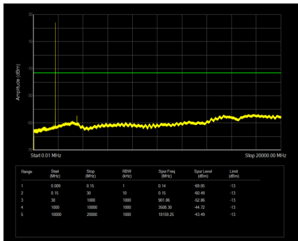
Band4 QPSK BW=1.4MHz Channel=20393 RB Size=1 Position=#0
