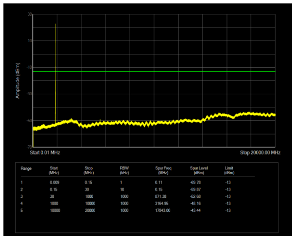
Band2 QPSK BW=5MHz Channel=18625 RB Size=1 Position=#0
