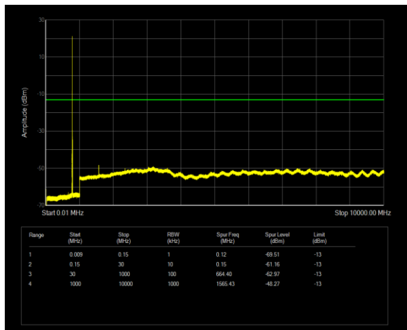
Band13 QPSK BW=5MHz Channel=23255 RB Size=1 Position=#0
