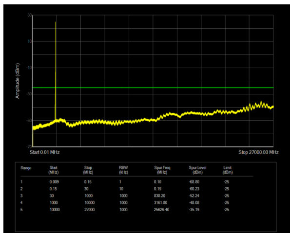
Band7 QPSK BW=10MHz Channel=21100 RB Size=1 Position=#0
