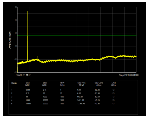
Band4 QPSK BW=10MHz Channel=20000 RB Size=1 Position=#0
