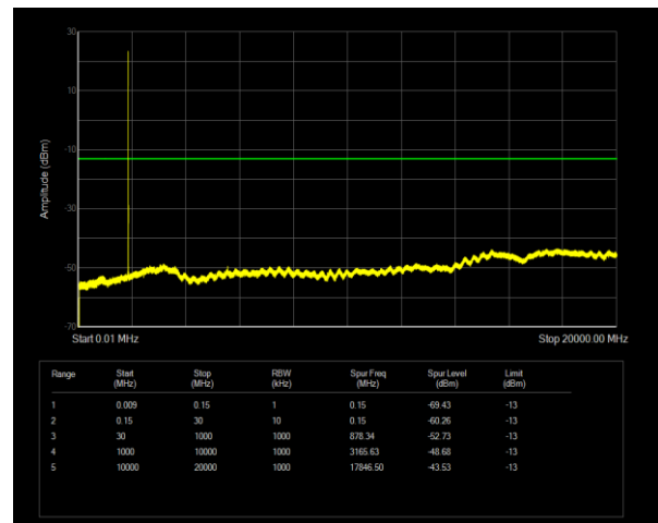
Band2 QPSK BW=3MHz Channel=18615 RB Size=1 Position=#0
