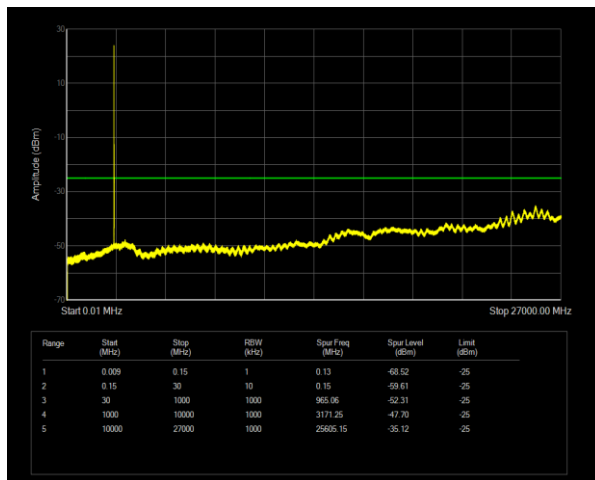
Band7 QPSK BW=5MHz Channel=21425 RB Size=1 Position=#0
