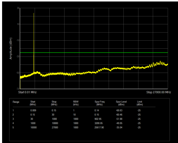
Band7 QPSK BW=15MHz Channel=20825 RB Size=1 Position=#0
