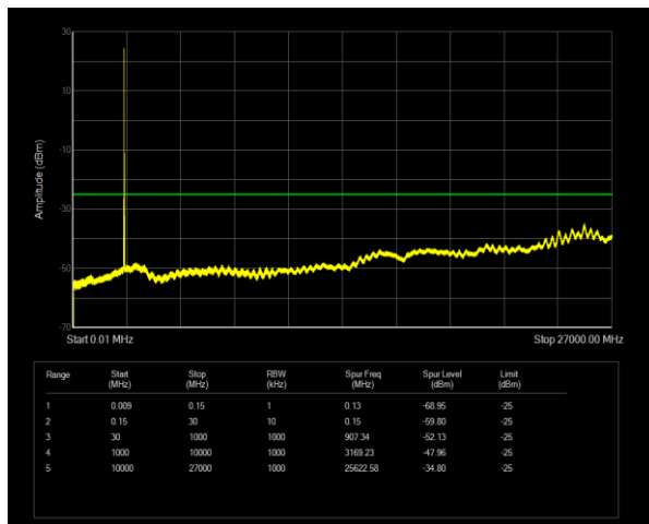
Band7 QPSK BW=15MHz Channel=21375 RB Size=1 Position=#0
