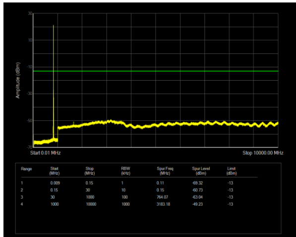
Band5 QPSK BW=5MHz Channel=20425 RB Size=1 Position=#0
