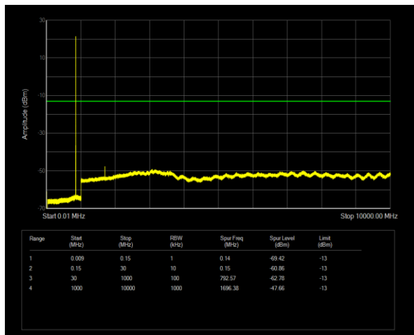
Band5 QPSK BW=1.4MHz Channel=20643 RB Size=1 Position=#0
