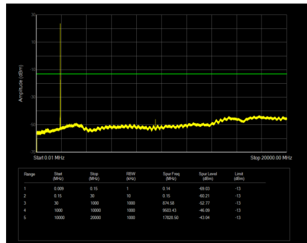
Band2 QPSK BW=10MHz Channel=19150 RB Size=1 Position=#0
