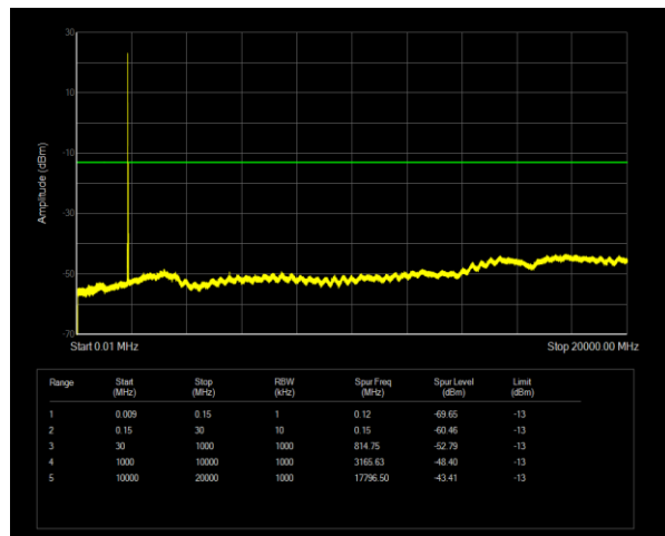
Band2 QPSK BW=15MHz Channel=18675 RB Size=1 Position=#0
