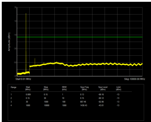
Band12 QPSK BW=1.4MHz Channel=23173 RB Size=1 Position=#0
