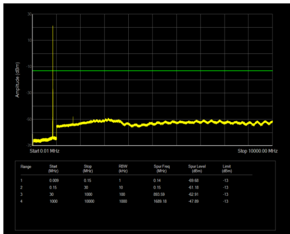
Band5 QPSK BW=5MHz Channel=20625 RB Size=1 Position=#0
