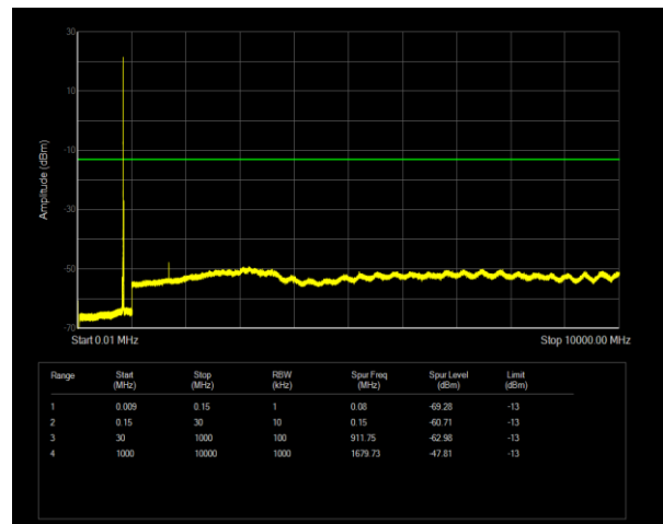
Band5 QPSK BW=10MHz Channel=20600 RB Size=1 Position=#0
