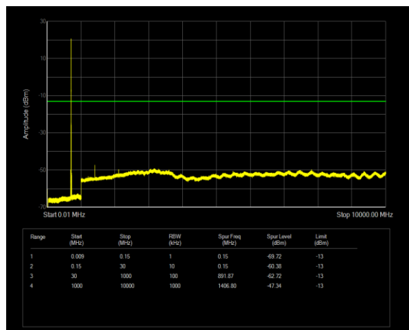
Band12 QPSK BW=10MHz Channel=23095 RB Size=1 Position=#0
