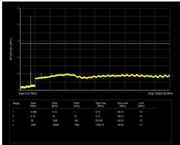
Band12 QPSK BW=1.4MHz Channel=23017 RB Size=1 Position=#0
