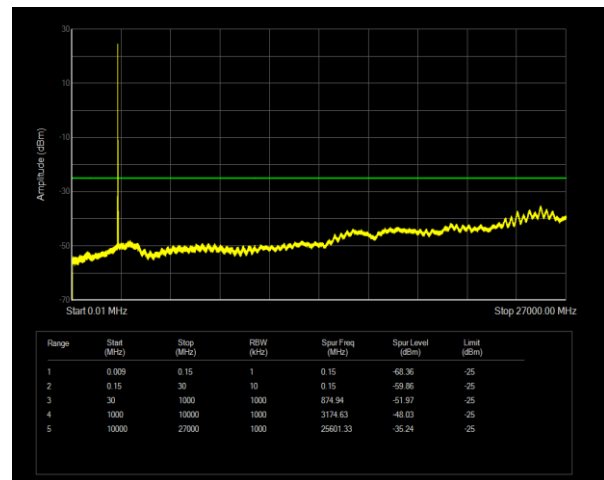
Band7 QPSK BW=20MHz Channel=20850 RB Size=1 Position=#0
