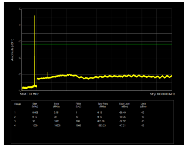
Band5 QPSK BW=3MHz Channel=20635 RB Size=1 Position=#0
