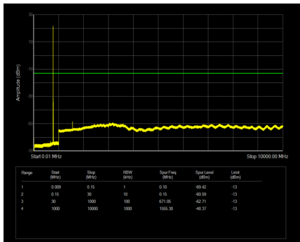
Band13 QPSK BW=5MHz Channel=23205 RB Size=1 Position=#0
