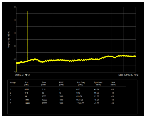
Band2 QPSK BW=5MHz Channel=19175 RB Size=1 Position=#0
