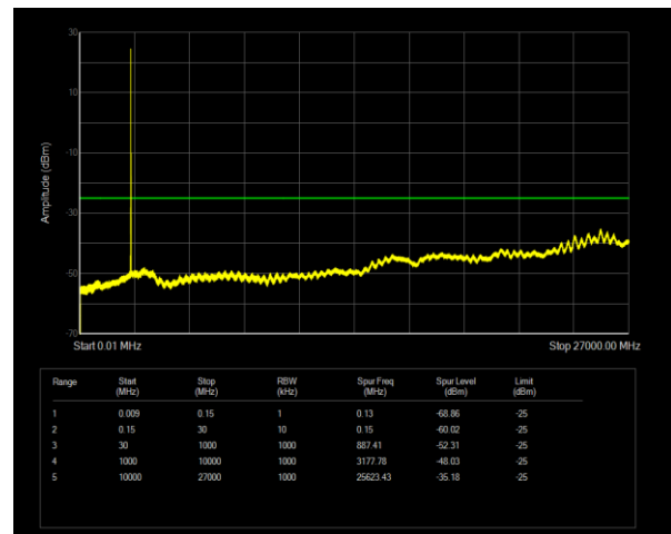
Band7 QPSK BW=10MHz Channel=20800 RB Size=1 Position=#0
