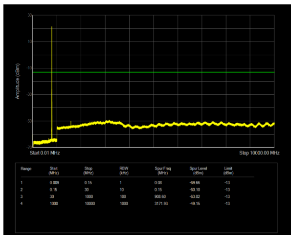
Band14 QPSK BW=5MHz Channel=23305 RB Size=1 Position=#0
