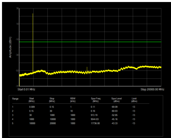
Band2 QPSK BW=1.4MHz Channel=19193 RB Size=1 Position=#0
