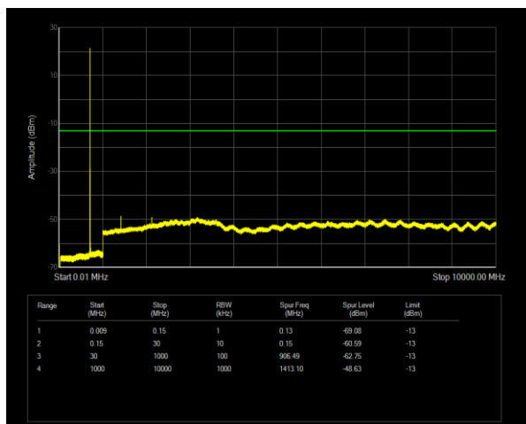
Band12 QPSK BW=3MHz Channel=23095 RB Size=1 Position=#0
