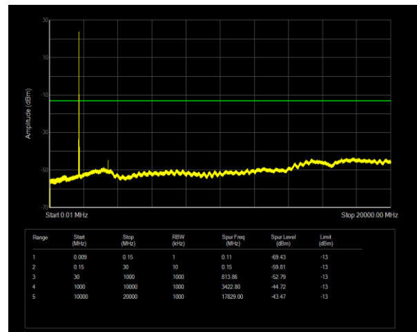
Band4 QPSK BW=20MHz Channel=20050 RB Size=1 Position=#0
