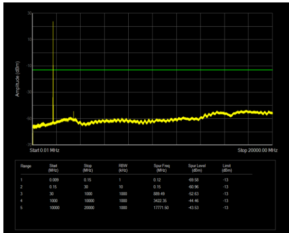
Band4 QPSK BW=15MHz Channel=20025 RB Size=1 Position=#0
