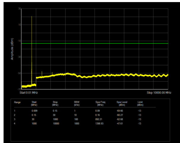
Band12 QPSK BW=3MHz Channel=23025 RB Size=1 Position=#0
