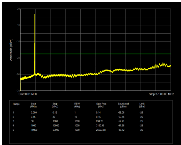
Band7 QPSK BW=20MHz Channel=21100 RB Size=1 Position=#0
