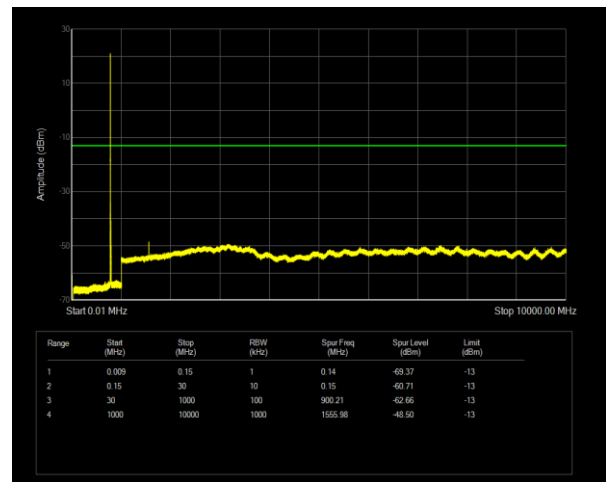
Band13 QPSK BW=10MHz Channel=23230 RB Size=1 Position=#0
