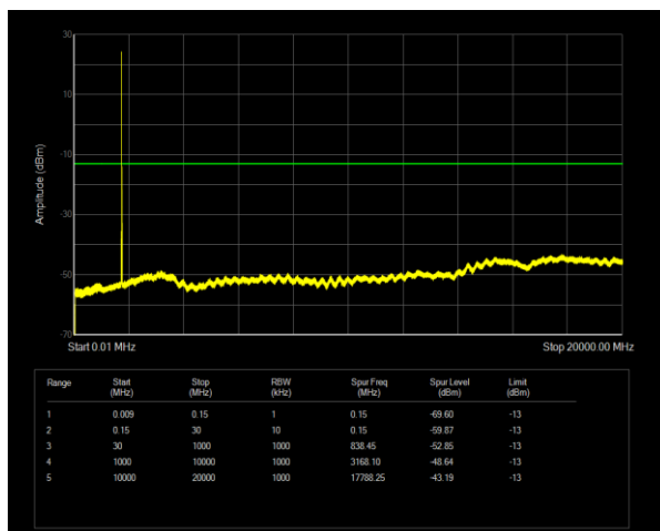
Band4 QPSK BW=10MHz Channel=20175 RB Size=1 Position=#0
