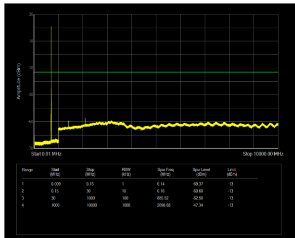
Band12 QPSK BW=5MHz Channel=23035 RB Size=1 Position=#0
