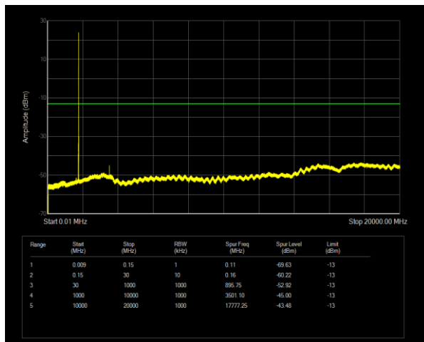
Band4 QPSK BW=5MHz Channel=20375 RB Size=1 Position=#0
