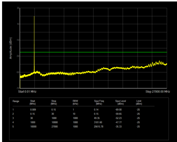
Band38 QPSK BW=10MHz Channel=38200 RB Size=1 Position=#0
