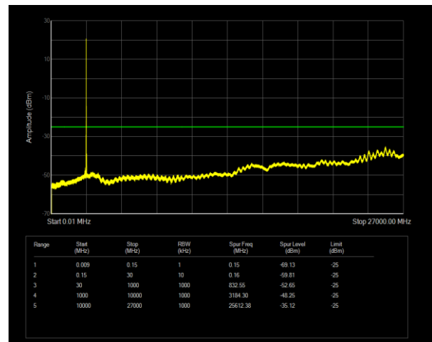
Band41 QPSK BW=15MHz Channel=41515 RB Size=1 Position=#0
