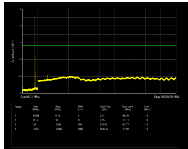
Band26(814-824) QPSK BW=10MHz Channel=26740 RB Size=1 Position=#0
