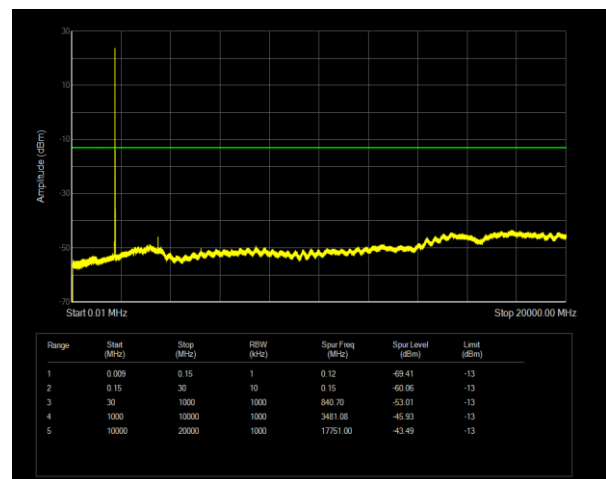
Band66 QPSK BW=10MHz Channel=132322 RB Size=1 Position=#0
