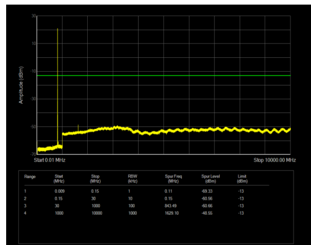
Band26(814-824) QPSK BW=3MHz Channel=26705 RB Size=1 Position=#0
