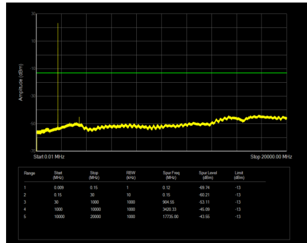
Band66 QPSK BW=1.4MHz Channel=131979 RB Size=1 Position=#0
