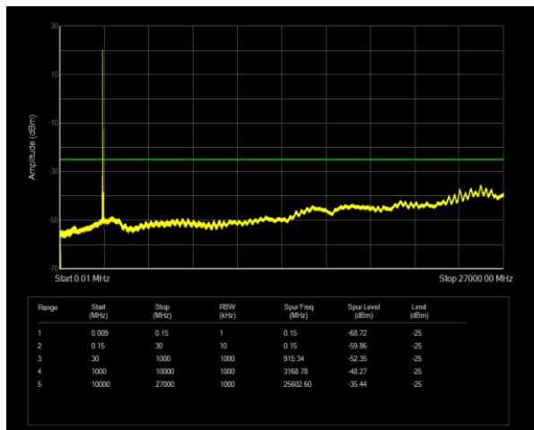
Band41 QPSK BW=15MHz Channel=40620 RB Size=1 Position=#0
