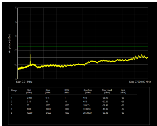
Band38 QPSK BW=20MHz Channel=37850 RB Size=1 Position=#0
