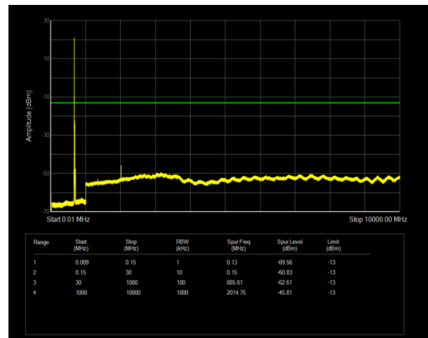
Band71 QPSK BW=20MHz Channel=133297 RB Size=1 Position=#0
