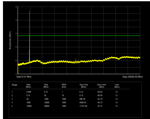
Band25 QPSK BW=20MHz Channel=26590 RB Size=1 Position=#0
