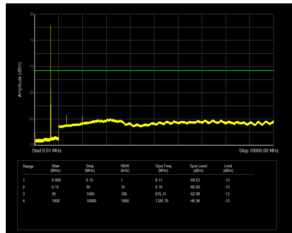
Band71 QPSK BW=5MHz Channel=133147 RB Size=1 Position=#0
