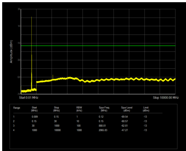
Band71 QPSK BW=10MHz Channel=133422 RB Size=1 Position=#0
