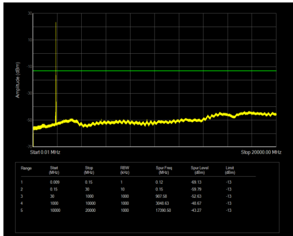
Band25 QPSK BW=20MHz Channel=26365 RB Size=1 Position=#0
