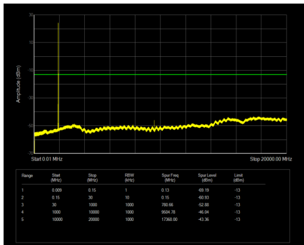
Band25 QPSK BW=15MHz Channel=26615 RB Size=1 Position=#0
