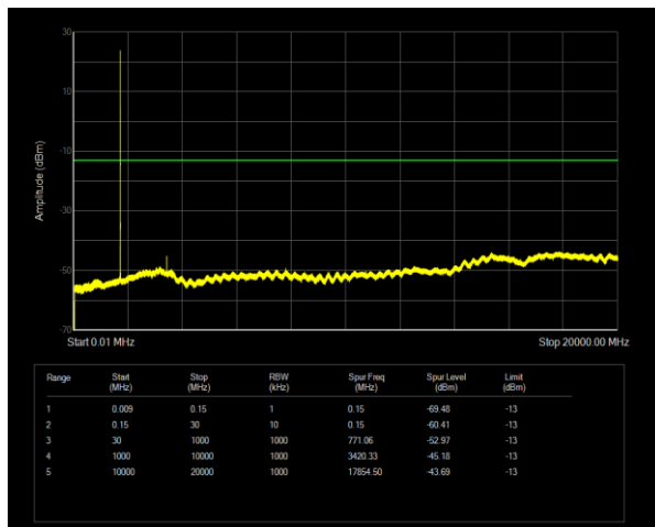
Band66 QPSK BW=3MHz Channel=131987 RB Size=1 Position=#0
