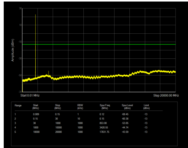
Band66 QPSK BW=5MHz Channel=131997 RB Size=1 Position=#0
