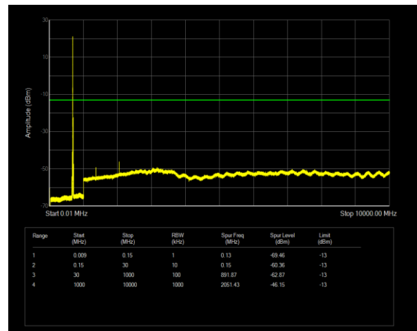
Band71 QPSK BW=15MHz Channel=133397 RB Size=1 Position=#0
