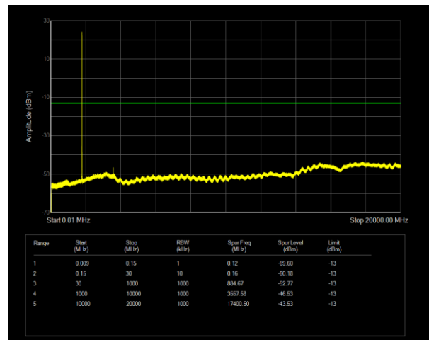
Band66 QPSK BW=1.4MHz Channel=132665 RB Size=1 Position=#0
