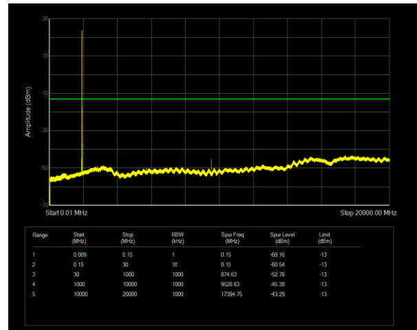
Band25 QPSK BW=10MHz Channel=26640 RB Size=1 Position=#0
