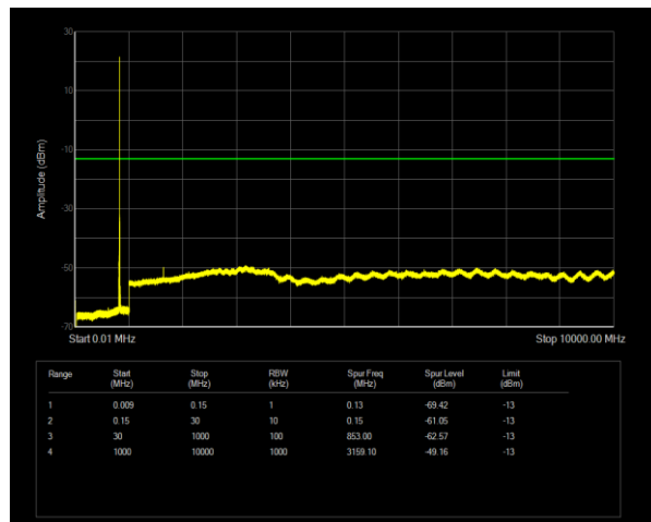
Band26(814-824) QPSK BW=5MHz Channel=26765 RB Size=1 Position=#0
