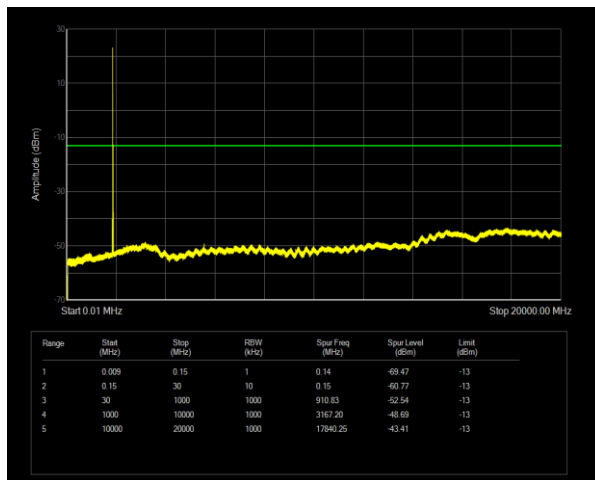
Band25 QPSK BW=15MHz Channel=26115 RB Size=1 Position=#0
