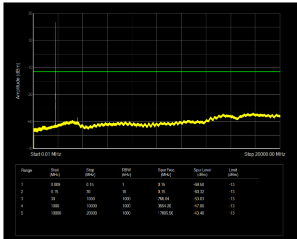
Band66 QPSK BW=3MHz Channel=132657 RB Size=1 Position=#0
