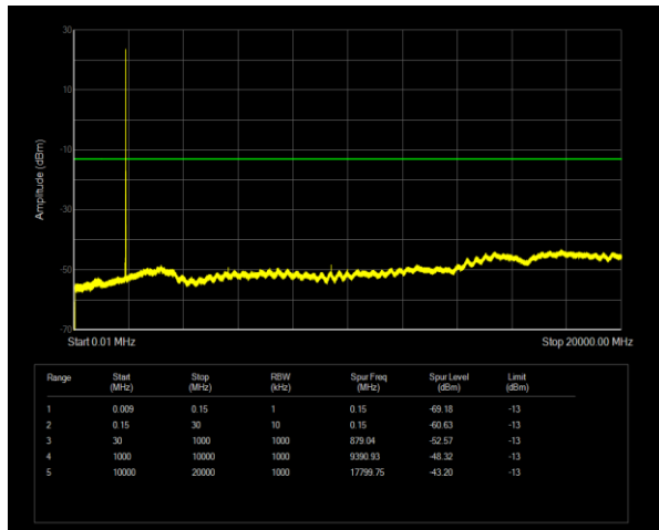
Band25 QPSK BW=10MHz Channel=26365 RB Size=1 Position=#0
