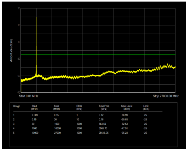
Band41 QPSK BW=20MHz Channel=41490 RB Size=1 Position=#0
