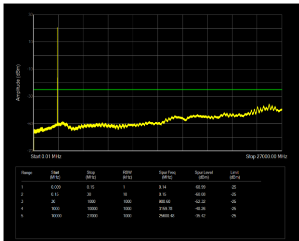
Band38 QPSK BW=10MHz Channel=37800 RB Size=1 Position=#0
