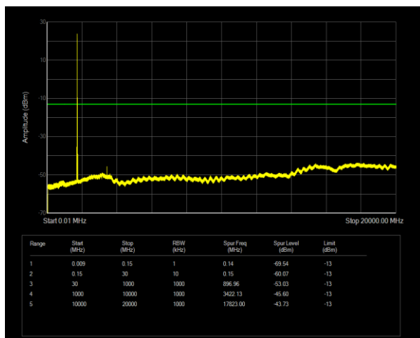
Band66 QPSK BW=20MHz Channel=132072 RB Size=1 Position=#0
