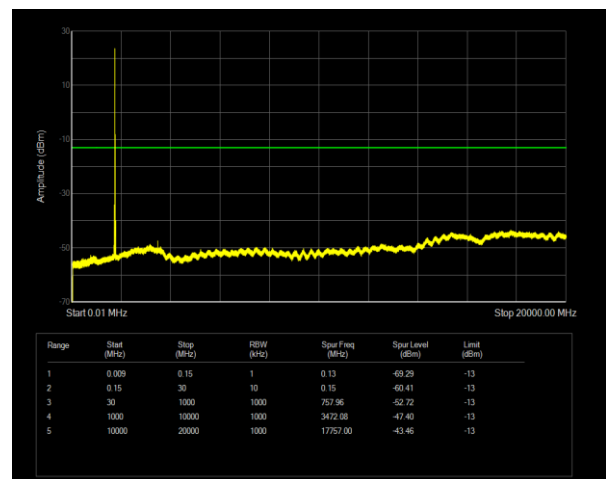
Band66 QPSK BW=20MHz Channel=132322 RB Size=1 Position=#0
