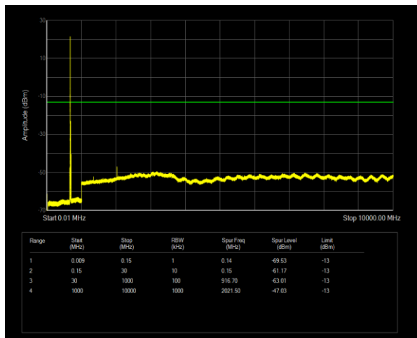
Band71 QPSK BW=15MHz Channel=133297 RB Size=1 Position=#0
