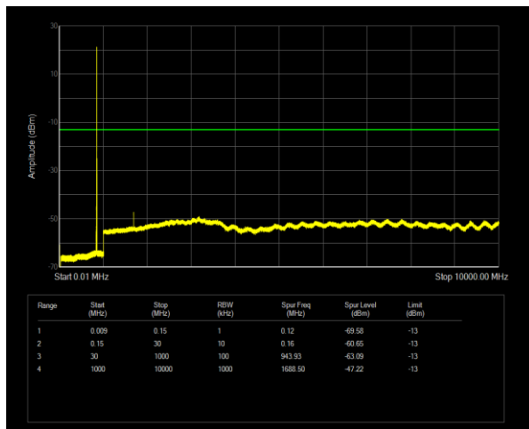
Band26(824-849) QPSK BW=5MHz Channel=27015 RB Size=1 Position=#0
