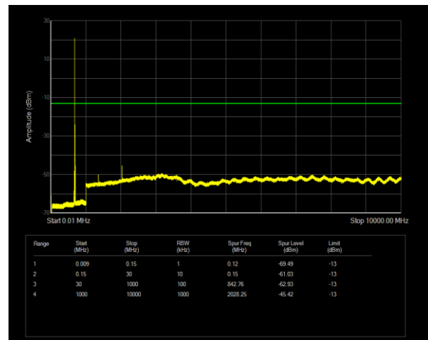
Band71 QPSK BW=10MHz Channel=133297 RB Size=1 Position=#0
