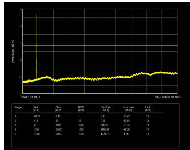
Band66 QPSK BW=5MHz Channel=132647 RB Size=1 Position=#0
