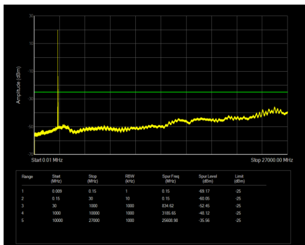
Band41 QPSK BW=20MHz Channel=39750 RB Size=1 Position=#0
