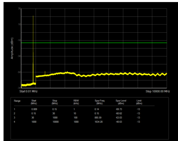
Band26(814-824) QPSK BW=5MHz Channel=26740 RB Size=1 Position=#0
