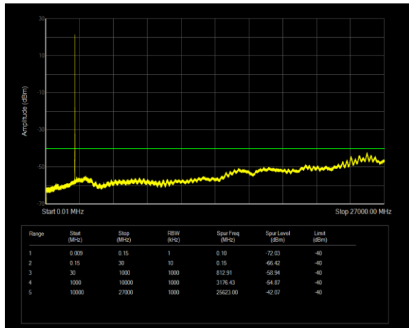
Band30 QPSK BW=5MHz Channel=27685 RB Size=1 Position=#0
