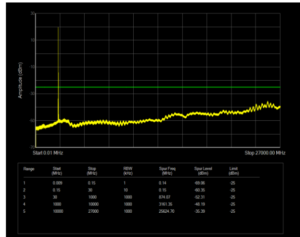
Band41 QPSK BW=15MHz Channel=39725 RB Size=1 Position=#0
