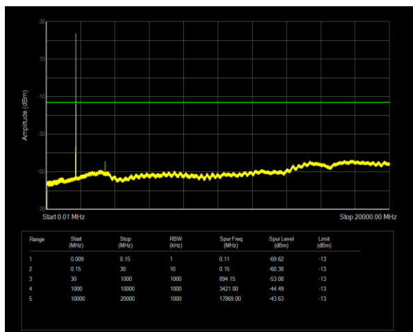
Band66 QPSK BW=10MHz Channel=132022 RB Size=1 Position=#0
