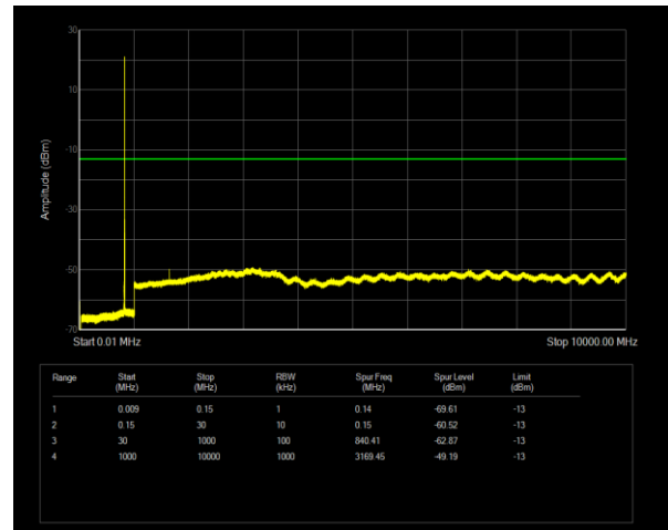
Band26(814-824) QPSK BW=3MHz Channel=26775 RB Size=1 Position=#0
