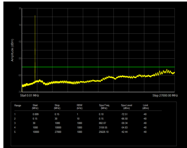
Band30 QPSK BW=5MHz Channel=27710 RB Size=1 Position=#0
