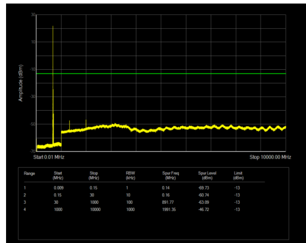
Band71 QPSK BW=15MHz Channel=133197 RB Size=1 Position=#0
