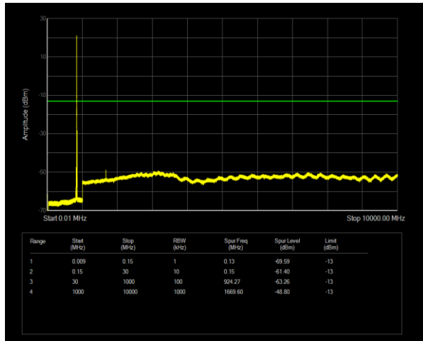
Band26(824-849) QPSK BW=15MHz Channel=26965 RB Size=1 Position=#0
