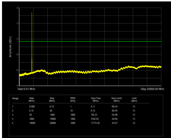
Band66 QPSK BW=10MHz Channel=132622 RB Size=1 Position=#0
