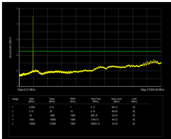
Band38 QPSK BW=5MHz Channel=38000 RB Size=1 Position=#0
