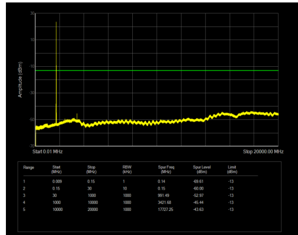
Band66 QPSK BW=15MHz Channel=132047 RB Size=1 Position=#0
