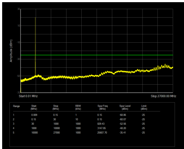
Band41 QPSK BW=5MHz Channel=40620 RB Size=1 Position=#0
