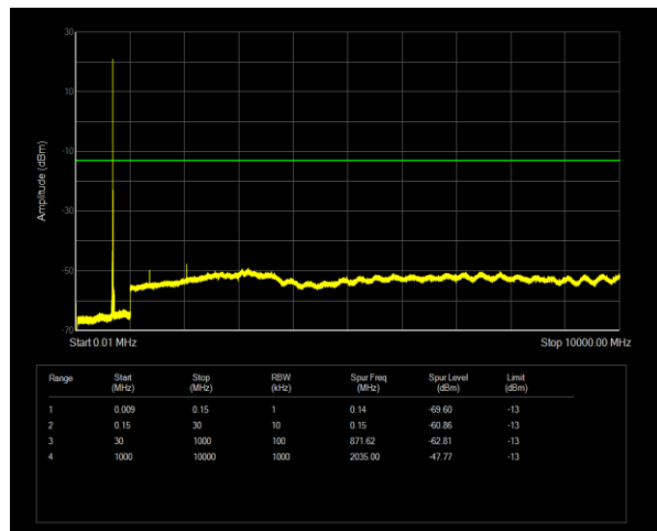
Band71 QPSK BW=5MHz Channel=133297 RB Size=1 Position=#0
