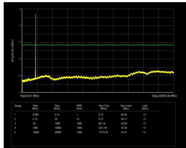
Band66 QPSK BW=15MHz Channel=132597 RB Size=1 Position=#0
