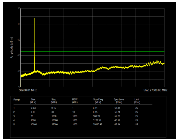
Band41 QPSK BW=10MHz Channel=40620 RB Size=1 Position=#0
