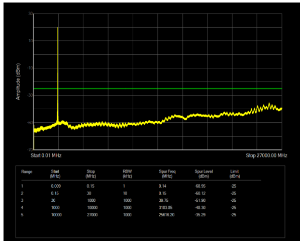
Band38 QPSK BW=20MHz Channel=38150 RB Size=1 Position=#0
