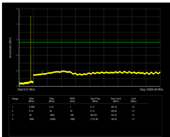
Band26(814-824) QPSK BW=1.4MHz Channel=26783 RB Size=1 Position=#0
