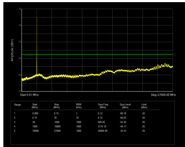
Band41 QPSK BW=5MHz Channel=41565 RB Size=1 Position=#0
