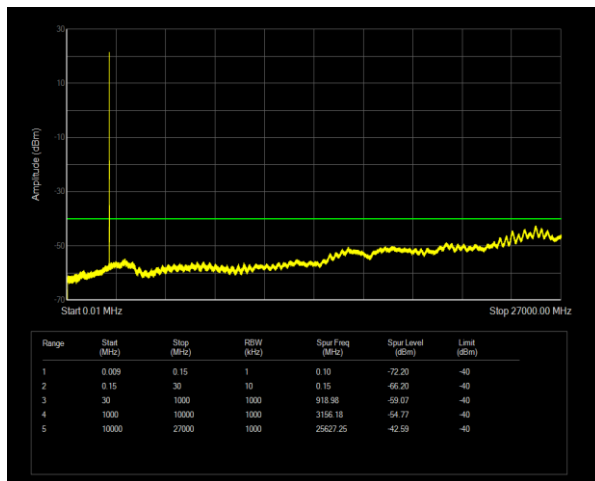
Band30 QPSK BW=5MHz Channel=27735 RB Size=1 Position=#0
