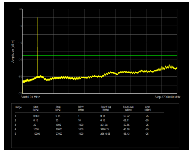
Band38 QPSK BW=5MHz Channel=37775 RB Size=1 Position=#0
