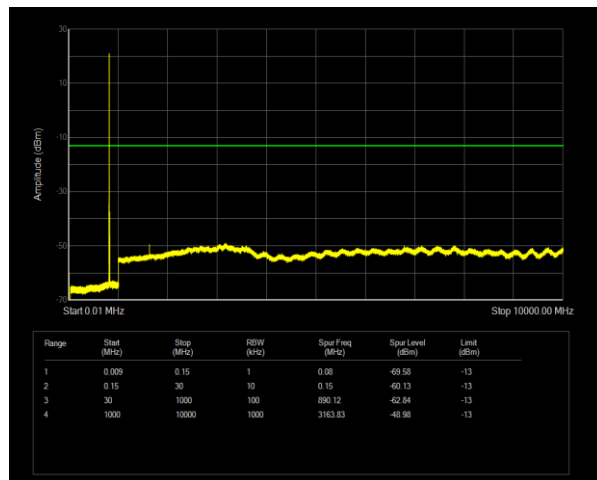
Band26(814-824) QPSK BW=5MHz Channel=26715 RB Size=1 Position=#0
