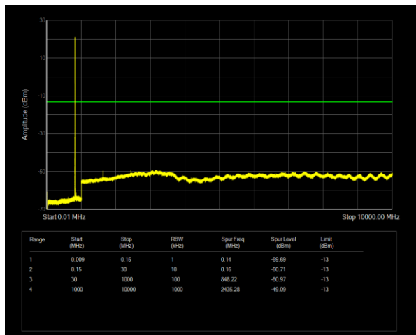
Band26(814-824) QPSK BW=1.4MHz Channel=26697 RB Size=1 Position=#0
