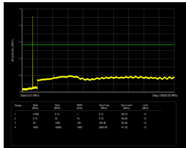
Band71 QPSK BW=5MHz Channel=133447 RB Size=1 Position=#0
