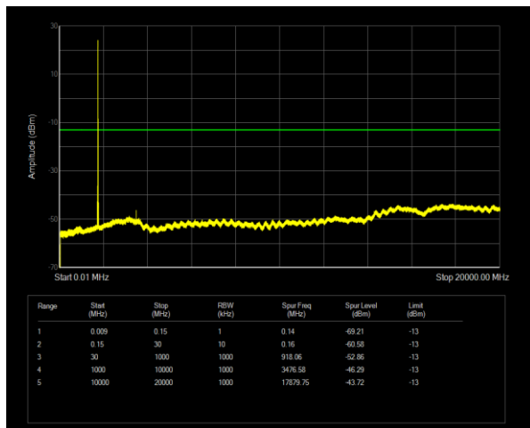
Band66 QPSK BW=15MHz Channel=132322 RB Size=1 Position=#0
