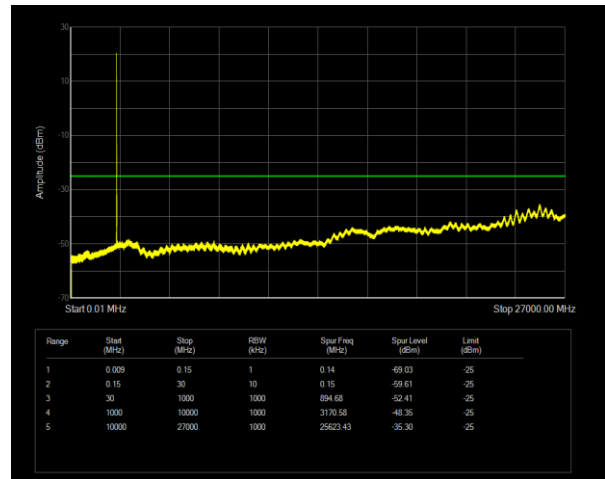
Band41 QPSK BW=5MHz Channel=39675 RB Size=1 Position=#0
