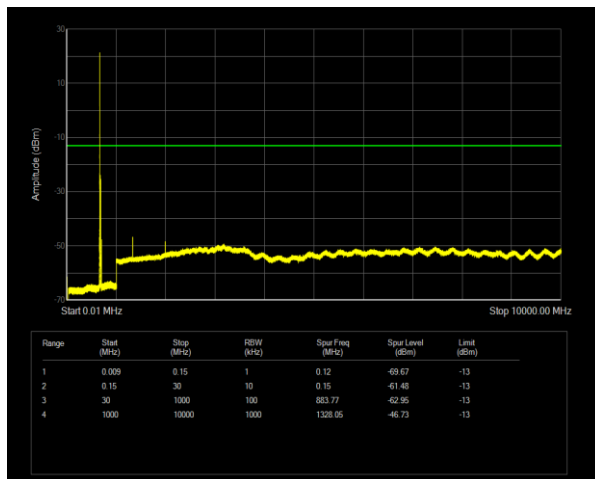
Band71 QPSK BW=20MHz Channel=133222 RB Size=1 Position=#0
