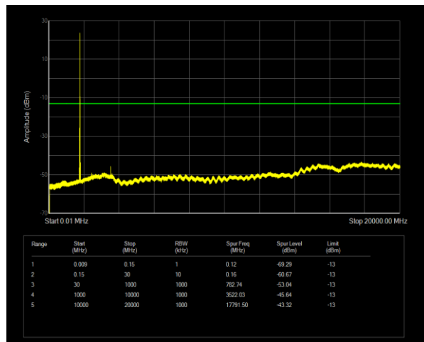
Band66 QPSK BW=20MHz Channel=132572 RB Size=1 Position=#0
