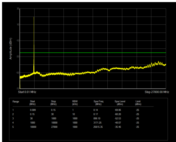
Band38 QPSK BW=15MHz Channel=38000 RB Size=1 Position=#0
