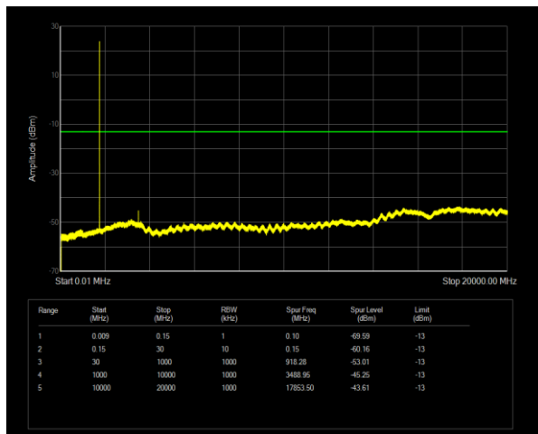
Band66 QPSK BW=1.4MHz Channel=132322 RB Size=1 Position=#0
