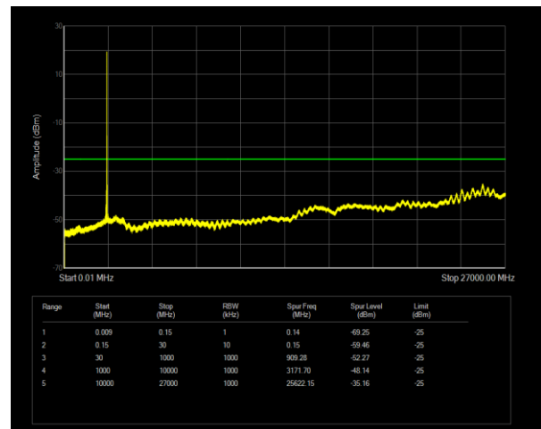
Band38 QPSK BW=15MHz Channel=38175 RB Size=1 Position=#0
