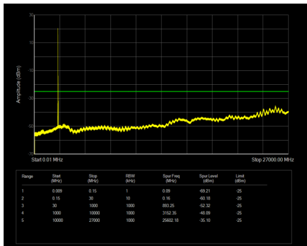
Band41 QPSK BW=10MHz Channel=39700 RB Size=1 Position=#0
