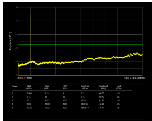
Band38 QPSK BW=5MHz Channel=38225 RB Size=1 Position=#0
