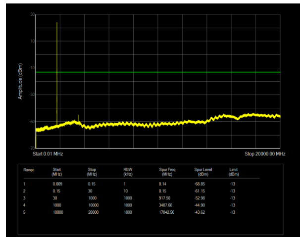
Band66 QPSK BW=3MHz Channel=132322 RB Size=1 Position=#0
