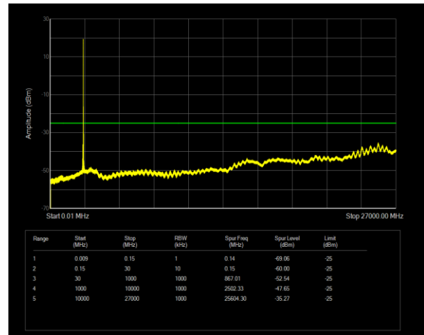
Band38 QPSK BW=15MHz Channel=37825 RB Size=1 Position=#0
