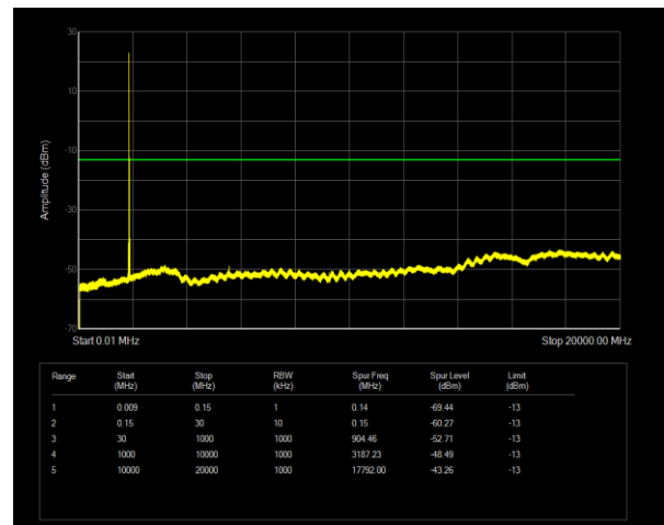
Band25 QPSK BW=20MHz Channel=26140 RB Size=1 Position=#0
