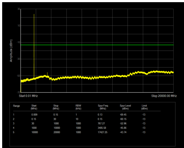
Band66 QPSK BW=5MHz Channel=132322 RB Size=1 Position=#0
