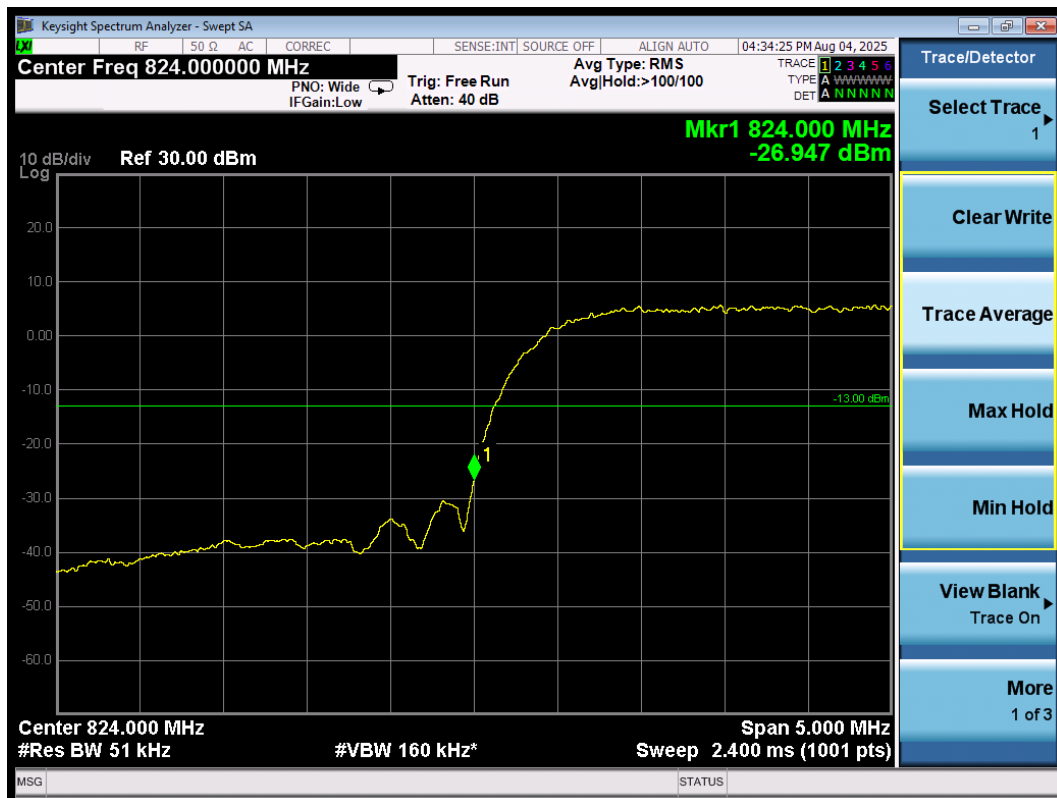
Band edge\B5\L
