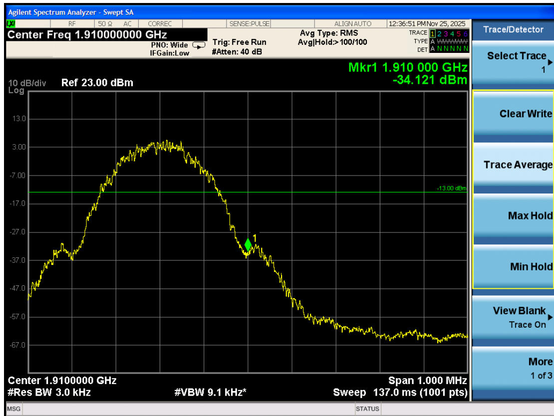
Band edge\GSM1900 H
