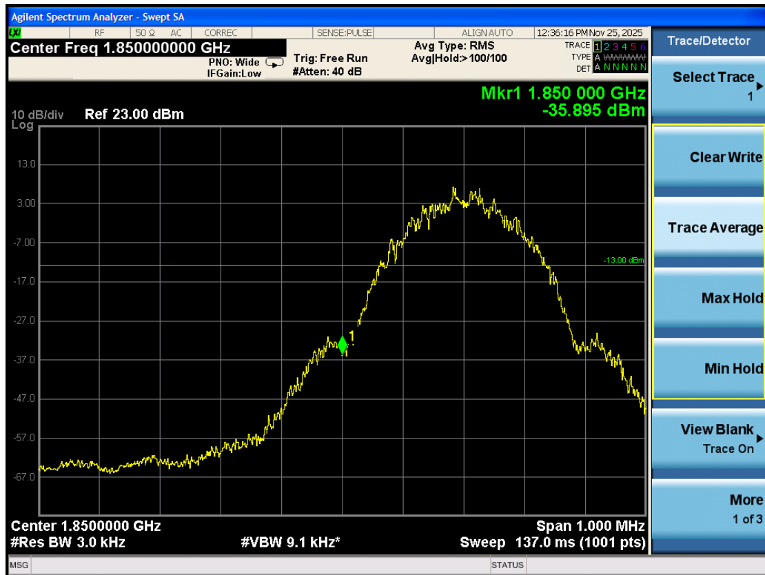
Band edge\GSM1900 L
