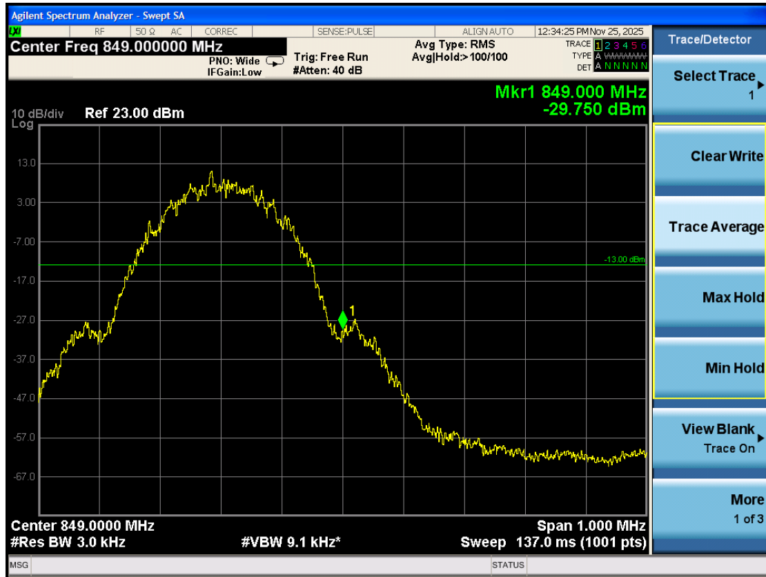
Band edge\GSM850 H
