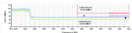
802.11ax HE40-Channel 46: Peak + Average
