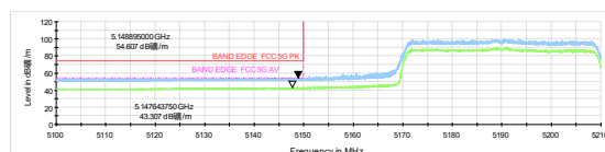
802.11ax HE40-Channel 38: Peak + Average
