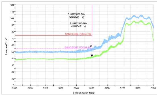
802.11a-Channel 36: Peak + Average
